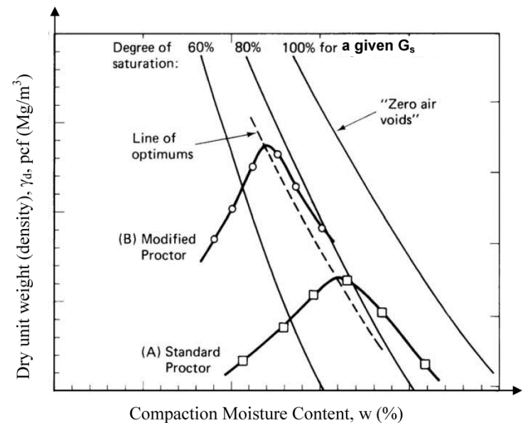
Figure 5-31. Compaction curves (after Holtz and Kovacs, 1981).
