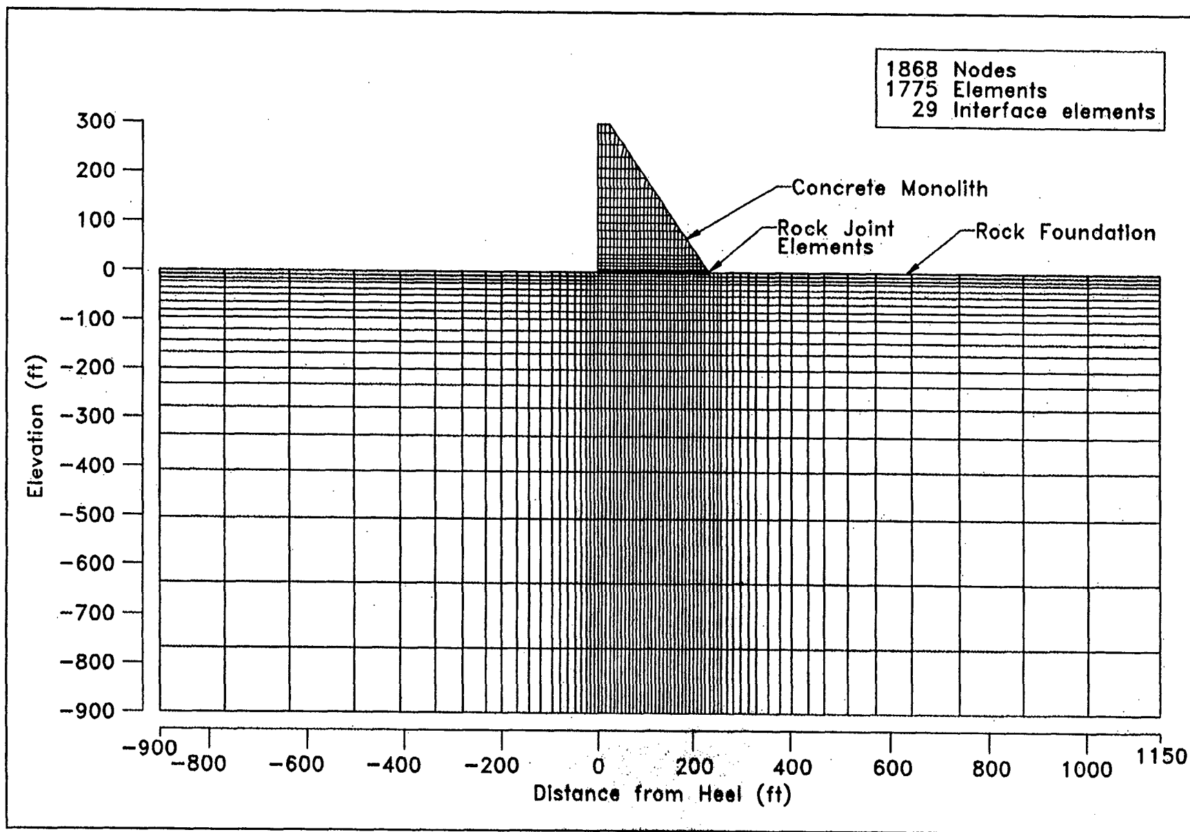
Figure 78. Finite element mesh used in analyses (1 ft = 0.305 m)
