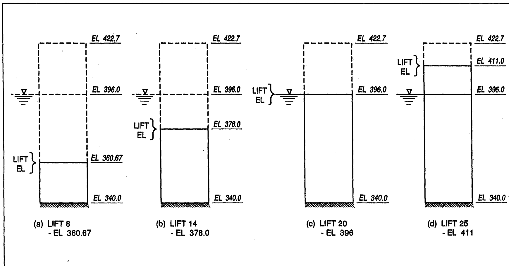
Figure B3. Four lift stages of the backfill placement analysis used in the evaluation
