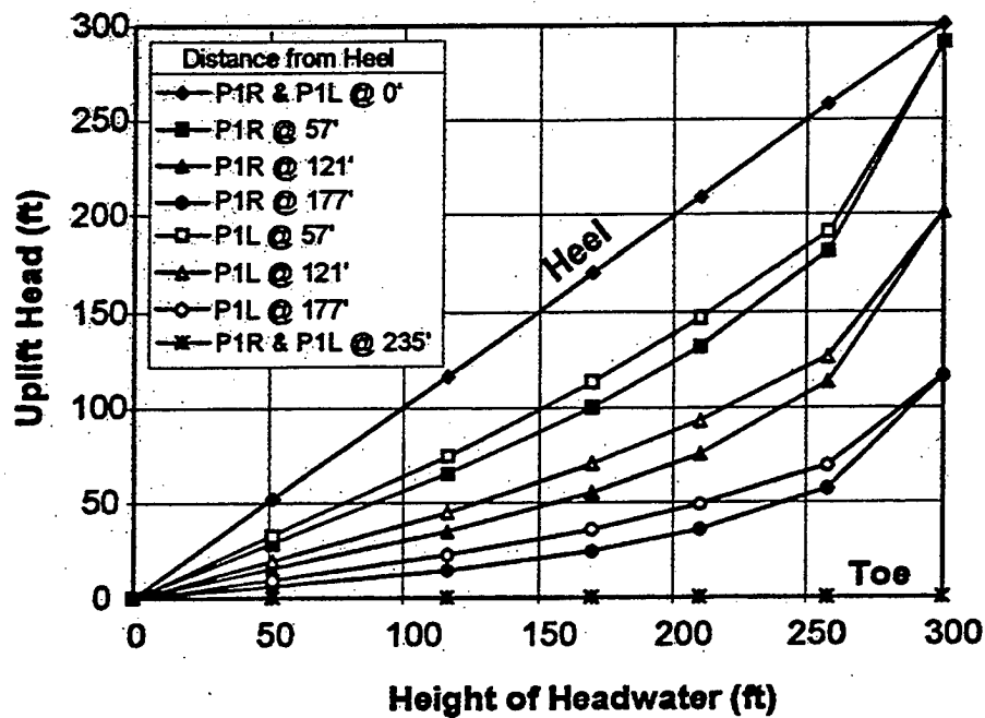
(a) Variation of uplift head for Pool 1
