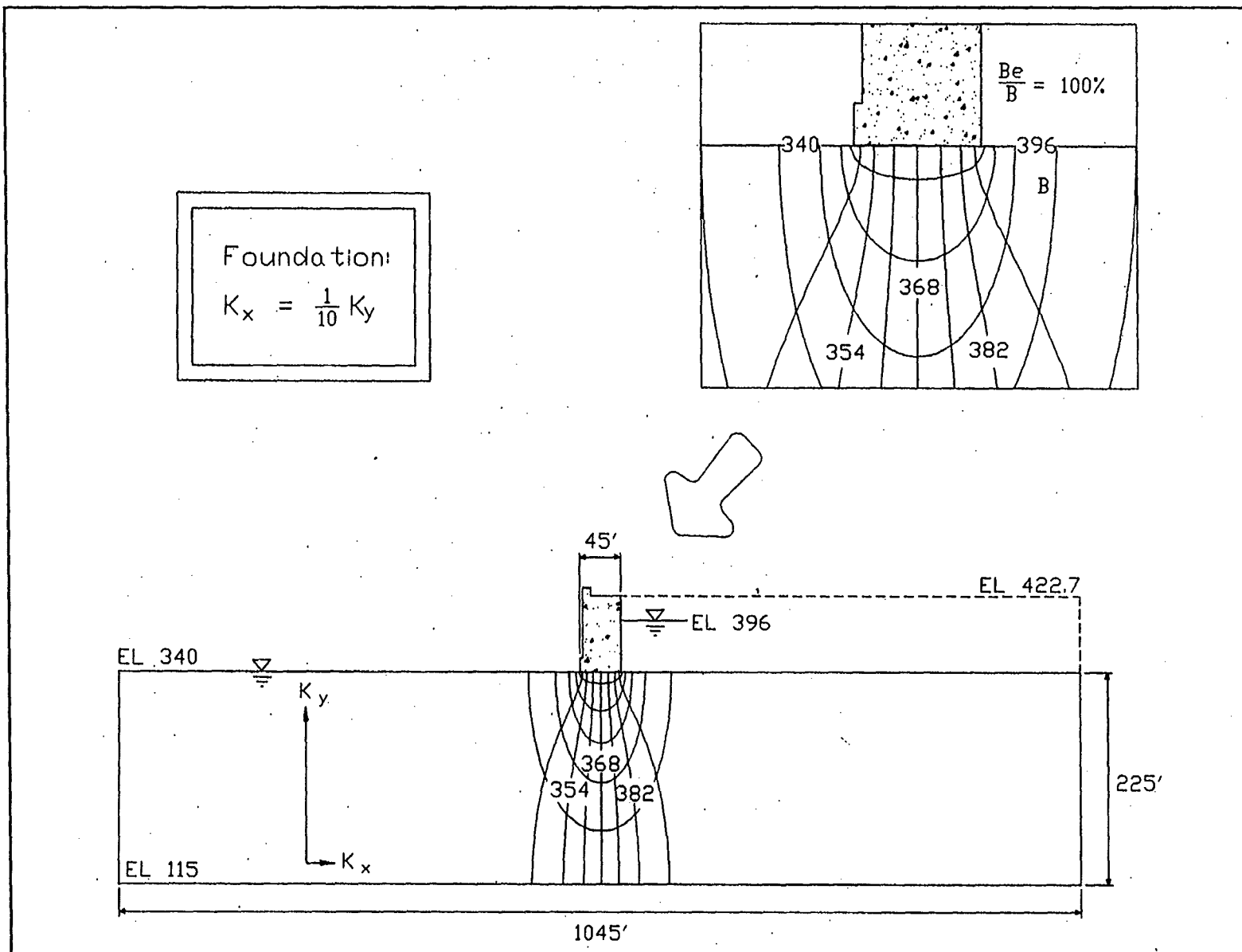
Figure 56. Results for B_e/B = 100 percent, K_x = 1/10 K_y (1 ft = 0.305 m)
