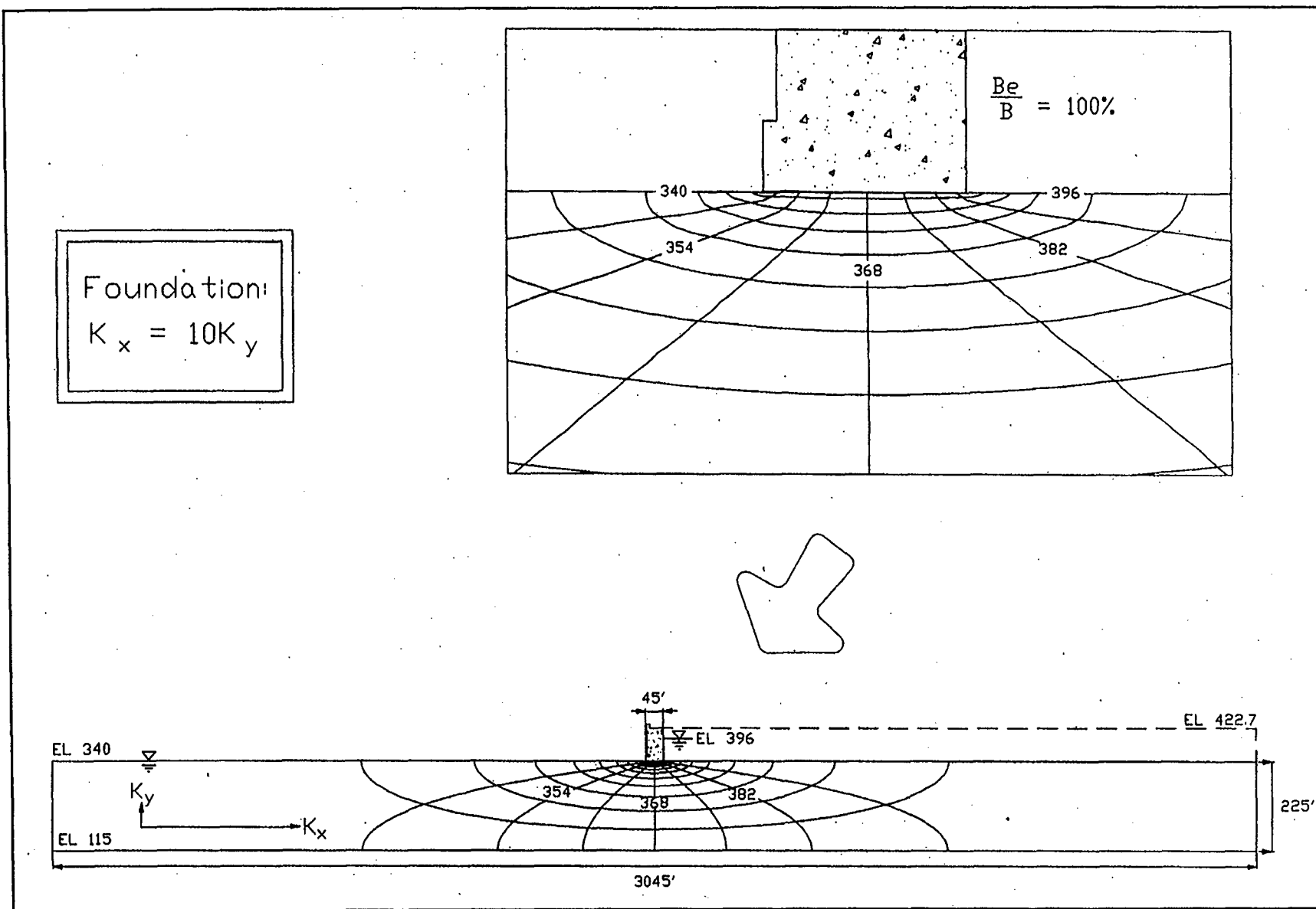
Figure 55. Results for B_e/B = 100 percent, K_x = 10K_y (1 ft = 0.305 m)
