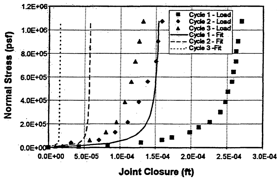
(a) Fit of experimental data using Bandis' equations for V_m and K_{ni}
