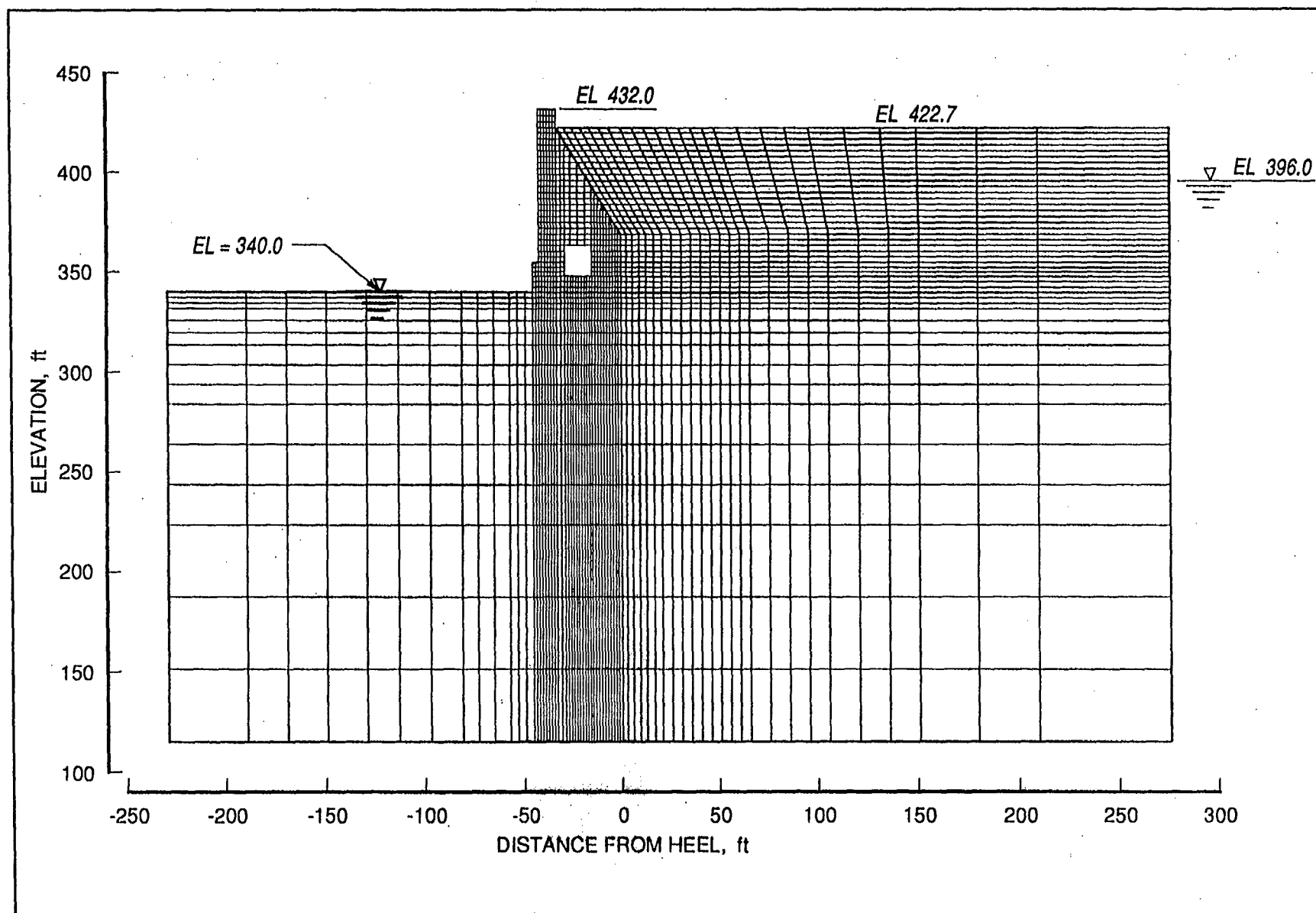
Figure 38. Finite element mesh of Locks 27 Monolith 7E, SOILSTRUCT-ALPHA backfill placement analysis (1 ft = 0.305 m)
