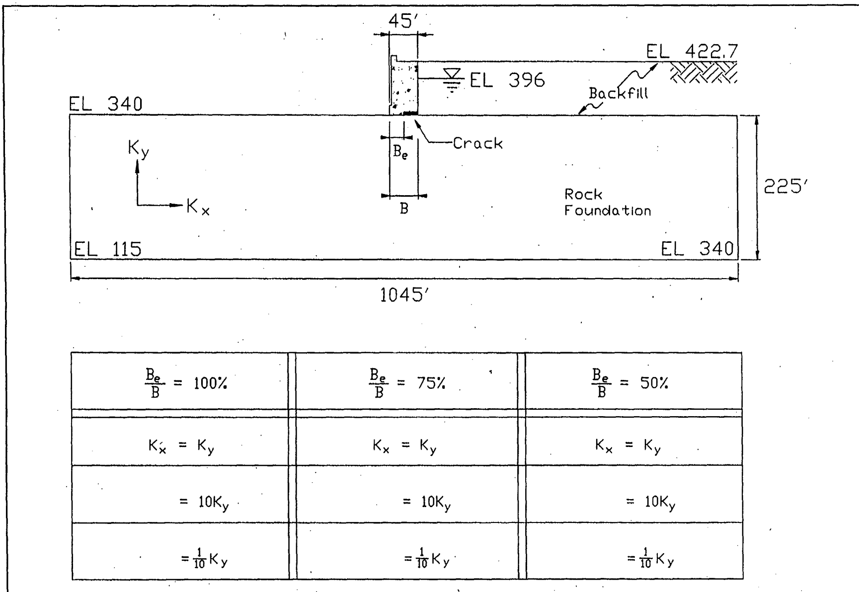
Figure 53. Problem geometry and cases considered (1 ft = 0.305 m)
