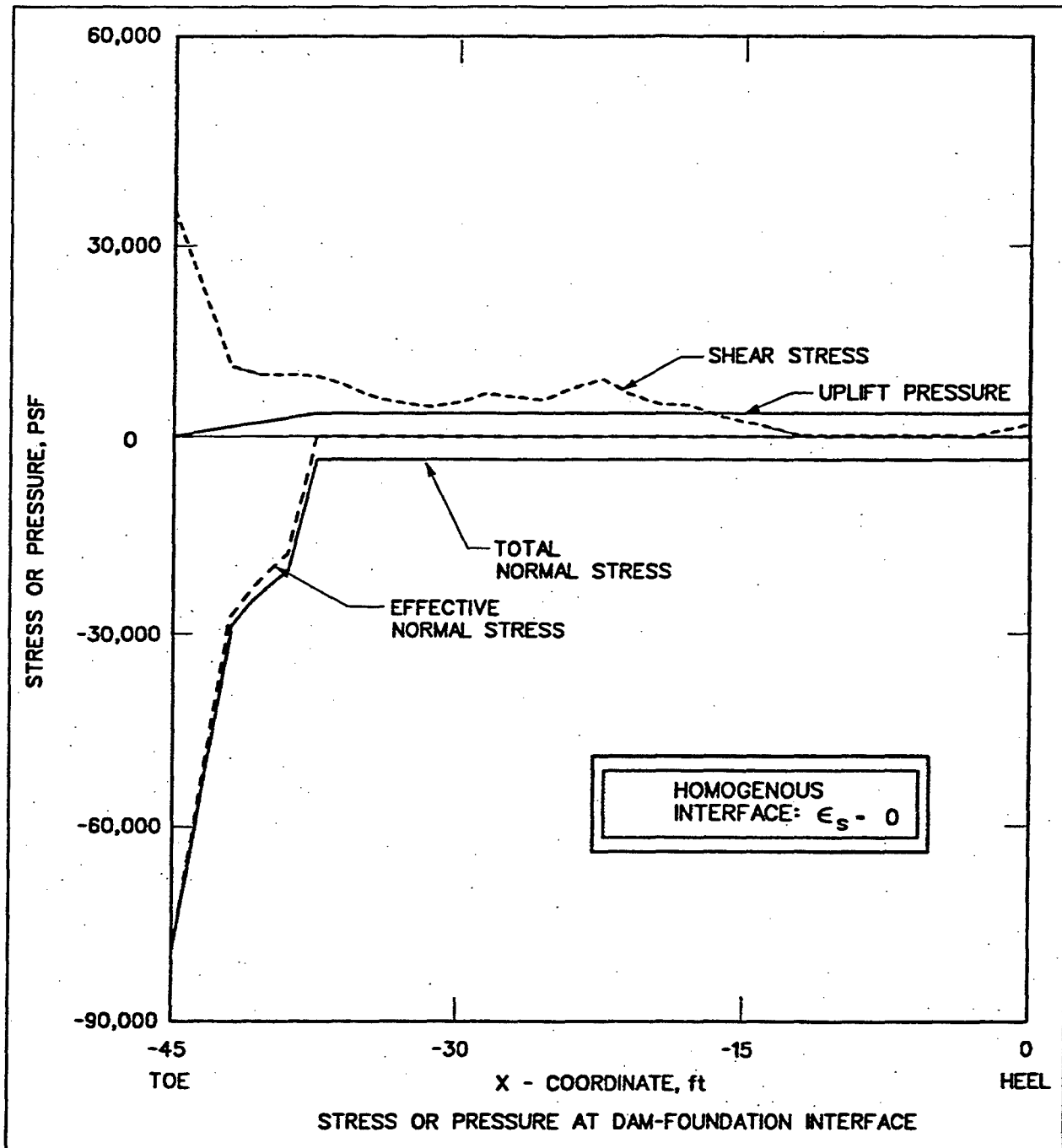
Figure 21. Stress profiles along interface of Locks 27 - homogeneous fracture criteria (1 ft = 0.305 m, 1 MPa = 20,885.5 psf)
