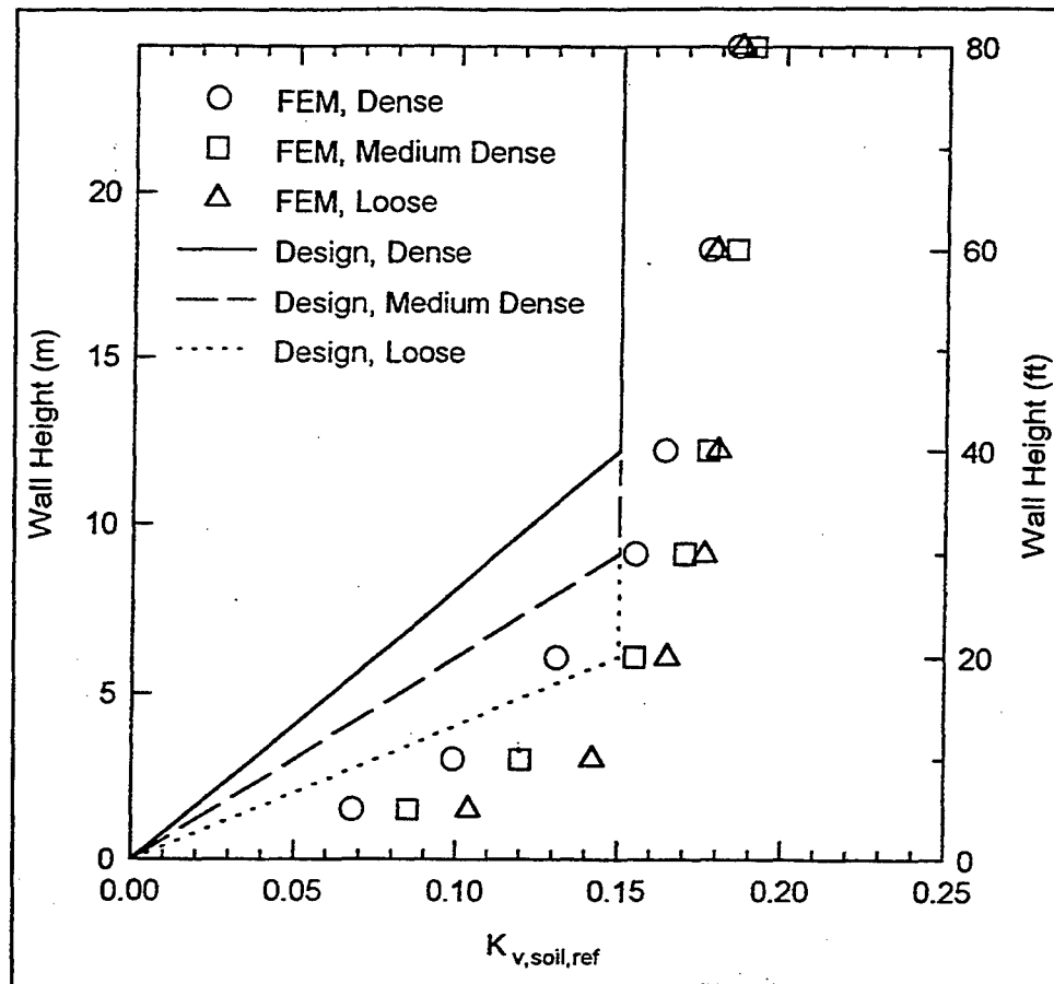
Figure 35. Values of K_{v, \text{soil}, \text{ref}} recommended for design (1 ft = 0.305 m)
