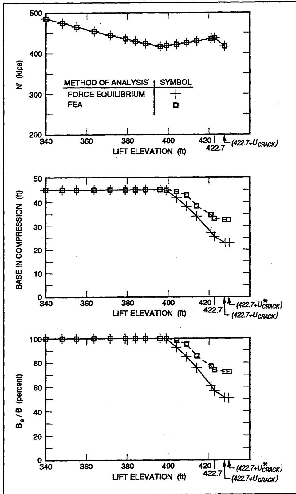
Figure A16. Variations in values of N' , B_o , and B_o/B from results of conventional force equilibrium and finite element analyses (1 ft = 0.305 m, 1 kip = 4.448 kN)
