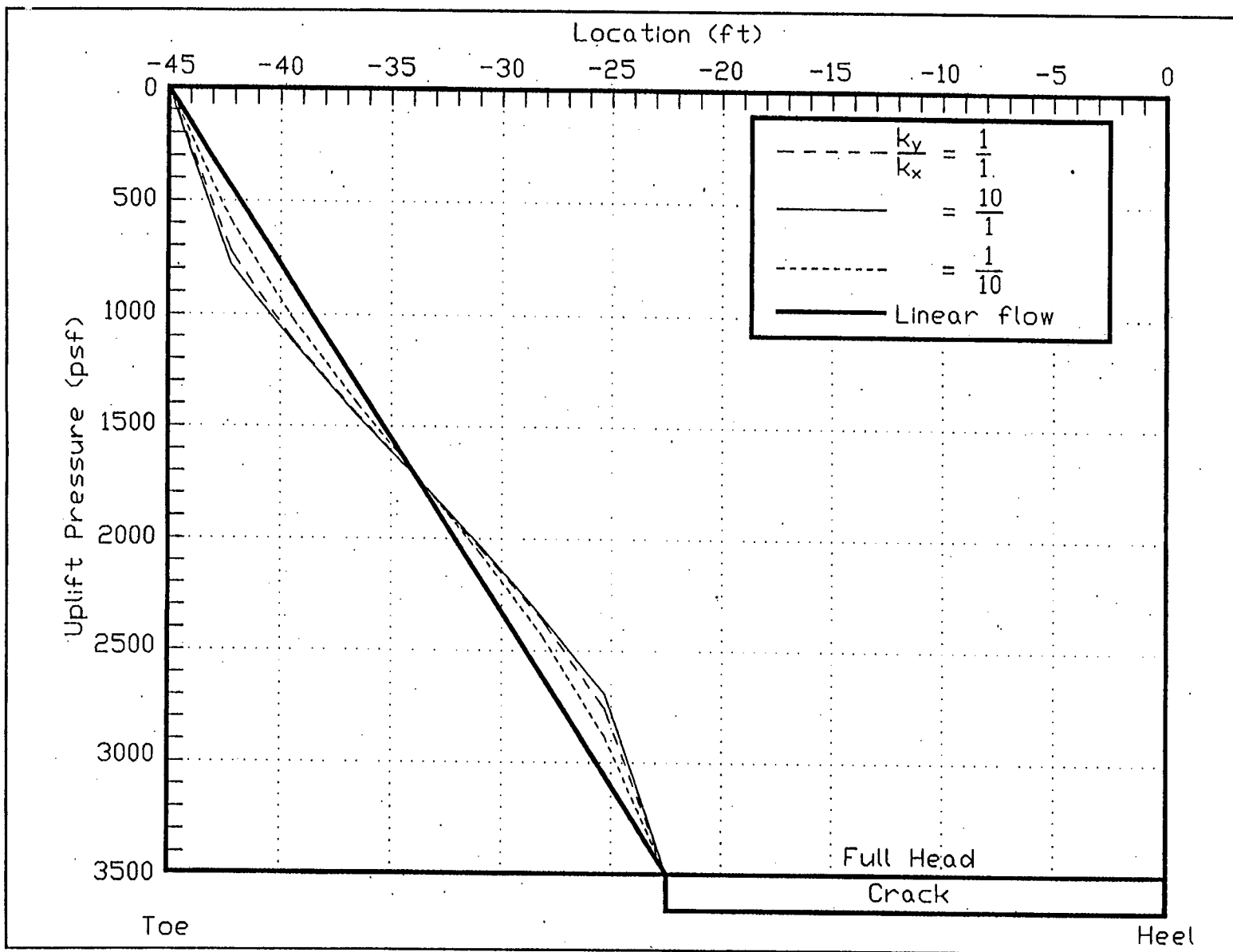
91 Figure 61. Uplift values for B_y/B = 50 percent (1 ft = 0.305 m, 1 MPa = 20,885.5 psf)
