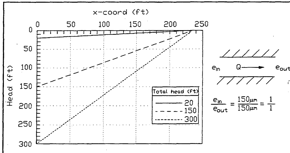
Figure 47. Variation in head along rock joint, e_{in}/e_{out} = 1 (1 ft = 0.305 m)
