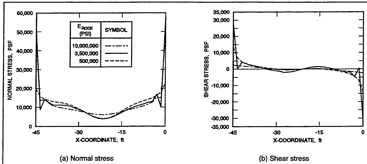
Figure 29. Variation of initial stress distributions along the base for different E_{\text{ROCK}} (1 ft = 0.305 m, 1 MPa = 20,885.5 psf)
