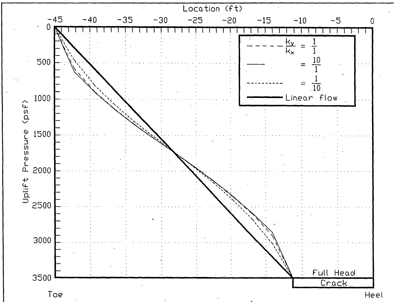
Figure 60. Uplift values for B_y/B = 75 percent (1 ft = 0.305 m, 1 MPa = 20,885.5 psf)
