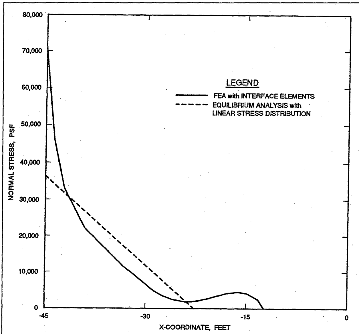
Figure 12. Normal stress distributions along the base of Monolith 7E (1 ft = 0.305 m, 1 MPa = 20,885.5 psf)
