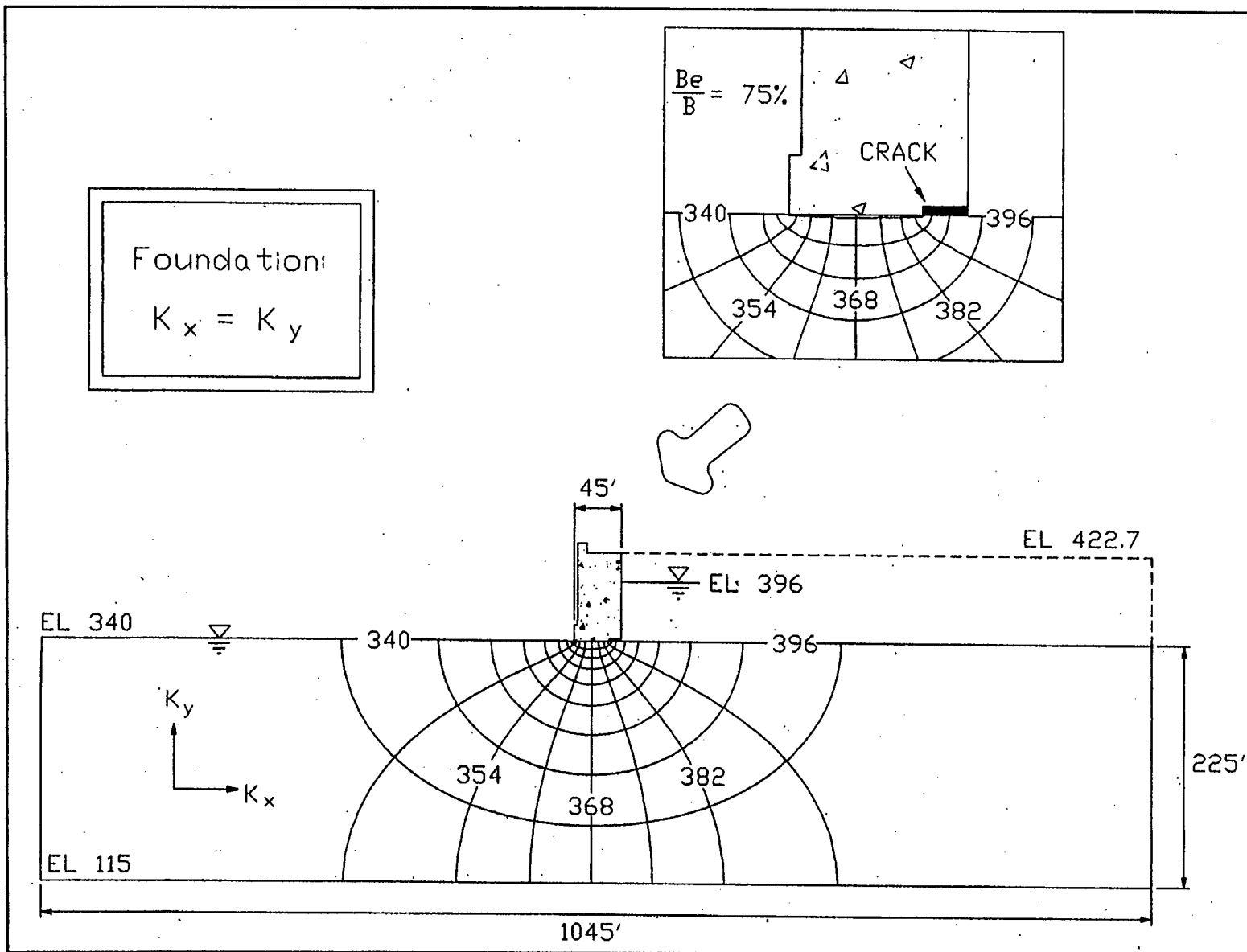
87 Figure 57. Results for B_e/B = 75 percent, K_x = K_y (1 ft = 0.305 m)
