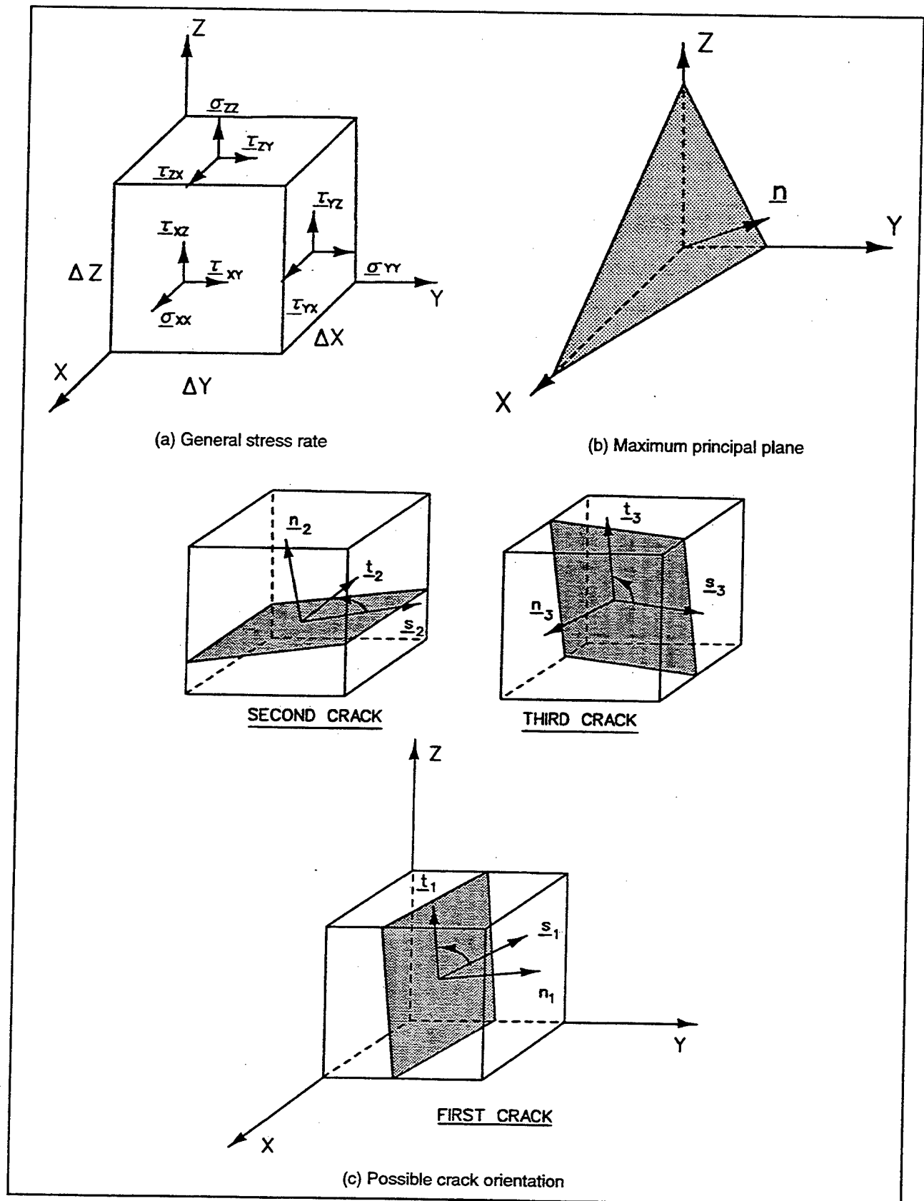
Figure 15. Smeared crack model used in CG-DAMS
