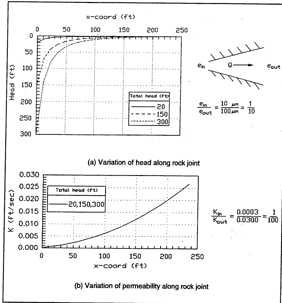
Figure 51. Head and permeability variation along rock joint, e_{in}/e_{out} = 1/10 (1 ft = 0.305 m, 1 ft/s = 0.305 m/s)
