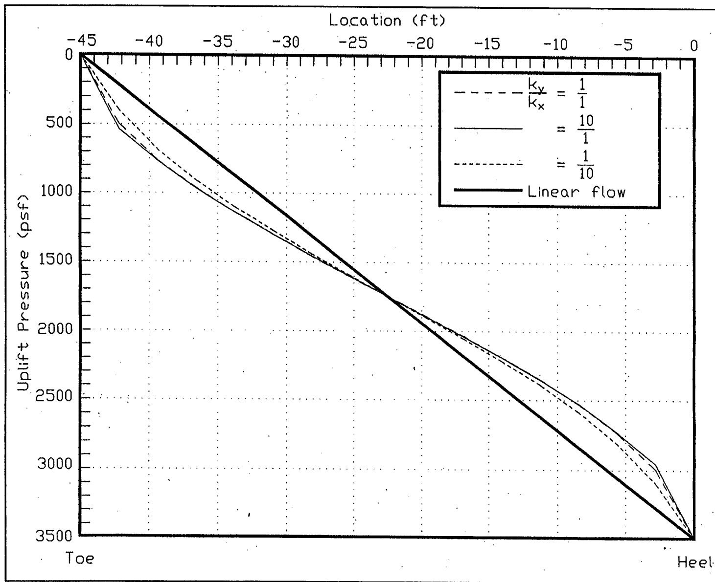
68 Figure 59. Uplift values for B_y/B = 100 percent (1 ft = 0.305 m, 1 MPa = 20,885.5 psf)
