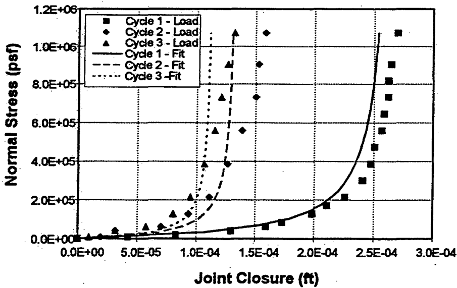
(b) Fit of experimental data using Bandis' equation for K_{ni} and values of V_m from experimentation
