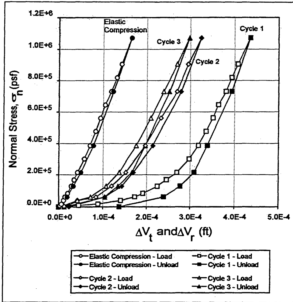
Figure 66. Laboratory results showing normal stress ( \sigma_n ) - total deformation ( \Delta V ) relationships for fresh dolerite under repeated loading cycles, and intact rock compression curves (after Bandis 1980) (1 ft = 0.305 m, 1 MPa = 20,885.5 psf)
