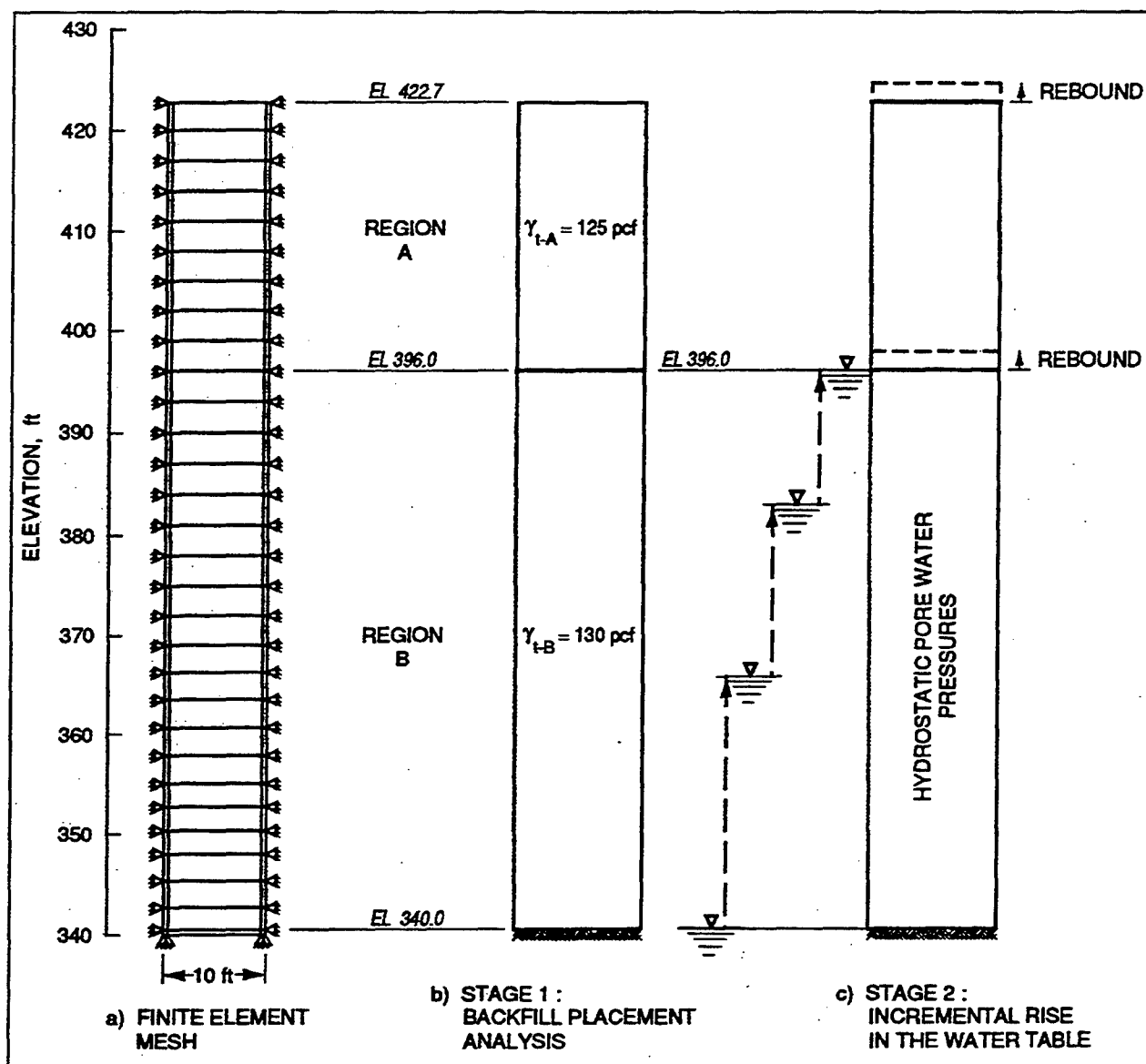
Figure H1. One-dimensional column analysis - postconstruction rise in the water table (1 ft = 0.305 m, 1 pcf = 16.018 kg/m 3 )
