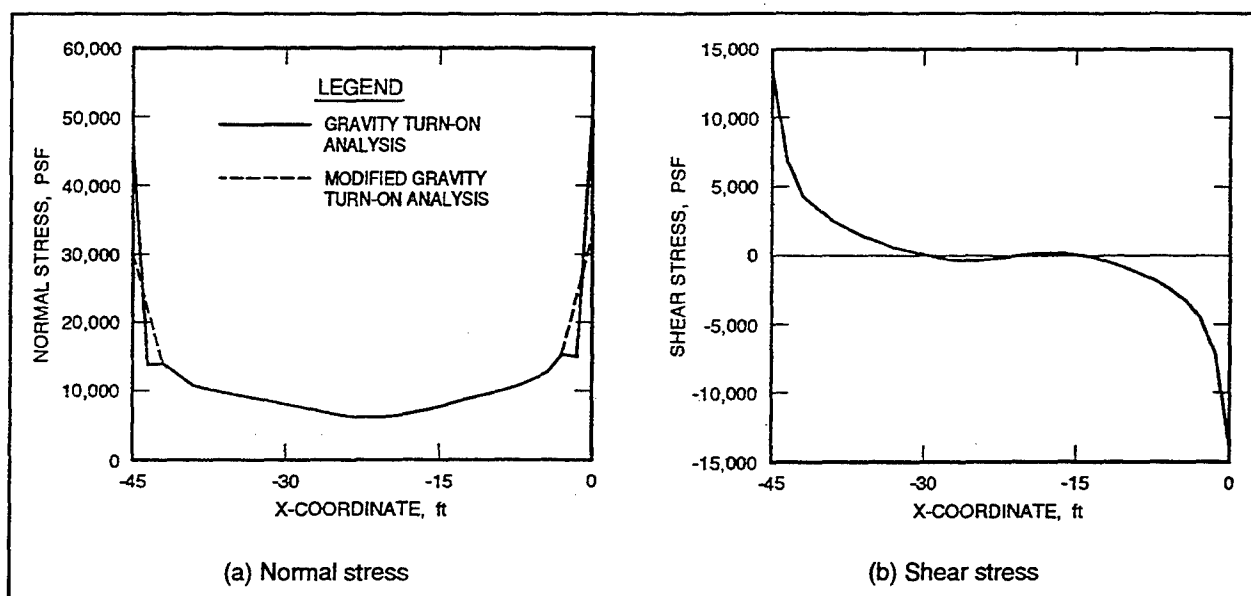
Figure 30. Initial stress distributions along the base - E_{\text{ROCK}} = 500,000 psi (1 ft = 0.305 m, 1 MPa = 20,885.5 psf)
