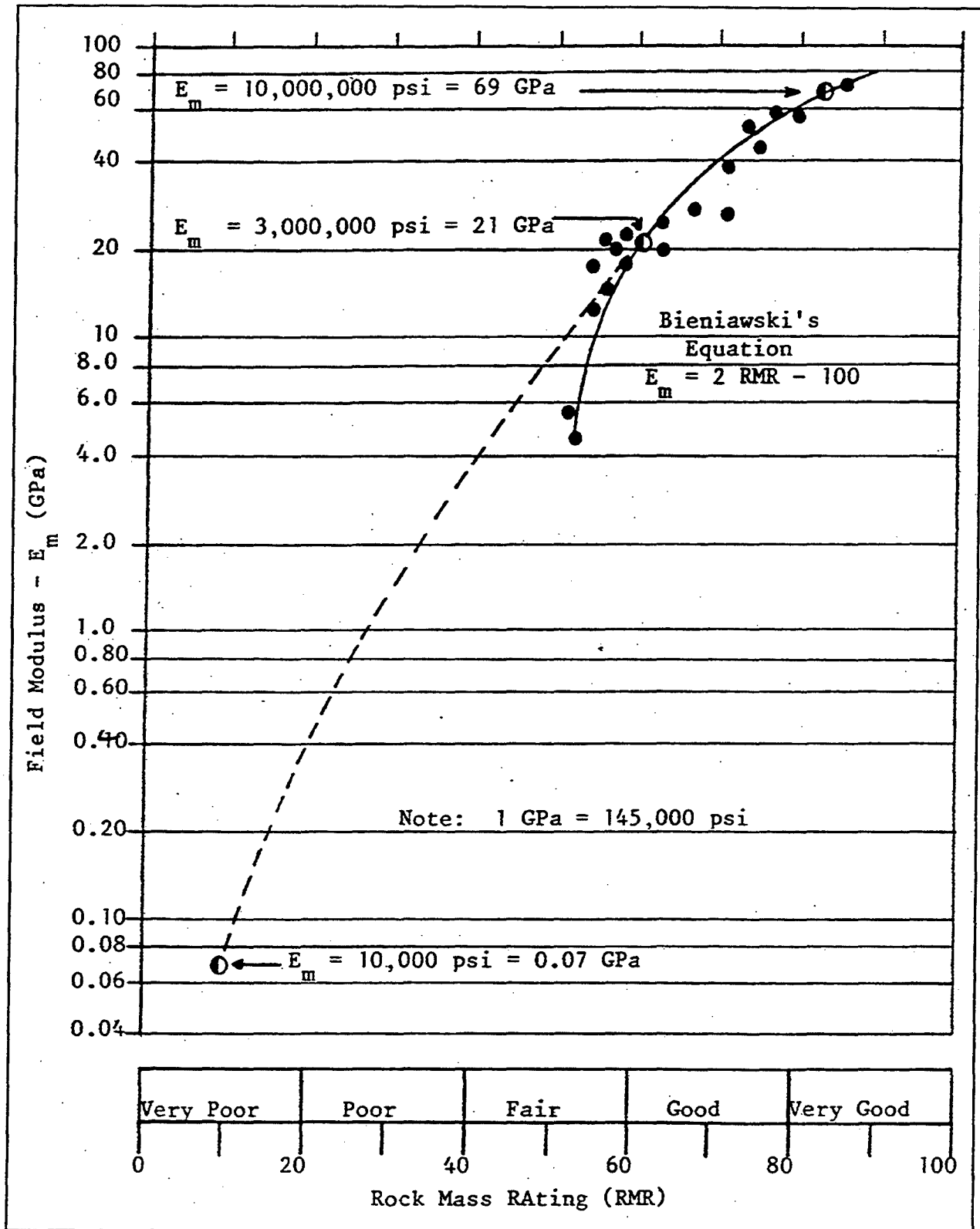
Figure 28. Relationship between rock modulus and rock mass rating (from Benson (1986), after Bieniawski (1978)) (1 MPa = 145.04 psi)
