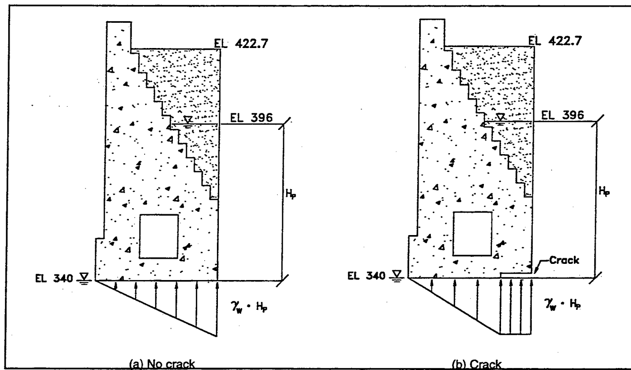
Figure 44. Empirical uplift water pressure distributions (from EM 1110-2-2200)
