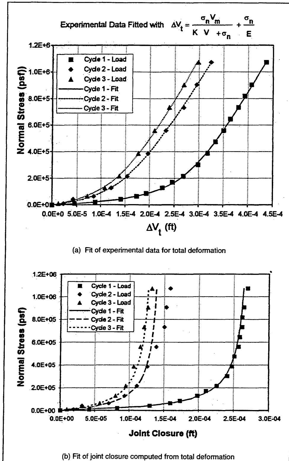
Figure 69. Fit of Bandis' experimental data for fresh dolerite (1 ft = 0.305 m, 1 MPa = 20,885.5 psf)
