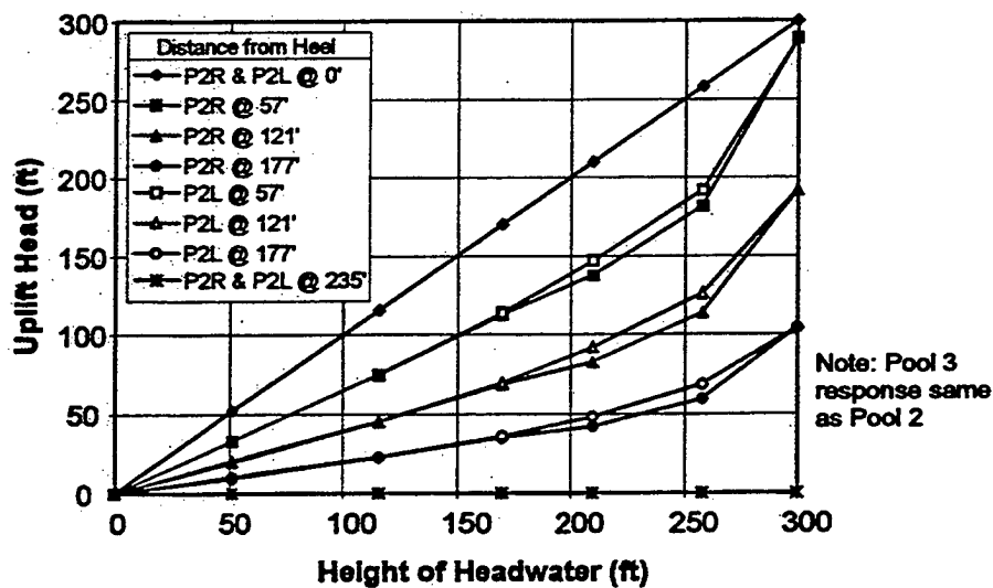
(b) Variation of uplift head at five locations along the joint headwater elevation
