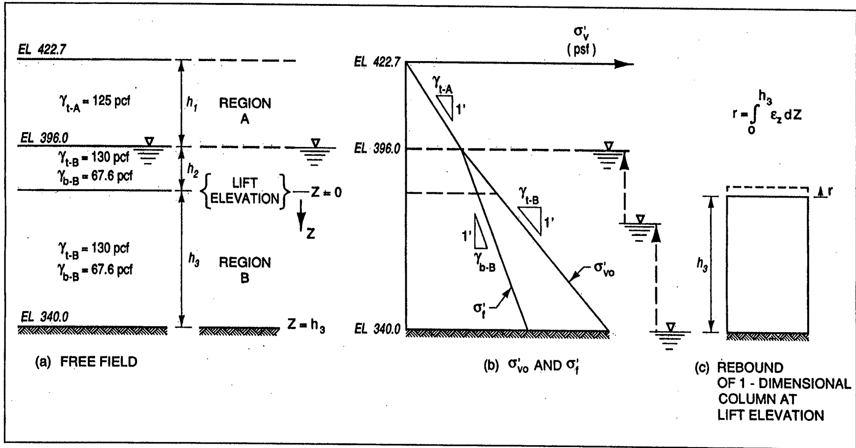
Figure H2. Lift elevation in region B with a postconstruction rise in the water table (1 ft = 0.305 m, 1 pcf = 16.018 kg/m 3 )
