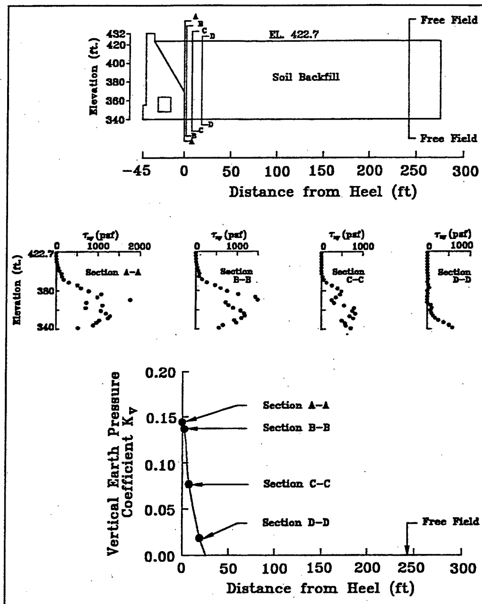
Figure 42. Variation of shear stress and vertical earth pressure coefficient with distance from the heel of Locks 27 Monolith 7E (1 ft = 0.305 m, 1 Mpa = 20,885.5 psf)
