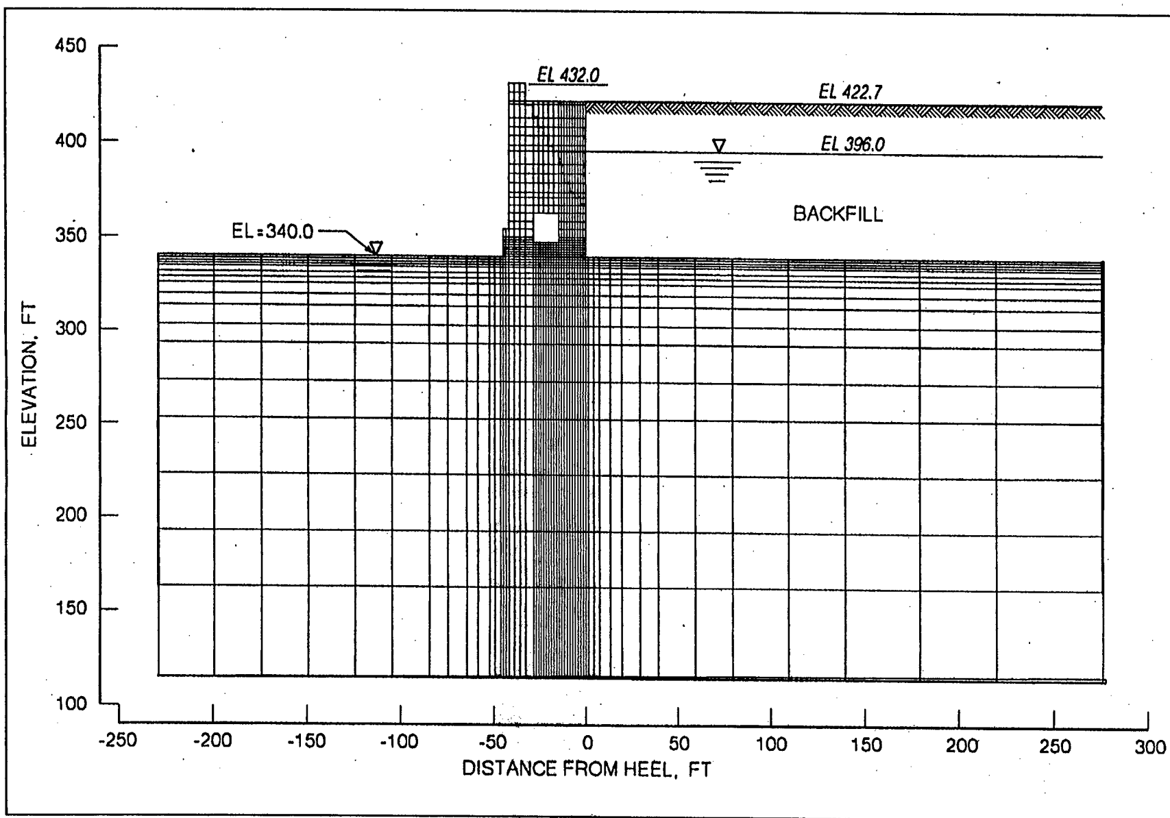
21 Figure 9. Finite element mesh of Locks 27 Monolith 7E - SOILSTRUCT-ALPHA following loads analyses (1 ft = 0.305 m) (Continued)
