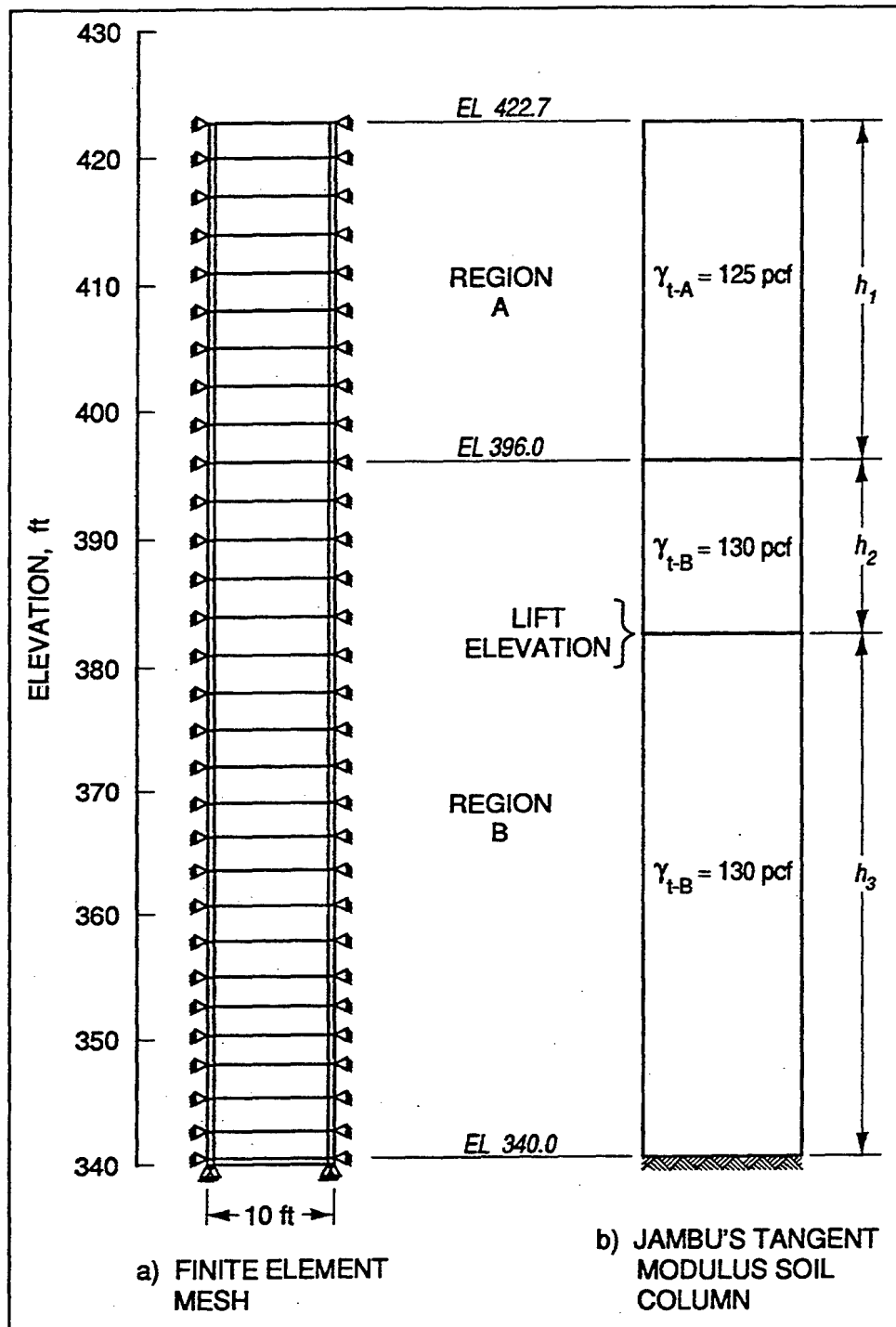
Figure G2. One-dimensional column analysis - lift elevation in region B (1 ft = 0.305 m, 1 pcf = 16.018 kg/m 3 )
