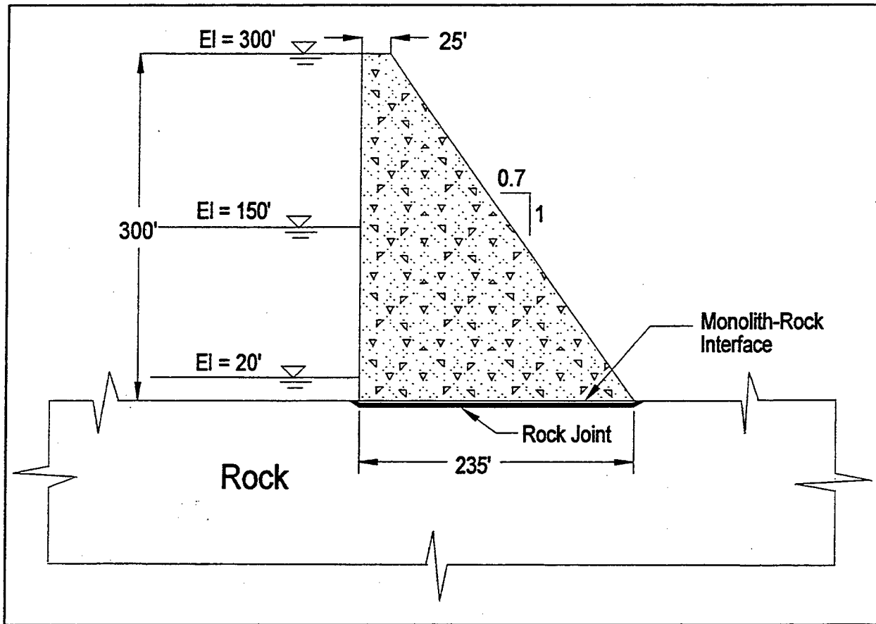
Figure 46. Geometry of dam used in study (1 ft = 0.305 m)
