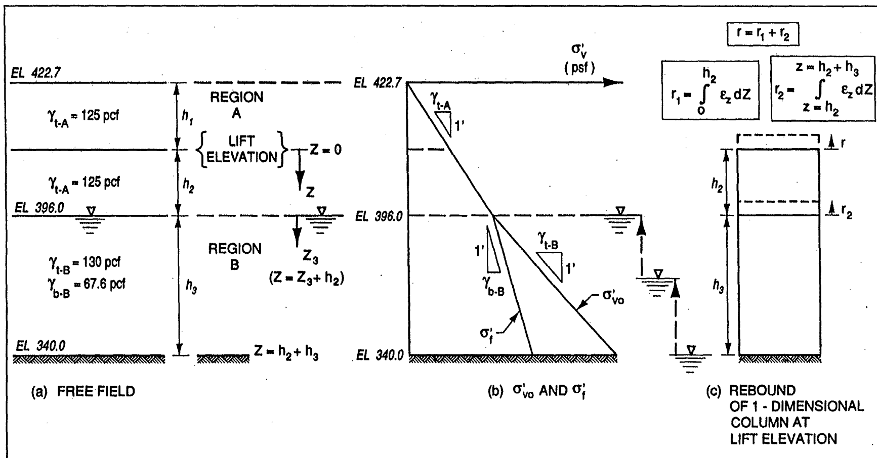
Figure H3. Lift elevation in region A with a postconstruction rise in the water table (1 ft = 0.305 m, 1 pcf = 16.018 kg/m 3 )
