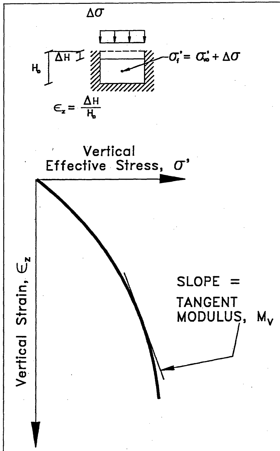
Figure D1. Nonlinear stress-strain relation typical for soils
