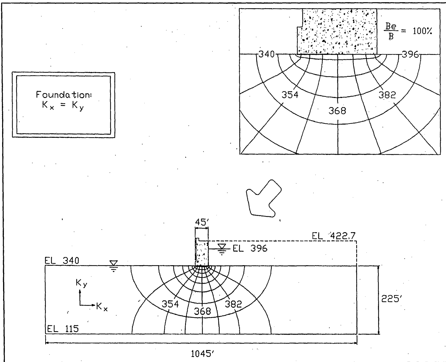
Figure 54. Results for B_e/B = 100 percent, K_x = K_y (1 ft = 0.305 m)
