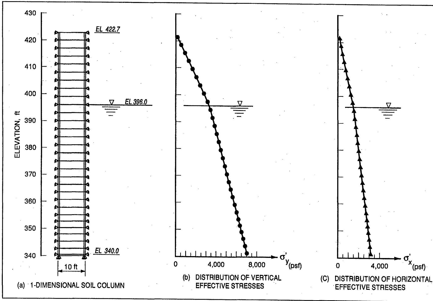
Figure B2. Results of 1-D soil column analysis using SOILSTRUCT (1 ft = 0.305 m, 1 MPa = 20,885.5 psf)
