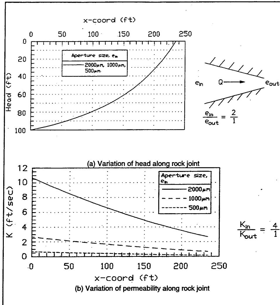
Figure 52. Head and permeability variation along rock joint, e_{in}/e_{out} = 2/1 , with varying e_m (1 ft = 0.305 m, 1 ft/s = 0.305 m/s)
