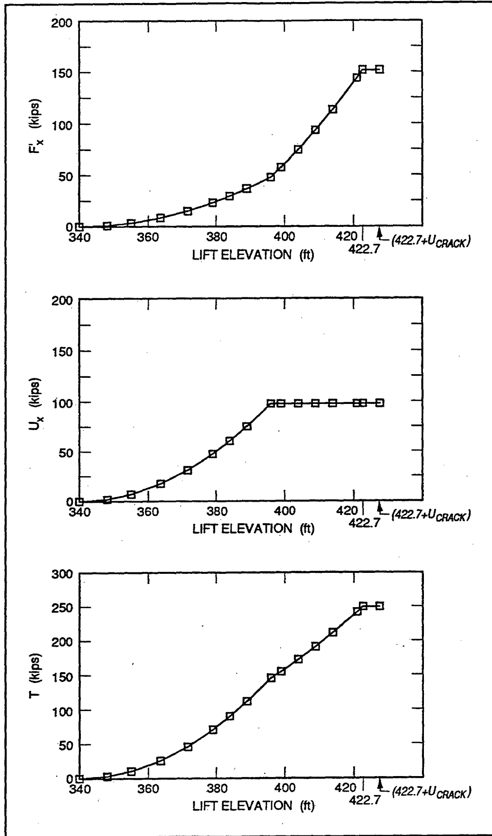
Figure A5. Variations in values of F'_x , U_x , and T with lift elevations (1 ft = 0.305 m, 1 kip = 4.448 kN)
