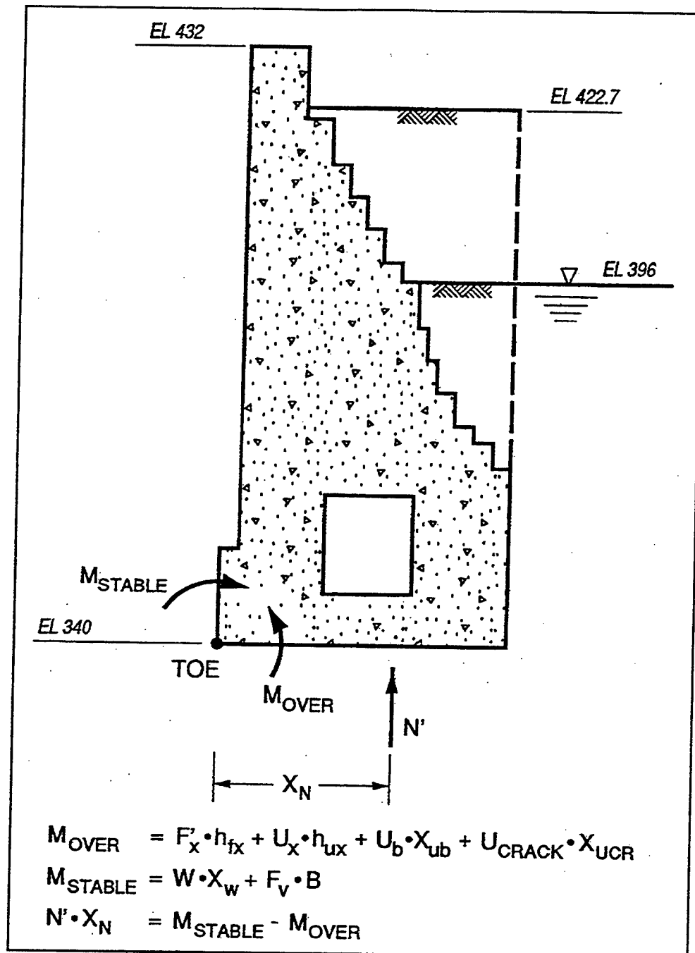
Figure 8. Moment equilibrium
