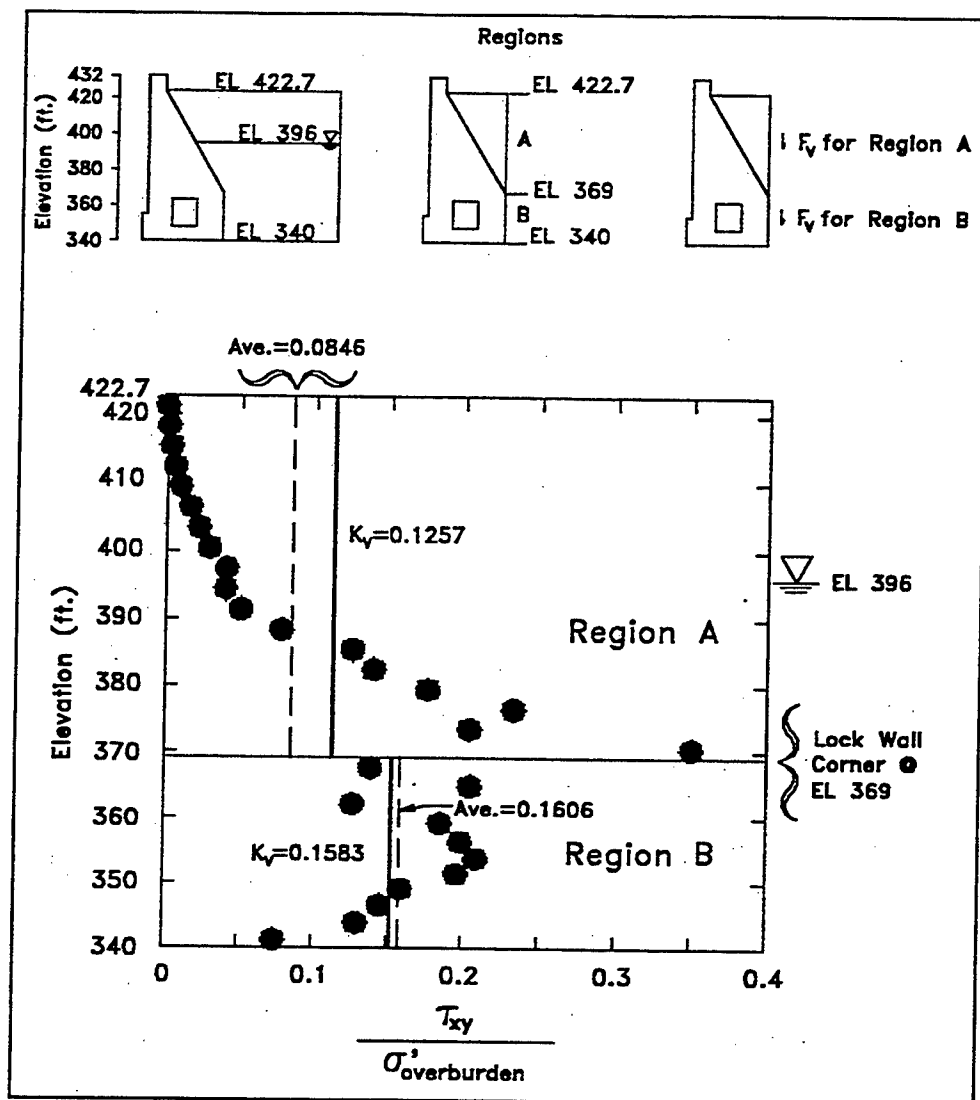
Figure 43. Variations in [\tau_{xy} / \sigma'_{\text{overburden}}] with elevation and K_v for two soil regions (1 ft = 0.305 m)
