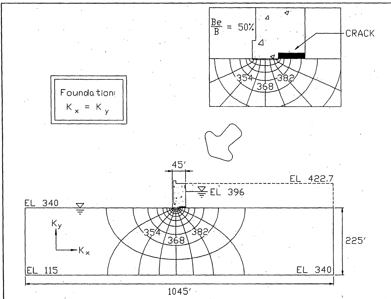
Figure 58. Results for B_e/B = 50 percent, K_x = K_y (1 ft = 0.305 m)
