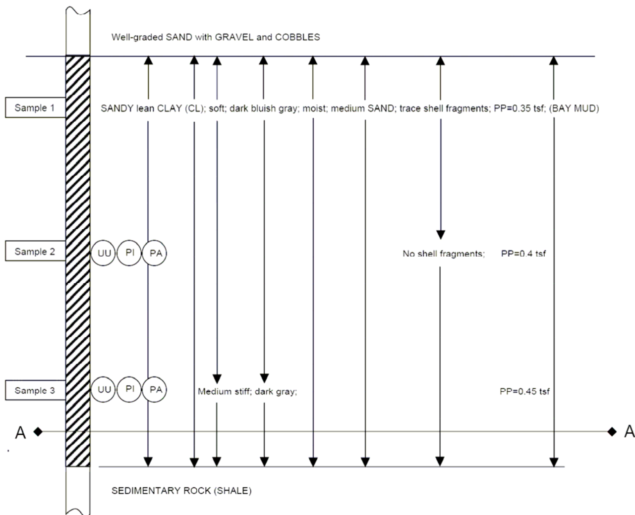
Figure 4-4 Layer Interpretation
