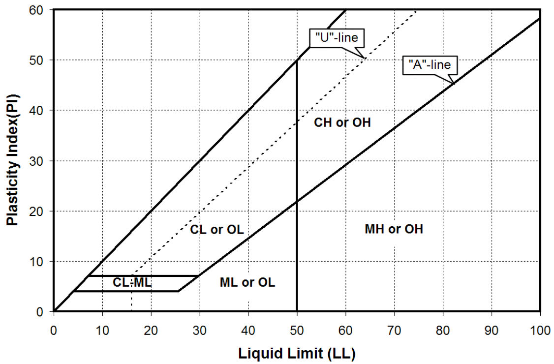
Figure 3-1 Classification of Fine-Grained Soil
