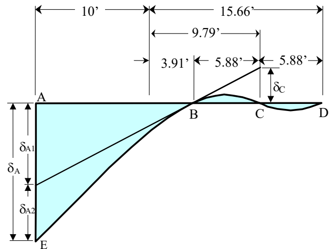
Figure 6-22. Deflected Shape
