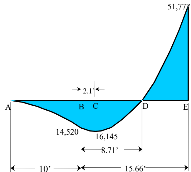
Figure 6-20. Shear Diagram
