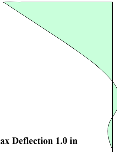
Figure 6-28. Deflection Diagram
