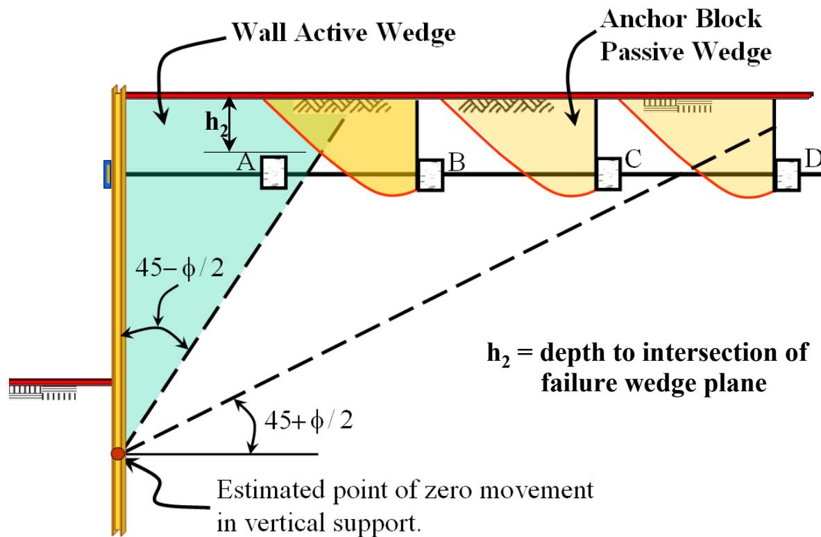
Figure 9-2. Anchor block
