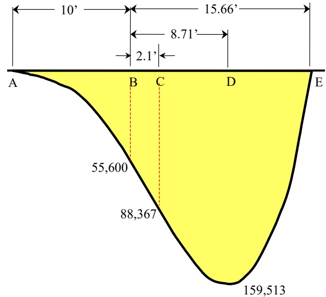
Figure 6-21. Moment Diagram
