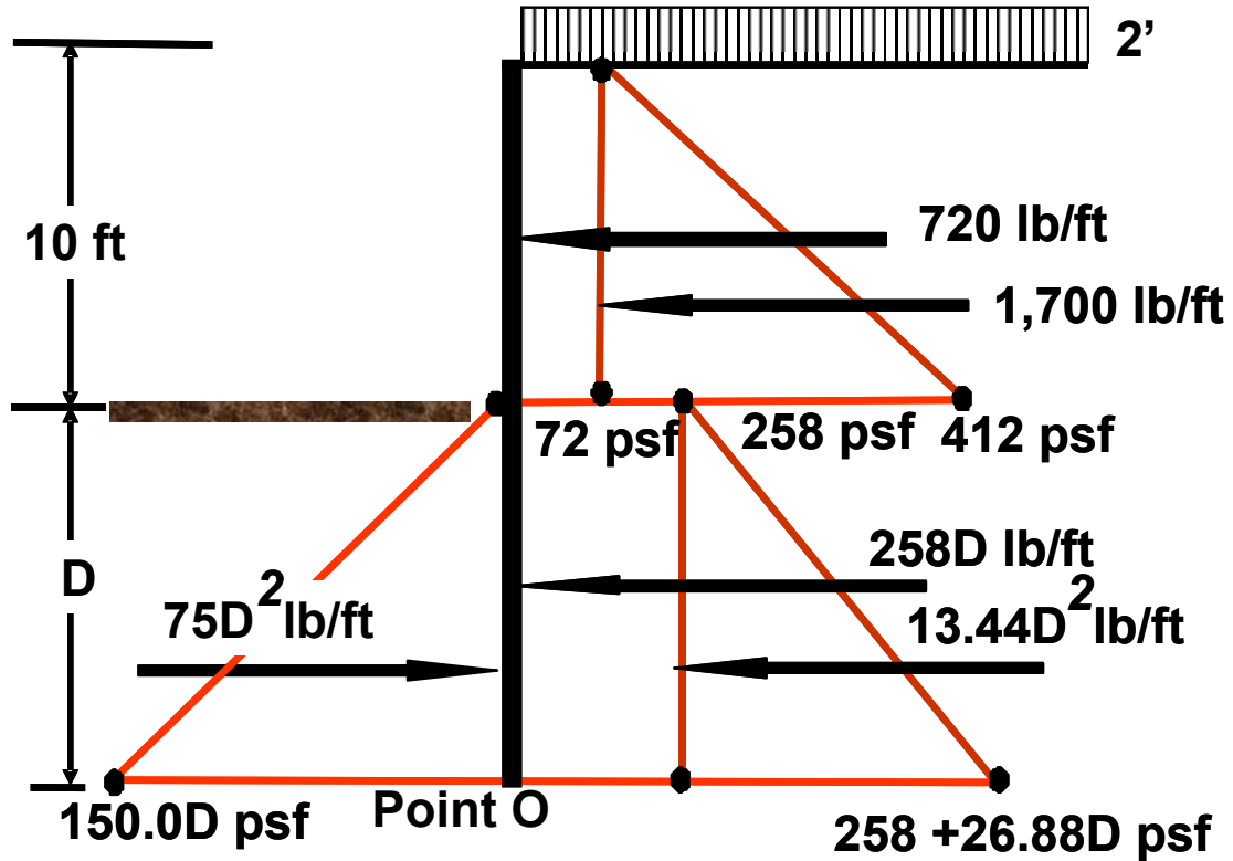
Figure 6-17. Pressure Diagram
