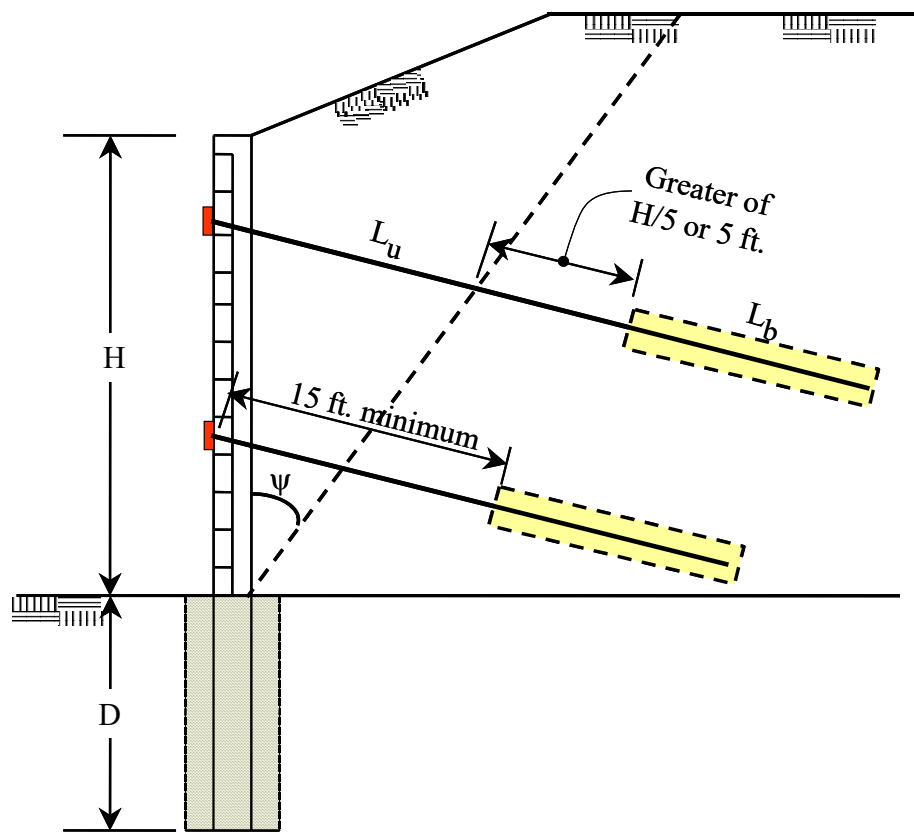
Figure 9-29. Bond Length
