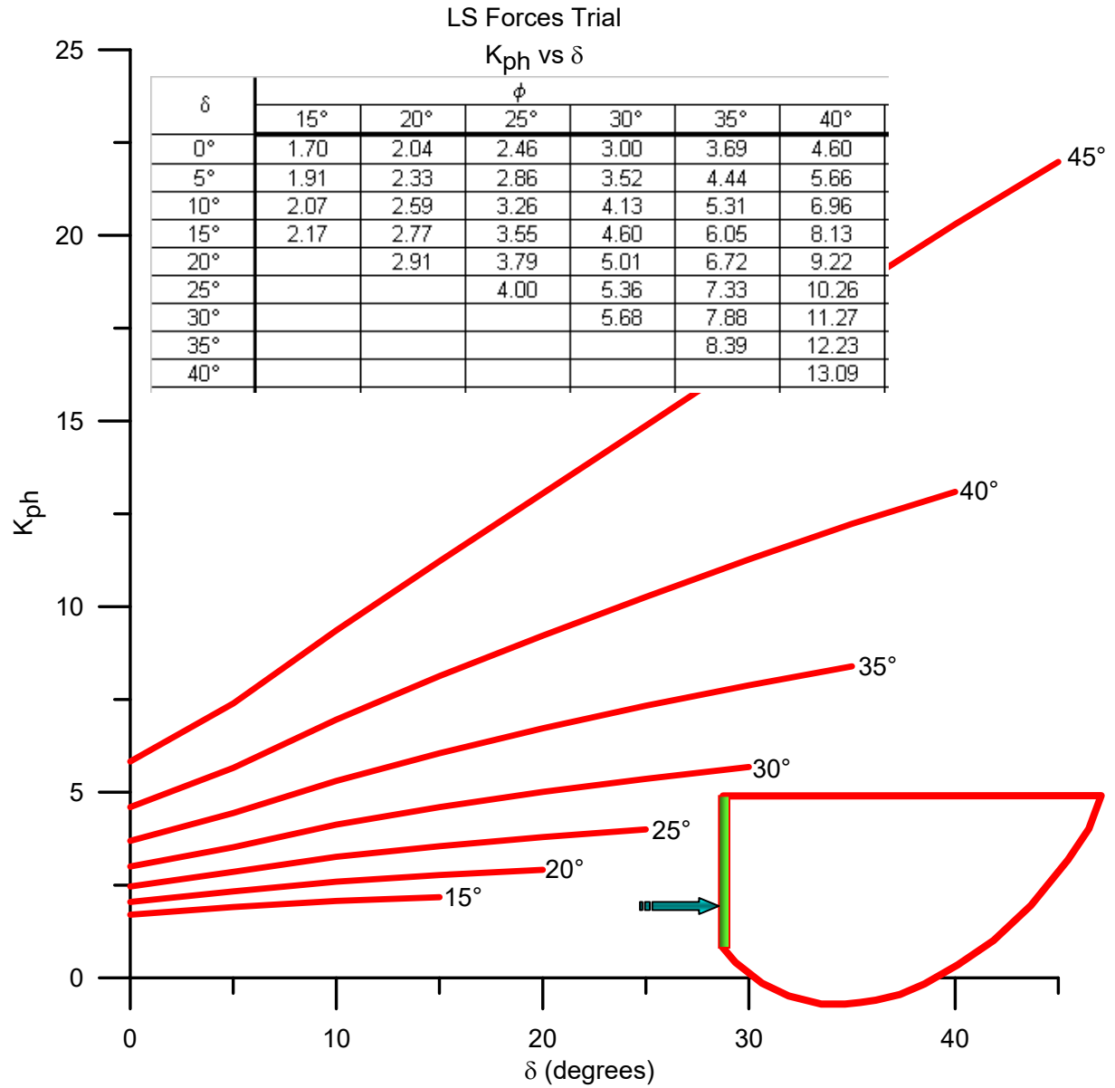
Figure 4-40. Log Spiral – Forces Method – Full Log Spiral – Trial
