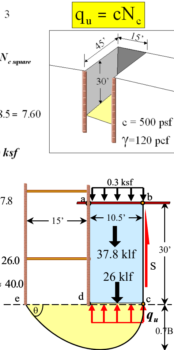
Figure 9-15. Heave example problem
