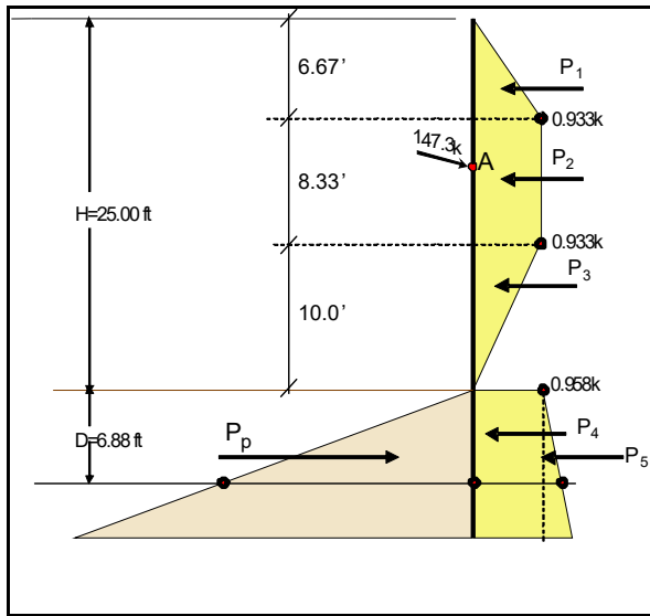
Figure 7-14. Pressure Diagram
