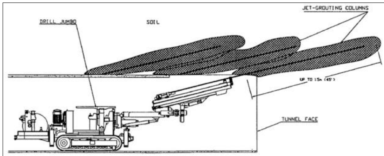
Figure 24-1. Jet grouting within a soft ground tunnel.
