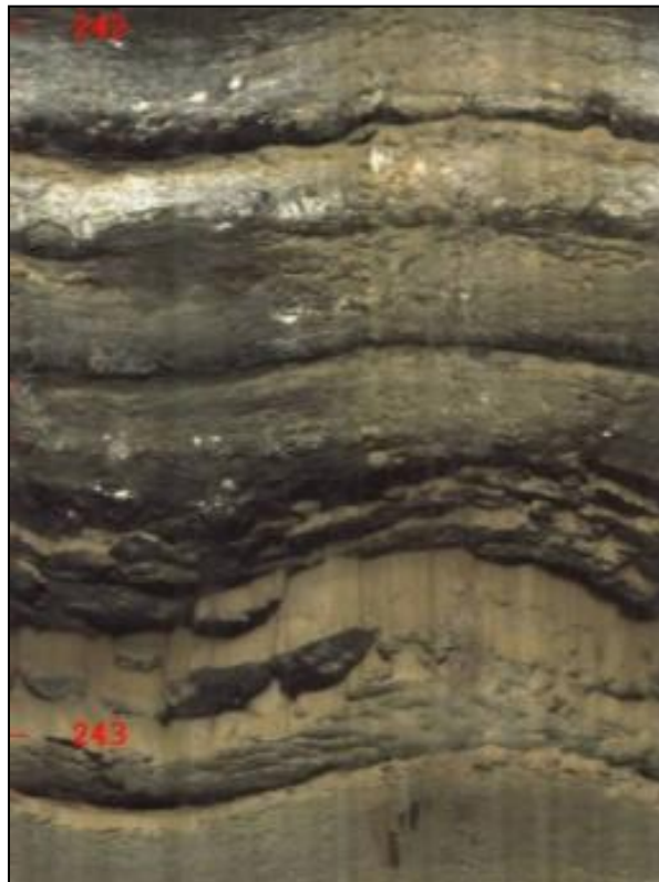
Figure 17-35. Bedding plane fractures at 0.1- to 0.2-ft intervals at Wolf Creek Dam – Leipers formation. The lower fractures are infilled. The vertical scales are feet.
