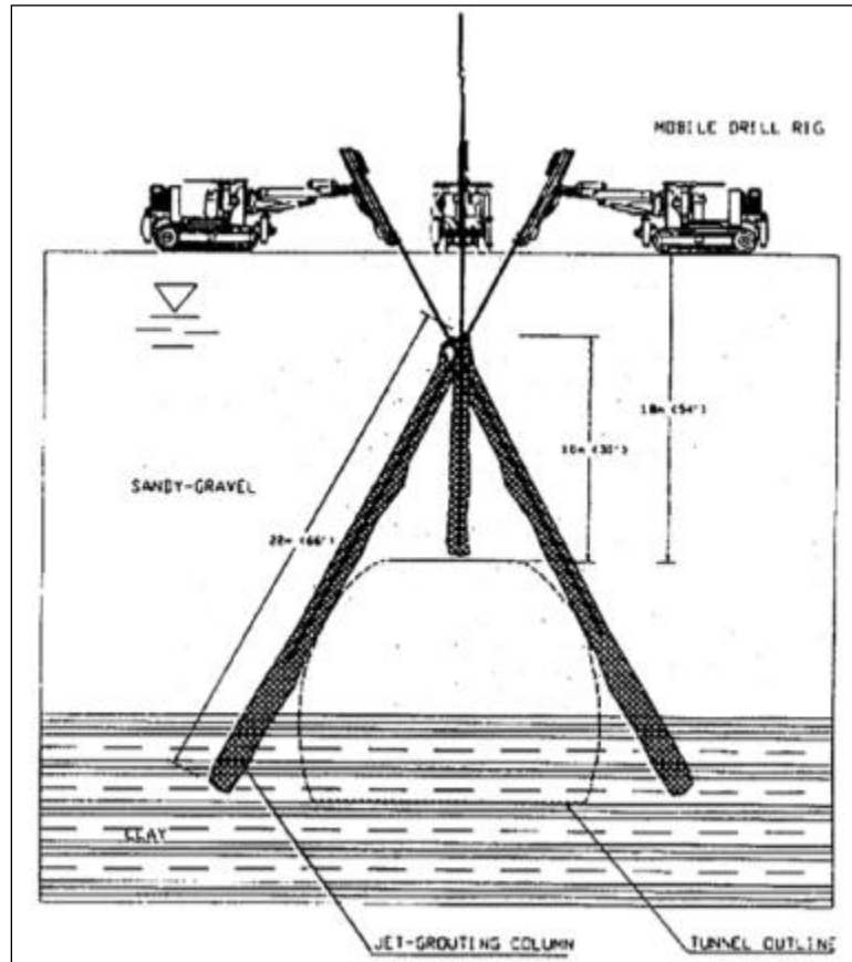
Figure 24-2. Jet grouting from the ground surface for a soft ground tunnel.
