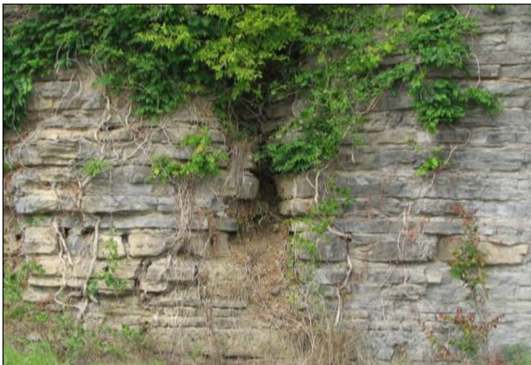
Figure 17-12. Near-surface vertical feature at Center Hill Dam (Nashville District).
