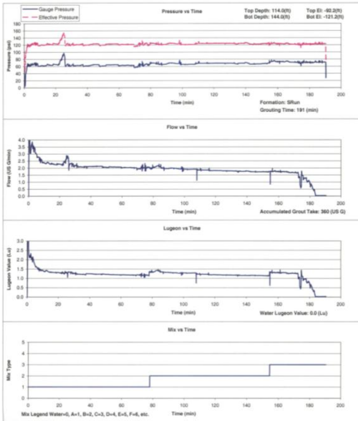
Figure 15-20. Abrupt refusal of a low Lugeon stage after a second mix change. The decision to thicken was based on time management of the stage and the extremely slow rate of approaching refusal under Mix 2.
