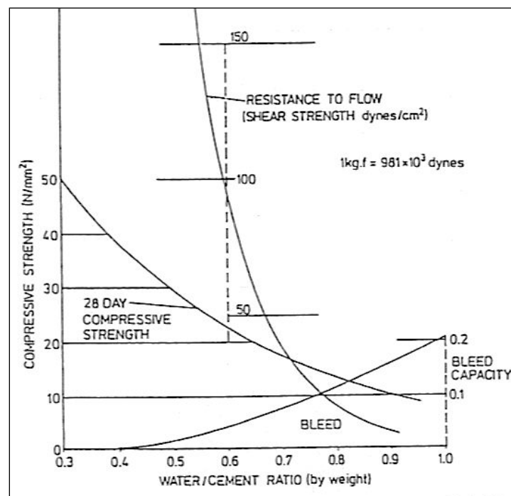
Figure 23-5. Effect of water content on cement grout properties.
