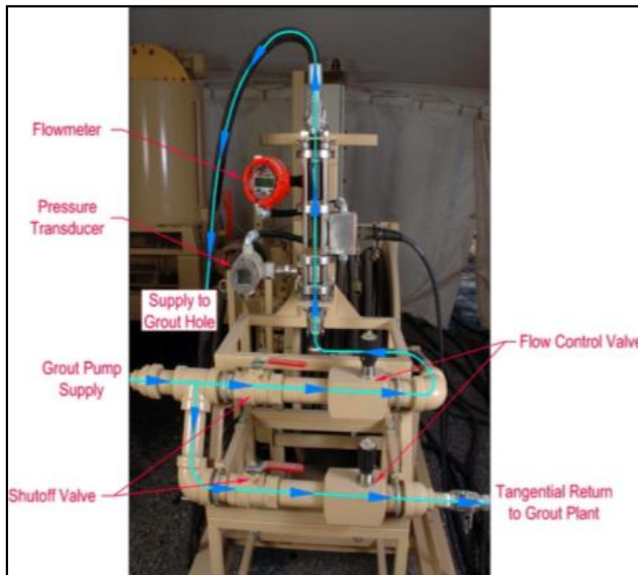
Figure 10-17. Header system for electronic monitoring of flow and pressure for HMG injection.
