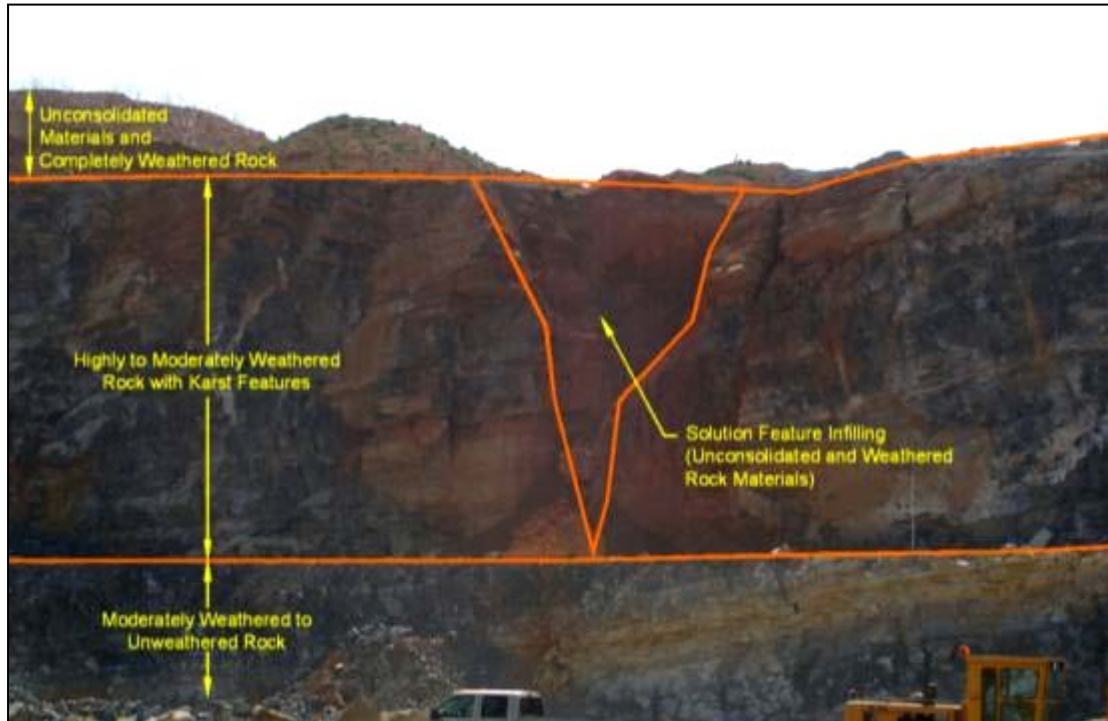
Figure 4-4. Geologic profile in a karst quarry in PA.
