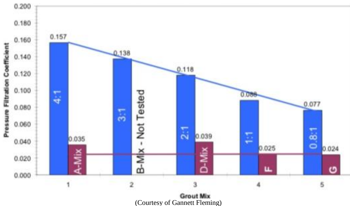
Figure 7-18. Pressure filtration coefficient values from the Penn Forest Dam mix testing program.
