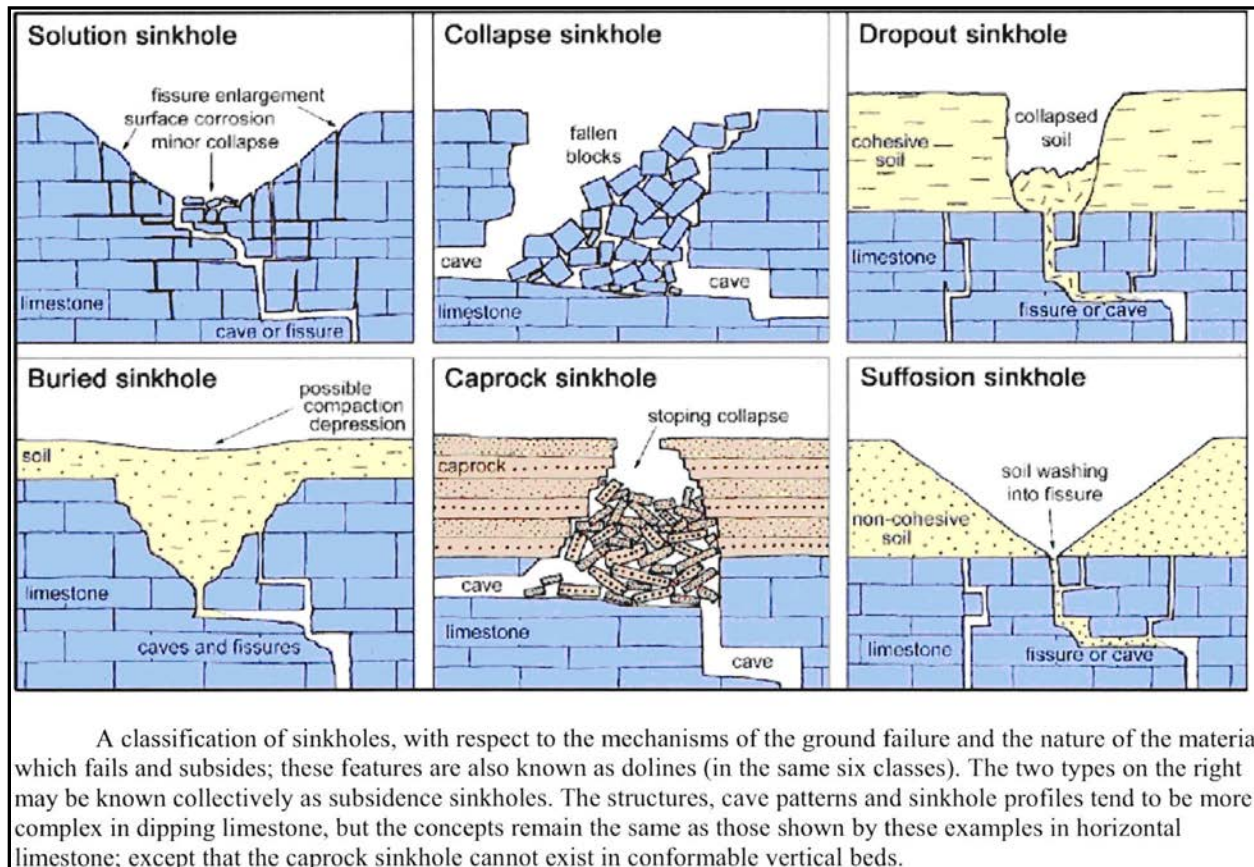
Figure 17-2. Sinkhole types.
