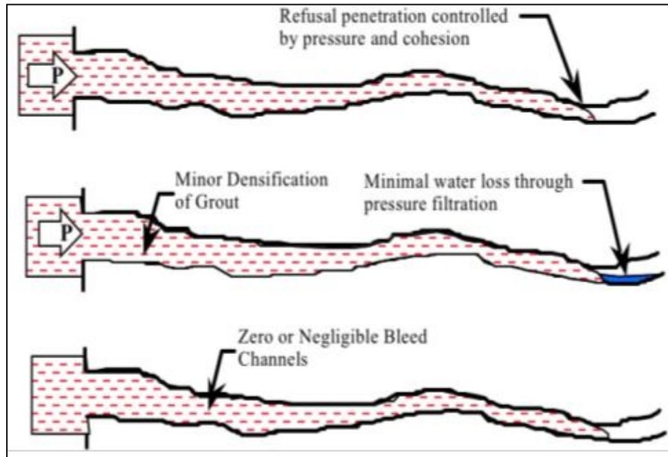
Figure 7-20. Grouting theory for balanced stable grouts.
