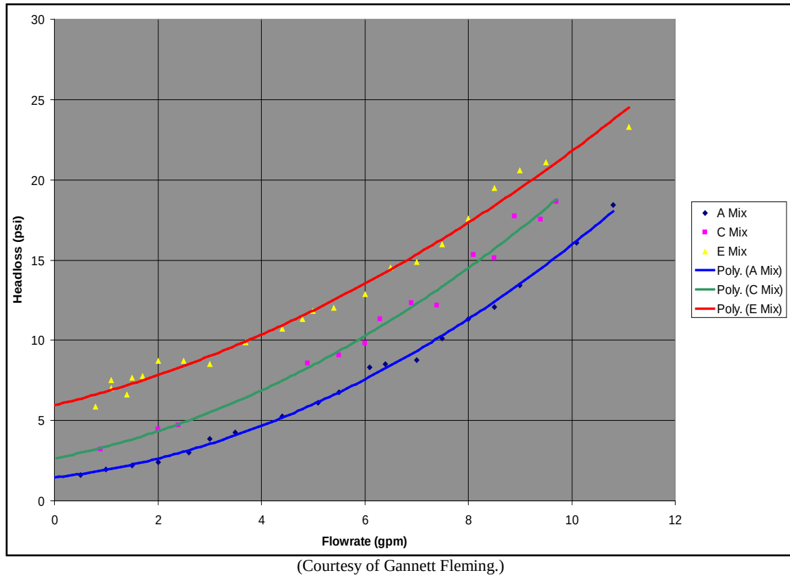
Figure 15-2. Example of field-determined head-loss curves for grout mixes.
