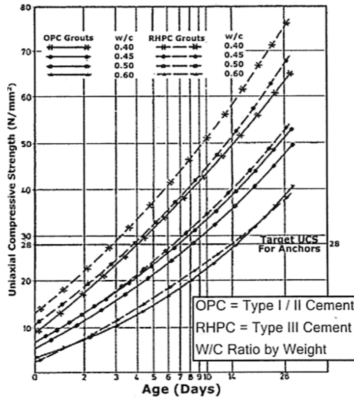
Figure 23-4. Strengths for various water-cement ratios.
