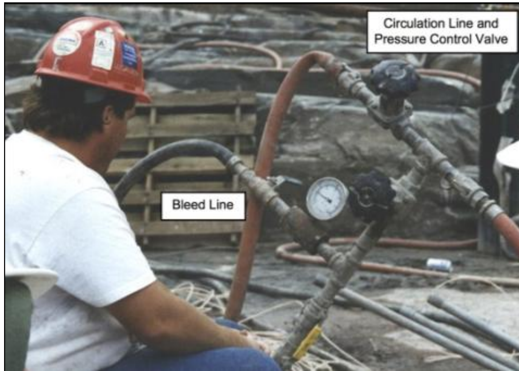
Figure 15-24. Standpipe arrangement for unstable grouts equipped with a bleed valve.
