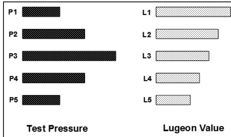
Figure 15-11. Clogging behavior.
