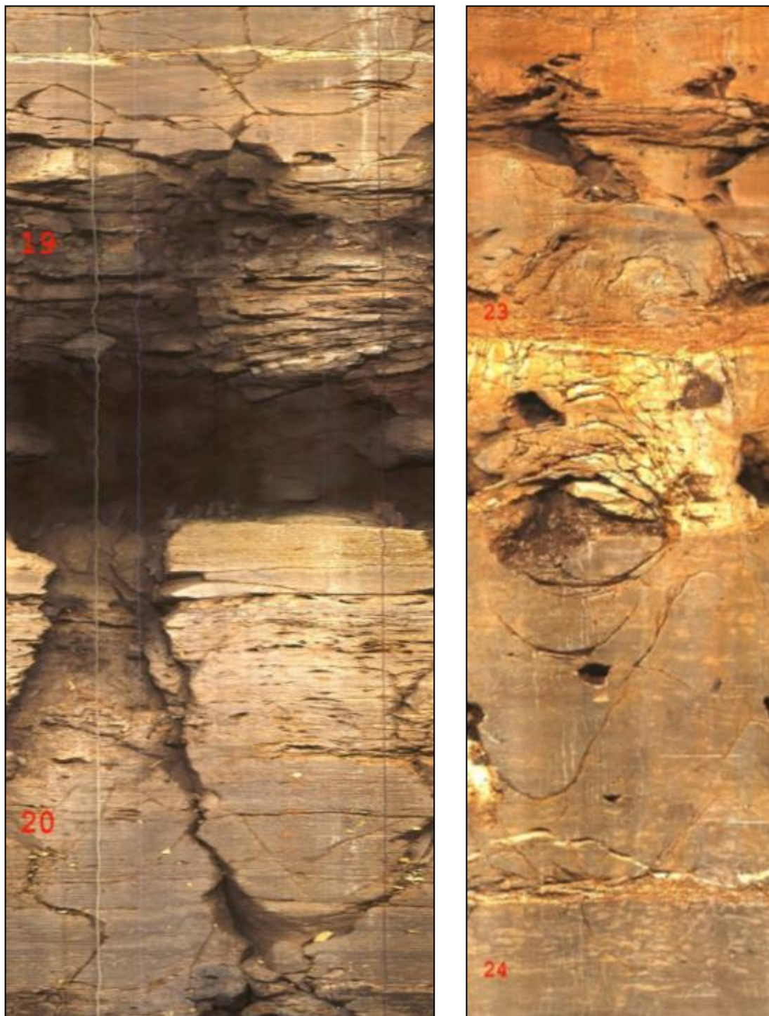
Figure 17-28. Clearwater Dam at shallow depth into rock (Little Rock District). The vertical scales are meters. Note the relatively clean, high-angle fractures and dissolution along bedding and as vugs.
