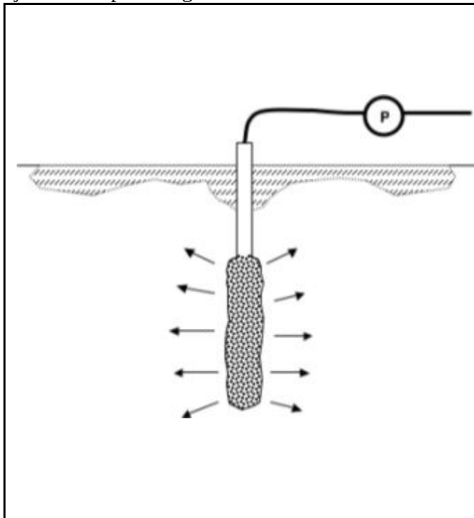
Figure 27-1. Injected grout mass displacing and compacting surrounding soil.
