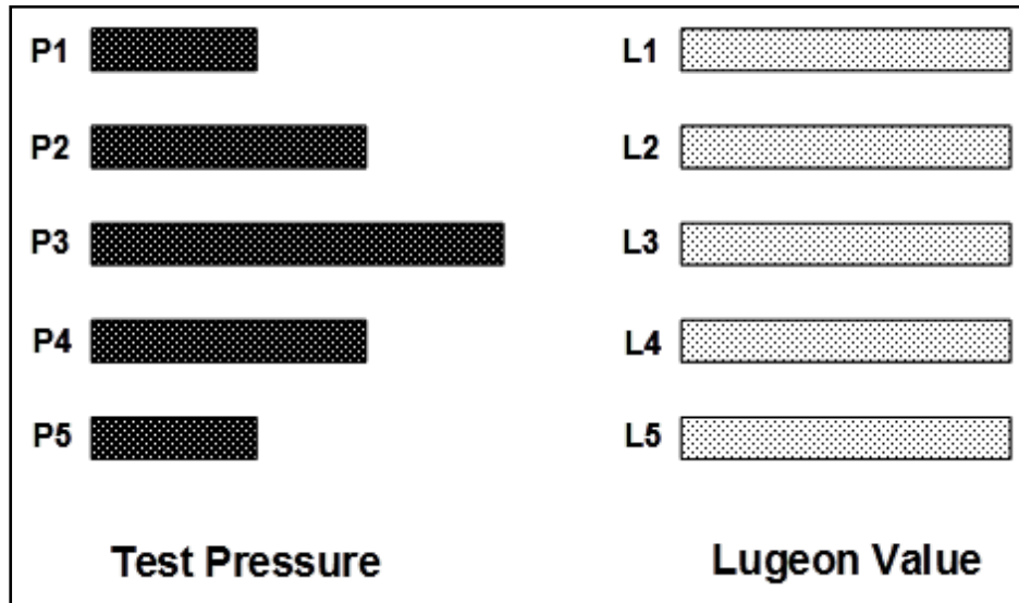
Figure 15-6. Laminar flow behavior. When the test section is composed of clean, finer fractures, there will normally be little variation of the Lugeon value with pressure because it is dominated by simple laminar flow. The permeability is constant within the range of pressures used.
