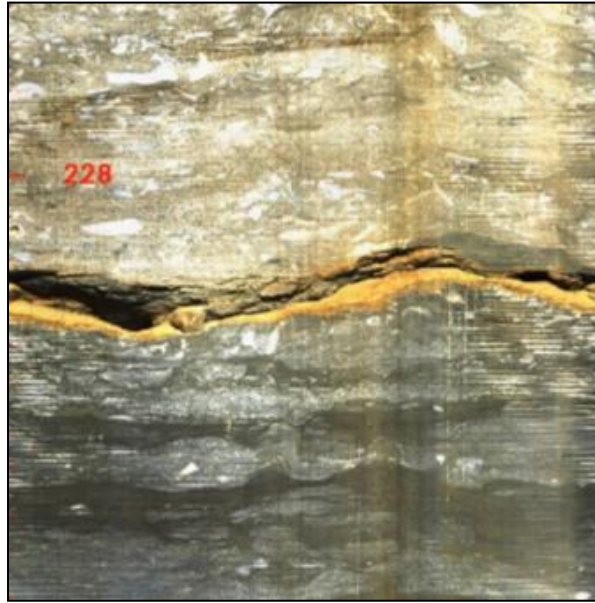
Figure 17-34. Weathered and partly infilled bedding plane fracture at Wolf Creek Dam, Leipers formation. The vertical scales are feet.
