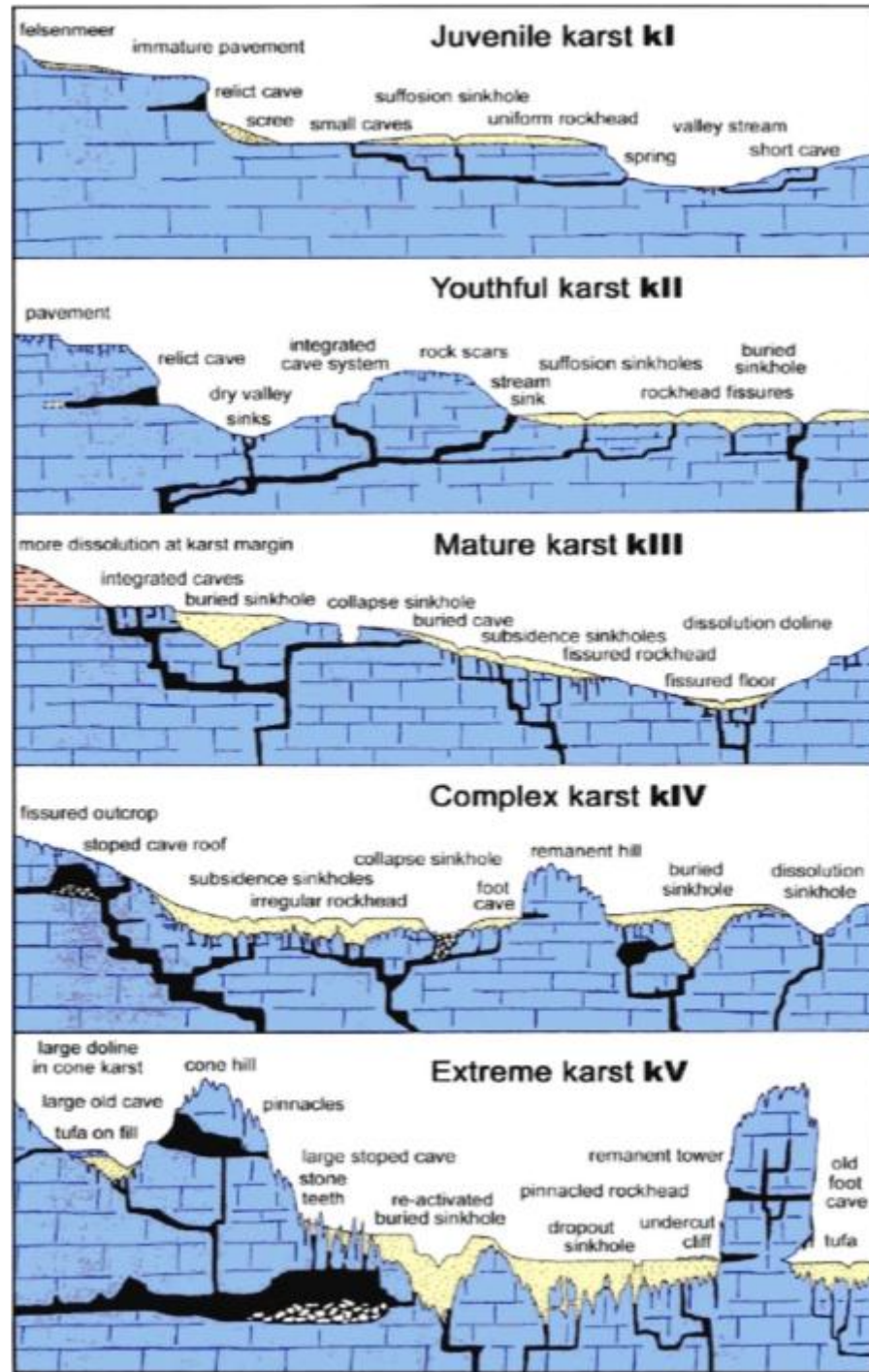
Figure 17-3. Schematics of karst classifications. Typical morphological features of karstic ground conditions with the five classes of karst (Table 17-2). These examples show horizontal bedding of the limestone; dipping bedding planes and inclined fractures add complexity to most of the features and also create planar failures behind steep cliff faces. The dotted ornament represents any type of clastic soil or surface sediment.
