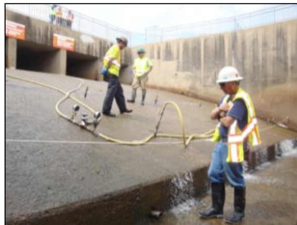
Figure 25-2. Backfill grouting operations to fill voids under the downstream parabolic spillway slab at Barker Dam outside of Houston, TX (Galveston District). Holes were drilled on 10-ft centers, and injection pressures were controlled by the manifold at the injection point. A circulating system was used to verify the volume of voids being filled with cementitious grout.
