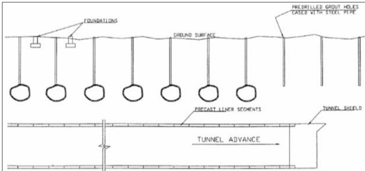
Figure 24-3. Compaction grouting from the ground surface for a soft ground tunnel.
