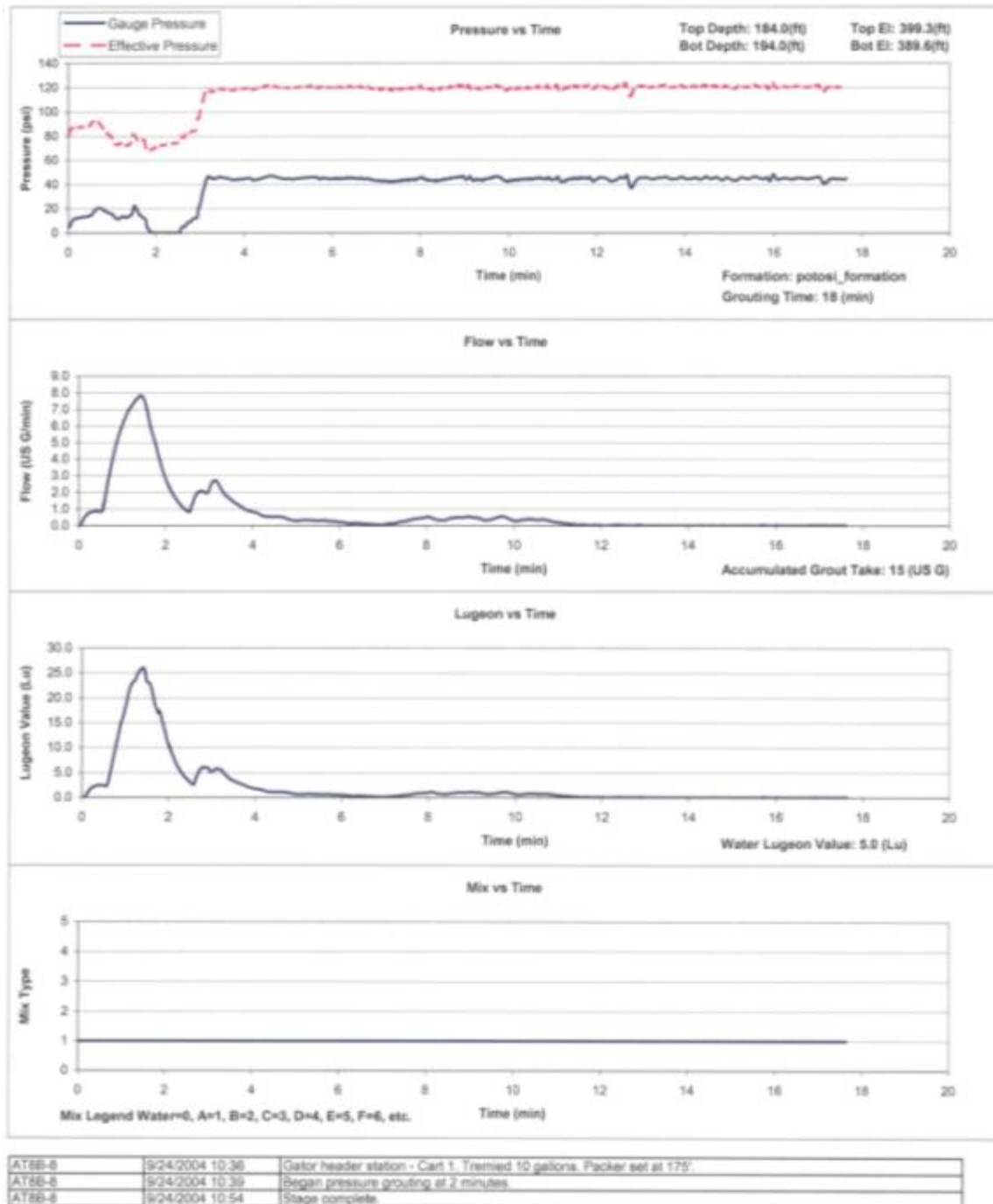
Figure 15-23. Rapid refusal on a tertiary hole.
