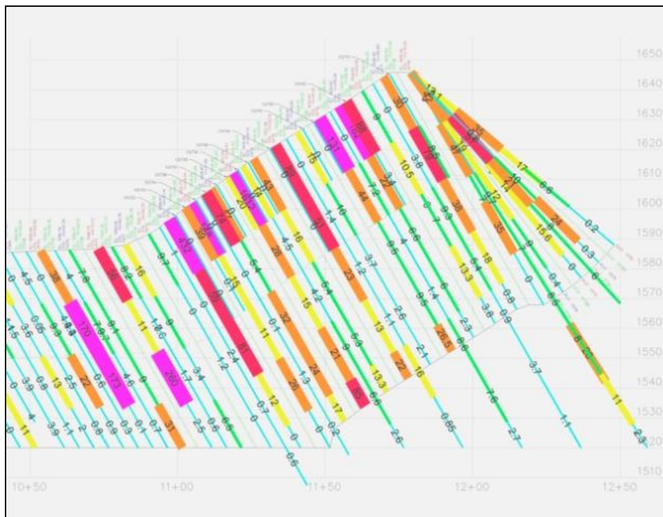
Figure 16-11. Computer-generated profile showing water pressure testing results with scaled color coding.
