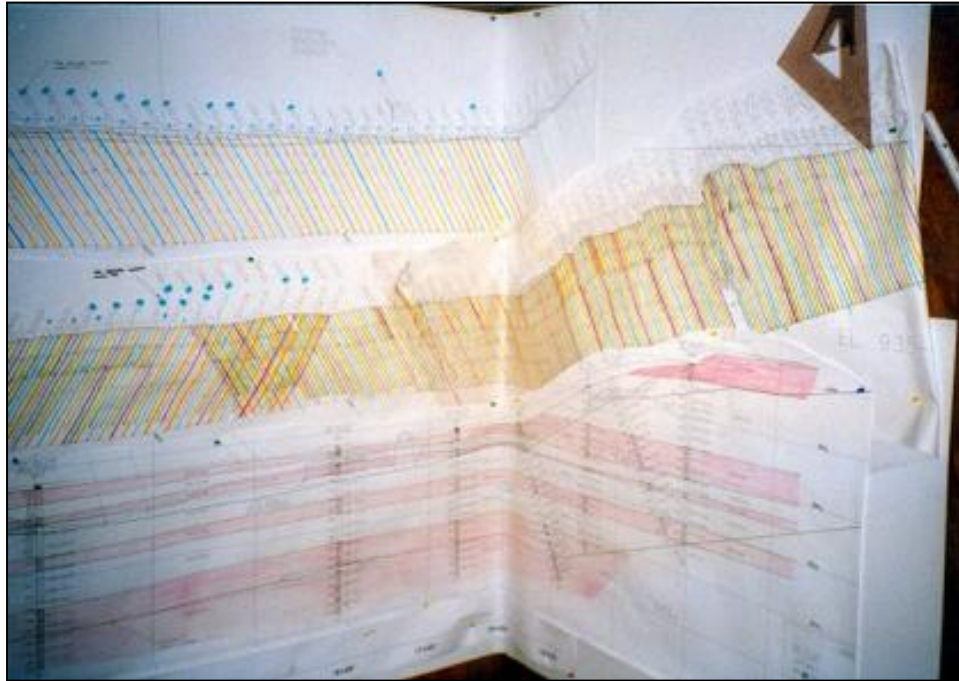
Figure 16-10. Hand-drawn profile containing all progress and results on a single sheet.
