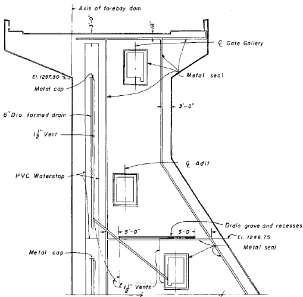
Figure 25-3. Metal seals inserted in the face of the first concrete placement and extended into the adjacent monolith, or second concrete placement to contain grout within area to be grouted.
