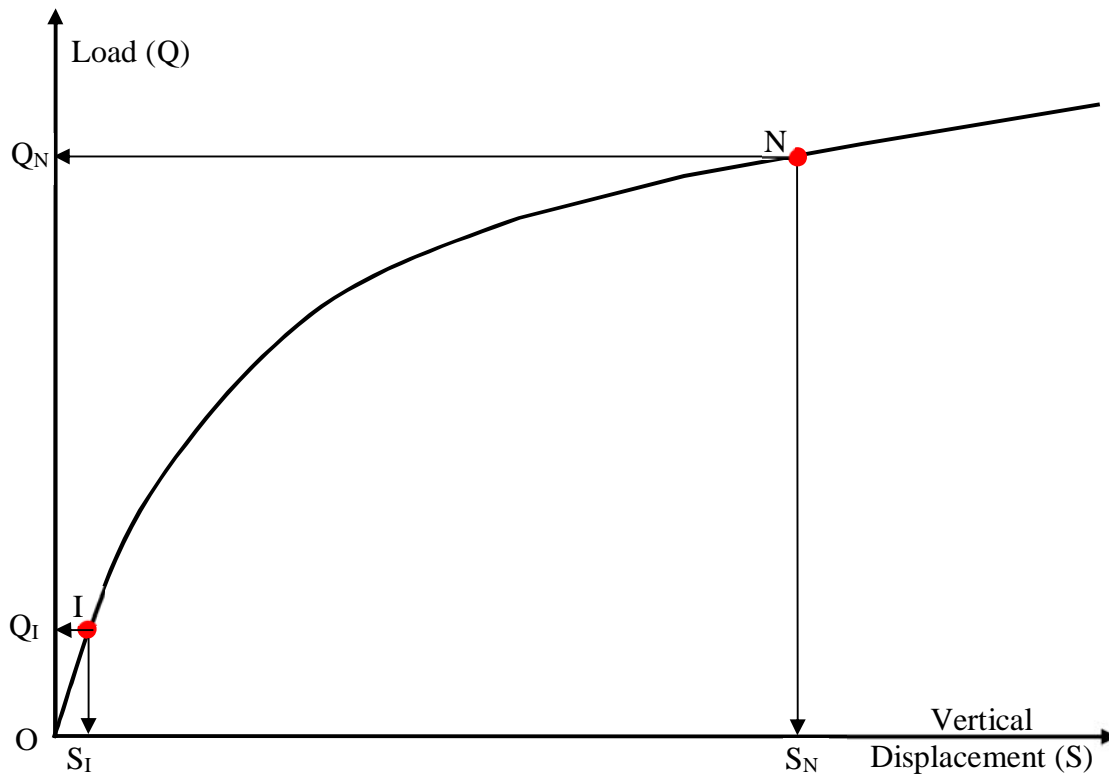
Figure 2-1. Schematic. Typical axial load versus vertical displacement curve ( Q-\delta ) for spread footing of width B_f .
