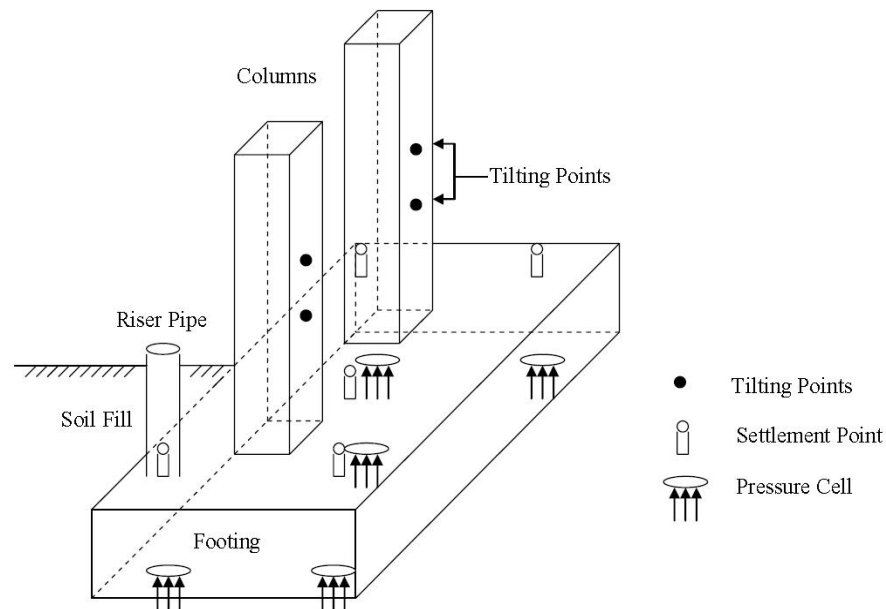
(a) General layout of instrumentation for monitoring settlement, bearing pressure and tilting
