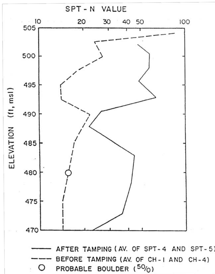
Figure 4-24. Increase in SPT values in a mine spoil after deep dynamic compaction.
