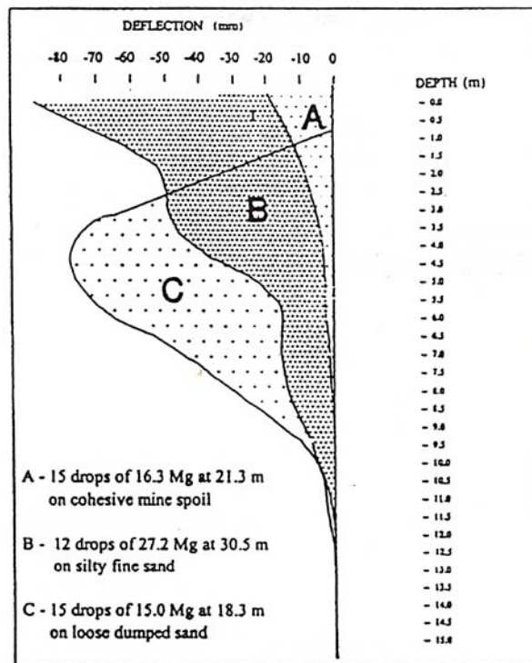
Figure 4-9. Lateral movements at 6 m (20 feet) from drop point.
