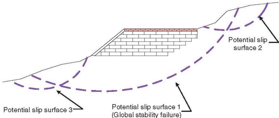
Figure 3-8. Multiple potential failure surfaces to consider with EPS-block geofoam slope systems.
