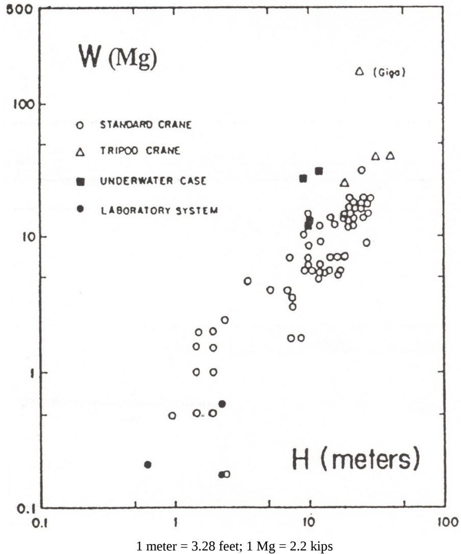
Figure 4-22. Relationship between tamper mass and drop height.
