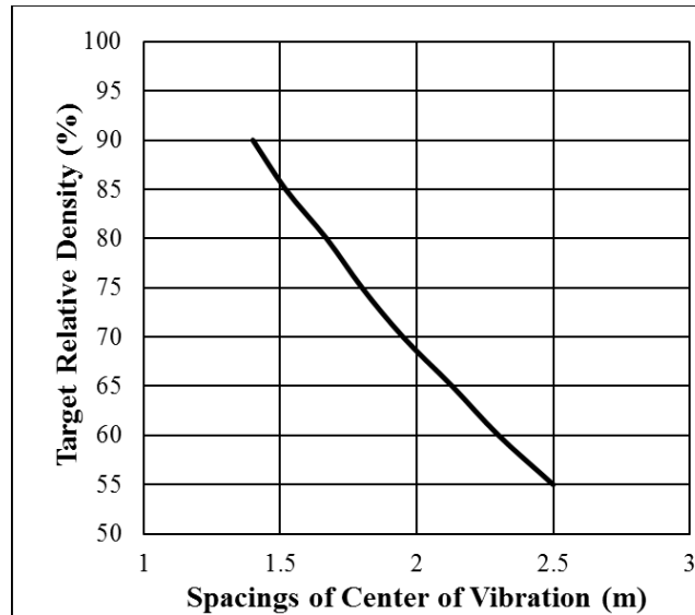
Figure 4-34. Relative density versus probe spacing for silty sands.
