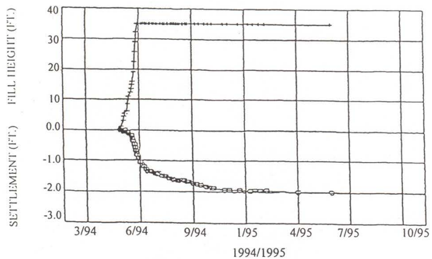
Figure 2-16. Tift Street west approach embankment field data.
