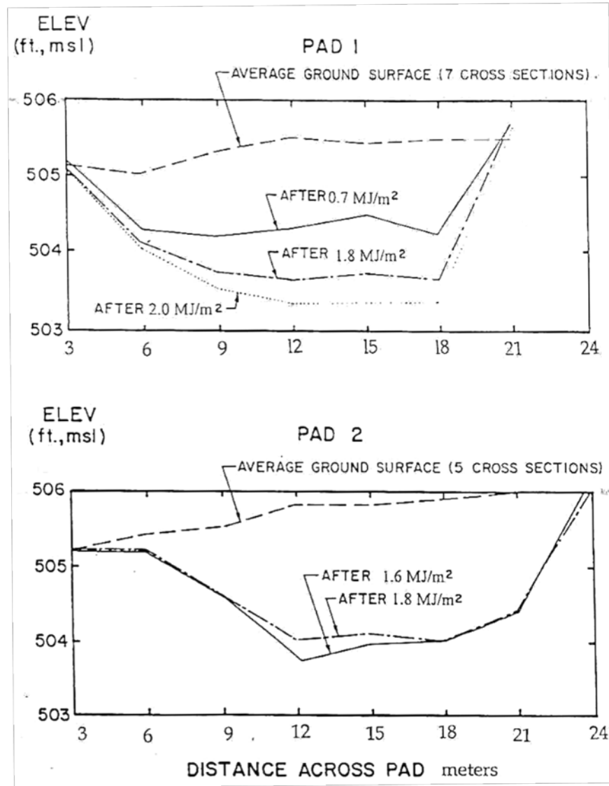
Figure 4-25. Induced settlement following deep dynamic compaction at the mine spoil project in Alabama.
