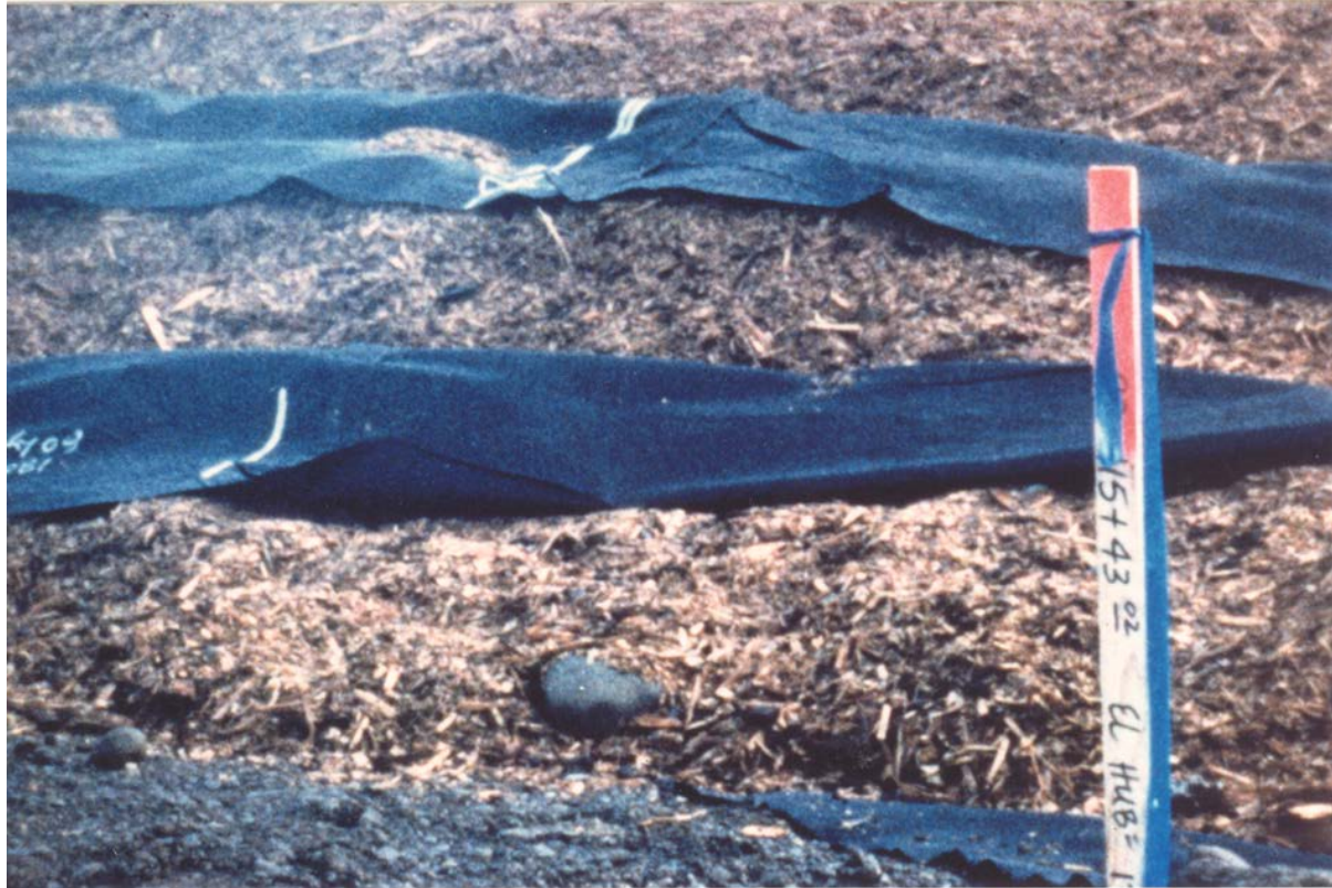
Figure 3-4. Embankment construction with wood fiber.
