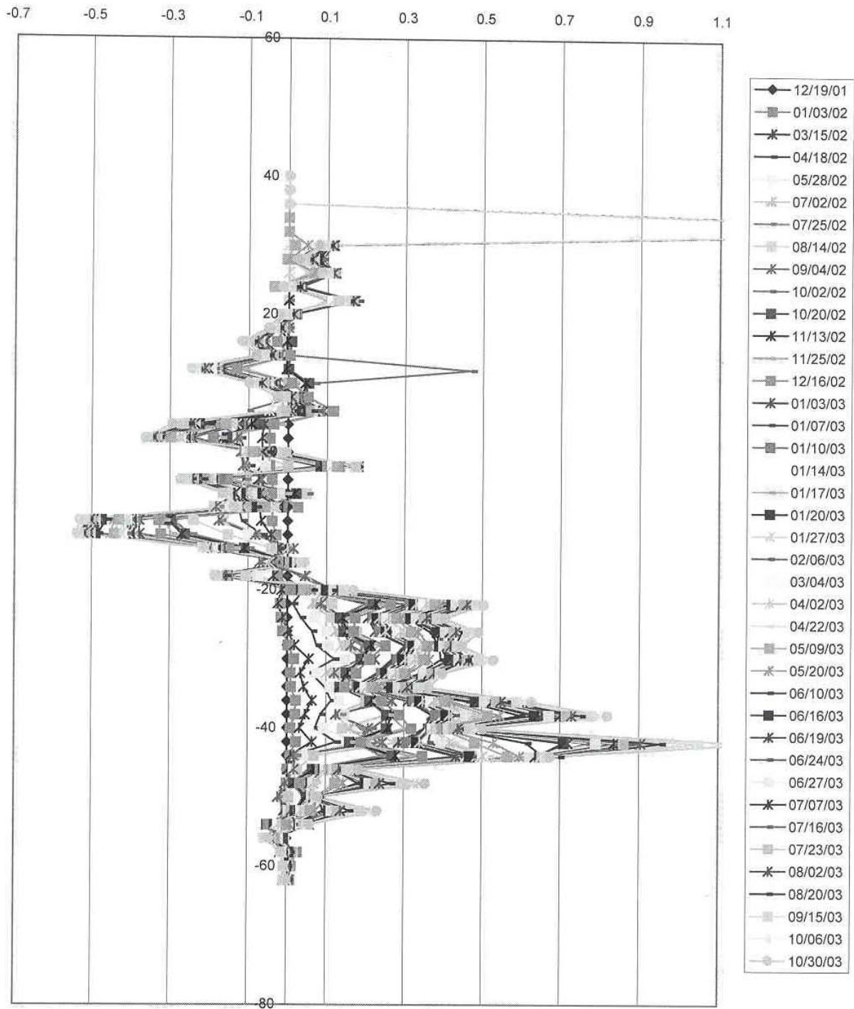
Figure 2-13. Incremental displacement versus depth.
