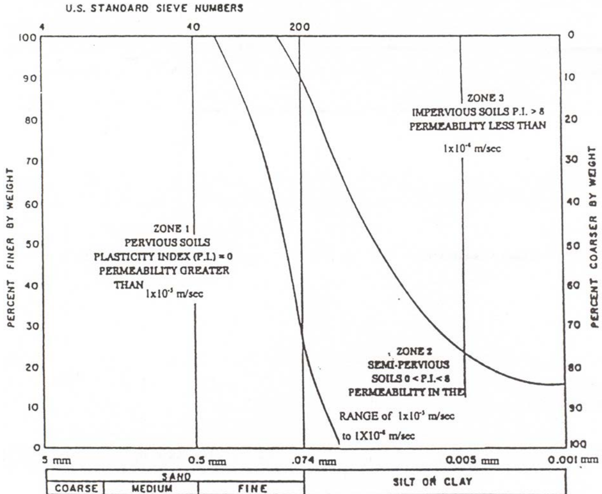
Figure 4-5. Grouping of soils for deep dynamic compaction.
