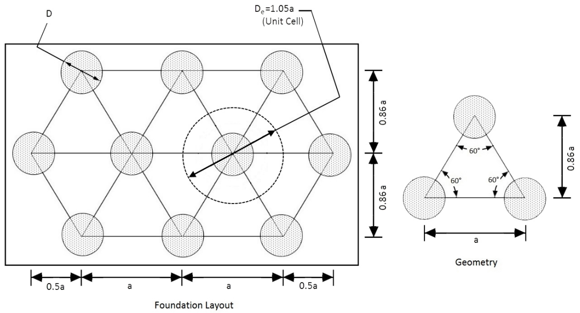
Figure 5-16. Equilateral triangular pattern of stone columns.
