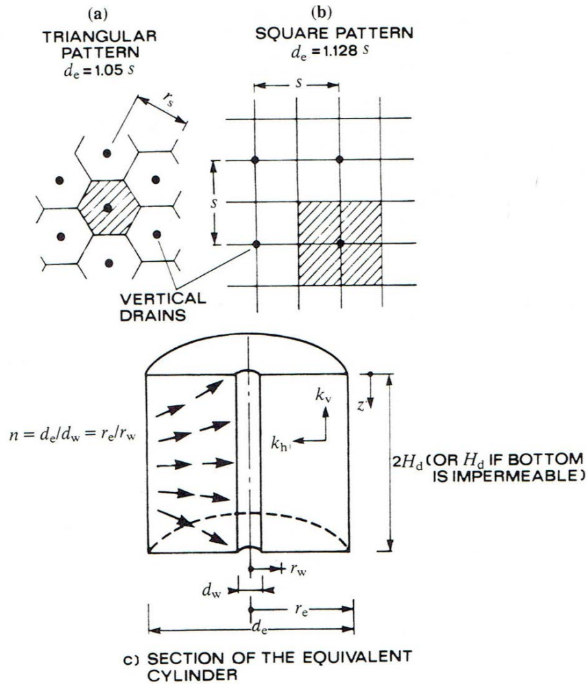
Figure 2-7. Drain patterns: triangular pattern (top left), square pattern (top right), equivalent cylinder (bottom).
