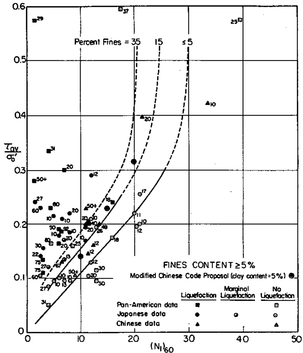
Figure 5-23. Relationship between stress ratio causing liquefaction and (N_1)_{60} values for silty sands for 7.5 magnitude earthquakes.
