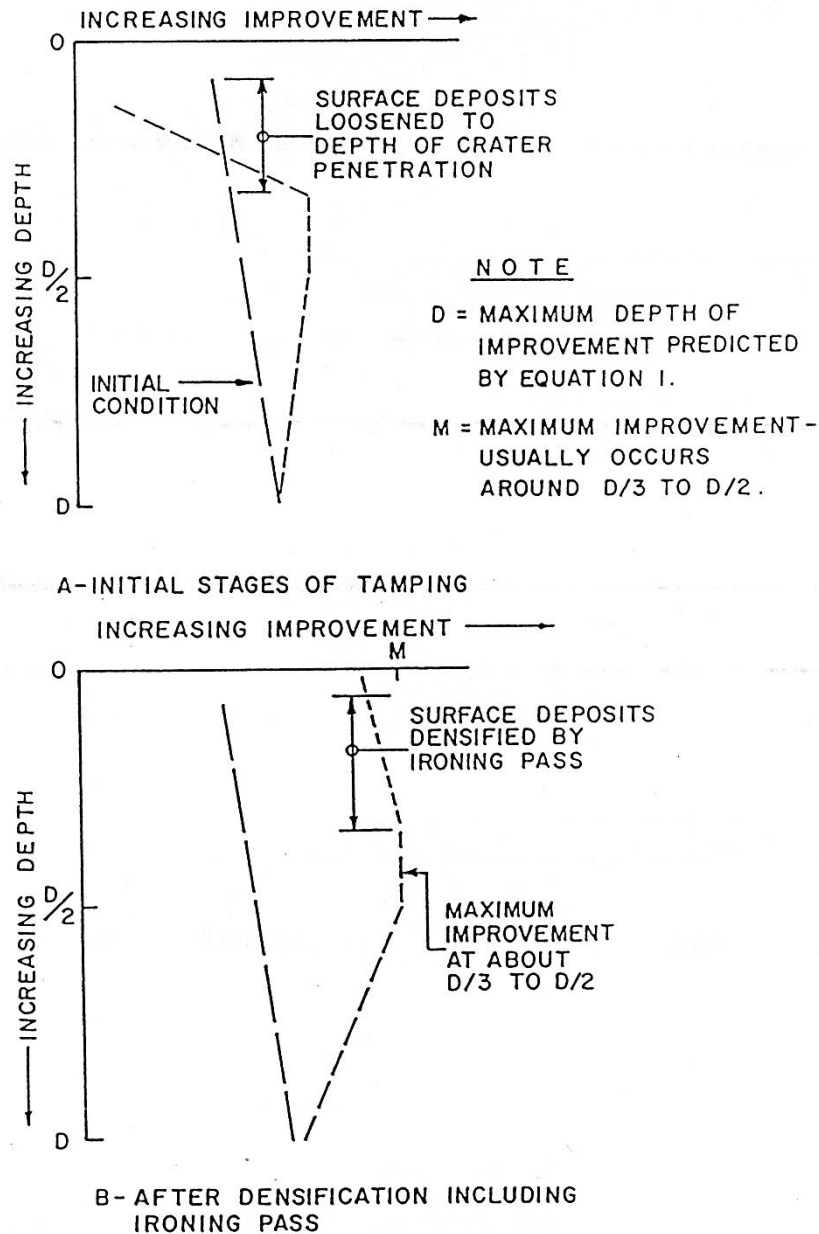
Figure 4-23. Variations in improvements with depth during deep dynamic compaction.
