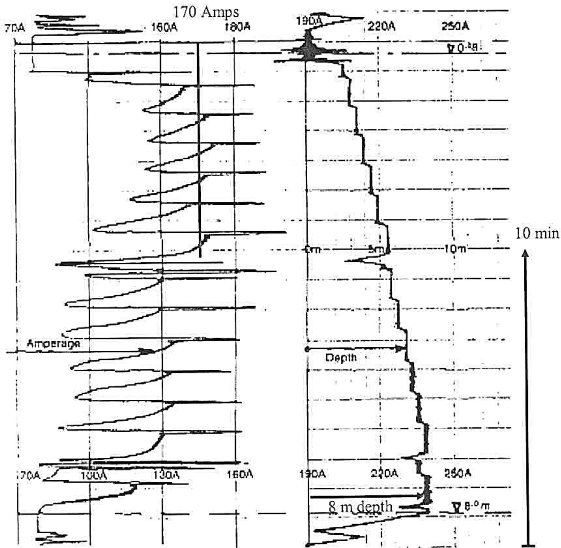
Figure 4-37. Typical data logger results: amps versus depth (left) and time versus depth (right).
