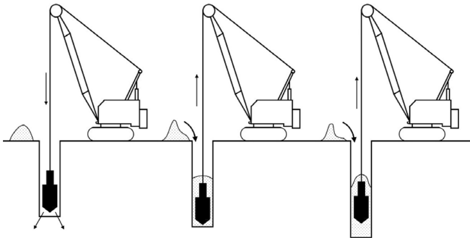
Figure 4-2. The vibro-compaction process.
