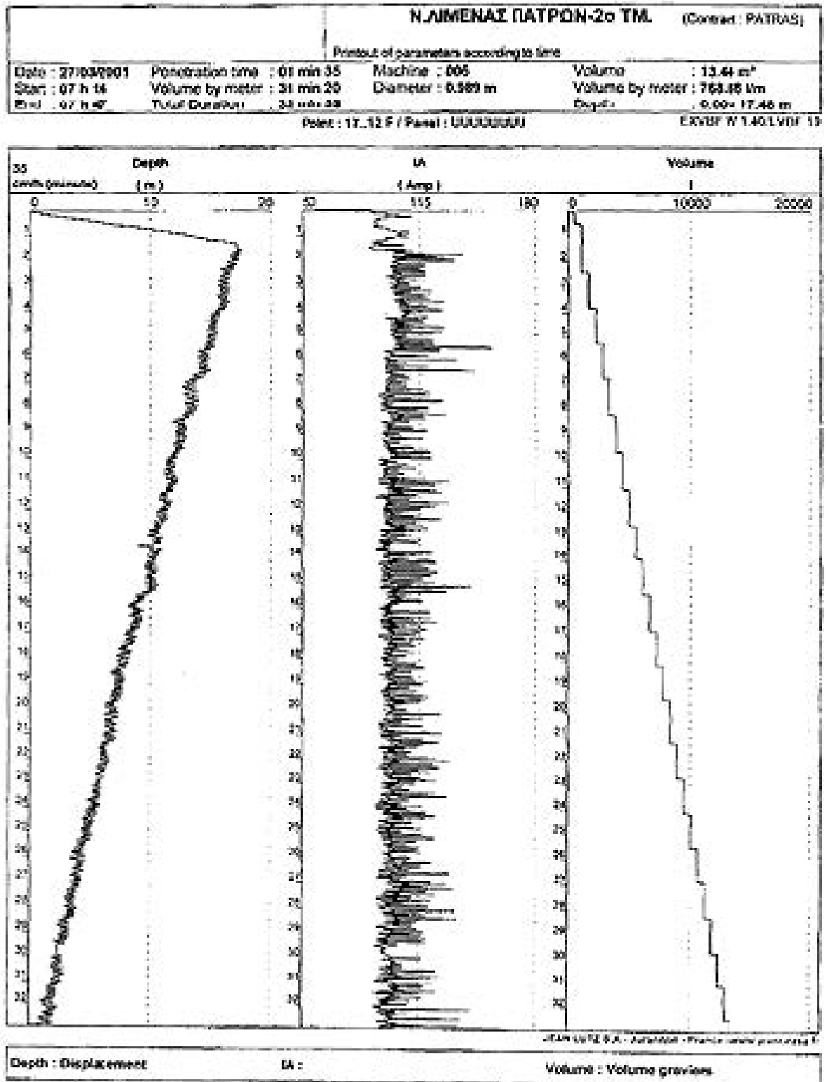
Figure 5-11. Quality control output over time for dry bottom feed vibro-displacement: depth (left), amperage (middle) and gravel (right).
