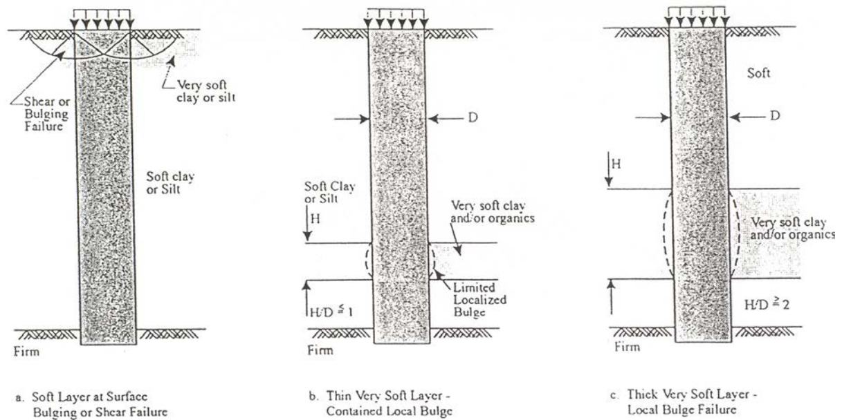
Figure 5-19. Failure modes of a single stone column in a non-homogeneous cohesive soil.
