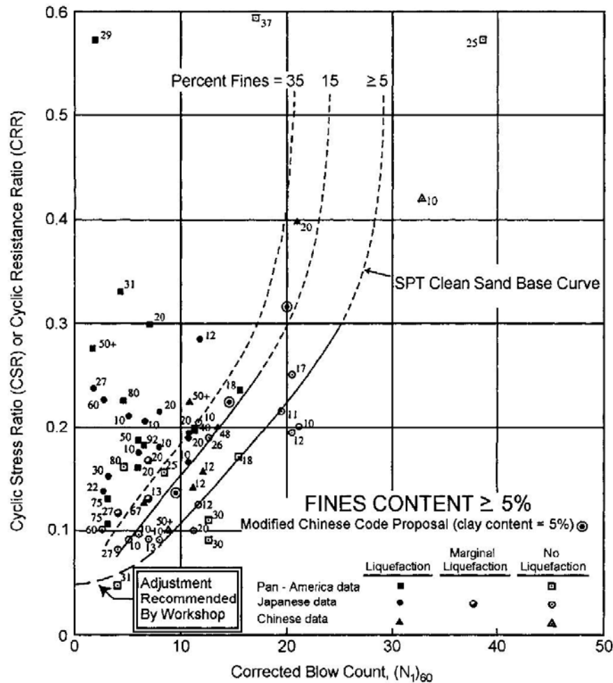
Figure 4-3. SPT liquefaction chart for magnitude 7.5 earthquakes.
