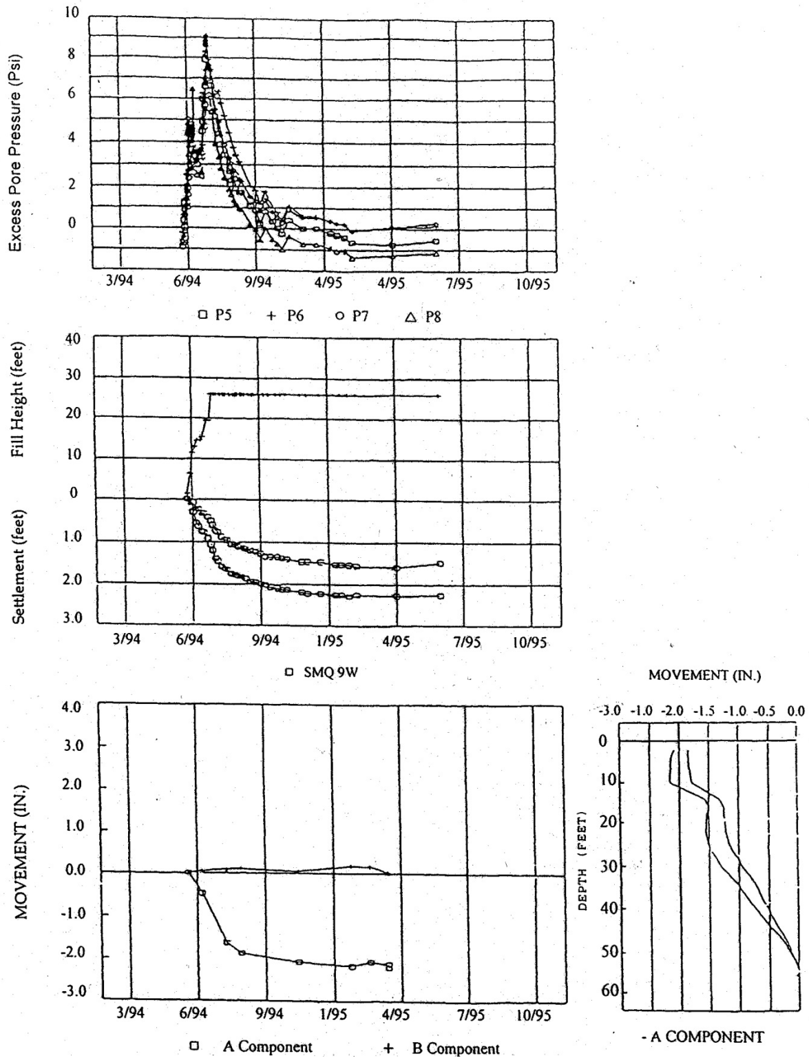
Figure 2-17. Tifft Street east approach embankment field data.
