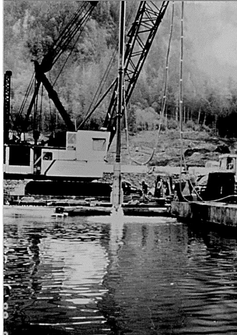
Figure 4-32. Vibrator suspended from a barge-mounted crane.
