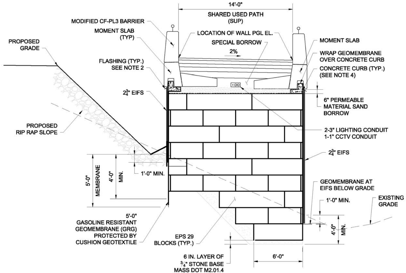
Massachusetts Department of Transportation Figure 3-11. Whittier Bridge typical ramp cross section.
