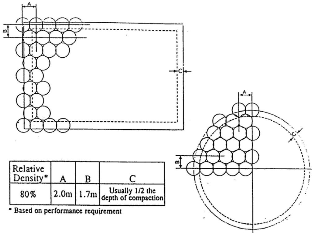
Figure 4-35. Typical compaction point spacing for area layouts.
