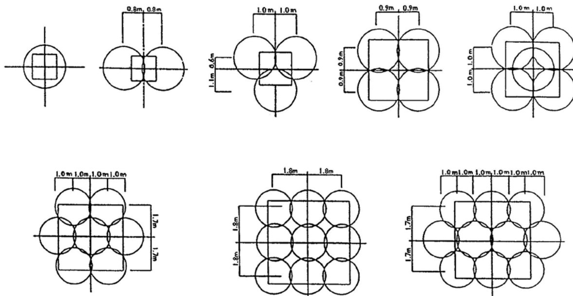
Figure 4-36. Typical compaction point layouts for column footings.
