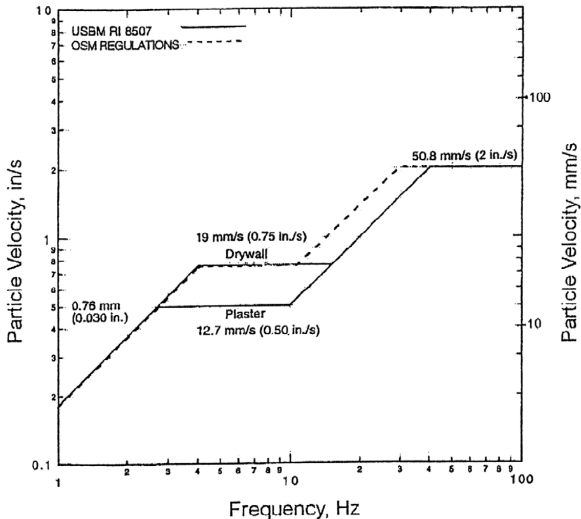
Figure 4-6. U.S. Bureau of Mines safe level of blasting vibrations for houses and Office of Surface Mining regulations.
