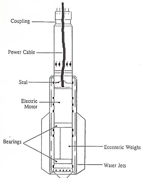
Figure 4-30. Cross-section of a typical vibrator.
