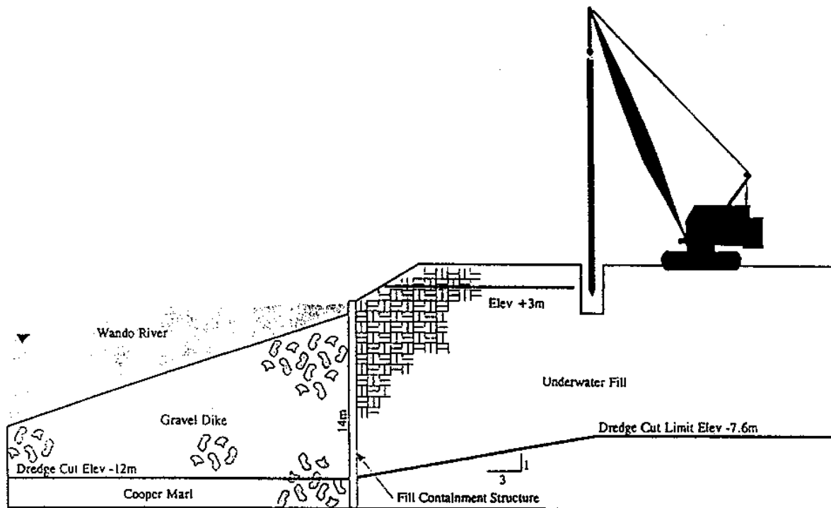
Figure 4-40. Vibro-compaction at Wando Terminal.
