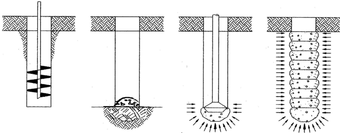
Figure 5-13. Replacement method, rammed aggregate pier construction process: from left to right, (1) make a cavity, (2) place stone at bottom of cavity, (3) ram stone to form bottom bulb, (4) place and ram thin lifts to form undulated side shaft.
