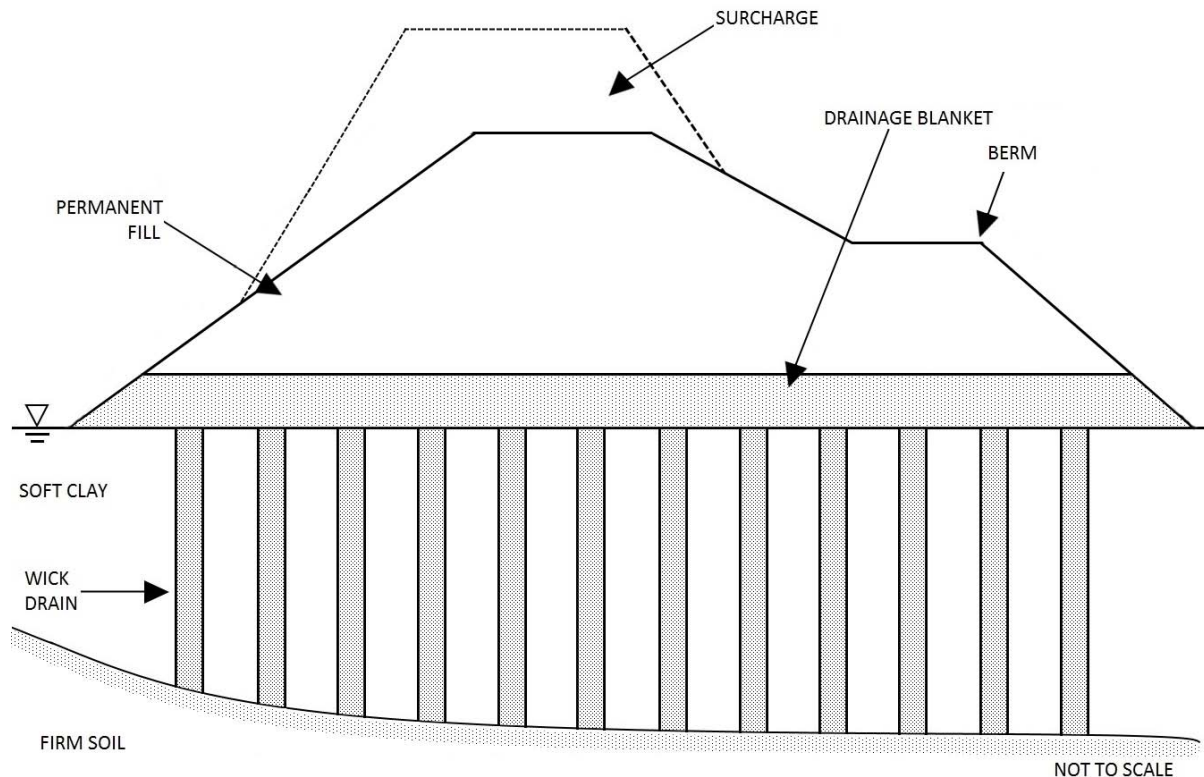
Figure 2-1. Prefabricated vertical drain installation for a highway embankment.
