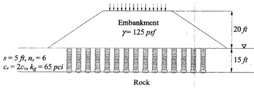
Figure 5-25. Aggregate column ground improvement layout.
