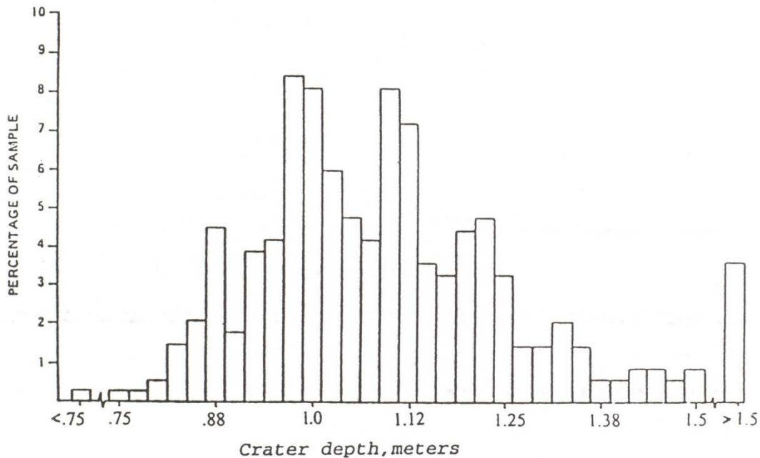
Figure 4-26. Statistical variation in crater depths at the mine spoil site in Alabama.
