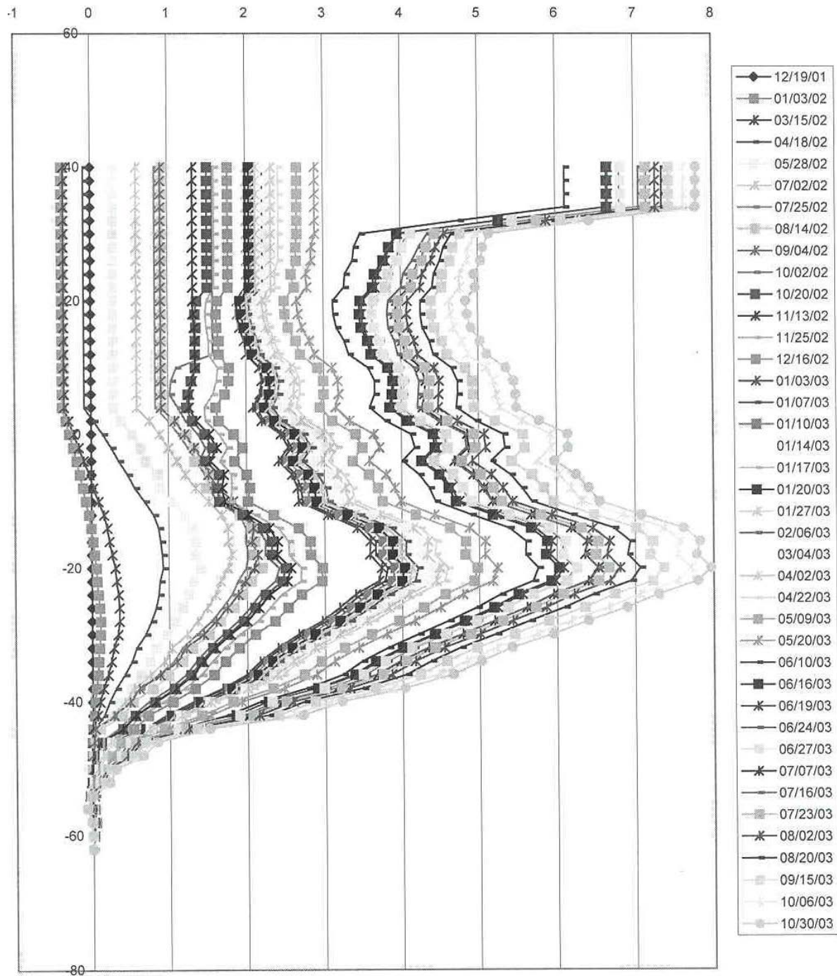
Figure 2-12. Cumulative displacement versus depth.
