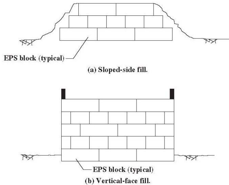
Figure 3-6. Typical EPS-block geofoam applications involving standalone embankments.
