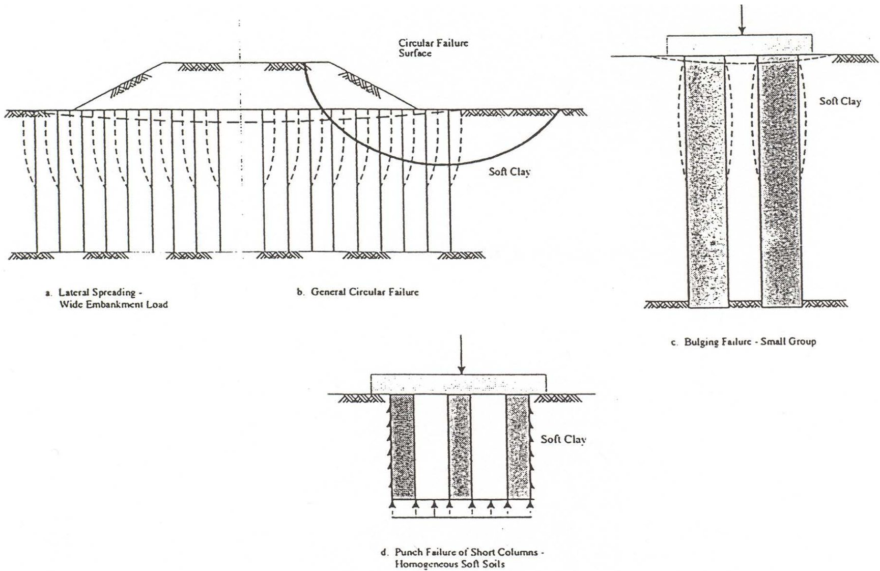
Figure 5-20. Failure modes of stone column groups.
