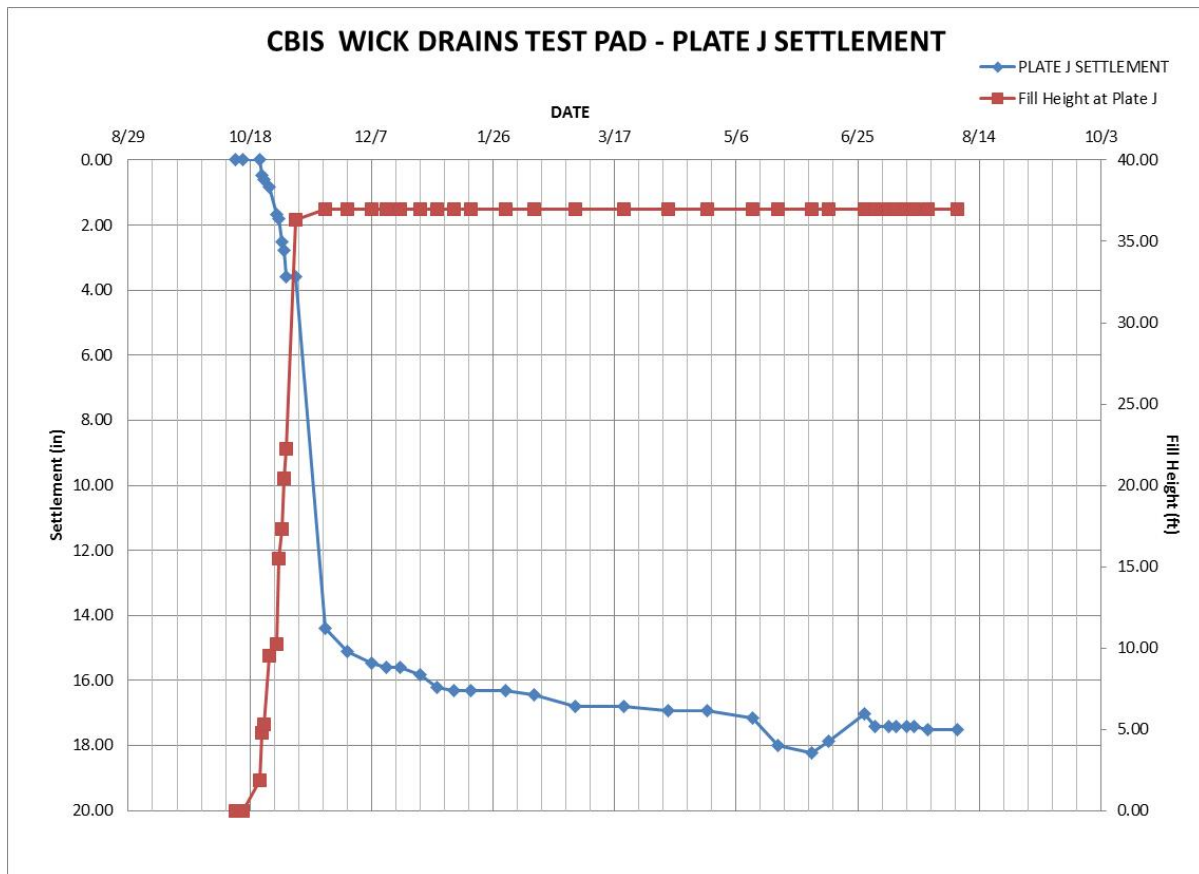
Figure 2-15. Settlement versus fill height for test pad.
