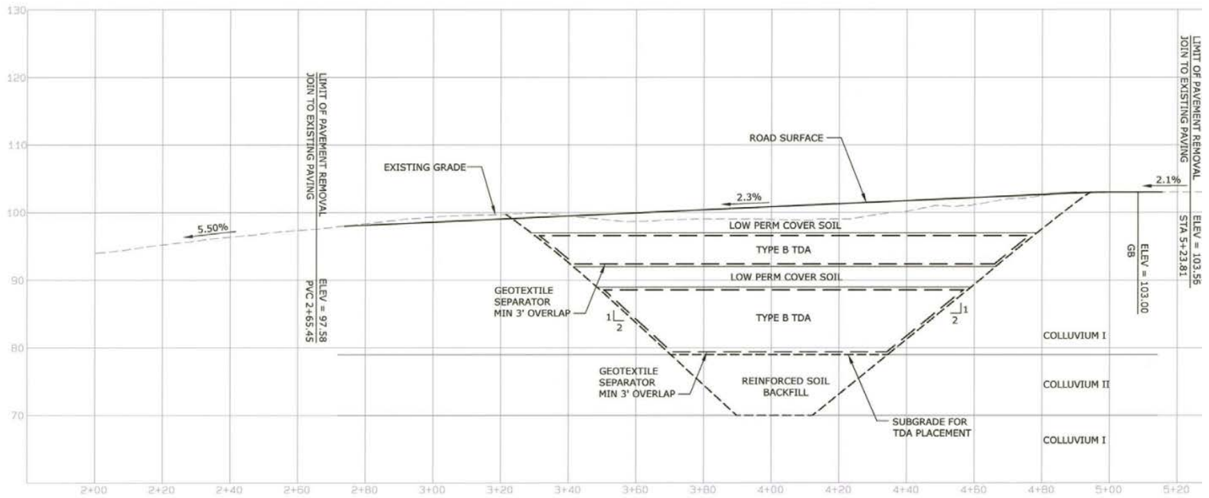
Figure 3-15. Marina Drive longitudinal section of fill replacement.
