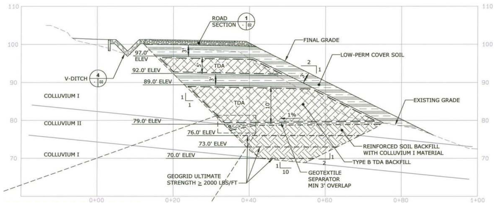
Figure 3-14. Marina Drive slope cross section.
