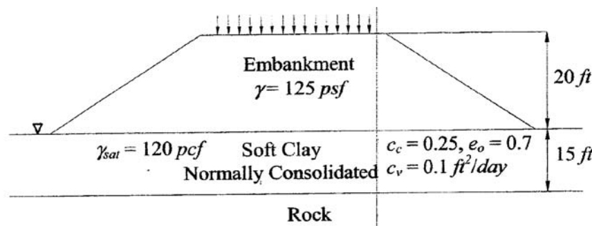
Figure 5-24. Example problem 1 geometry.
