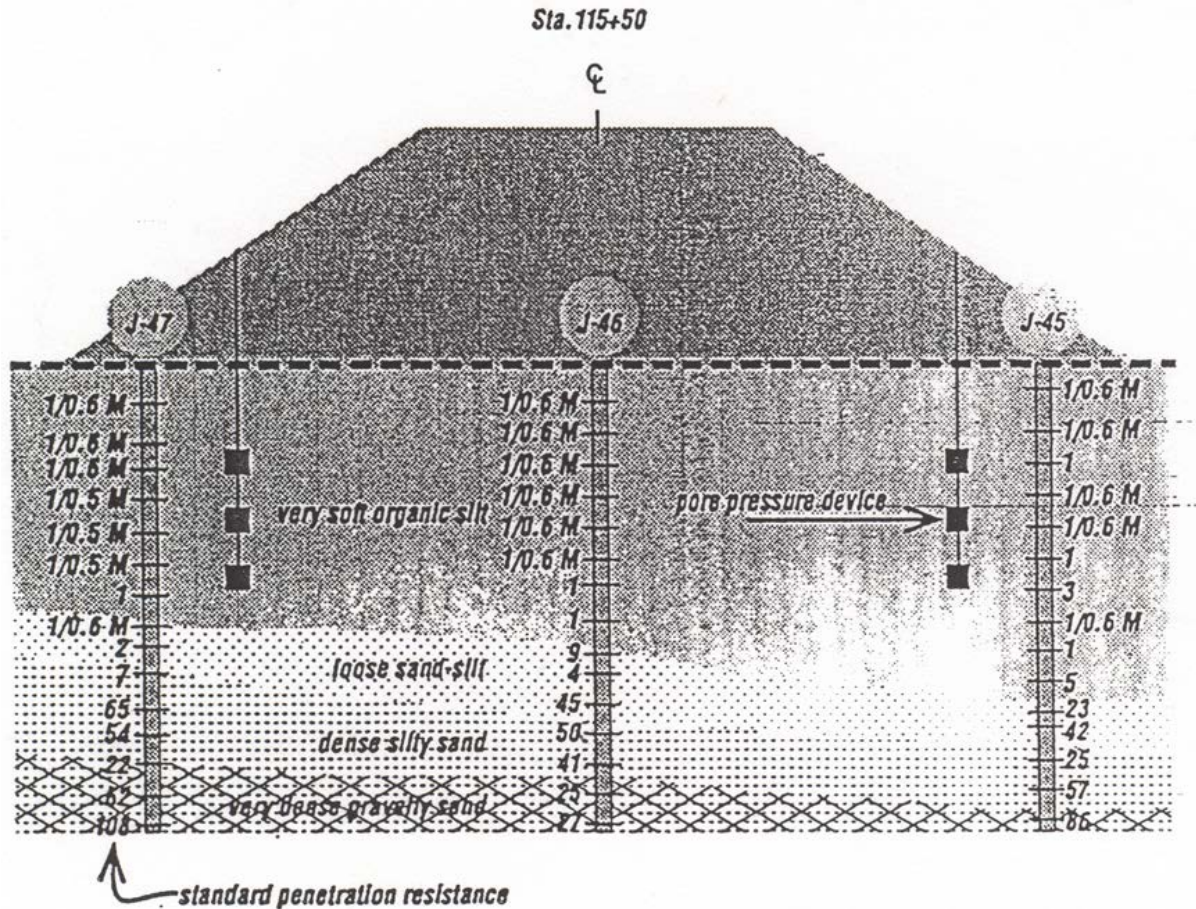
Figure 3-18. Soil cross-section at wood fiber fill location, Washington project.
