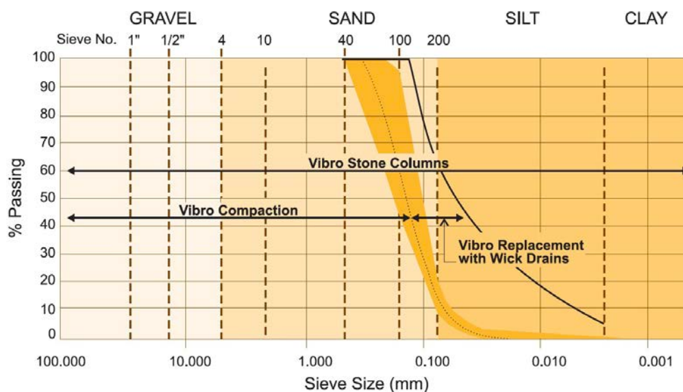
Figure 5-1. Soils applicable for stone columns.
