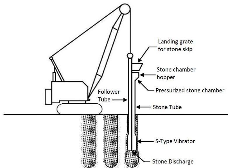
Figure 5-3. Bottom feed vibro-displacement.
