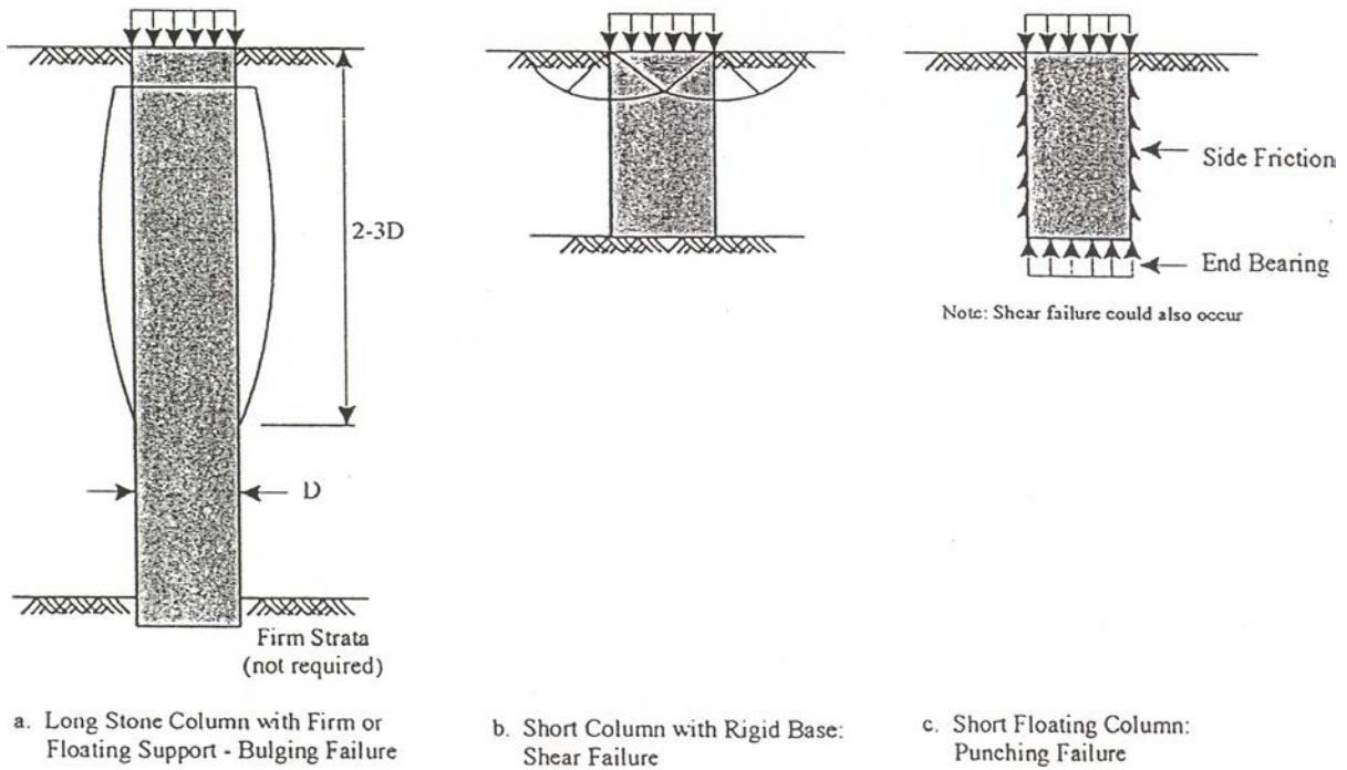
Figure 5-18. Failure modes of a single stone column in a homogenous soft layer.
