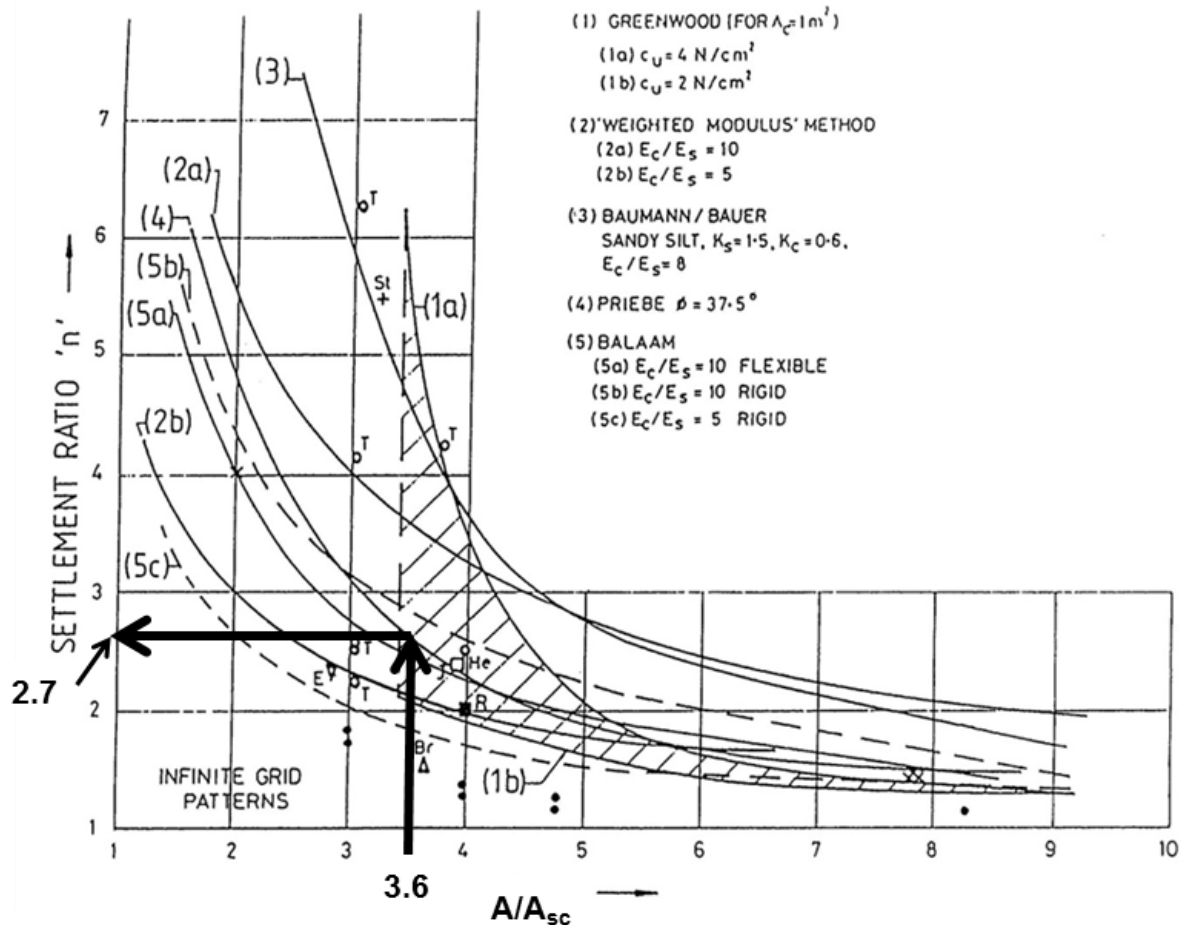
Figure 5-27. Example problem 2 settlement ratio determination.
