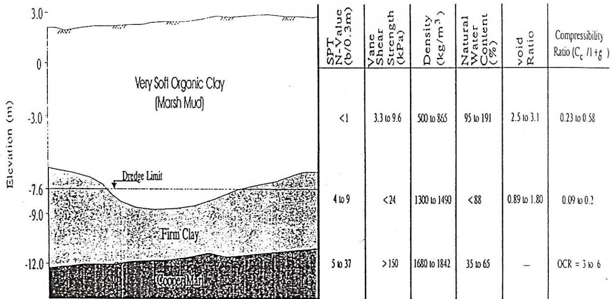
Figure 4-41. Generalized subsurface profile of Area C.
