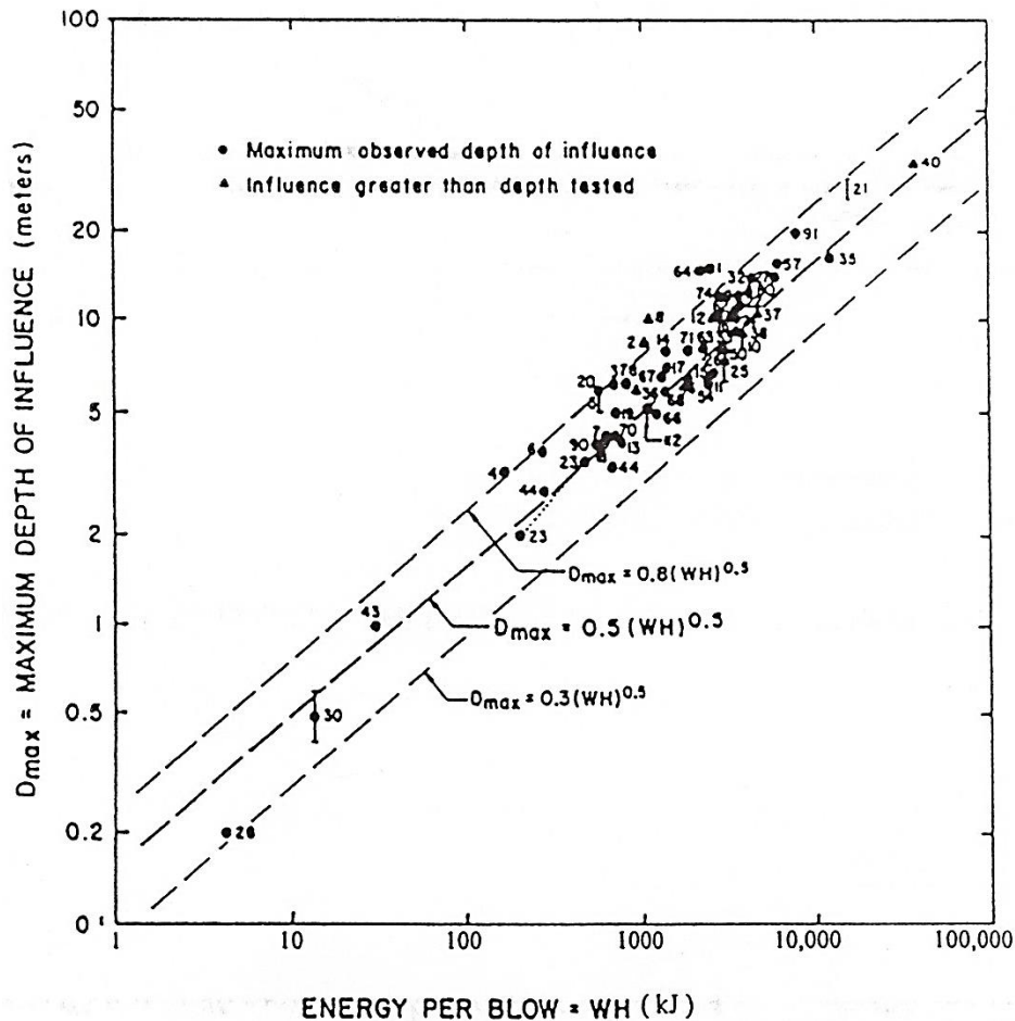
Figure 4-21. Trend between apparent maximum depth of influence and energy per drop.
