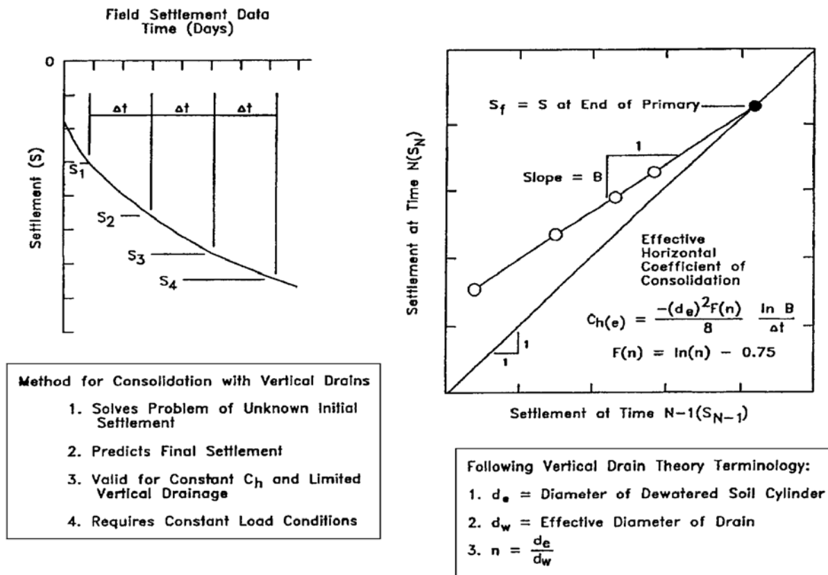
Figure 2-8. Asaoka (1978) method for determining c_h and end of primary consolidation.
