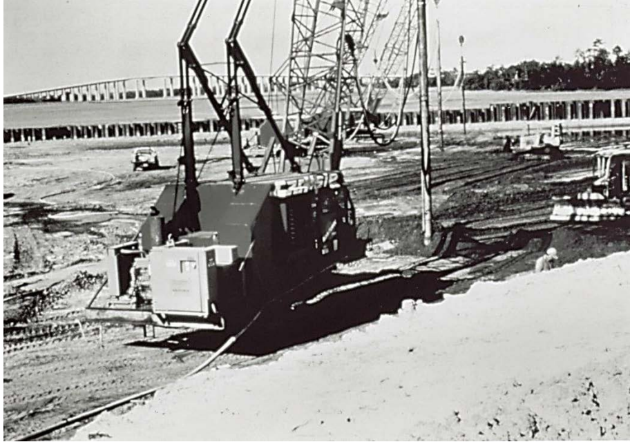
Figure 4-42. Densification of loose sand backfill during vibro-compaction at Wando Terminal.
