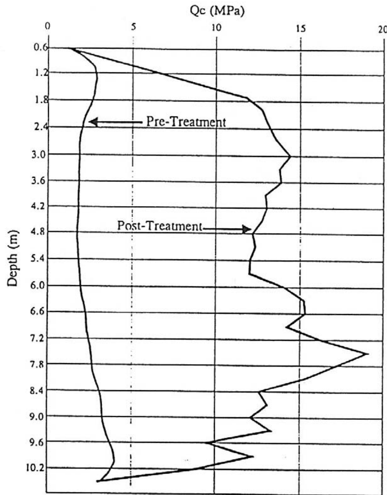
Figure 4-43. Sample cone penetration results.
