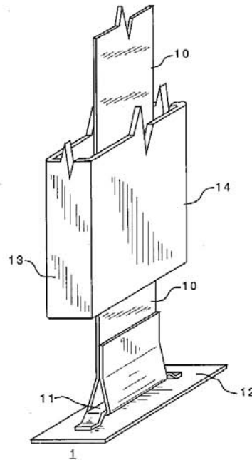
Figure 2-3. Typical prefabricated vertical drain installation equipment: installation rig (top), box mandrel (bottom).
