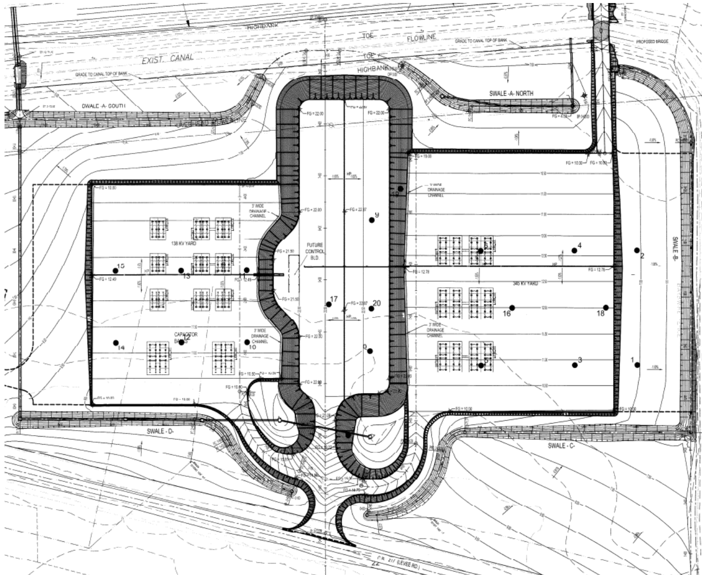
Figure 2-18. Final grading plan for Jones Creek Substation fill project.
