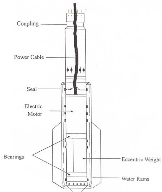
Figure 5-5. Typical vibrator cross-section.
