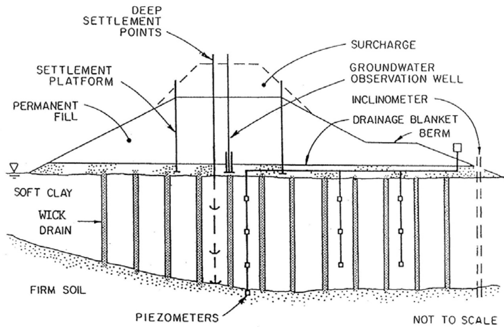
Figure 2-14. PVD Installation showing typical instrumentation and monitoring.
