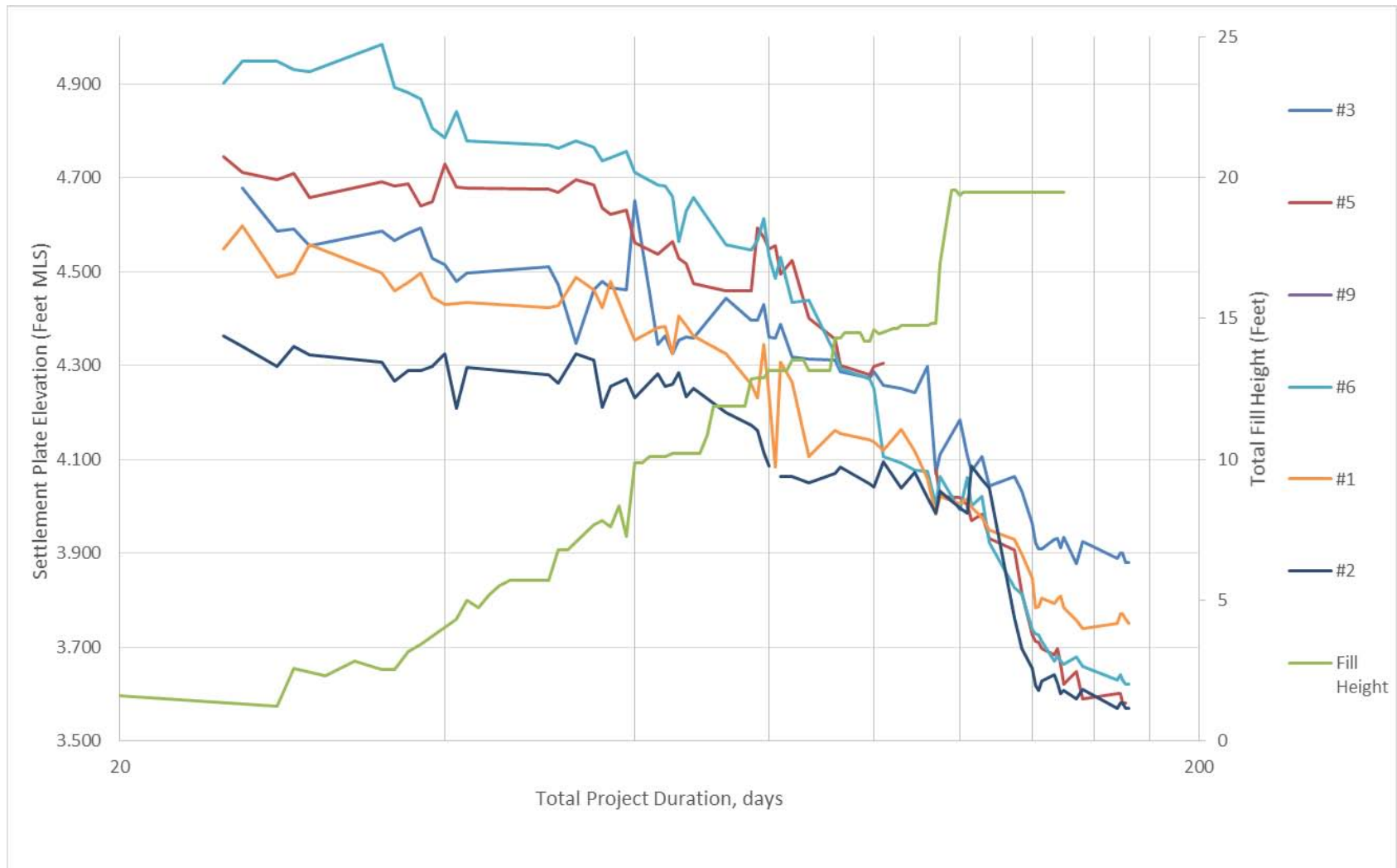
Figure 2-19. Settlement plate data and fill height versus project duration.
