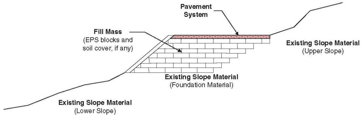
Figure 3-7. Major components of an EPS-block geofoam slope system.
