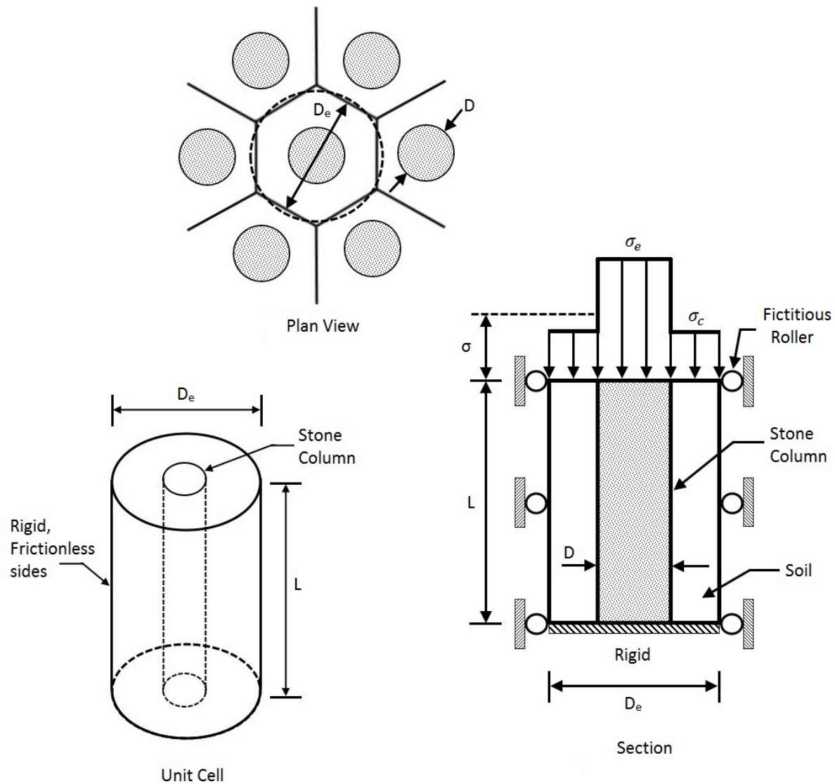
Figure 5-17. Unit cell idealization.
