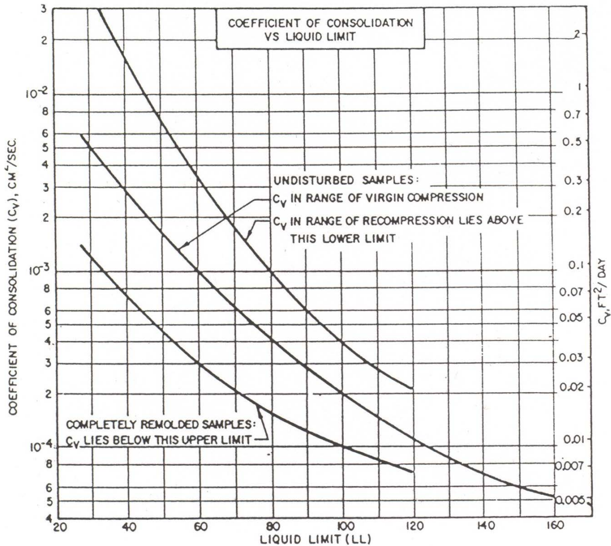
Figure 2-10. Coefficient of consolidation versus liquid limit.
