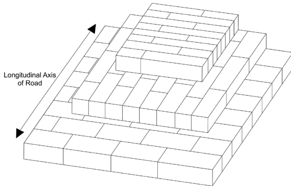
Figure 3-9. Isometric view of typical EPS block layout.
