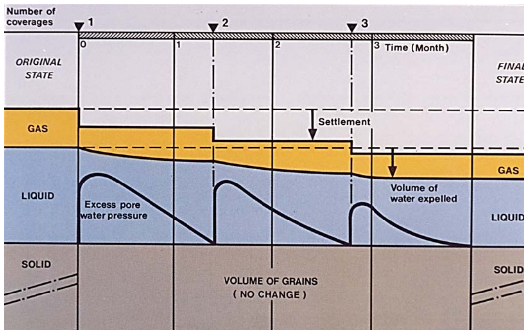
Figure 4-4. Phase diagram model of soil behavior during deep dynamic compaction.
