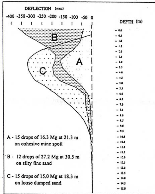
Figure 4-8. Lateral movements at 3 m (10 feet) from drop point.
