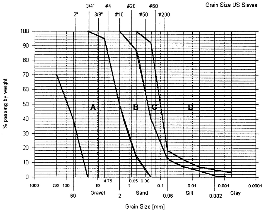
Figure 4-27. Range of soil types treated by vibro-compaction.
