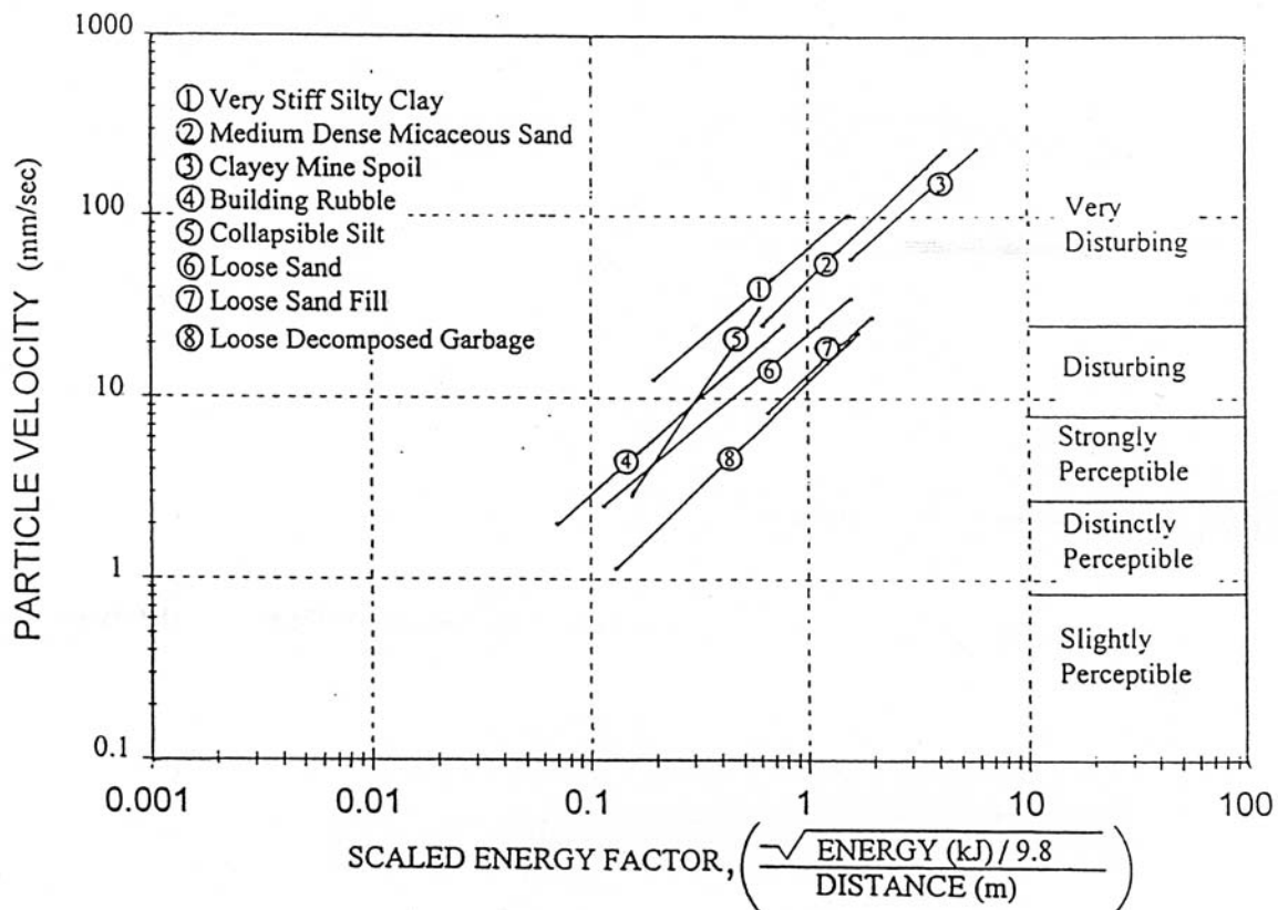
Figure 4-7. Scaled energy factor versus particle velocity.
