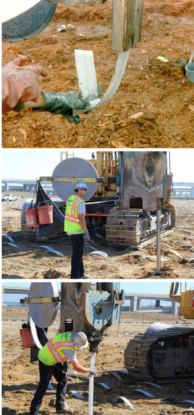
Figure 2-4. Typical prefabricated vertical drain installation procedure: placing the anchor on the drain (top), inserting the mandrel into the ground (middle), cutting the drain after withdrawing the mandrel (bottom).
