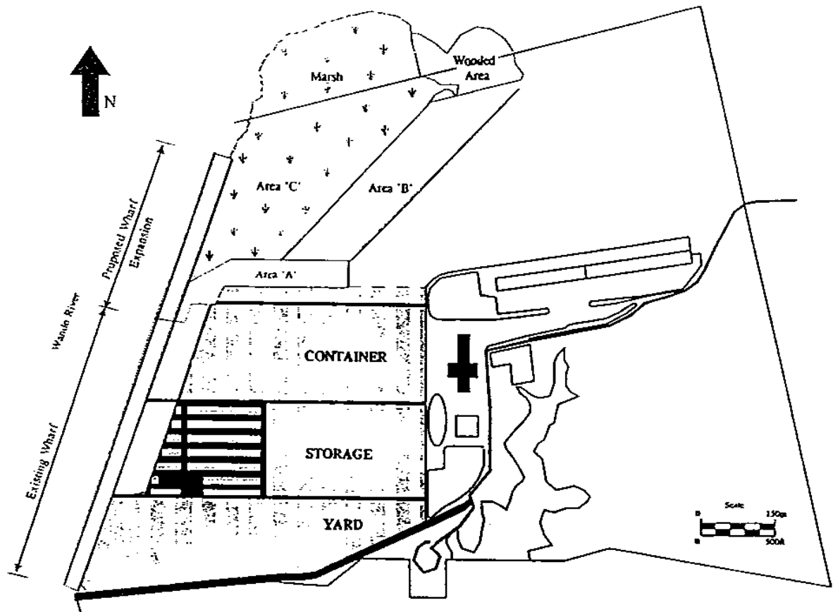
Figure 4-39. State Pier 41, Wando Terminal.
