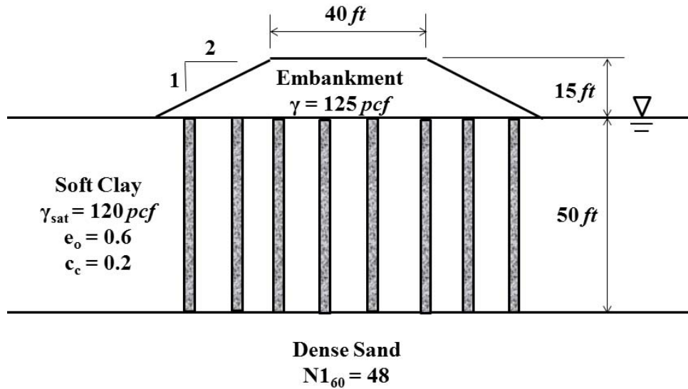
Figure 5-26. Example problem 2 geometry and soils.
