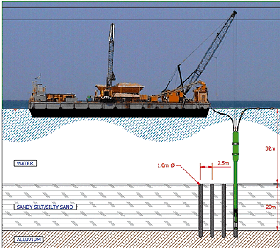
Figure 5-10. Marine double-lock gravel pump.
