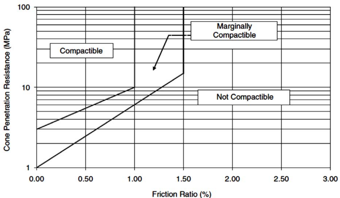
Figure 4-28. Soil compactibility based on cone penetration resistance and friction ratio.
