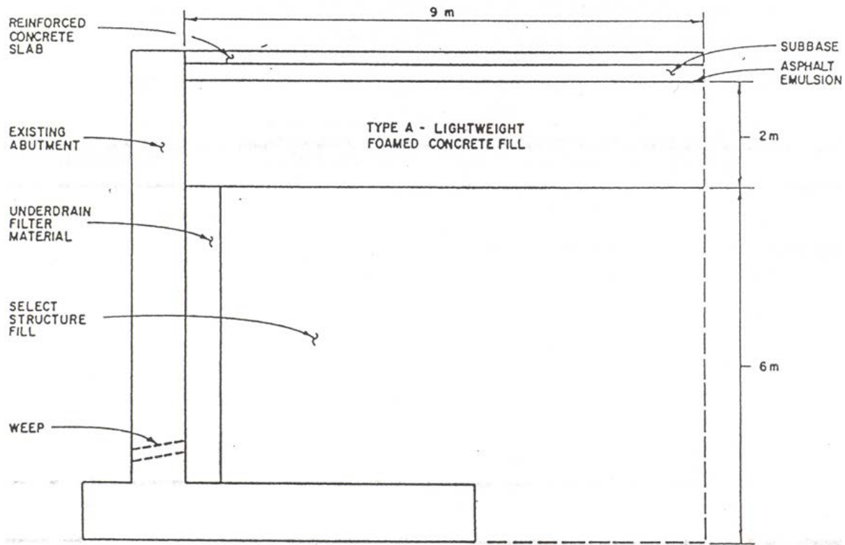
Figure 3-13. Foamed concrete fill behind existing abutment, New York project.
