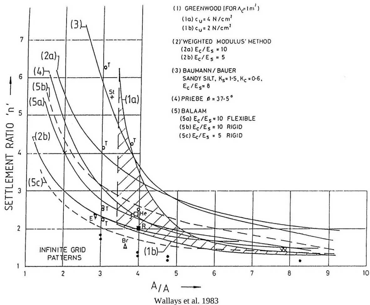
Figure 5-21. Comparison of elastic theories and field observations.
