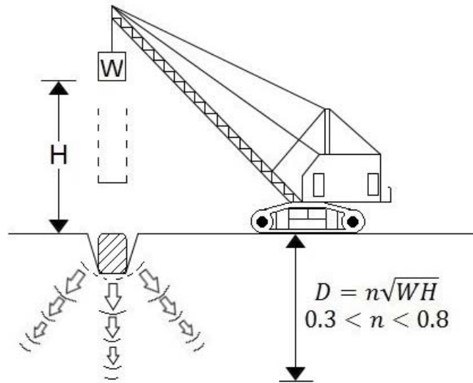
Figure 4-1. Schematic illustration of deep dynamic compaction.
