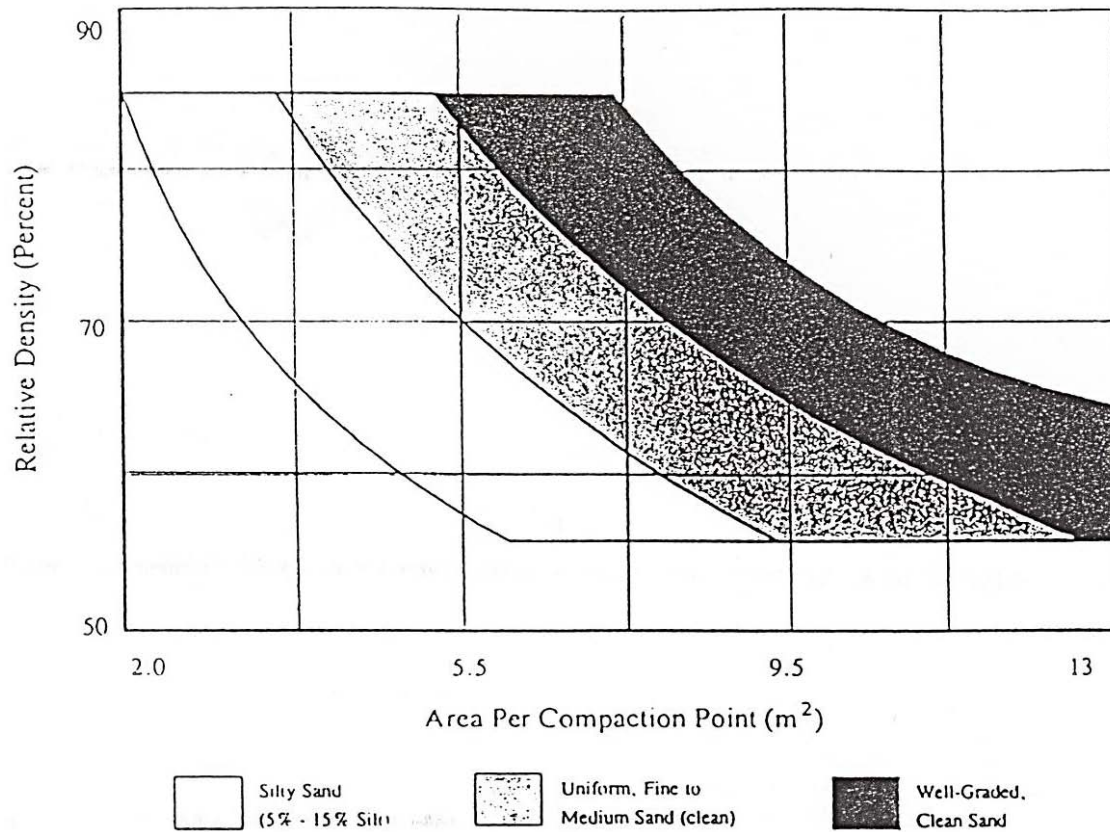
Figure 4-33. Approximate variation of relative density with tributary area.
