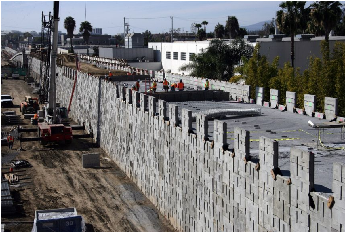
Figure 3-2. Foamed concrete MSE wall backfill for light rail project in California.
