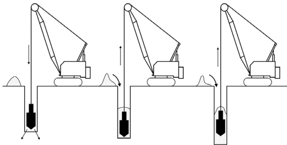
Figure 5-2. Top feed vibro-replacement.
