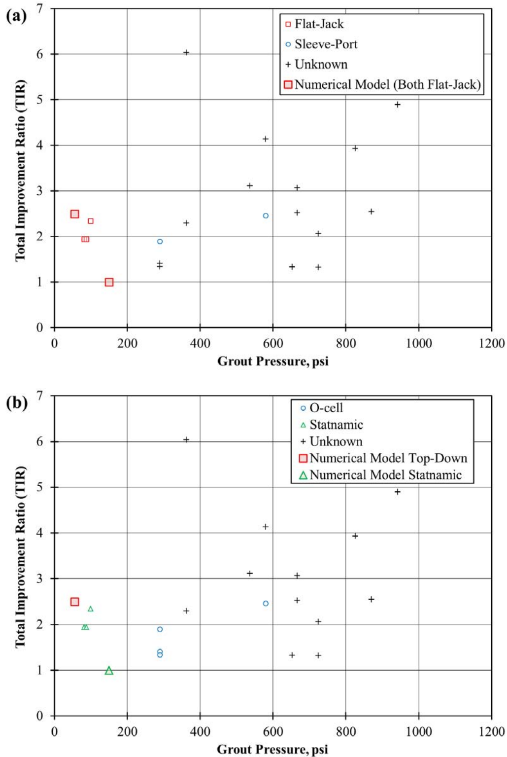
Figure 9.5: TIR vs. grout pressure for shafts tipped in clay, plotted according to: (a) grouting apparatus, and (b) load test type.
