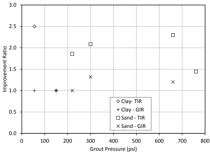
Figure 8.20: Calculated GIR and TIR for the respective cases plotted as a function of the maximum sustained grout pressure for the respective shafts.
