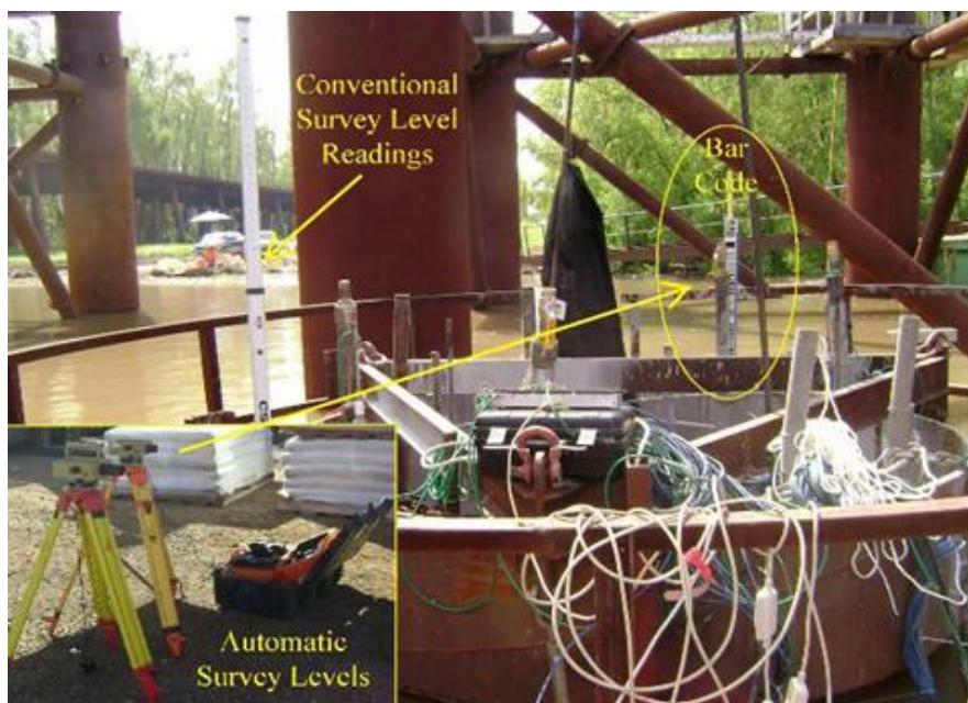
Figure 6.3: Photograph of the survey level readings (automatic and manual) during grouting (courtesy of Applied Foundation Testing).
