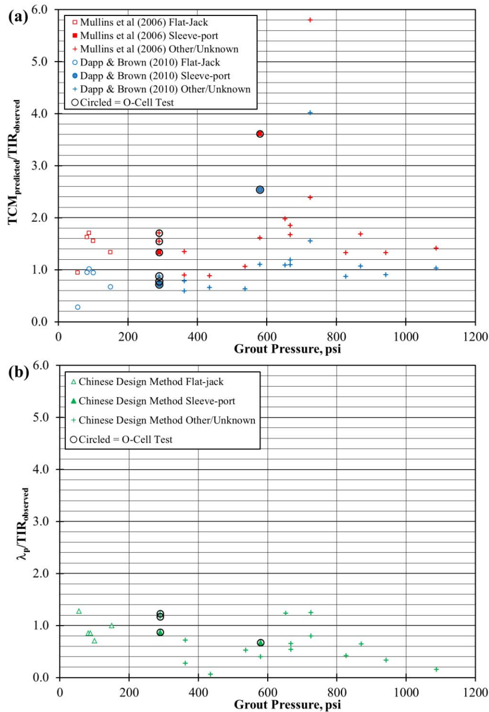
Figure 9.9: Ratio of predicted TCM to observed TIR for: (a) TCM using GPI from load test measurements, and (b) component multiplier methods vs. maximum reported grout pressure for shafts tipped in clay.
