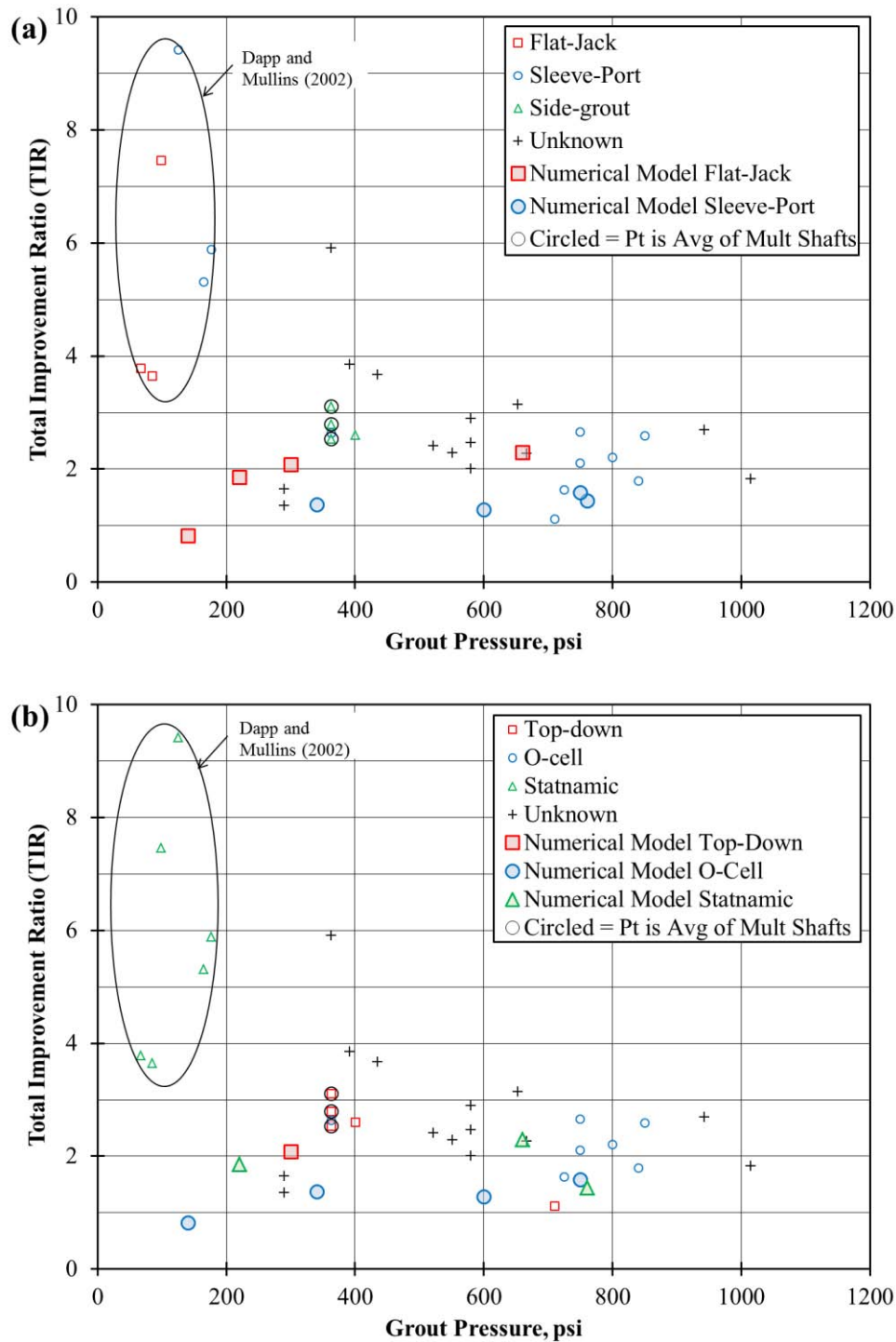
Figure 9.2: TIR vs. grout pressure for shafts tipped in sand, plotted according to: (a) grouting apparatus, and (b) load test type.
