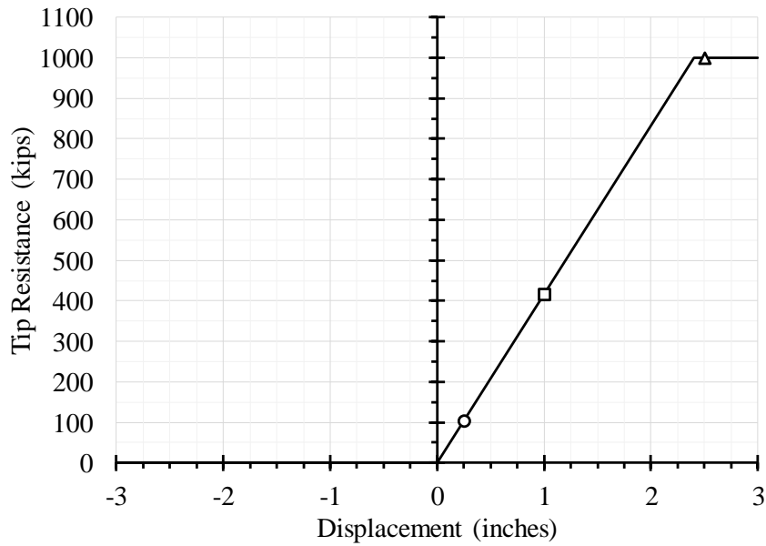
Figure 8.3: Load-transfer ( q - w ) model for tip resistance.
