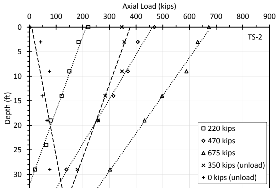
Figure 10.10: Interpreted load transfer for Test Shaft TS-2.
