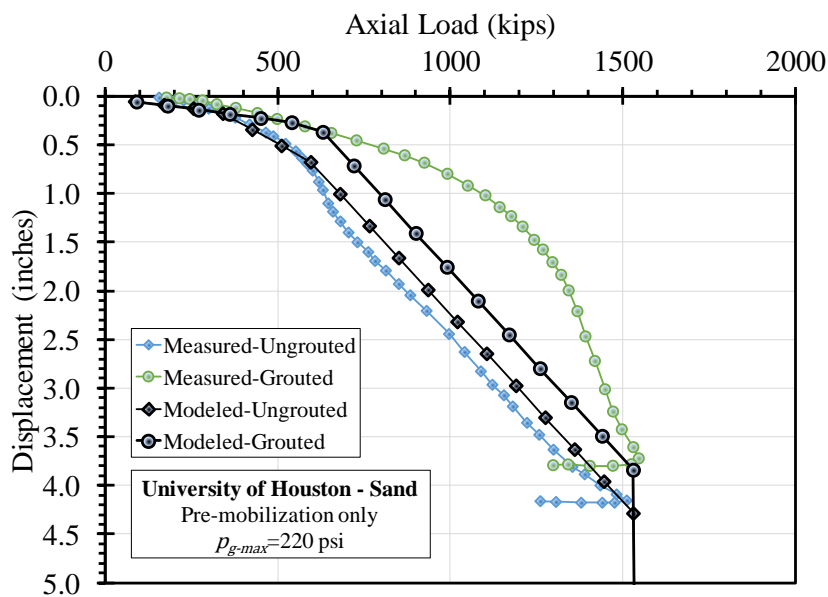
Figure 8.13: Predicted and measured load-displacement response for ungrouted and post-grouted test shafts from the University of Houston Sand site. Predicted response for grouted shaft considers pre-mobilization only with no ground improvement.
