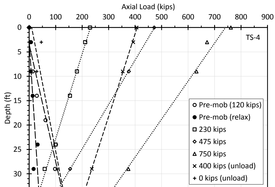
Figure 10.11: Interpreted load transfer for Test Shaft TS-4.
