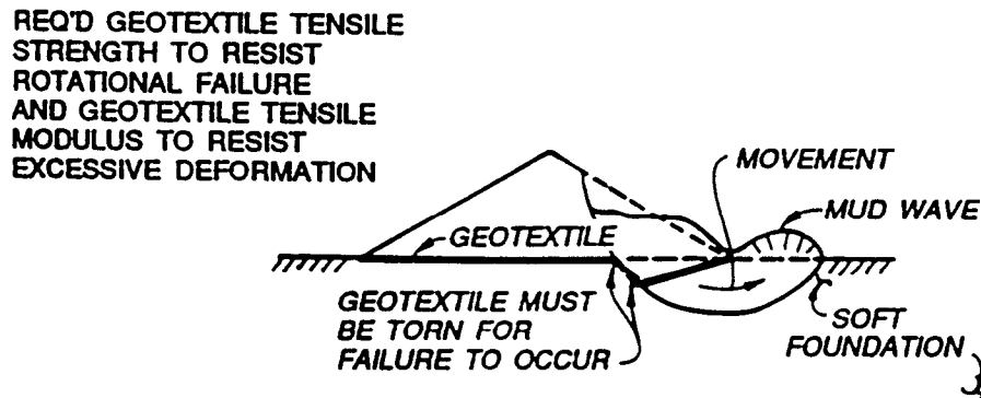
b. POTENTIAL EMBANKMENT ROTATIONAL SLOPE/FOUNDATION FAILURE
