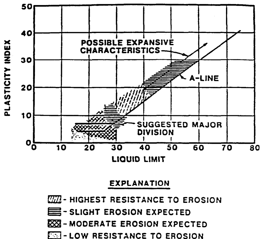
SUGGESTED TREND OF EROSION CHARACTERISTICS FOR FINE-GRAINED COHESIVE SOILS WITH RESPECT TO PLASTICITY
