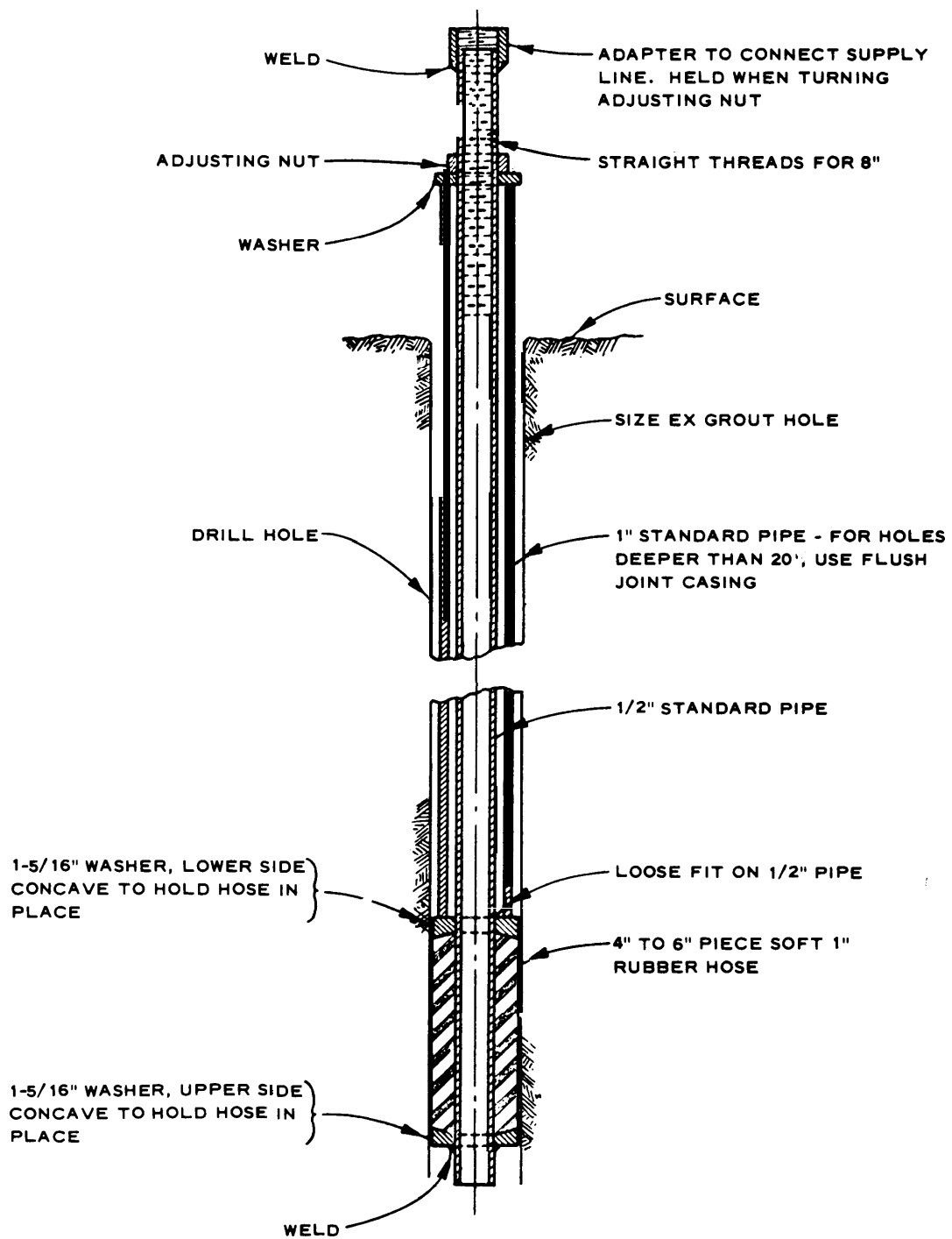
Figure 19. Mechanical packer
