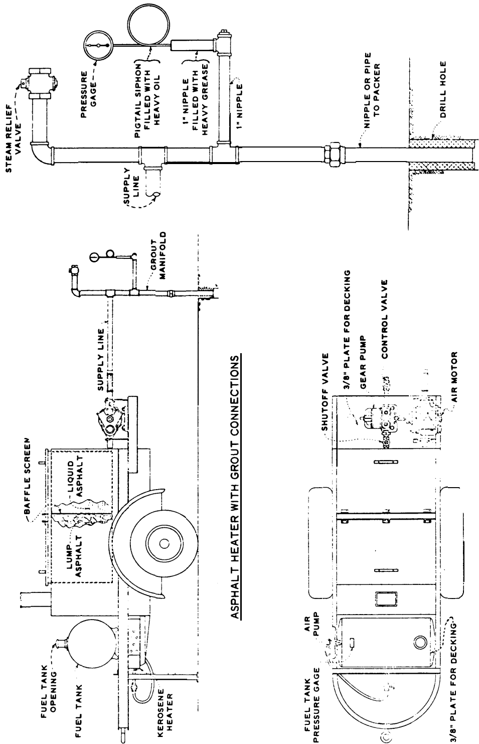
TYPICAL ASPHALT GROUTING MANIFOLD AND CONNECTIONS
