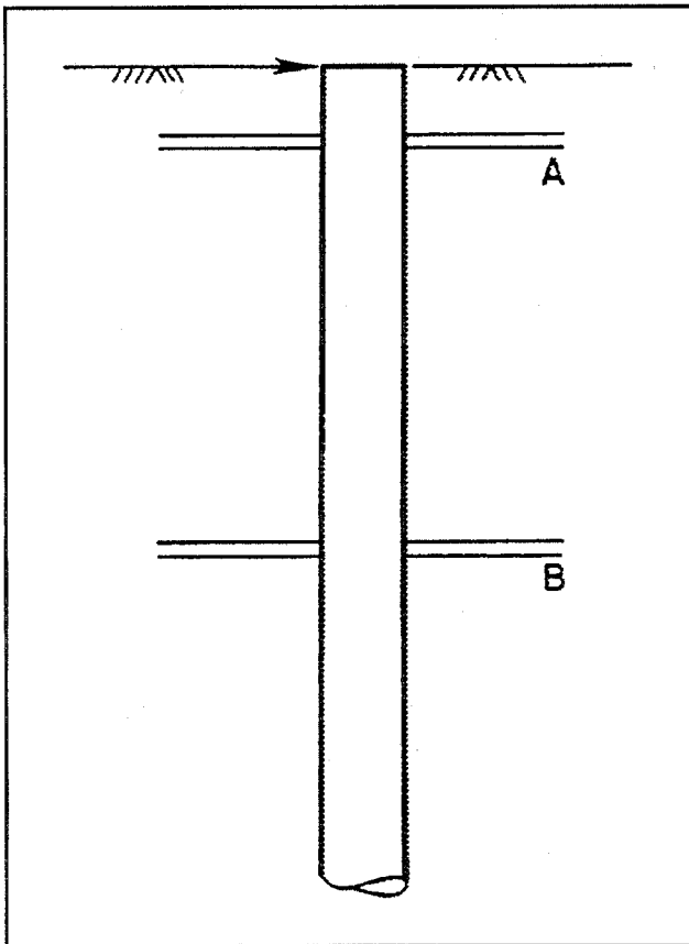
Figure 4-3. Pipe pile and soil elements
