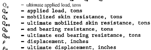
Figure 1-5. Axial-load deflection relationship
