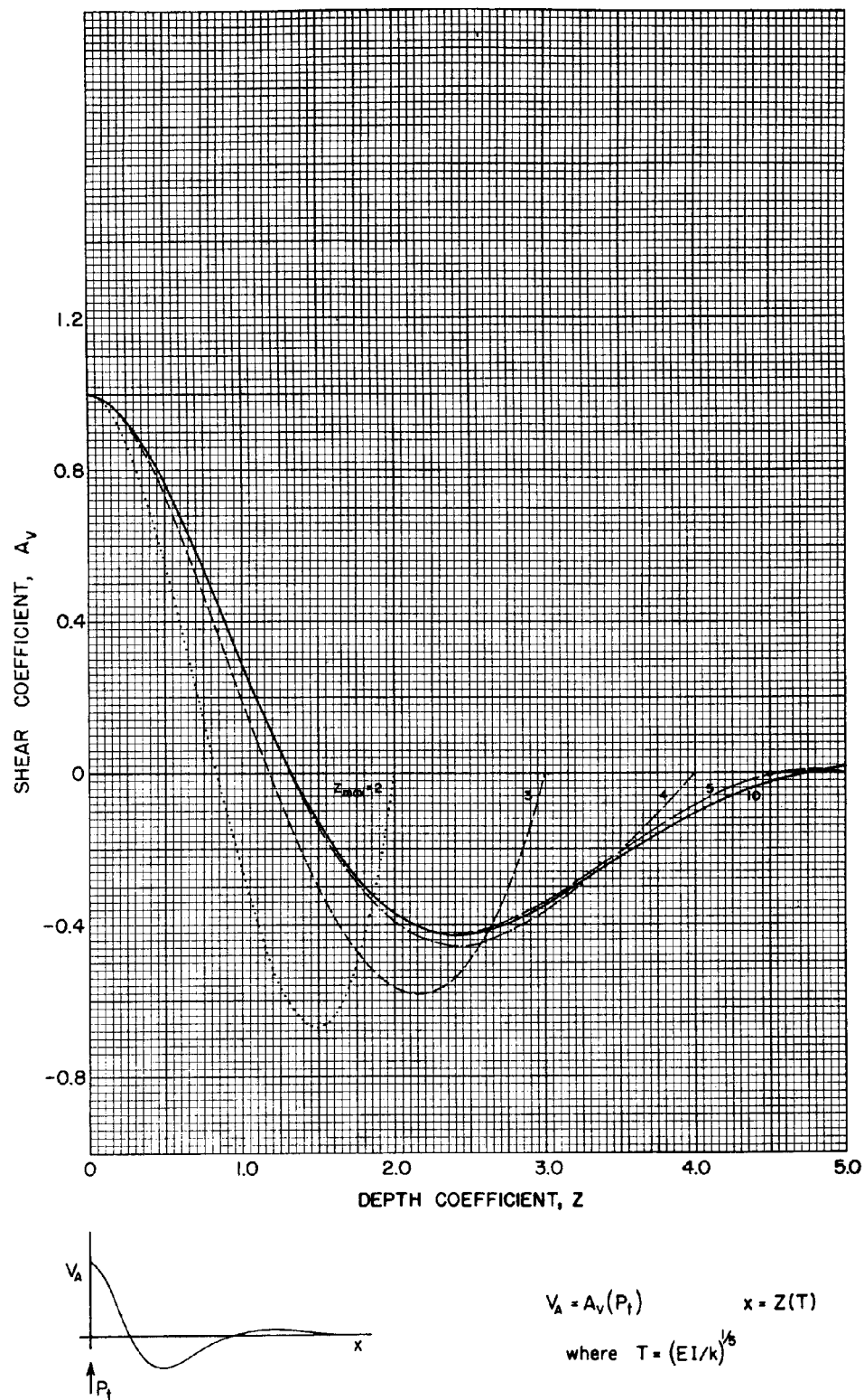
Figure 4-23. Shear produced by lateral load at mudline
