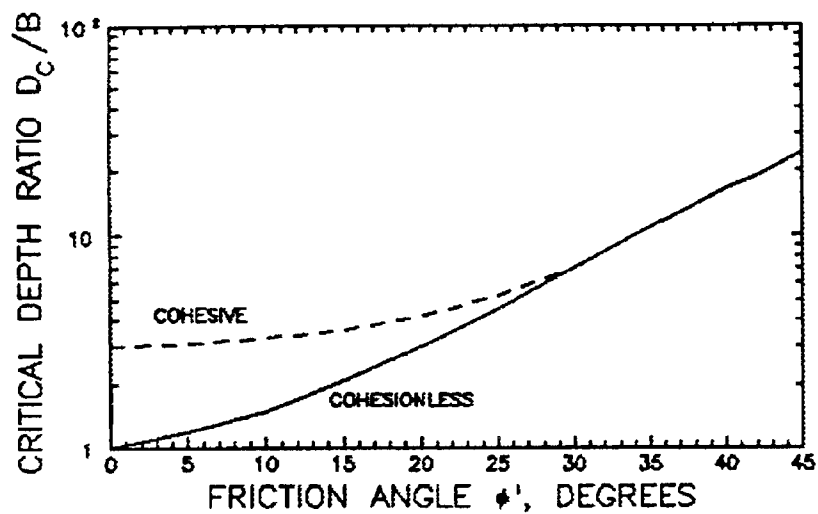
a. D_c/B VERSUS FRICTION ANGLE
