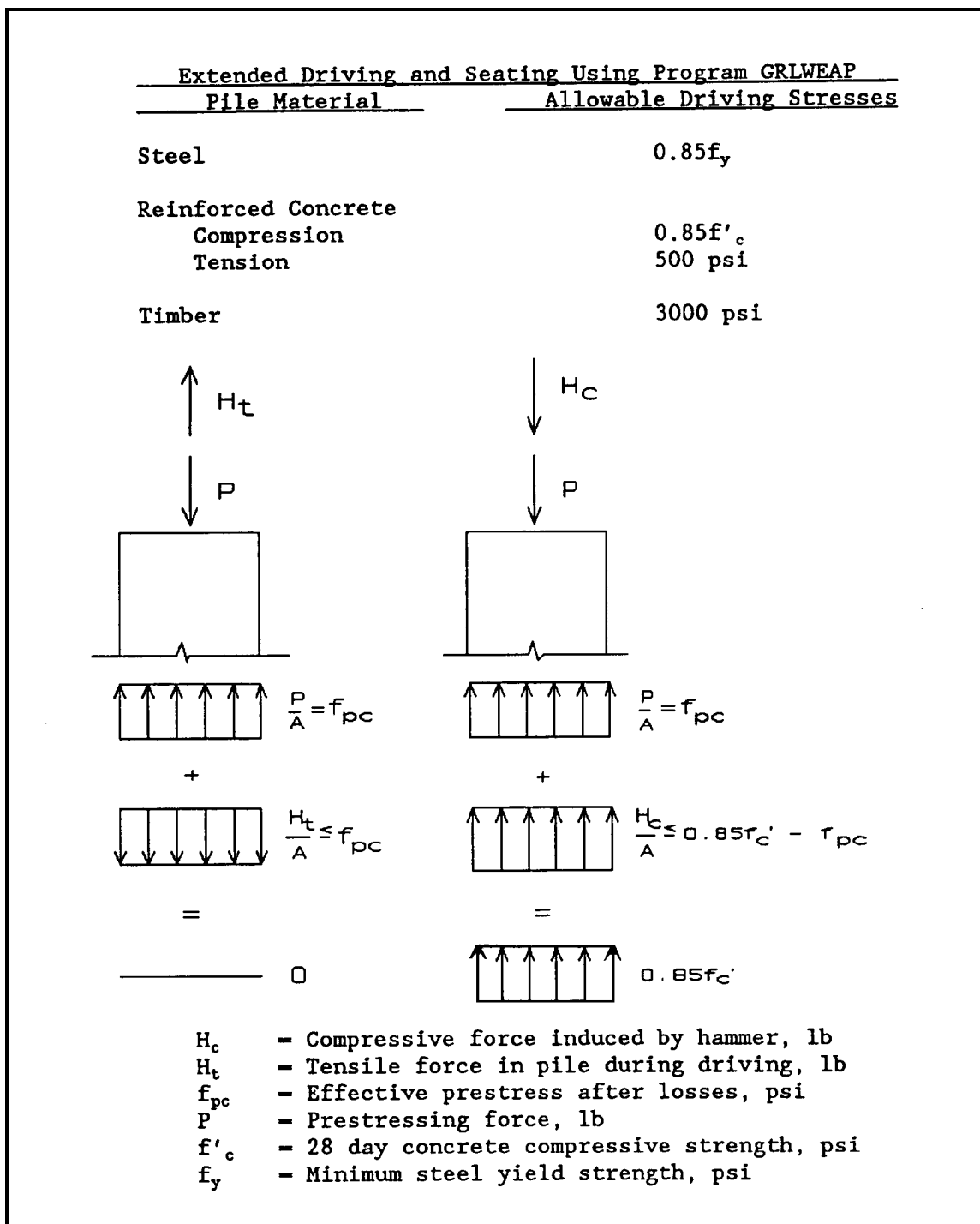
Figure 2-2. Limits to pile driving stresses
