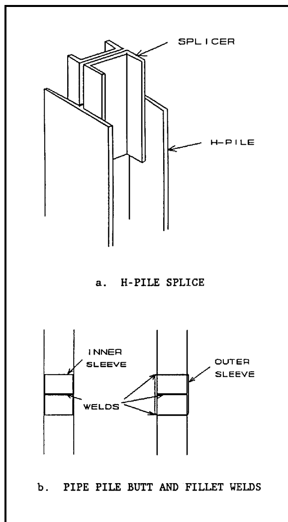
Figure 1-3. Steel pile splices
