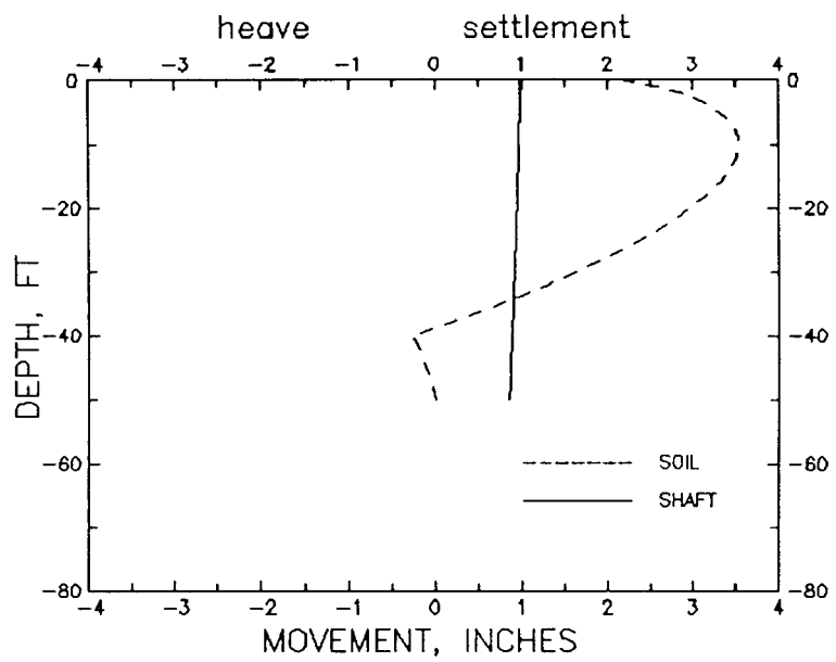
c. DISPLACEMENT-DEPTH BEHAVIOR, FILE MDEP
