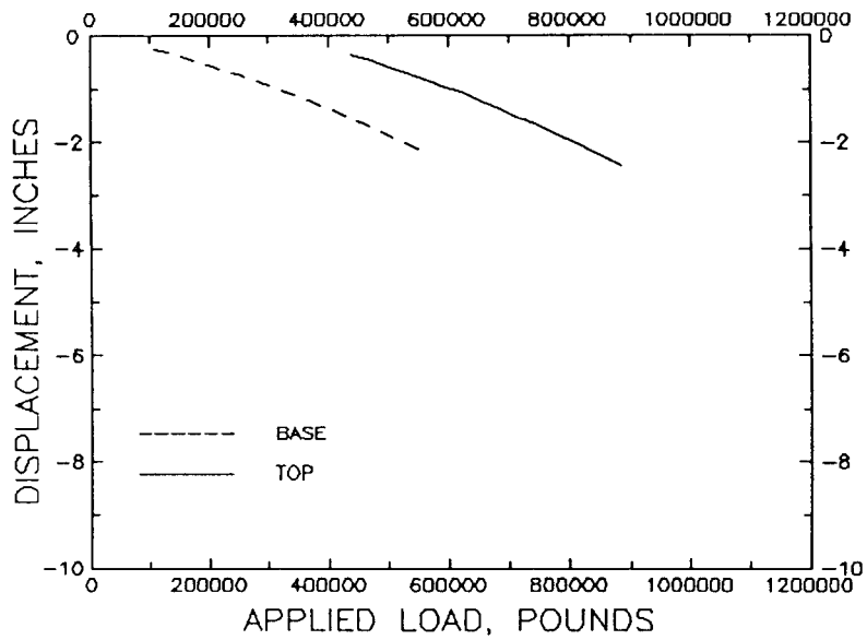
a. LOAD-DISPLACEMENT BEHAVIOR, FILE LDCOM
