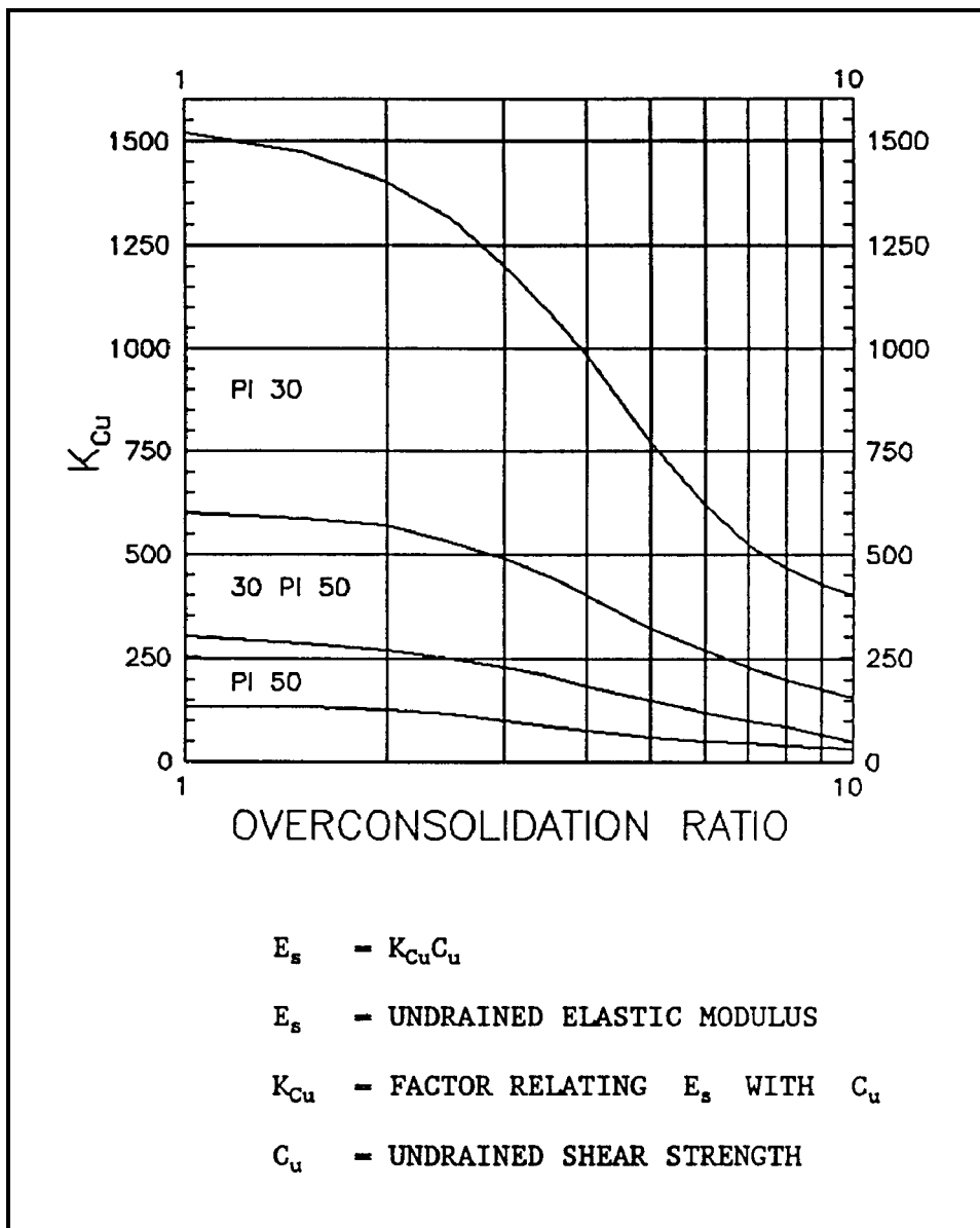
Figure 1-8. Variation K_{cu} for clay with respect to undrained shear strength and overconsolidation ratio
