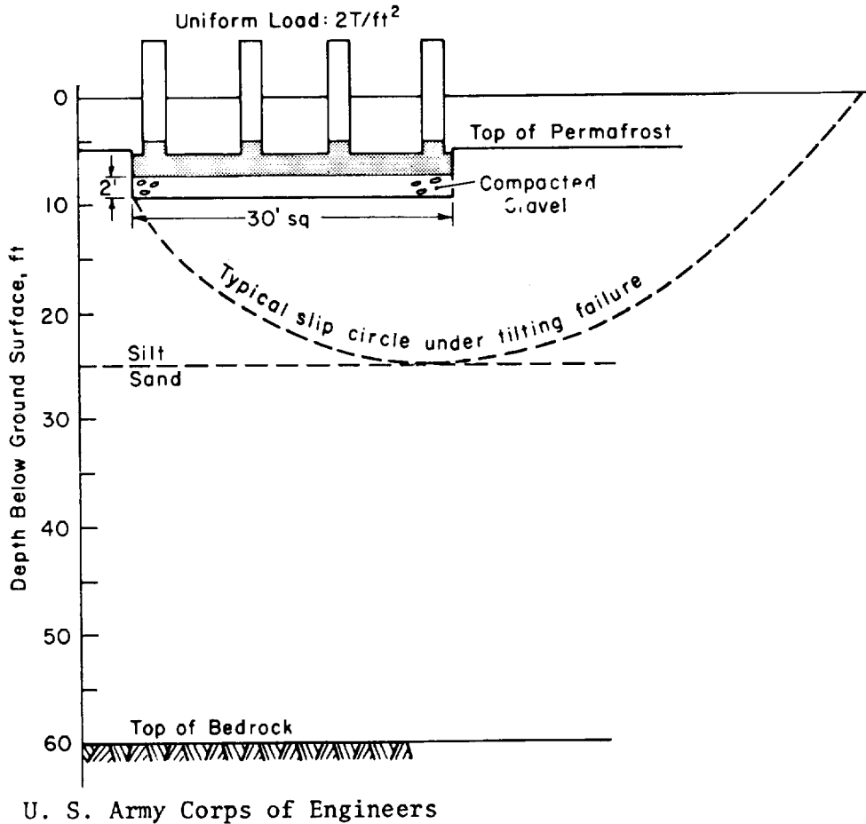
Figure 4-68. Conditions for bearing capacity analysis of square raft (by CRREL). Desired factor of safety = 2.0. A uniform load can be assumed for closely spaced individual footings or piers, or the area beneath piling.
