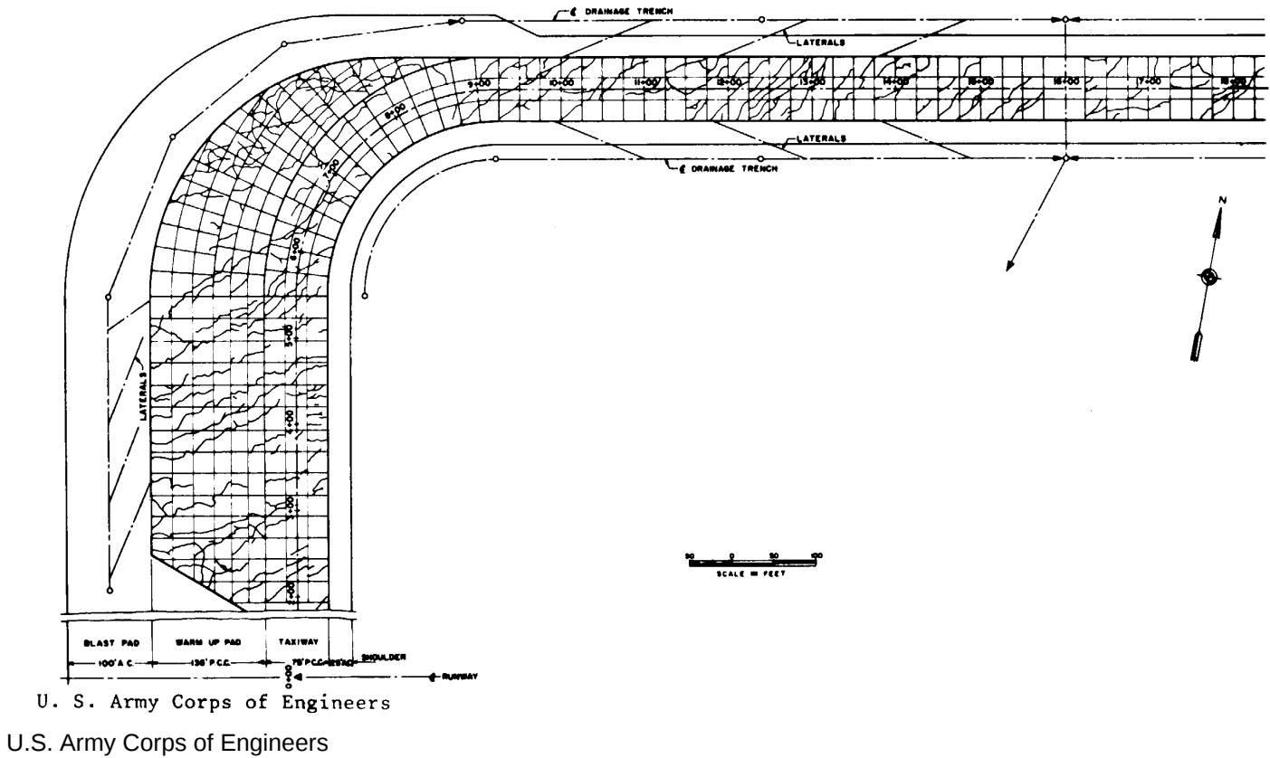
Figure 3-8. Pattern of cracks in taxiway pavement, Elmendorf AFB, Alaska
