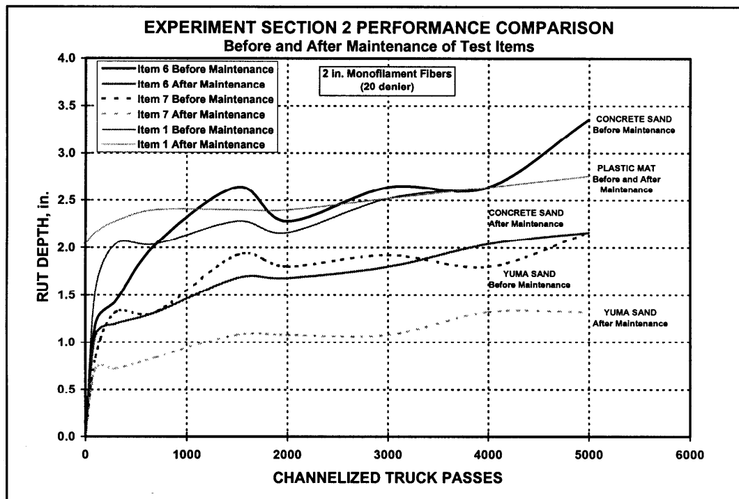
Figure 41. Effect of maintenance on items 1, 6, and 7 of section two
