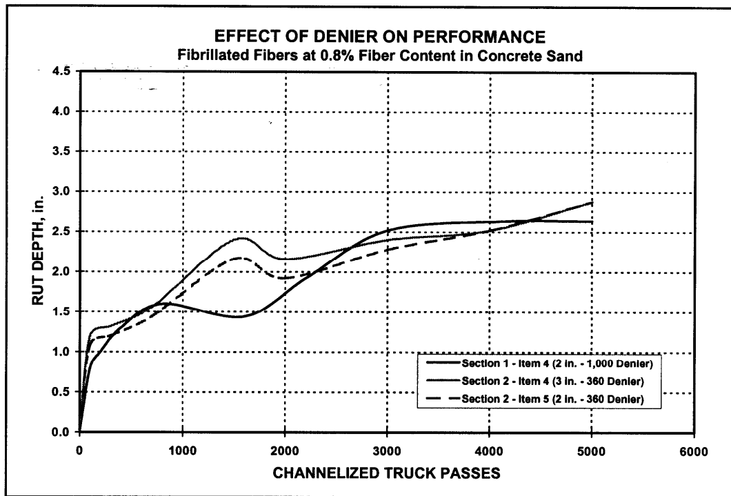
Figure 40. Performance comparison of two deniers of fibrillated fibers
