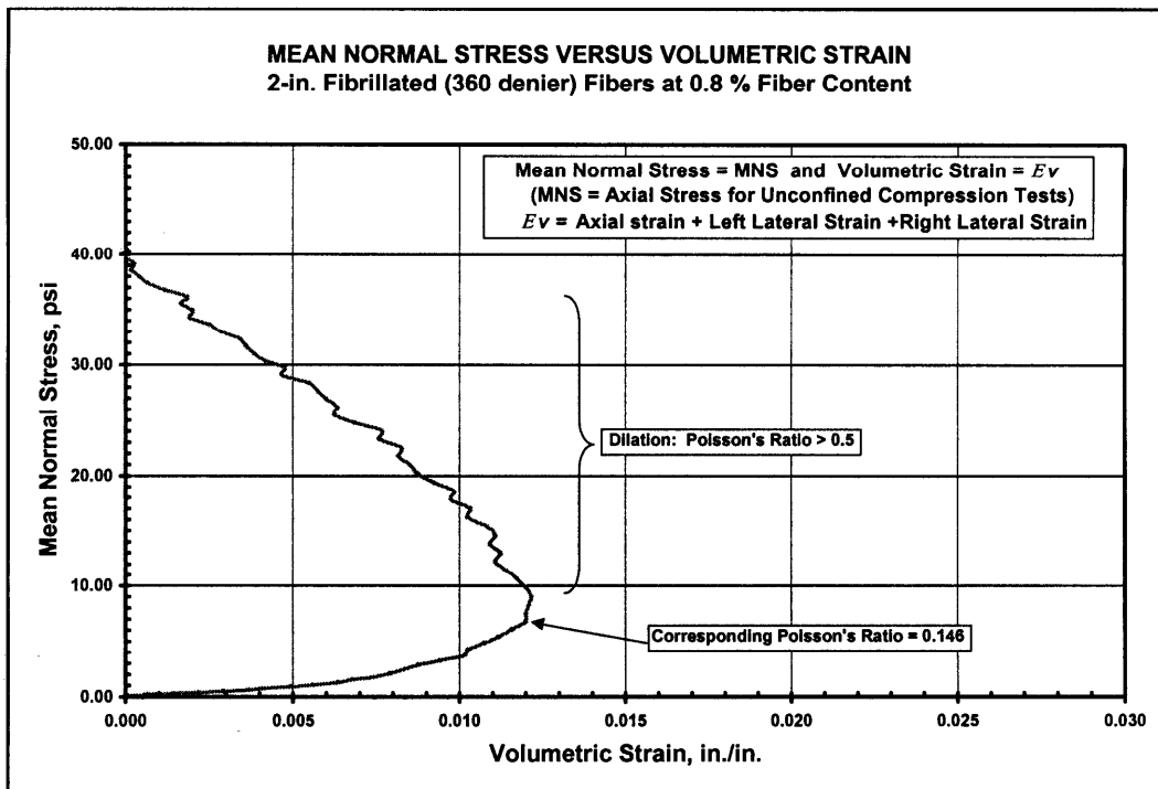
Figure 47. Typical plot of mean normal stress versus volumetric strain for fiber-stabilized materials
