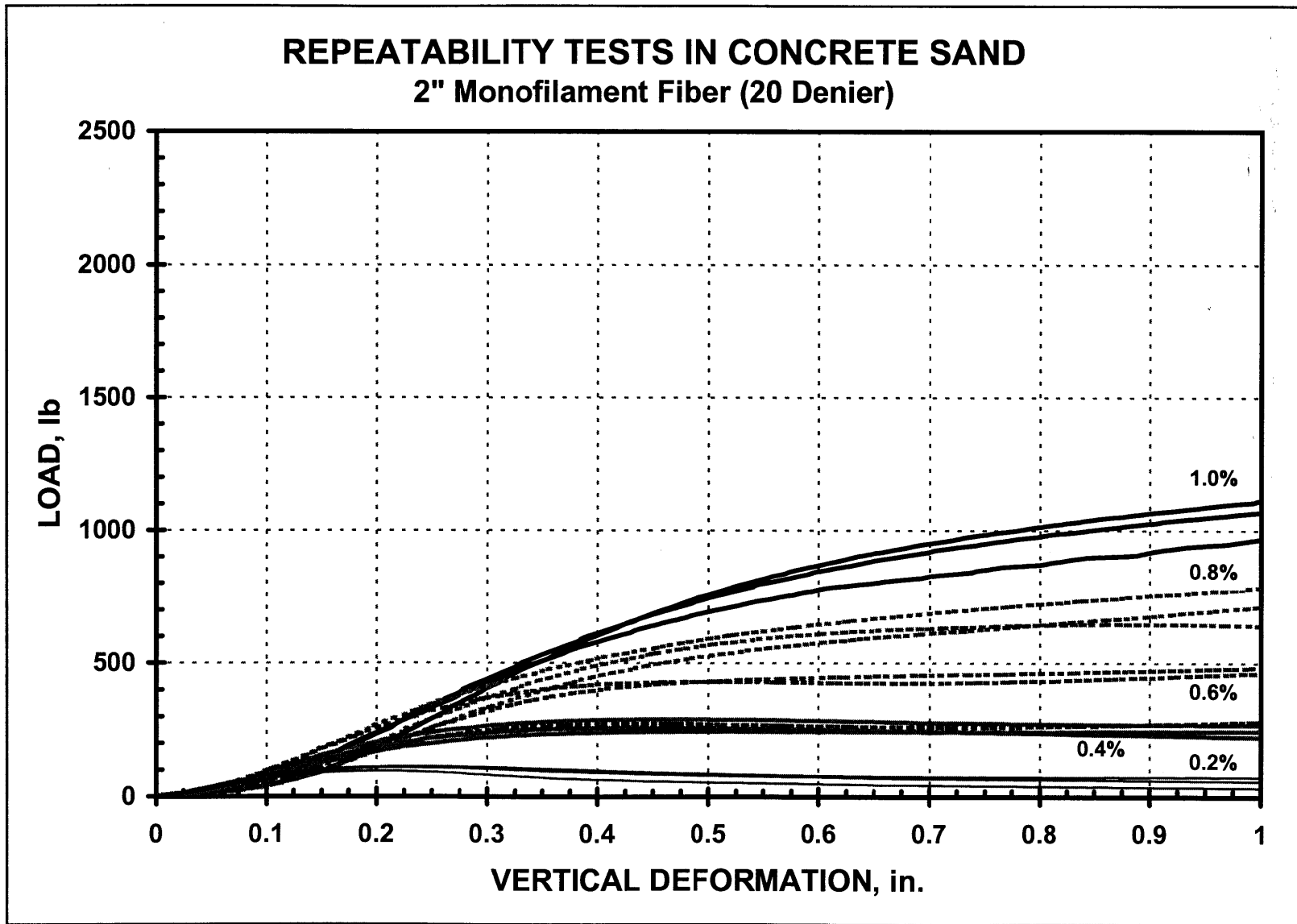
Figure 28. Repeatability tests for 2-in. monofilament (20 denier) fibers in concrete sand
