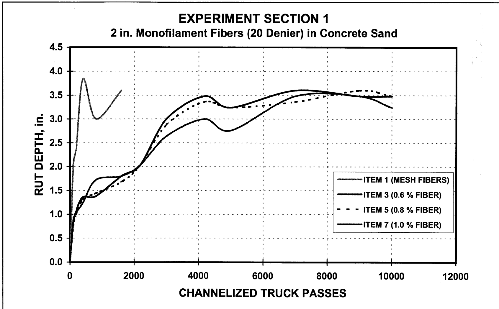
Figure 33. Rut depth measurements for the monofilament fiber items 1, 3, 5, and 7 of experiment section one
