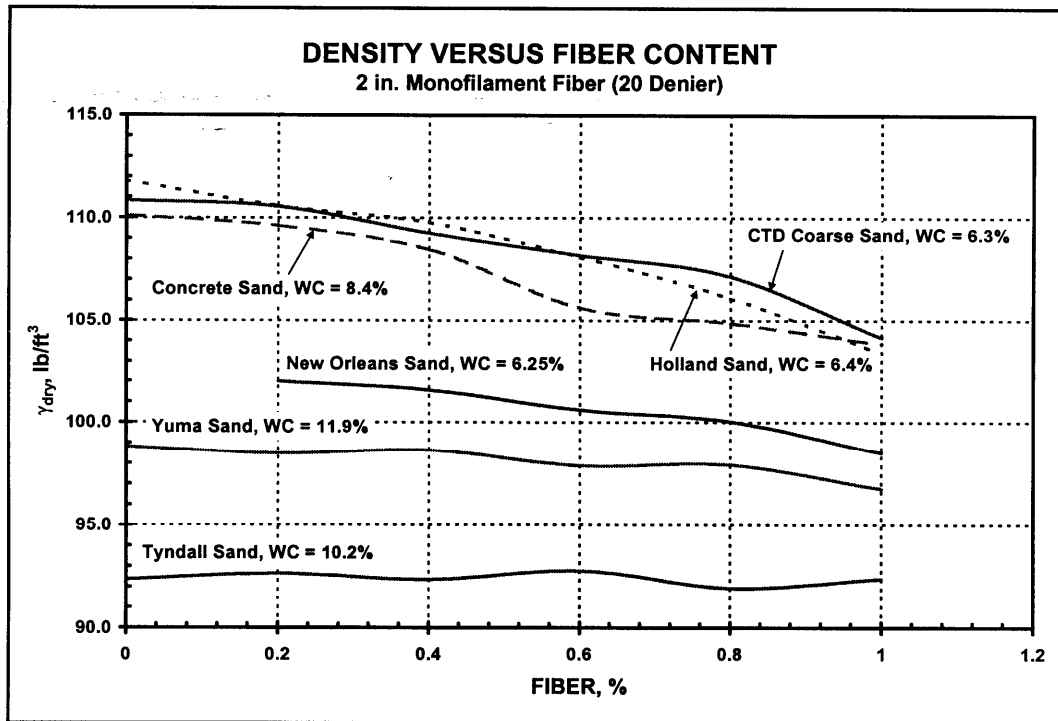
Figure 25. Typical decrease in sample density in different sands with increasing fiber content
