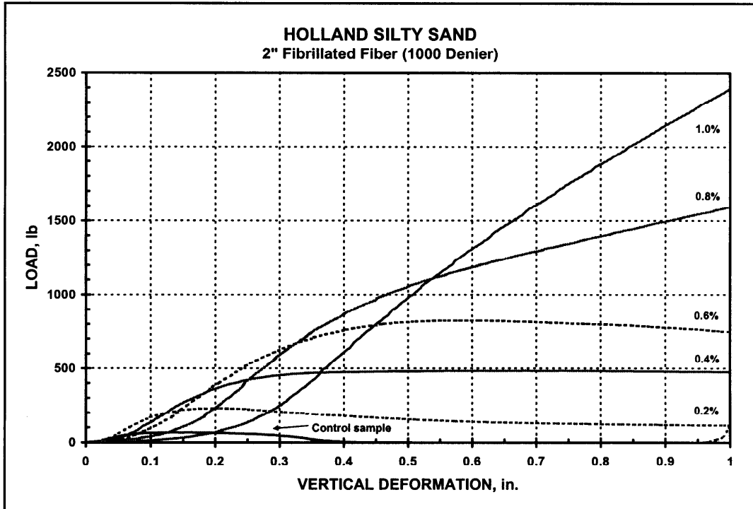
Figure 16. Performance of 2-in. fibrillated (1,000 denier) fibers in Holland LZ sand
