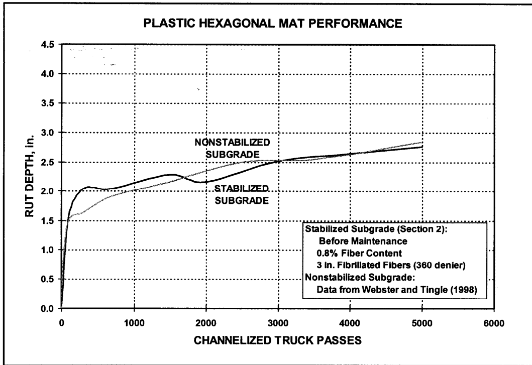
Figure 38. Plastic hexagonal mat performance over stabilized and nonstabilized concrete sand subgrades
