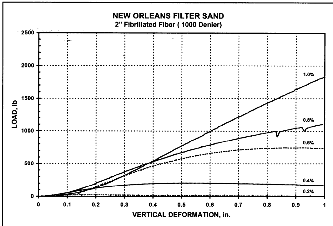
Figure 15. Performance of 2-in. fibrillated (1,000 denier) fibers in New Orleans filter sand
