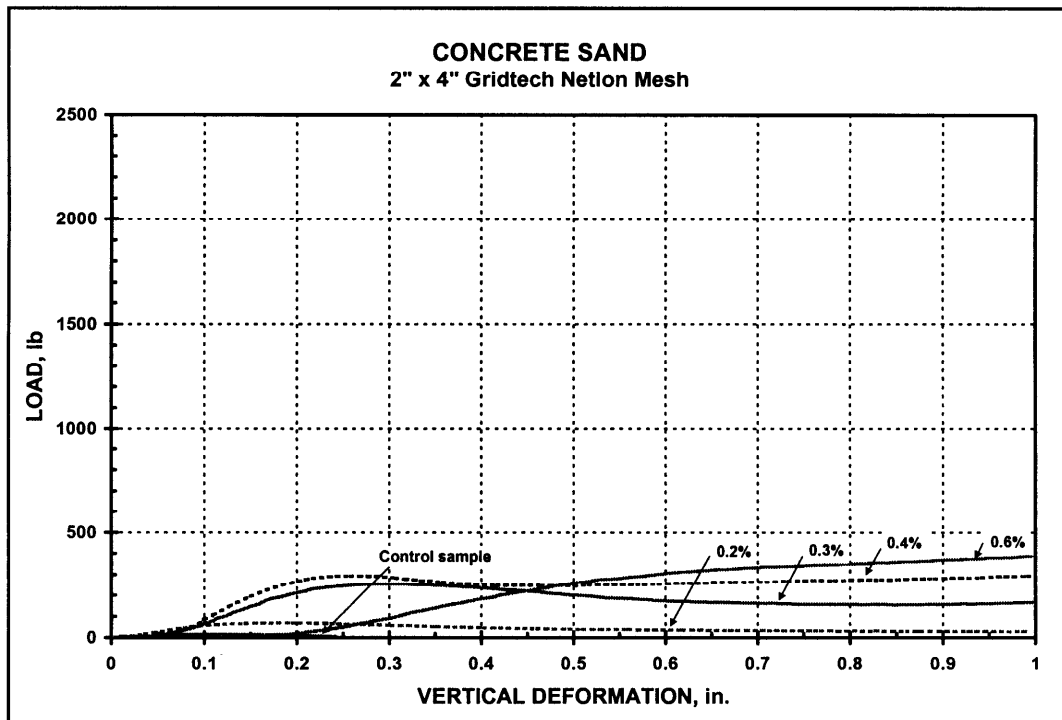
Figure 22. Performance of Netlon mesh fiber elements in concrete sand
