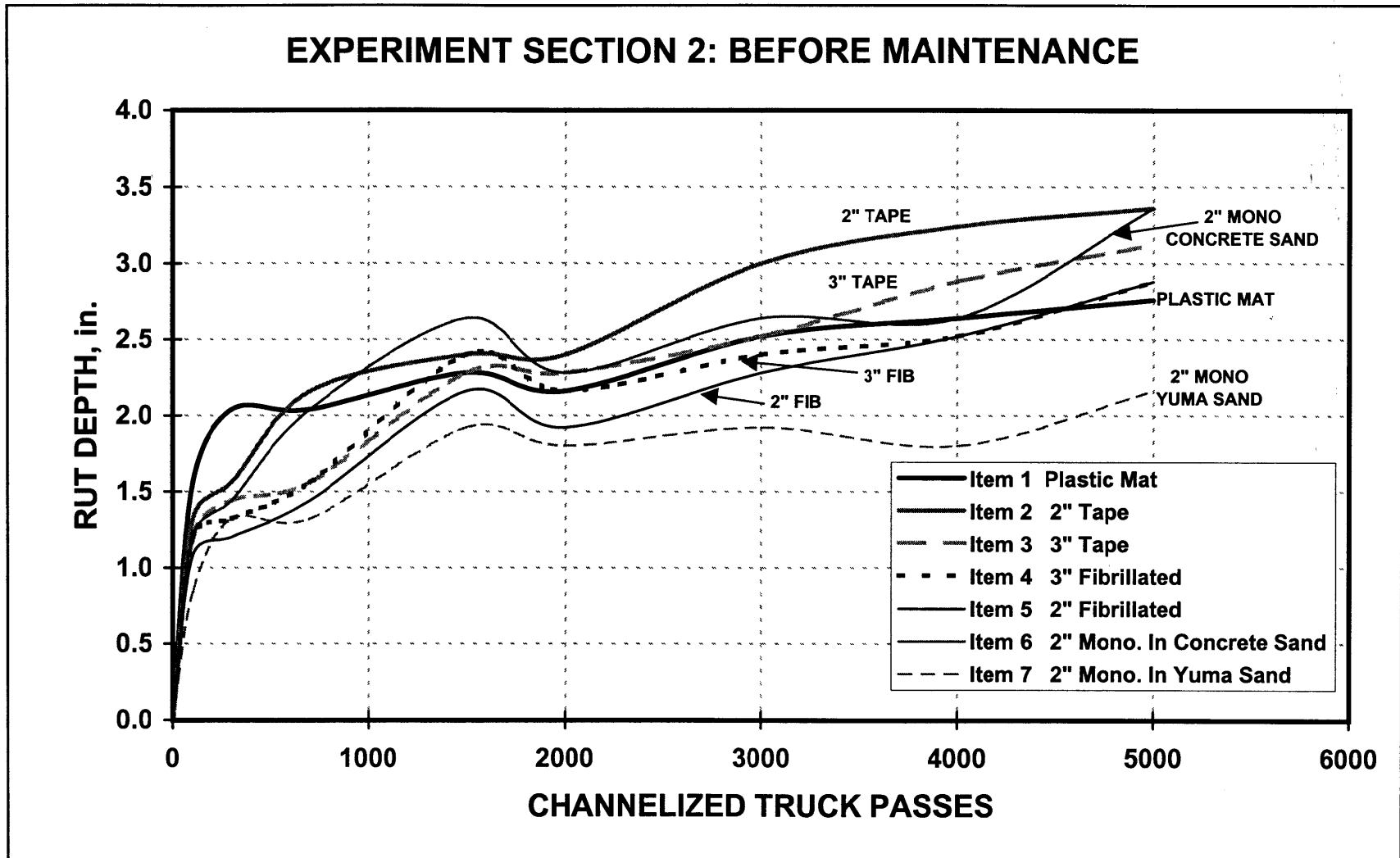
Figure 35. Rut depth measurements for all items of experiment section two before maintenance
