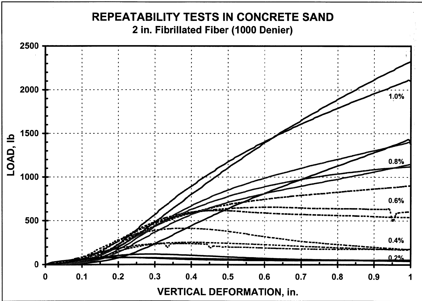
Figure 29. Repeatability tests for 2-in. fibrillated (1,000 denier) fibers in concrete sand
