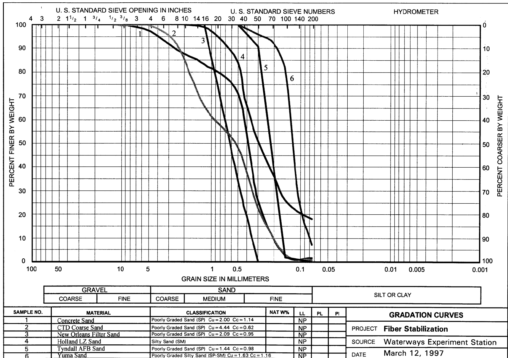
Figure 1. Gradation curves for tested sands
