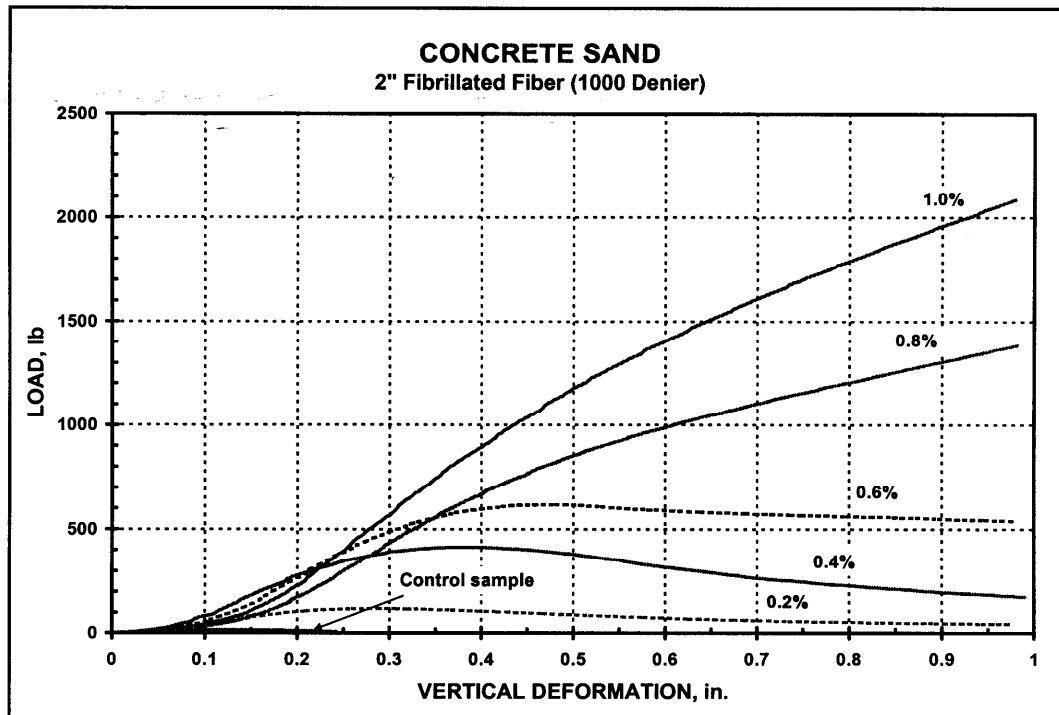
Figure 13. Performance of 2-in. fibrillated (1,000 denier) fibers in concrete sand
