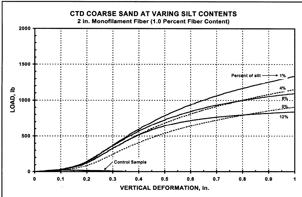
Figure 26. Effect of silt content on specimen performance
