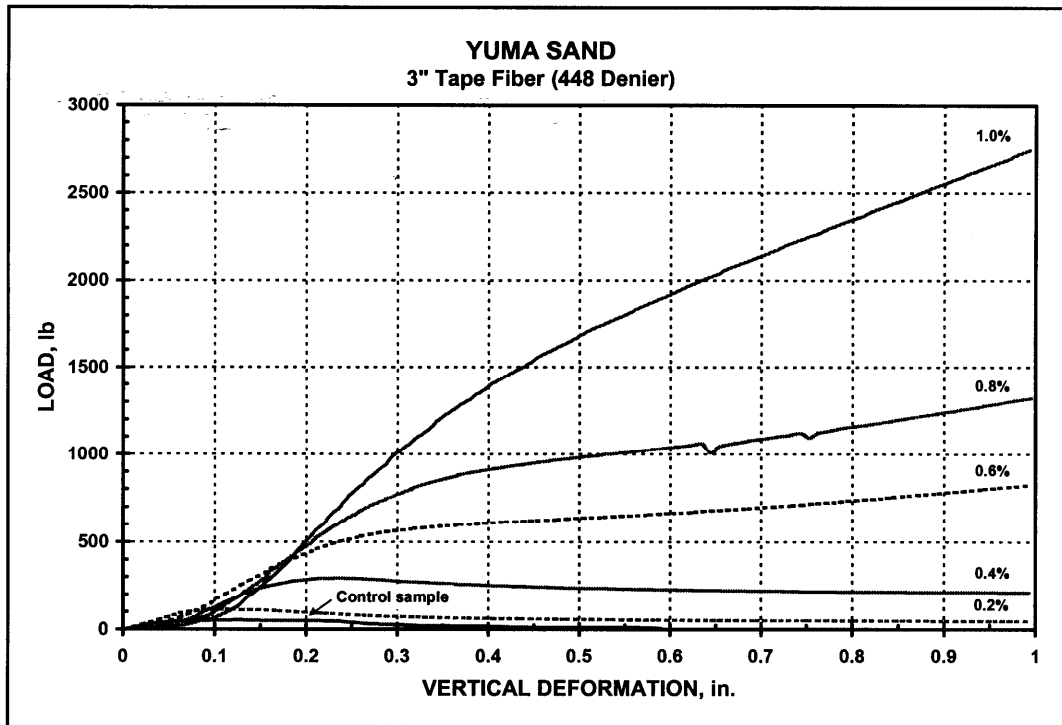
Figure 21. Performance of 3-in. tape (448 denier) fibers in Yuma sand
