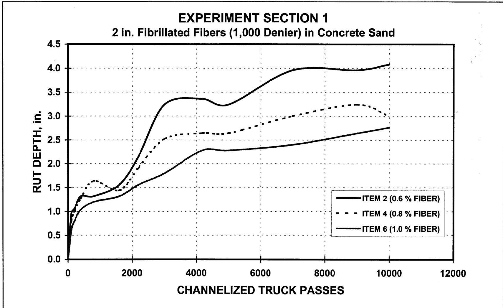
Figure 34. Rut depth measurements for the fibrillated fiber items 2, 4, and 6 of experiment section one
