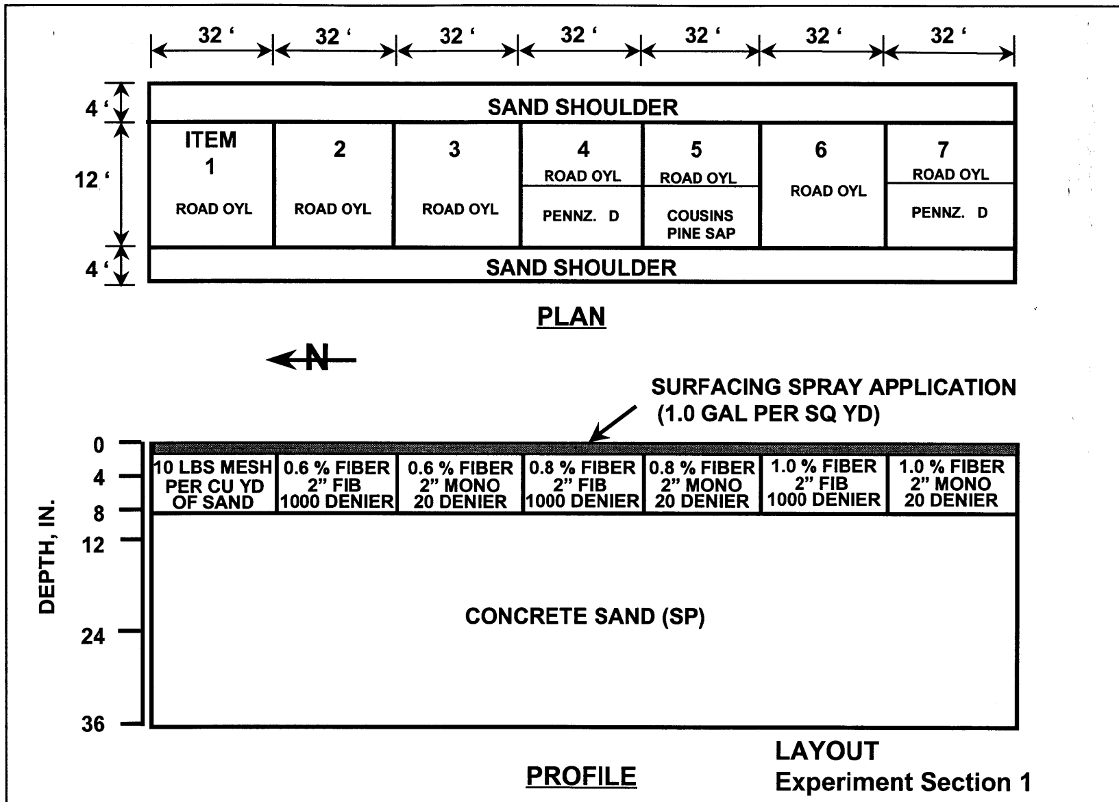
Figure 30. Plan and profile of experiment section one
