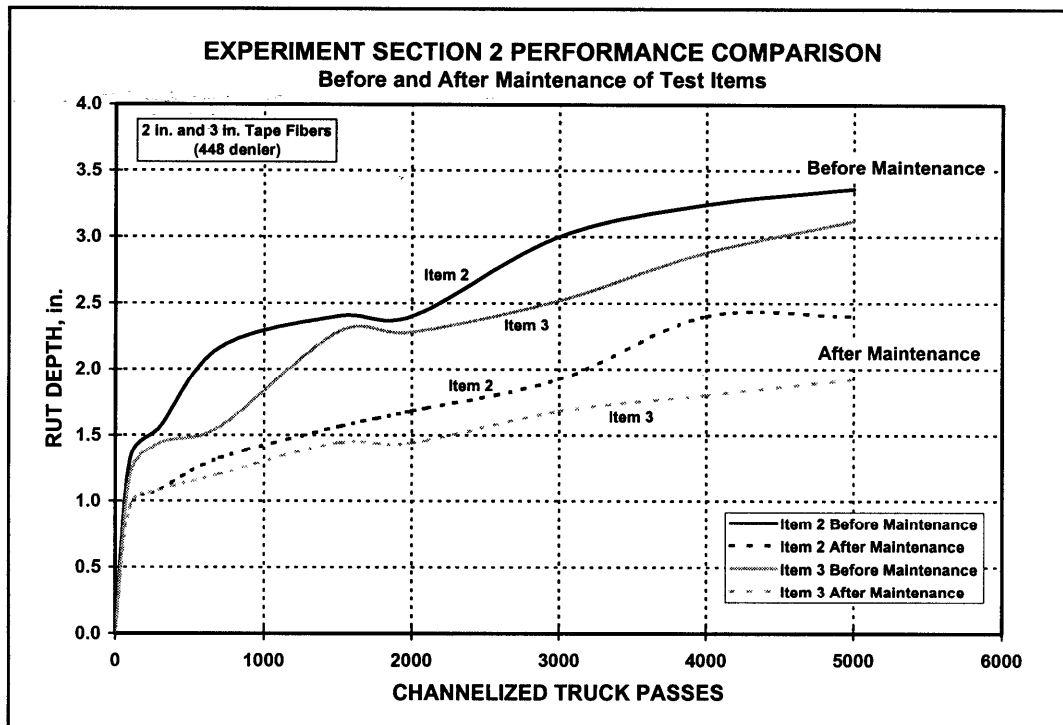
Figure 42. Effect of maintenance on items 2 and 3 of section two
