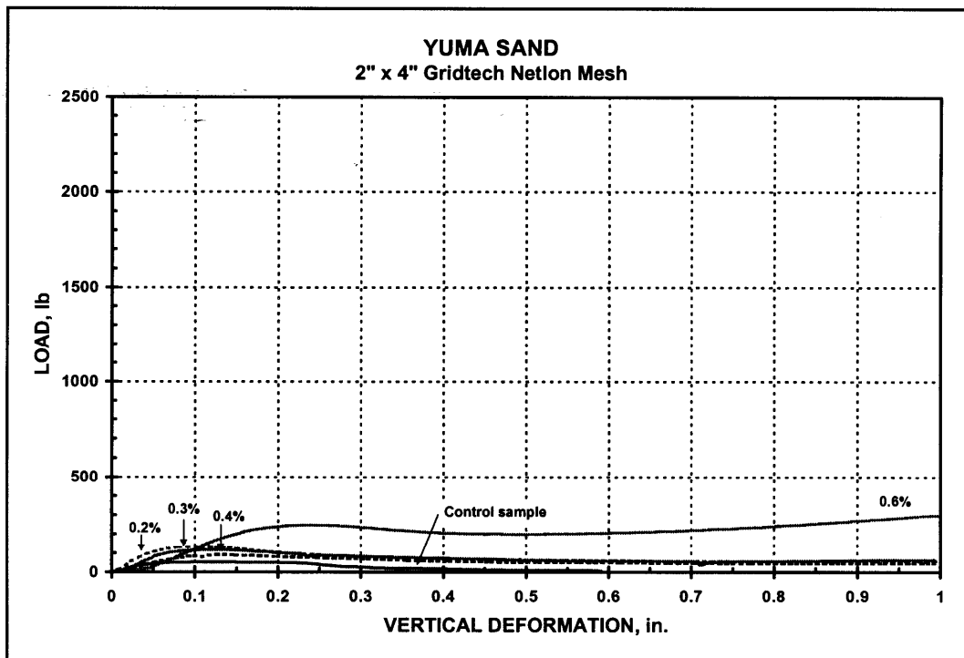
Figure 23. Performance of Netlon mesh fiber elements in Yuma sand
