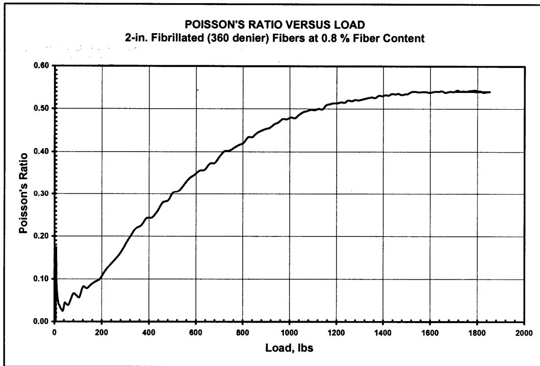
Figure 46. Typical plot of Poisson's ratio versus load for fiber-stabilized sand materials
