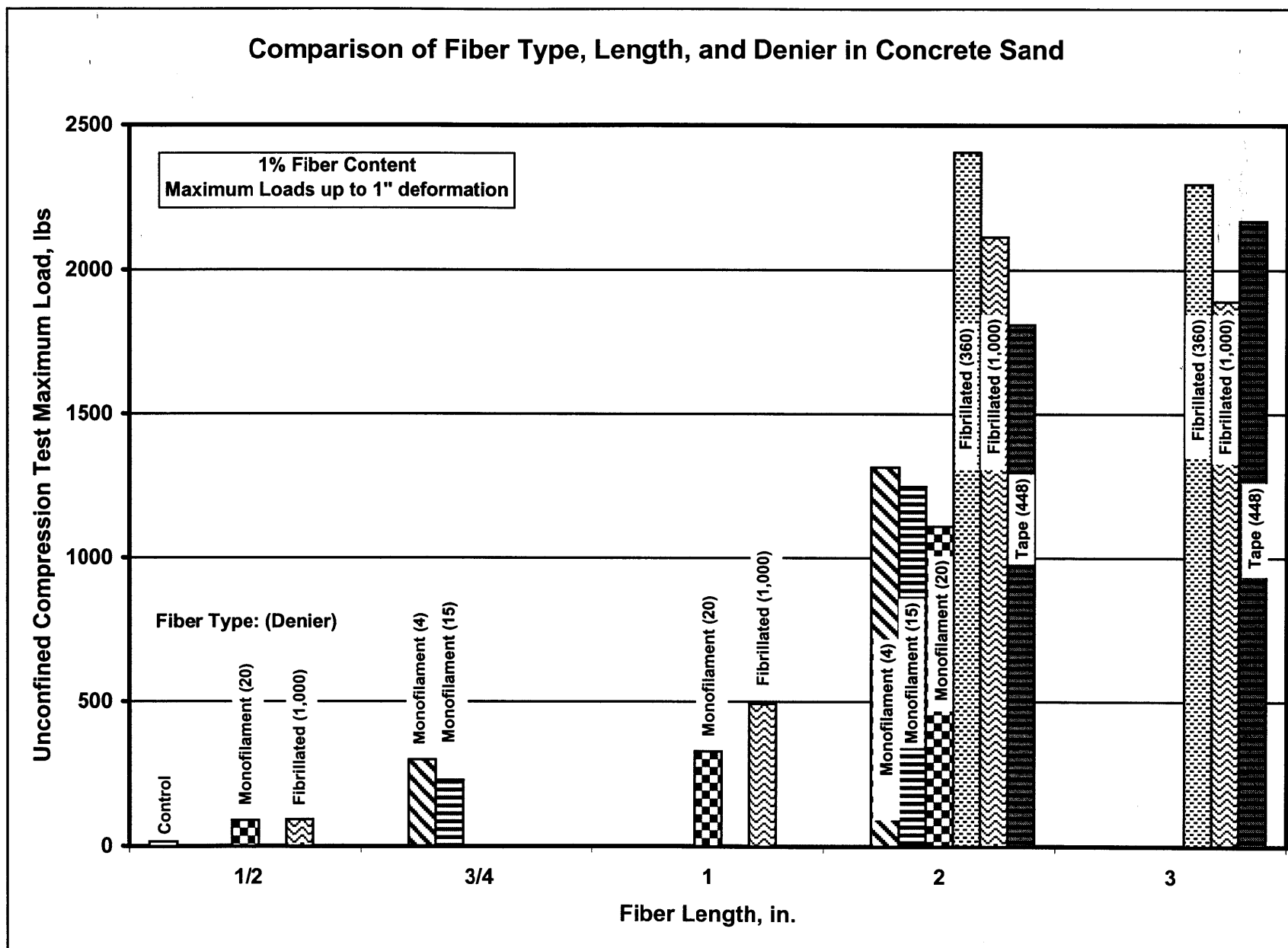
Figure 6. Comparison of fiber type, length, and denier in concrete sand
