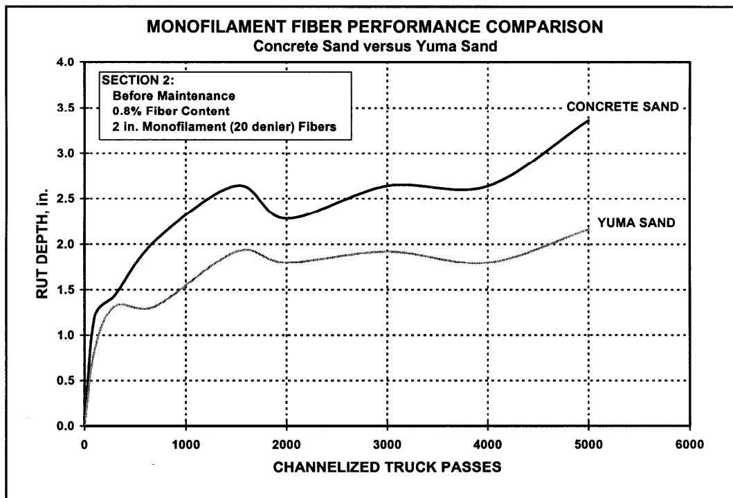
Figure 39. Comparison of concrete sand and Yuma sand items
