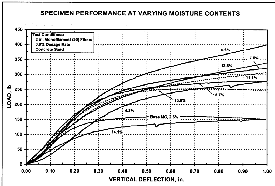
Figure 27. Influence of moisture content on specimen performance
