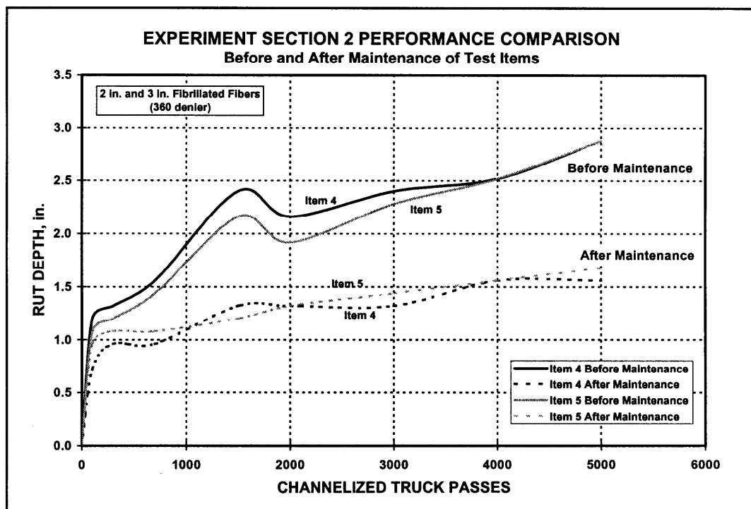
Figure 43. Effect of maintenance on items 4 and 5 of section two
