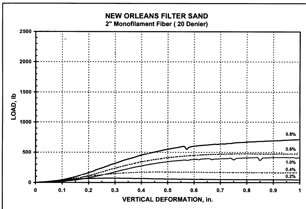
Figure 9. Performance of 2-in. monofilament (20 denier) fibers in New Orleans filter sand
