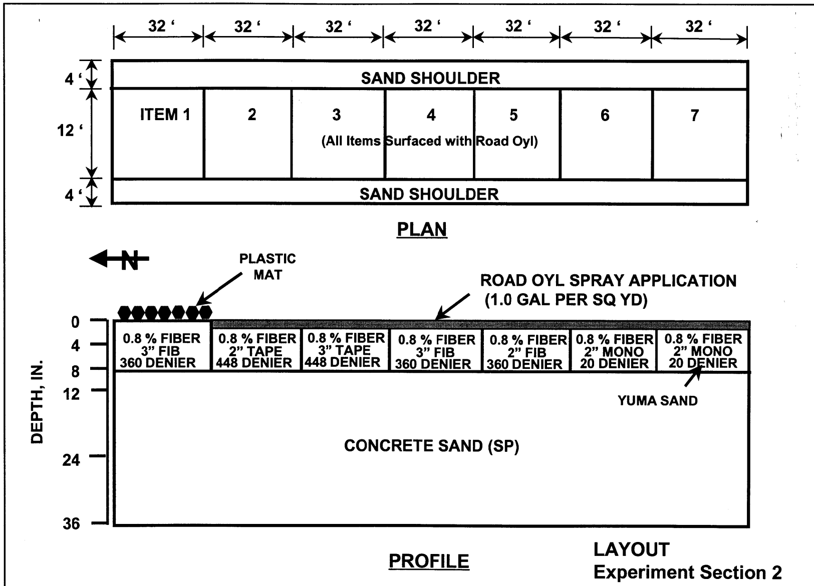
Figure 31. Plan and profile of experiment section two
