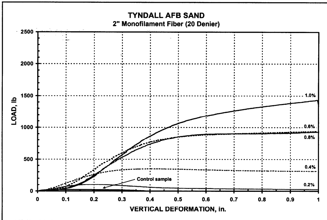
Figure 11. Performance of 2-in. monofilament (20 denier) fibers in Tyndall AFB sand
