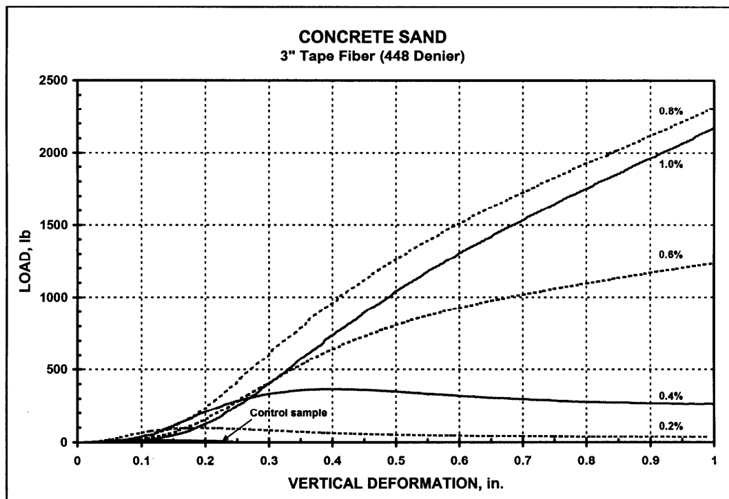
Figure 20. Performance of 3-in. tape (448 denier) fibers in concrete sand
