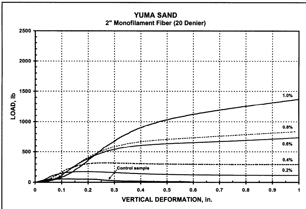
Figure 12. Performance of 2-in. monofilament (20 denier) fibers in Yuma sand
