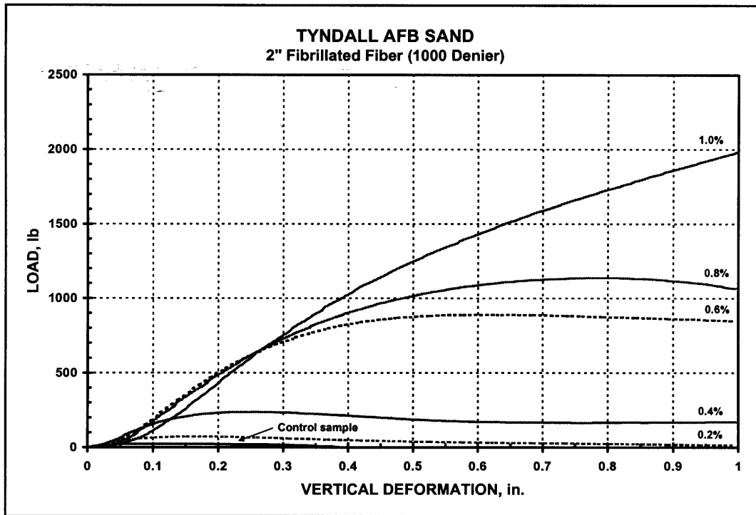
Figure 17. Performance of 2-in. fibrillated (1,000 denier) fibers in Tyndall AFB sand
