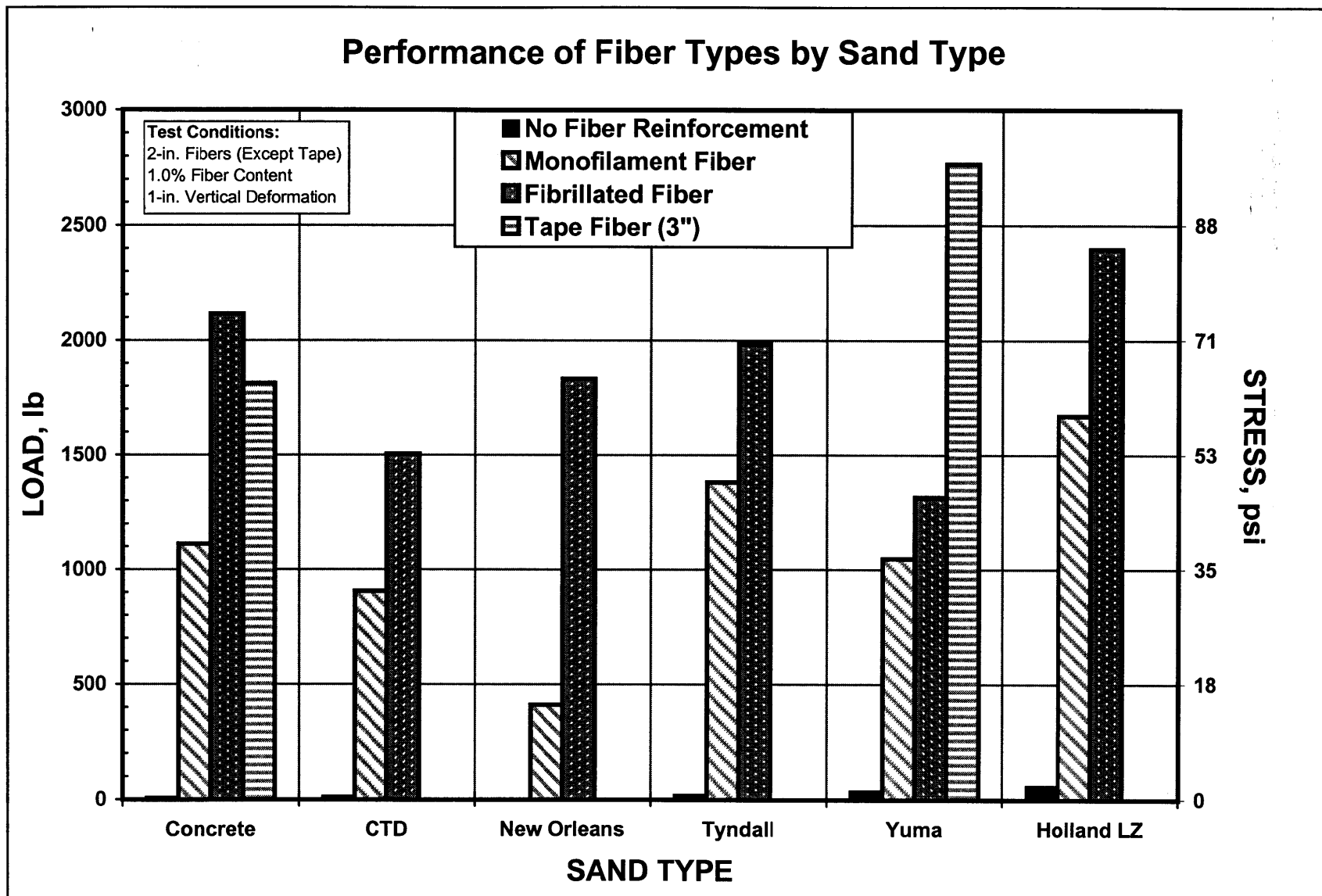
Figure 5. Performance of fiber types in different sands
