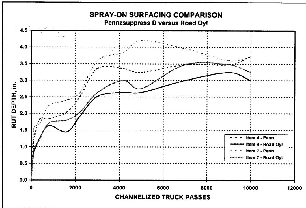
Figure 44. Comparison of spray-on surfacings, Pennzsuppress D versus Road Oyl
