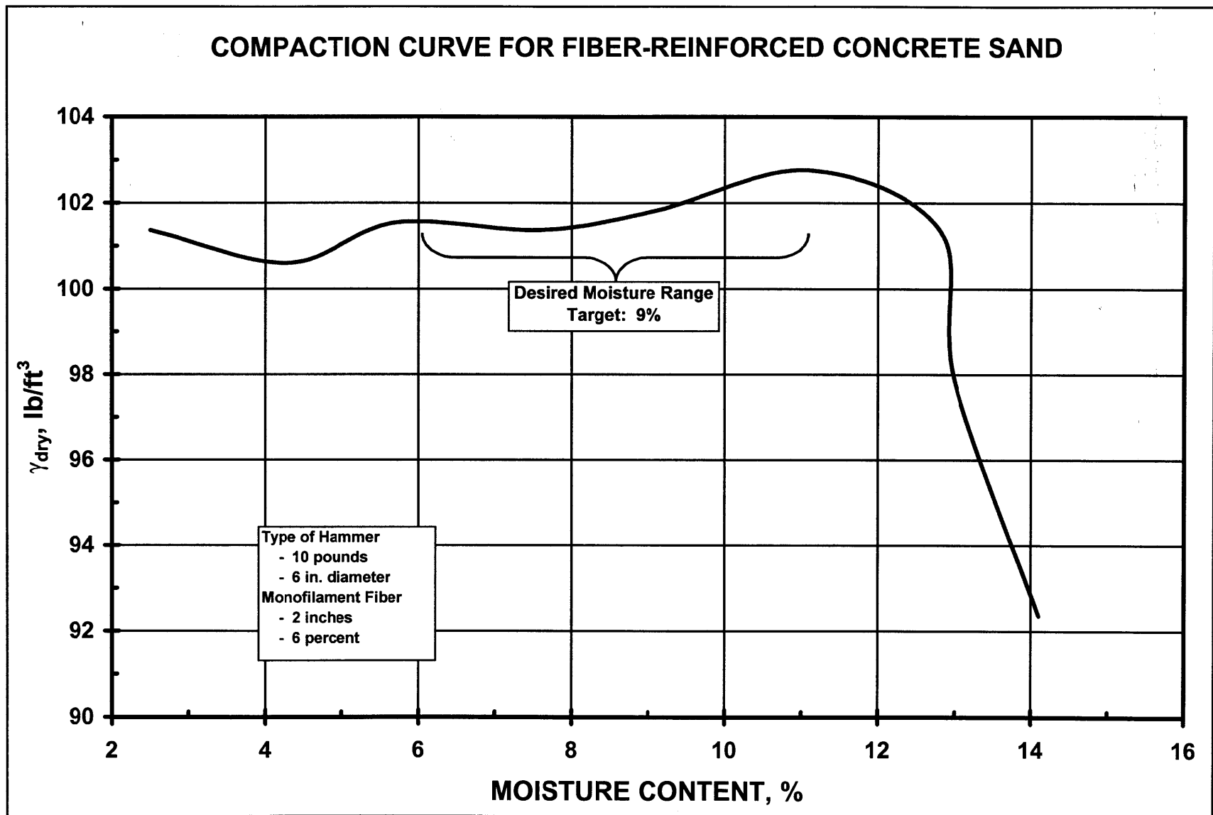
Figure 2. Effect of moisture content on density of concrete sand
