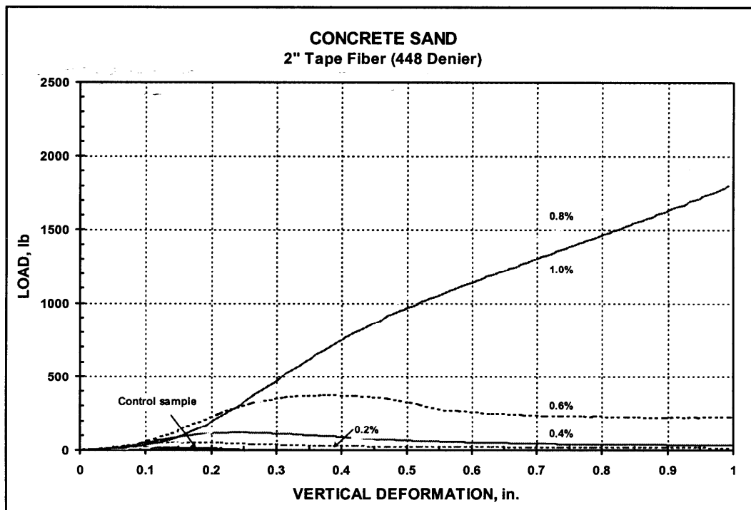
Figure 19. Performance of 2-in. tape (448 denier) fibers in concrete sand
