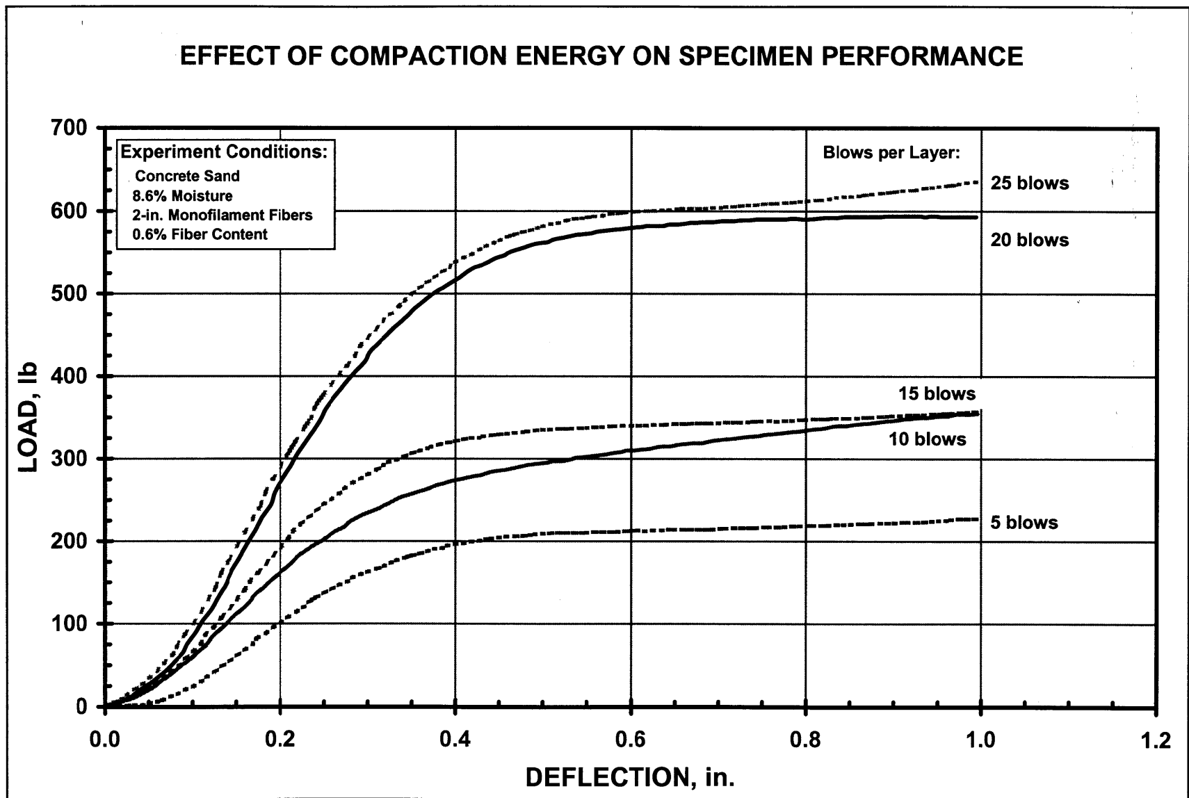
Figure 3. Unconfined compression test results at varying compaction efforts
