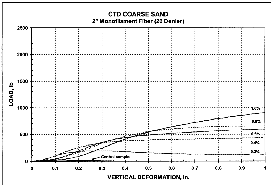
Figure 8. Performance of 2-in. monofilament (20 denier) fibers in CTD coarse sand
