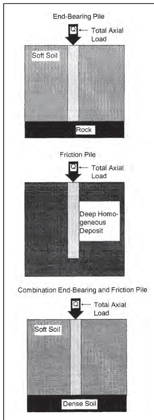
Figure 6-4. Bearing piles
