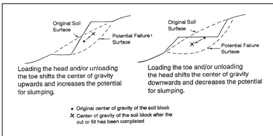
Figure 10-11. Road construction across short slopes
