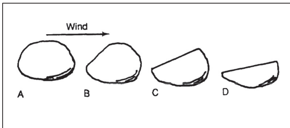
Figure 3-31. Cutting of a ventifact
