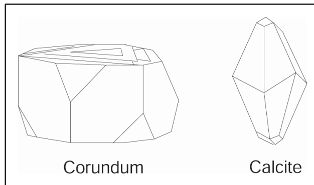
Figure 1-1. Crystal forms
