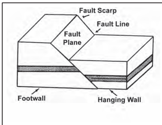
Figure 2-11. Fault terminology
