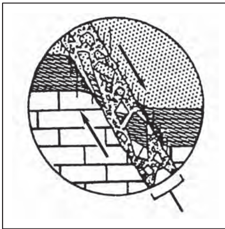
Figure 2-9. Fault zone
