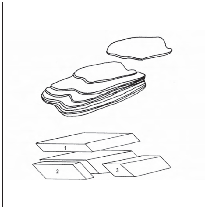
Figure 1-2. Cleavage
