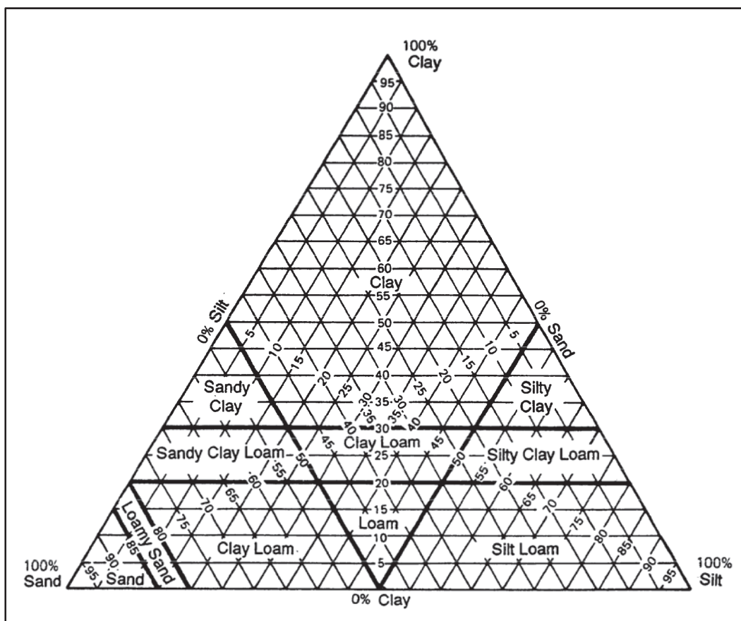
Figure 5-10. US Department of Agriculture textural classification chart
