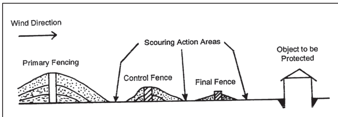
Figure 9-35. Three fences installed to control dune formation
