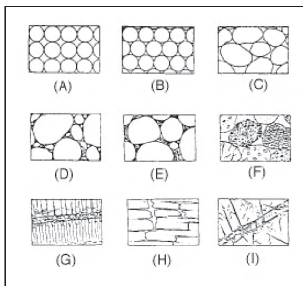
Figure 7-4a. Porosity in rocks
