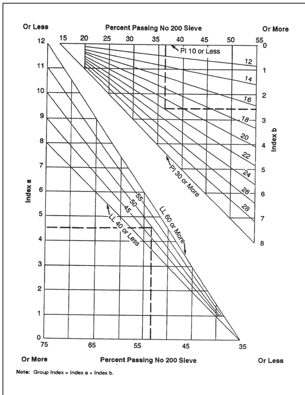
Figure 9-5. Group index for determining average cement requirements
