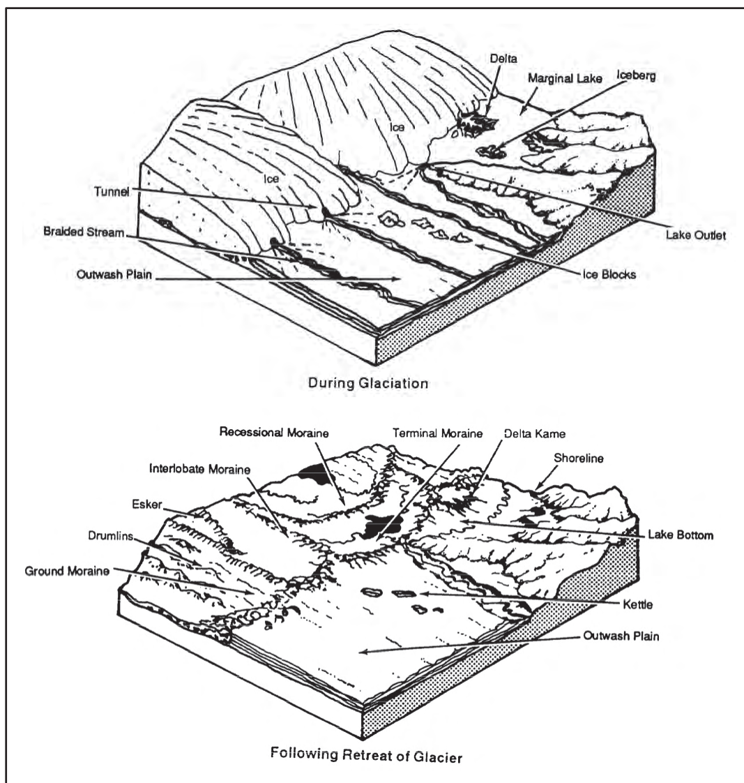
Figure 3-22. Continental glaciation
