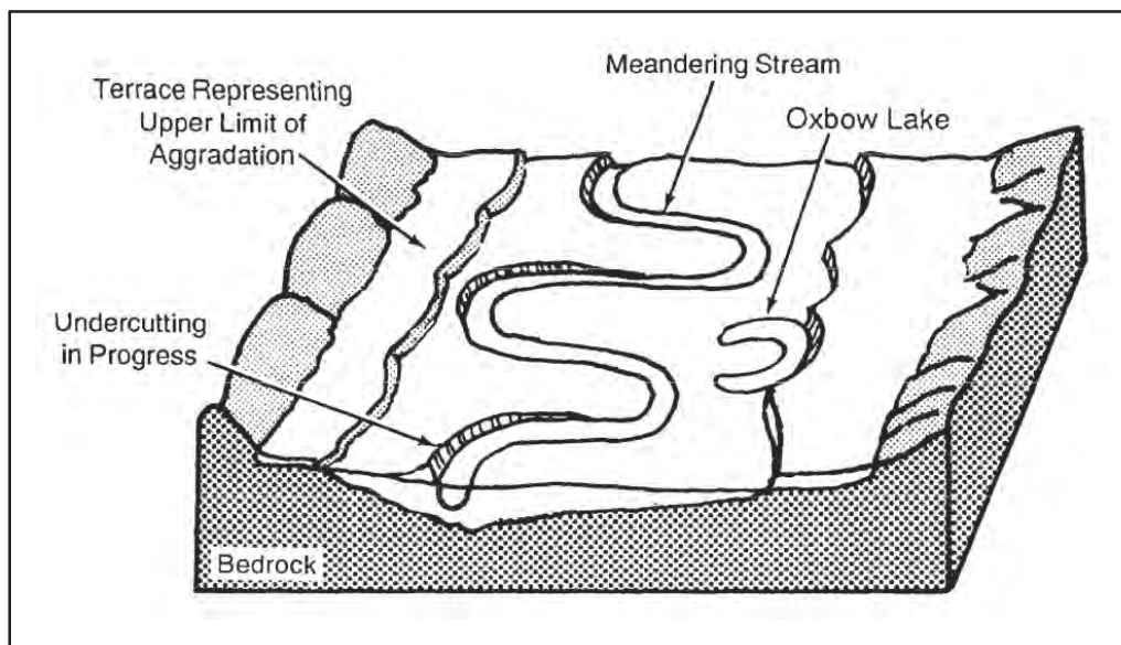
Figure 3-12. Alluvial terraces
