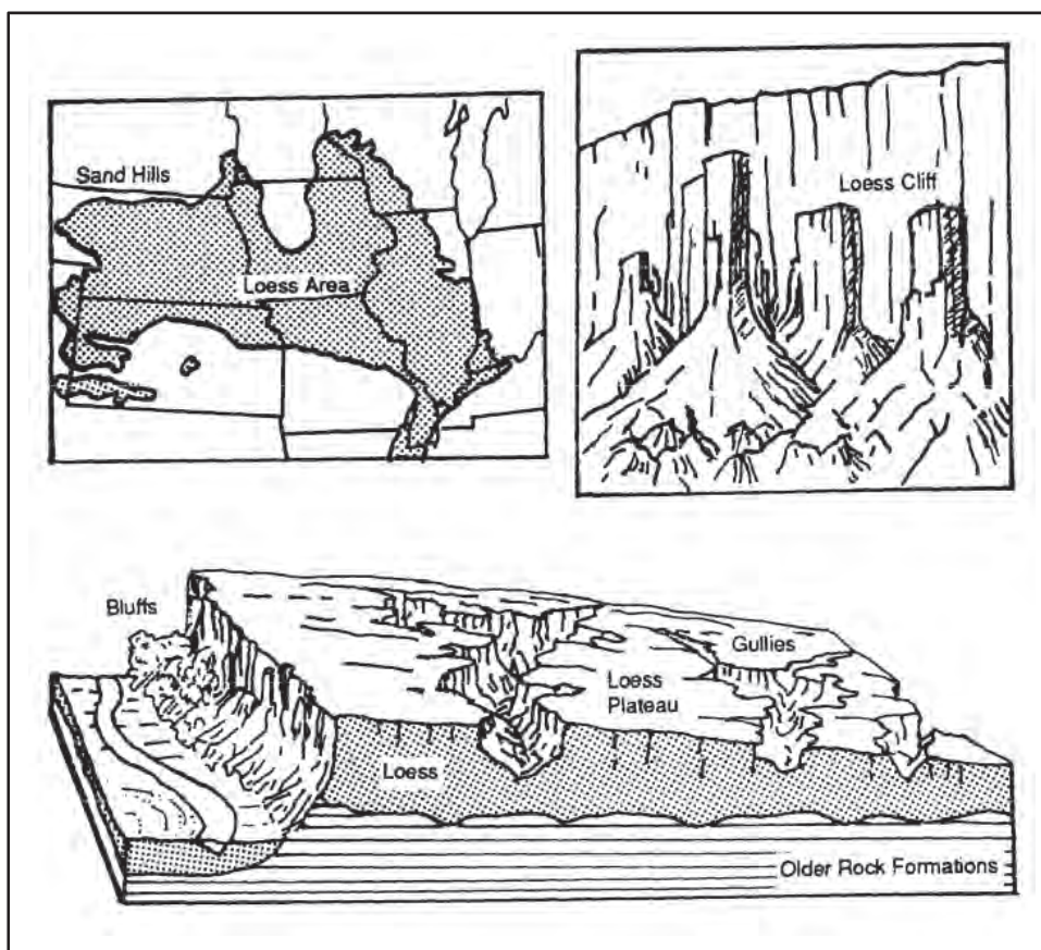
Figure 3-34. Loess landforms
