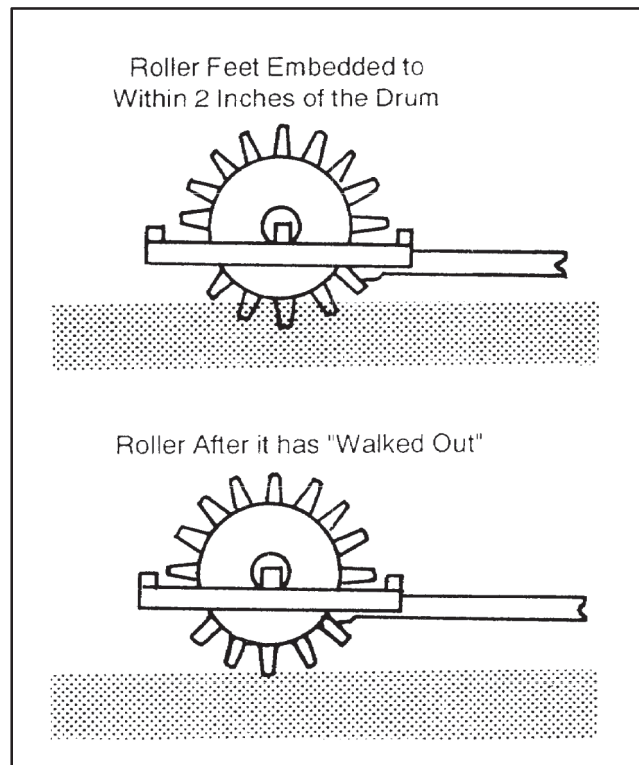
Figure 8-7. Compaction by a sheep's foot roller
