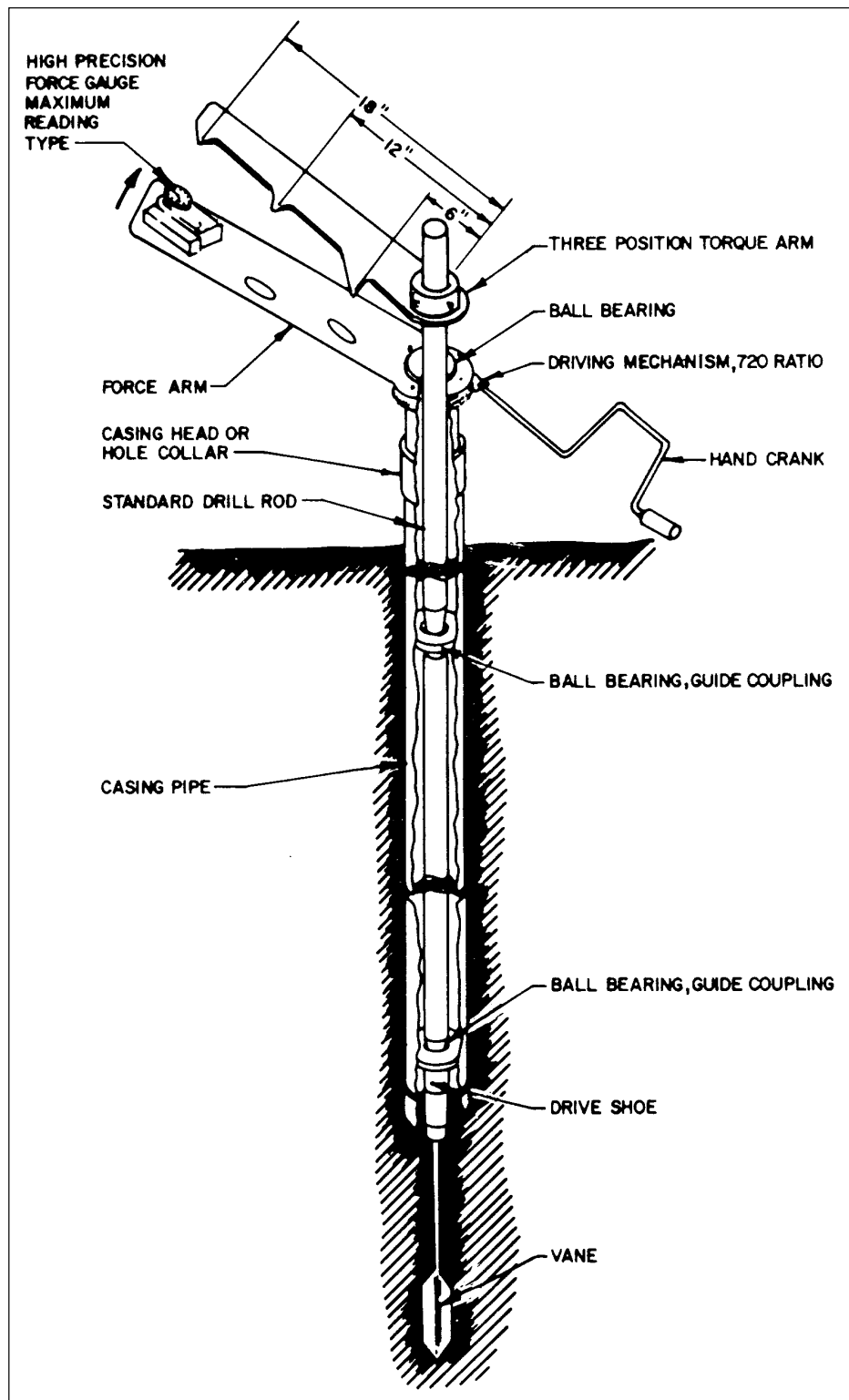
Figure 13, Vane Shear Test Equipment (After NAVFAC, 1986)
