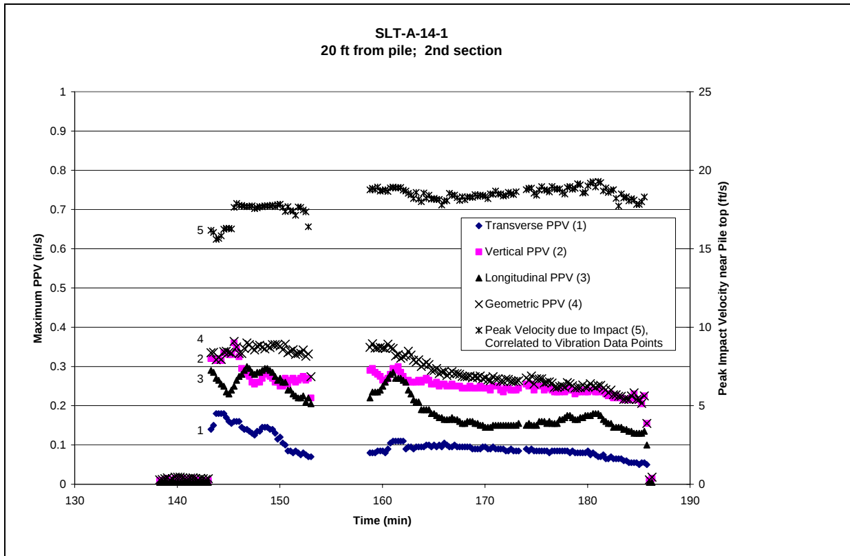
Figure 33. Vibration and velocity near the pile top due to impact (VT1) versus time.
