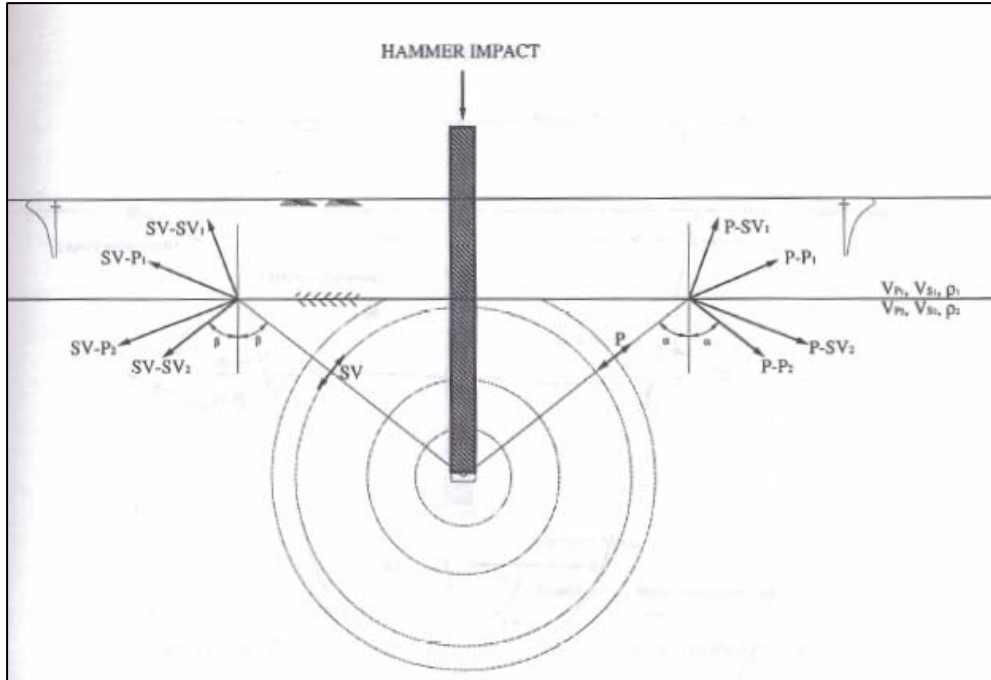
Figure 2. Transmission, Reflection and Refraction of a Compressive (P) and Shear Wave (SV) in a Layered Media (from Woods, 1997).
