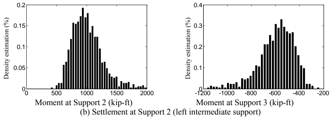
Figure 2.8 Histograms of the maximum positive and negative moments of Bridge A4058 under random support settlements: mean=1 in. and COV=0.25
