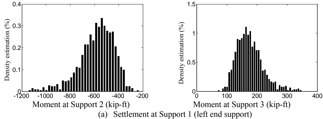
Figure 2.7 Bridge A4058 under a random support settlement: mean=1 in. and COV=0.25
