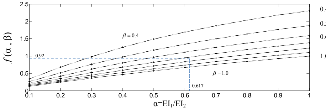
(b) For negative moment at support 3
