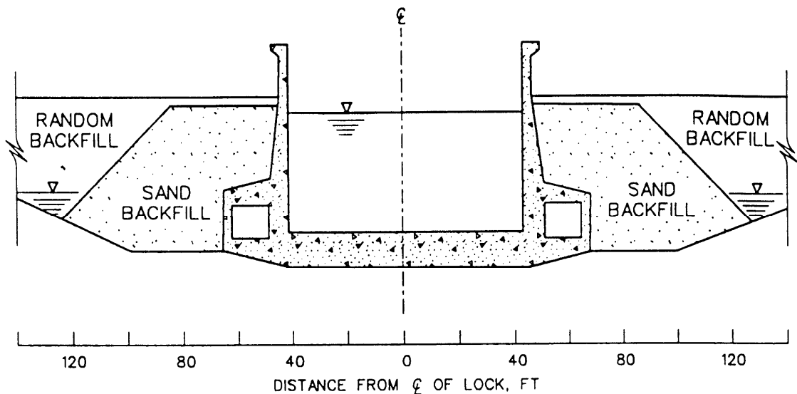
a. Cross section of Port Allen Lock
