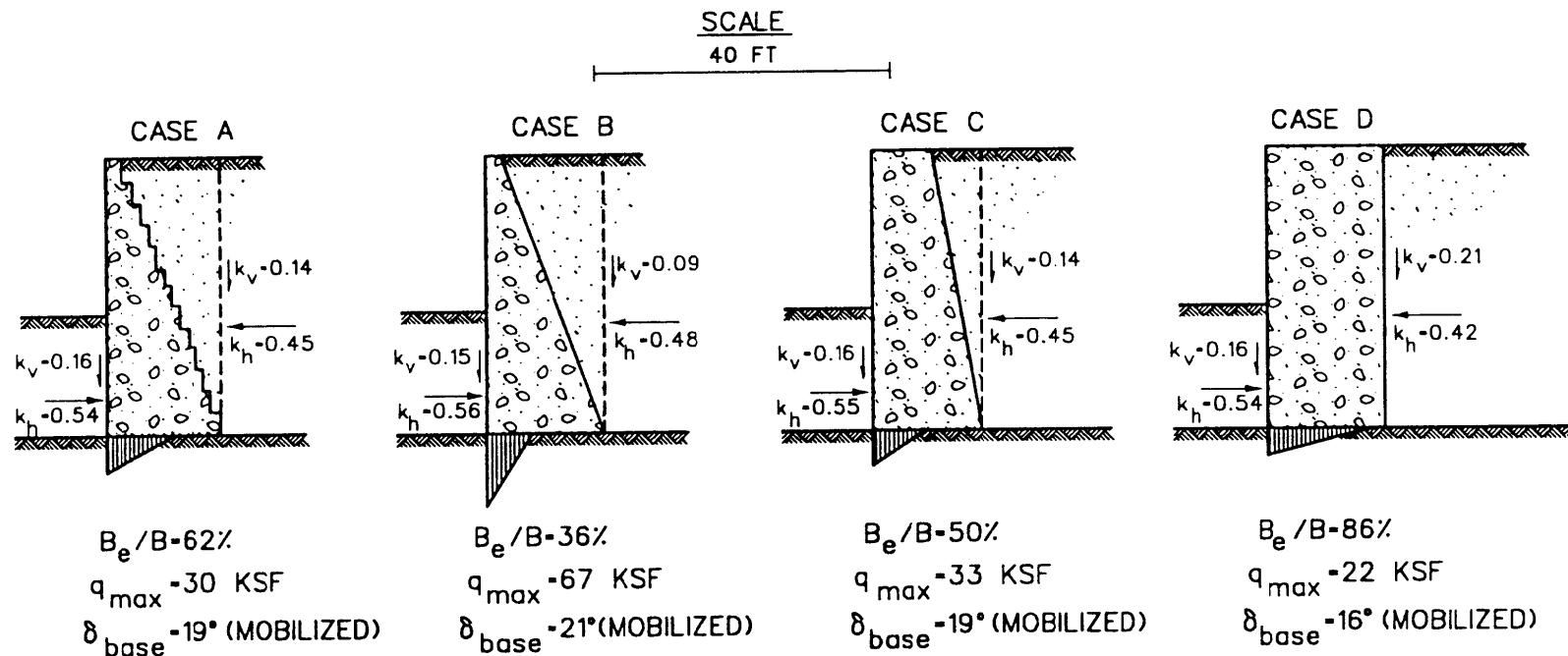
Figure 18. Results of finite element analyses of four retaining walls on rock (Ebeling, Duncan, and Clough 1989)
