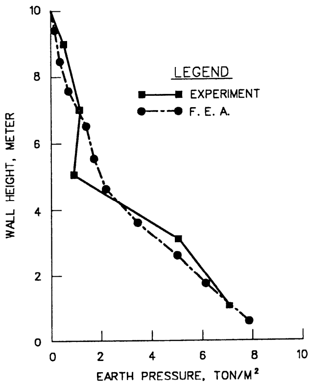
Figure 9. Earth pressure distribution in study by Bhatia and Bakeer (1989)
