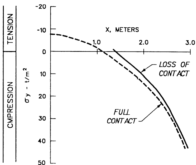
b. Contact stress distribution
