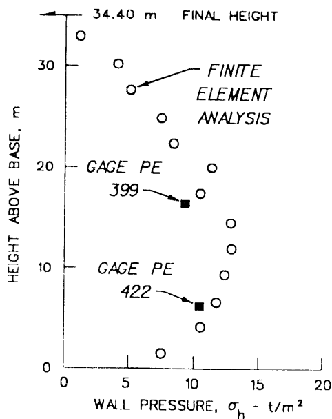
d. Results of nonlinear finite element calculations and gages PE 399 and PE 422 - after backfilling
