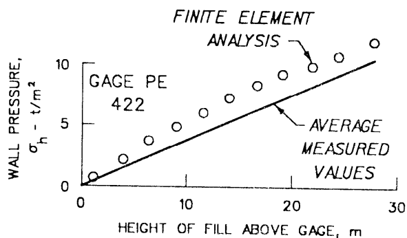
c. Results of nonlinear finite element calculations and gage PE 422 - during backfilling
