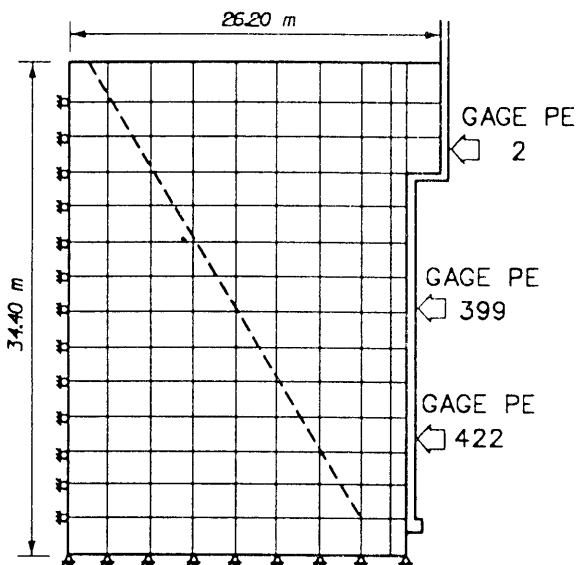
a. Cross section with finite element mesh and earth pressure cells
