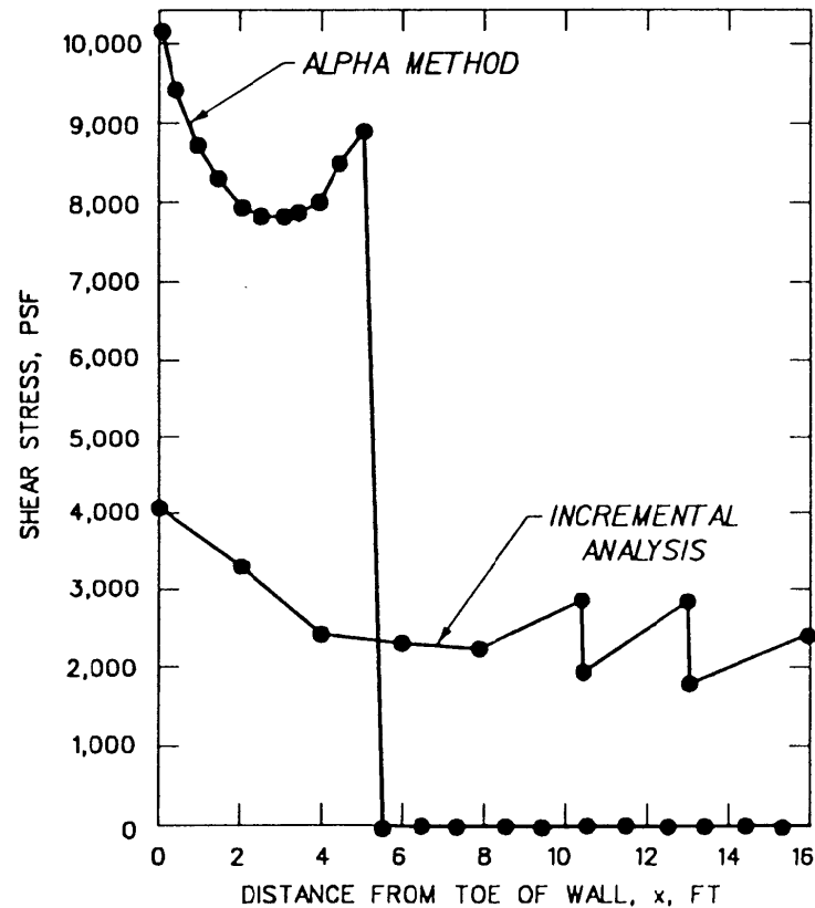
Figure 22. Stress distributions along the base for 0.5 \sigma_v load (Ebeling et al. 1988)
