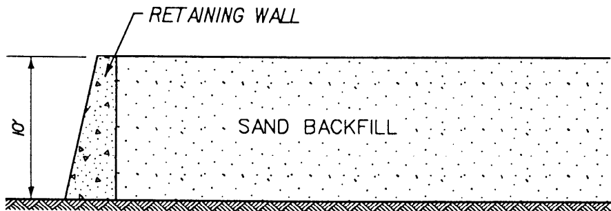
b. Retaining wall—finite element representation
