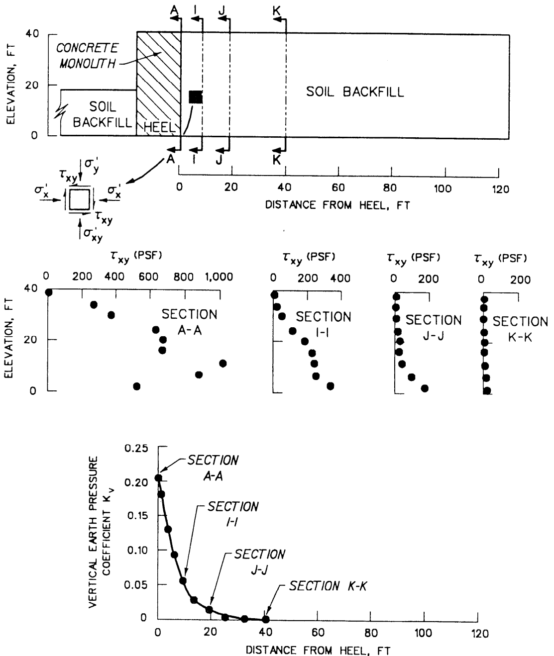
Figure 17. Variation of distribution of shear stress and vertical earth pressure coefficient with distance from the heel of the wall (Ebeling, Duncan, and Clough 1989)
