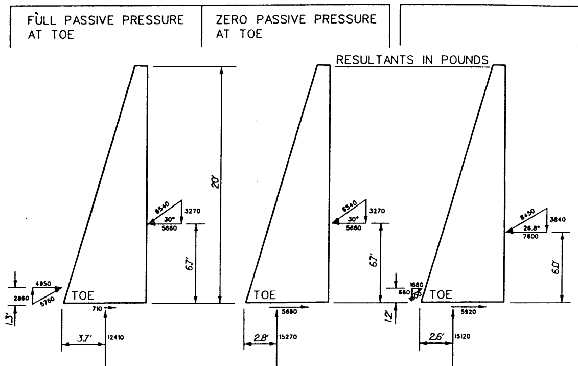
Figure 12. Earth pressure resultants acting on wall from classical earth pressure theory and finite element results (Clough and Duncan 1971)
