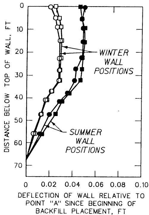
Figure 4. Temperature-induced wall movements and changes in earth pressure at Port Allen Lock (Clough and Duncan 1969)
