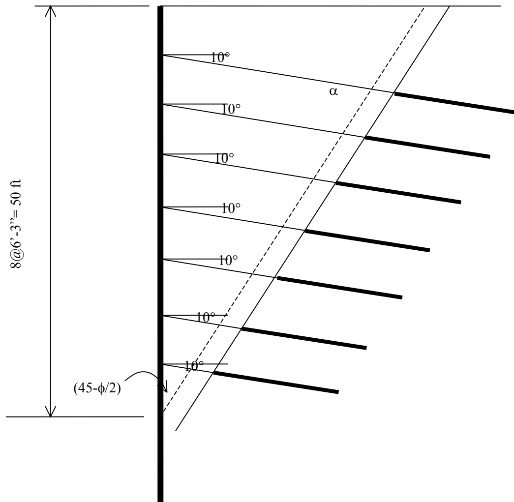
Figure 4.4. Seven-tier anchor
