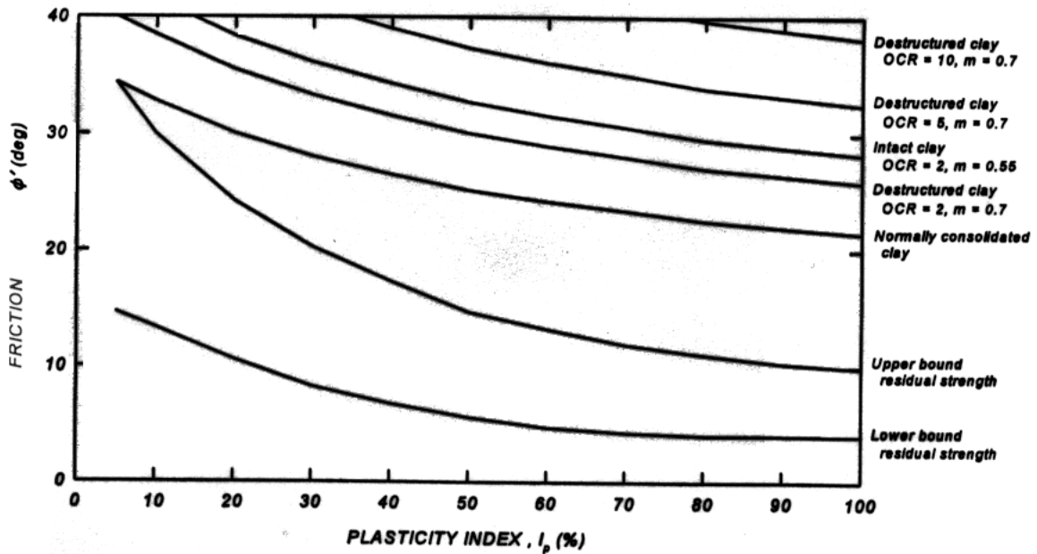
Figure A.4. Friction angle \phi' for clays in different states as a function of plasticity index (after Figure 37, FHWA-RD-97-130)
