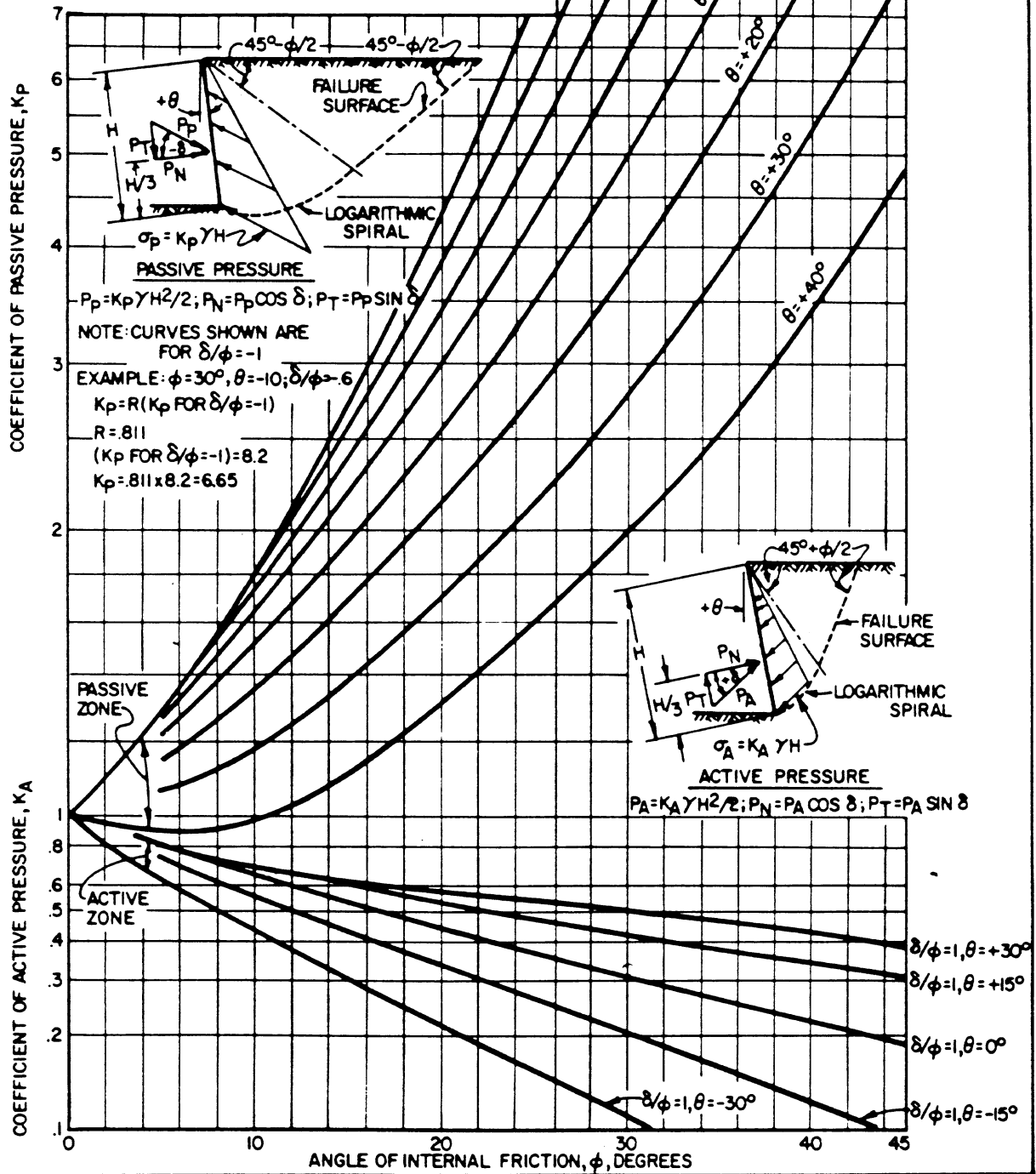
Figure 16. Active and passive earth pressure coefficients (effect of wall inclination).
