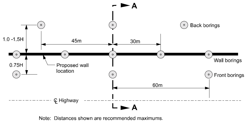
Typical plan
