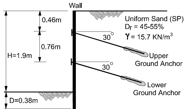
Figure 18. Cross section of model wall (modified after FHWA-RD-98-067, 1998).
