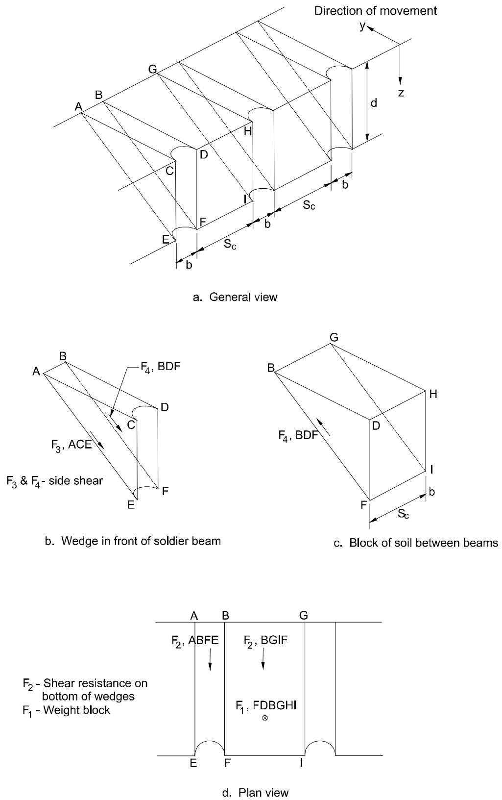
Figure B-5. Failure wedges for soldier beams in clay (after Wang and Reese, 1986).
