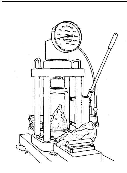
Figure 4-6. Compression tester
