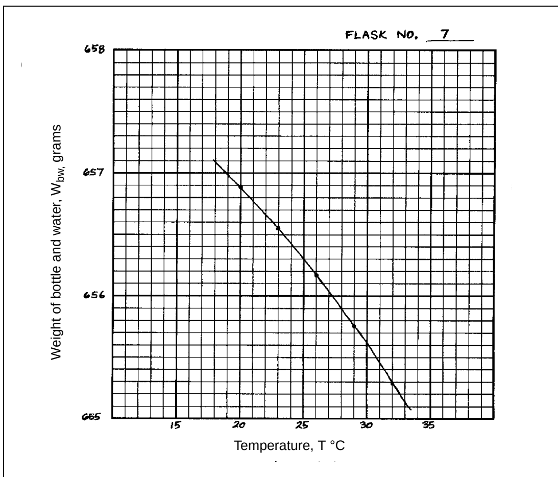
Figure 2-37. Calibration curve for a volumetric flask
