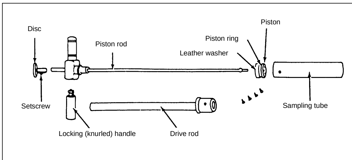
Figure 2-19. Soil-trafficability sampler
