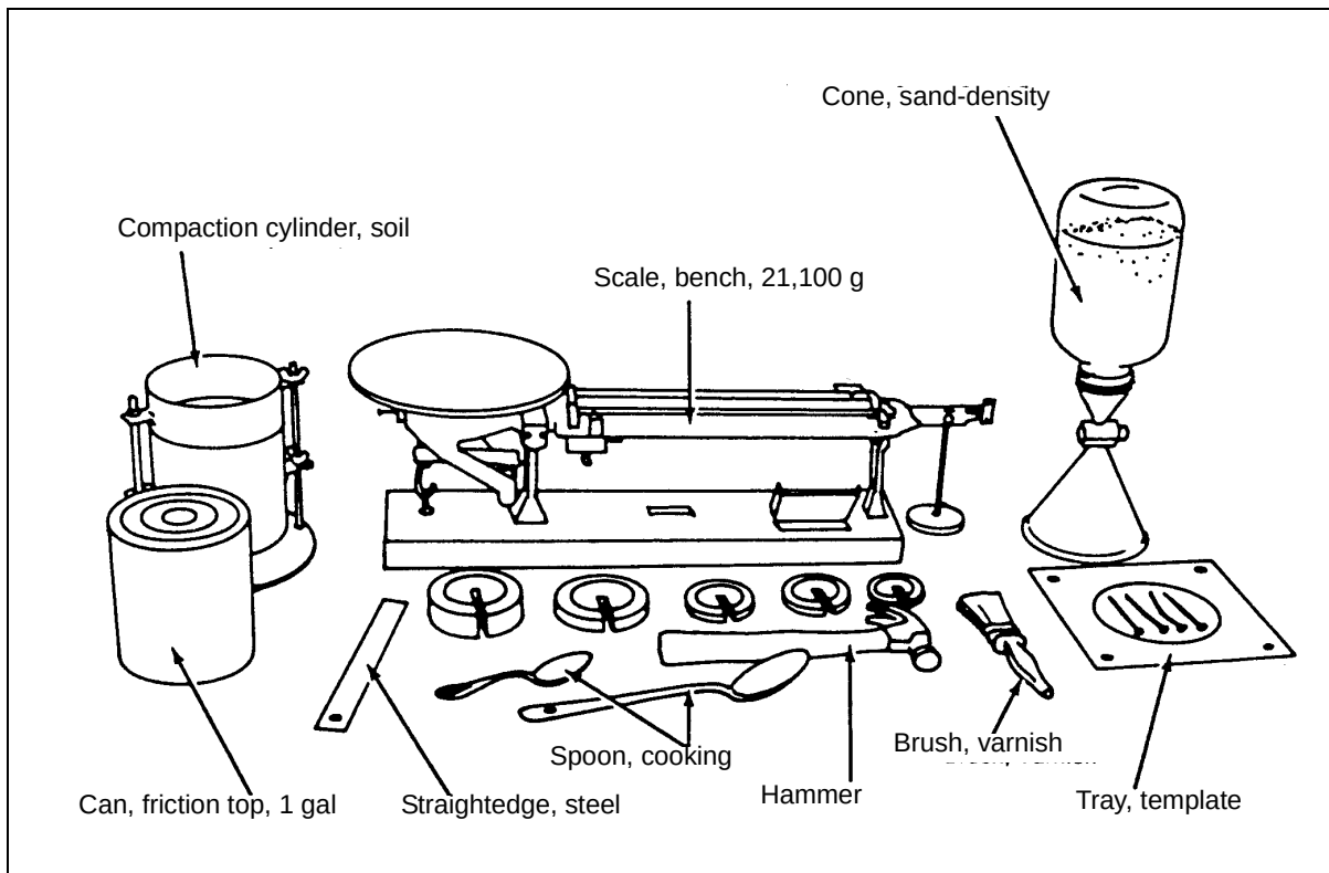
Figure 2-62. Sand-displacement-method apparatus
