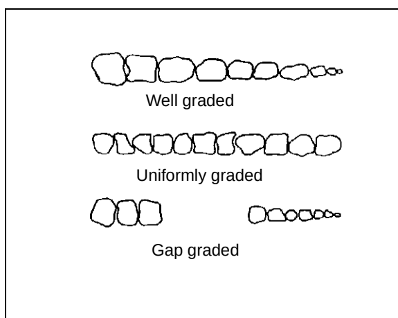
Figure 2-2. Soil gradation
