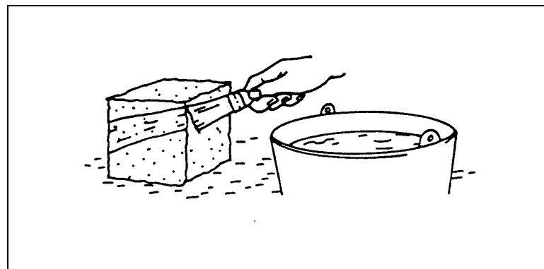
Figure 2-15. Applying paraffin to seal a chunk sample
