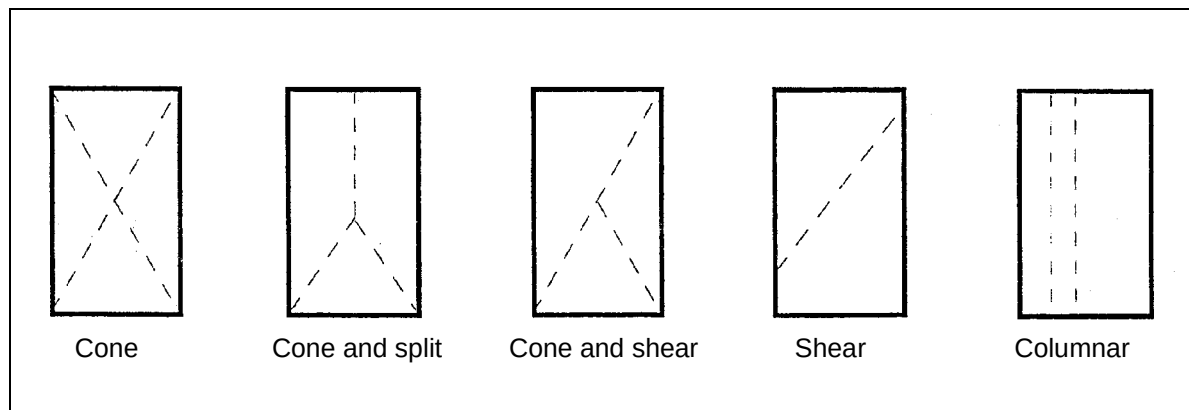
Figure 4-7. Types of fractures
