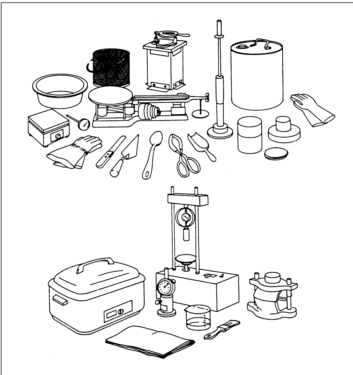
Figure 3-13. Apparatus for bituminous mix design—Marshall method
