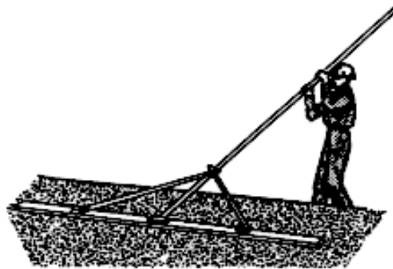
View 3. Long-handled wood float and floating operation
