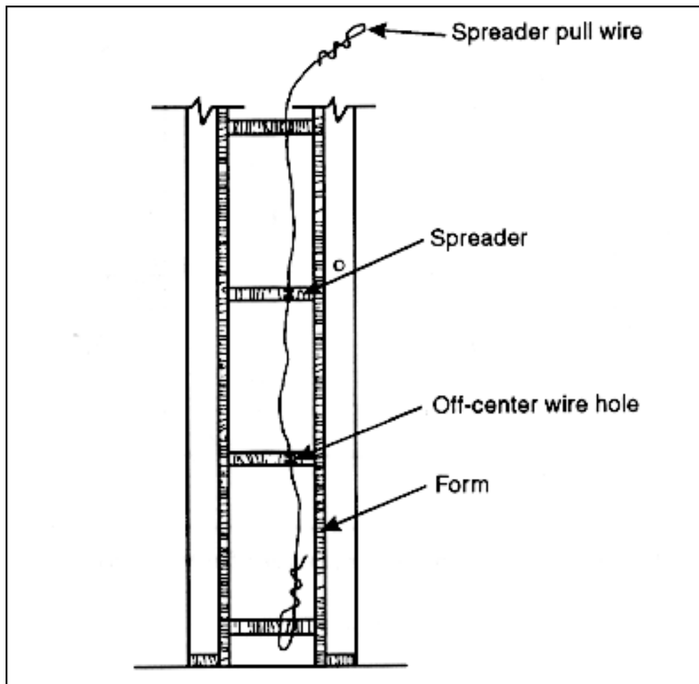
Figure 4-17. Removing wood spreader
