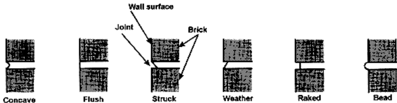
Figure 9-18. Joint finishes
