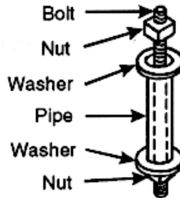
Figure 4-27. Anchor bolt with pipe sleeve
