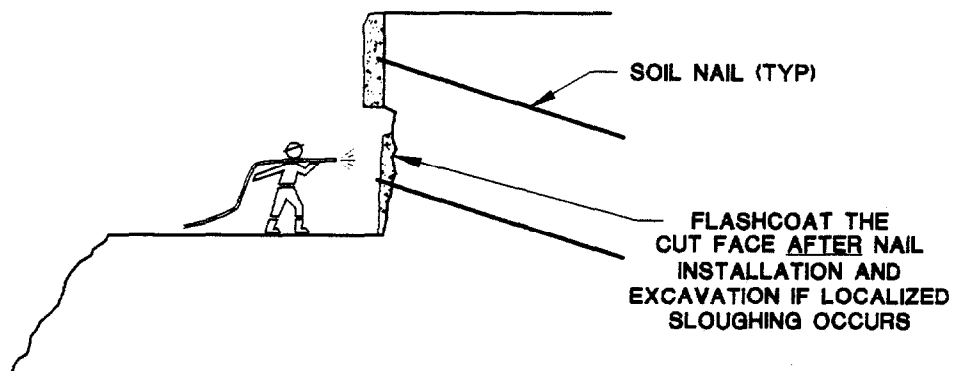
FLASHCOAT SHOTCRETING
