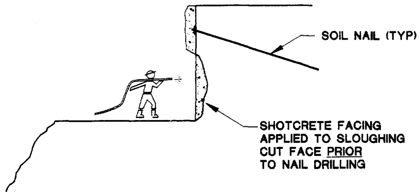
SHOTCRETE FLASHCOAT PRIOR TO DRILLING
