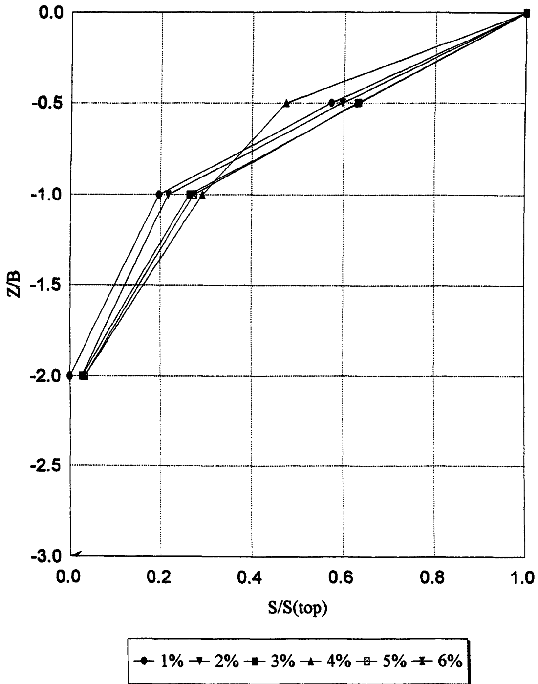
Figure E4: Settlement Versus Depth for 3.0-m(n) Footing With Varying Percentages of B
