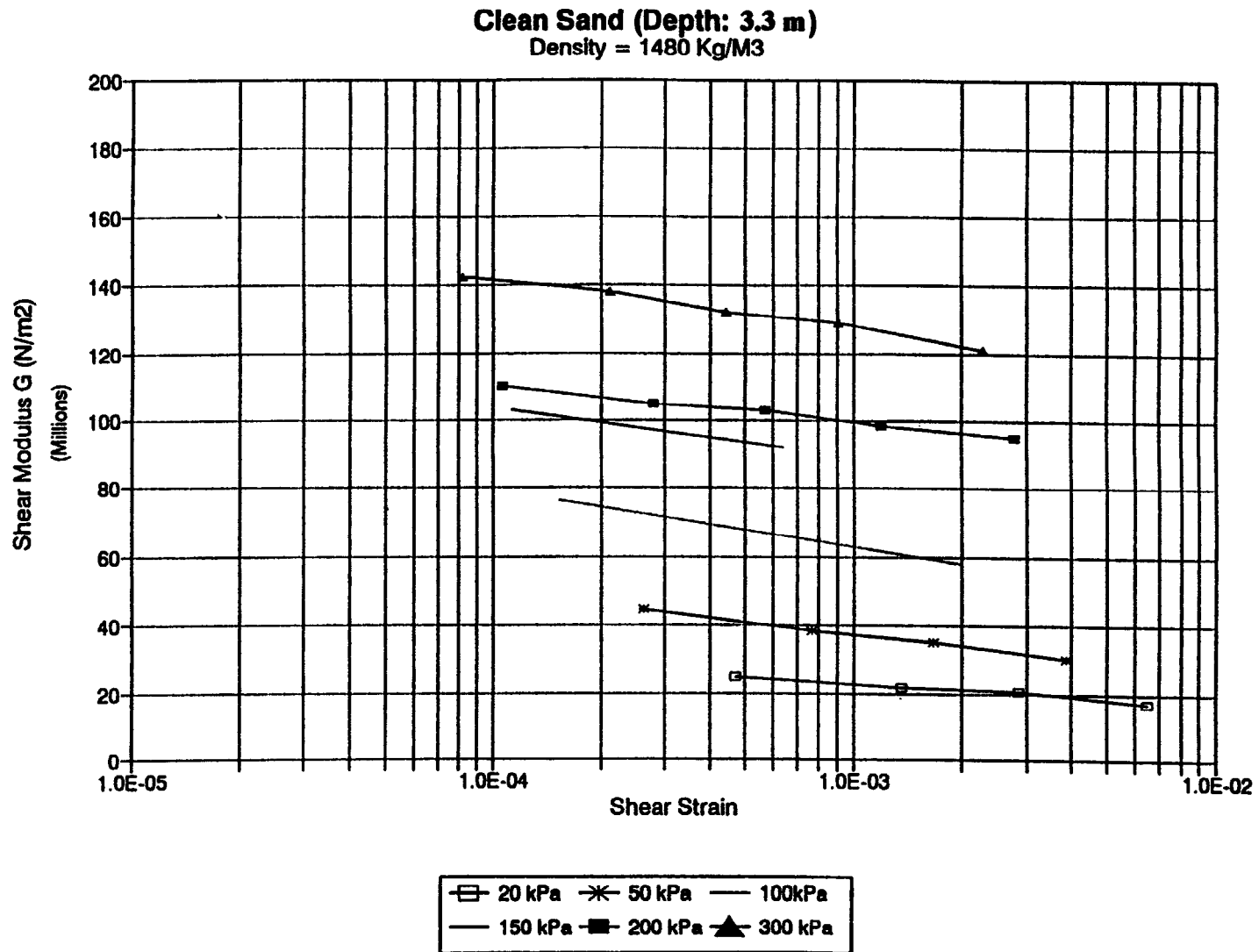
Figure A19: Resonant Column Test Results @ 3.3 m
