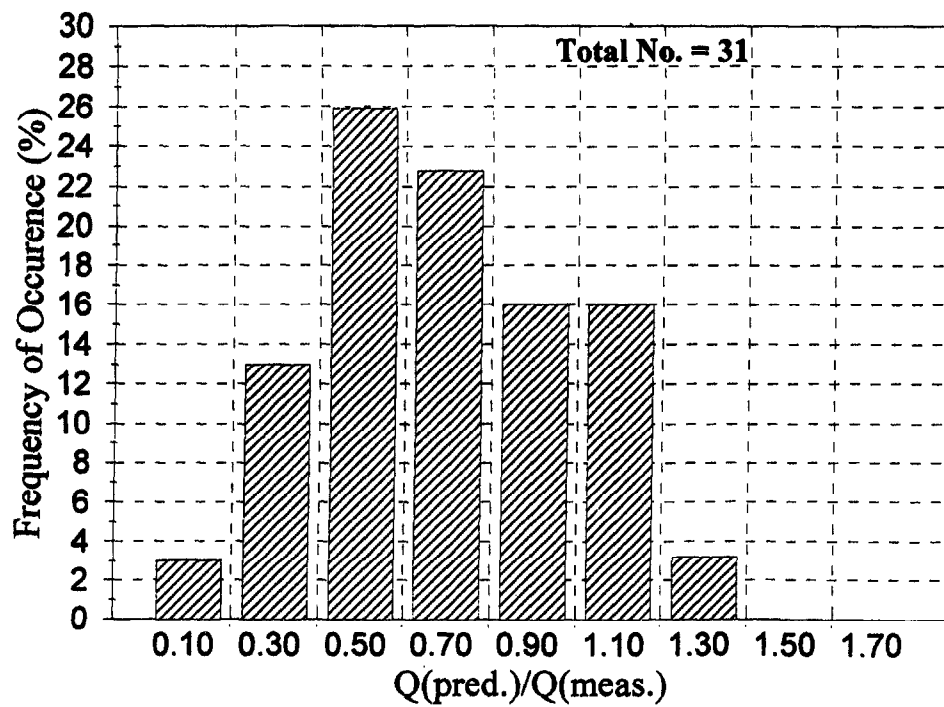
Figure 5.2: Distribution of Q_{pred.}/Q_{meas.} for 25-mm Settlement: 3-m North Footing
