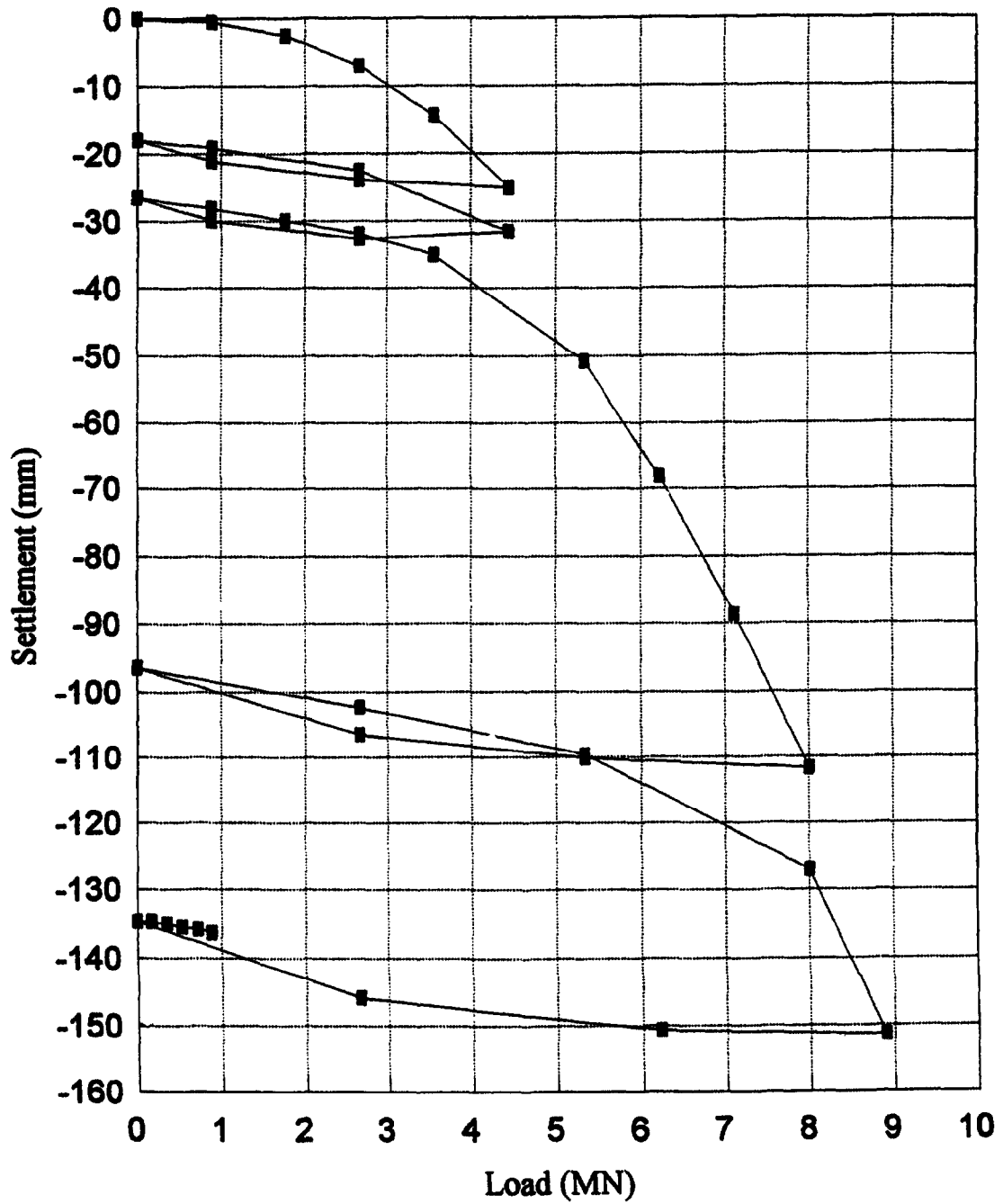
Figure B10: Load Settlement Curve for 3.0-m(s) Footing - Avg. 30-Minute Curve
