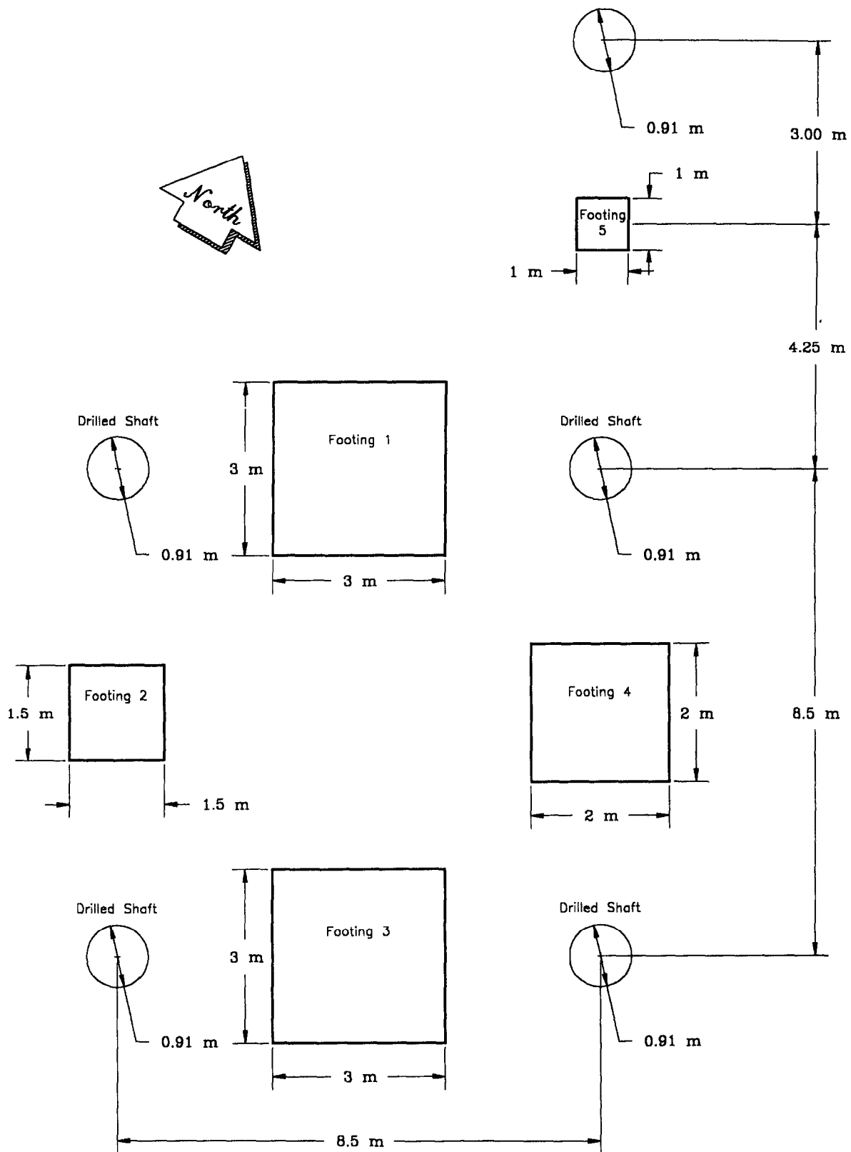
Figure 4.1: Footing/Pier Layout
