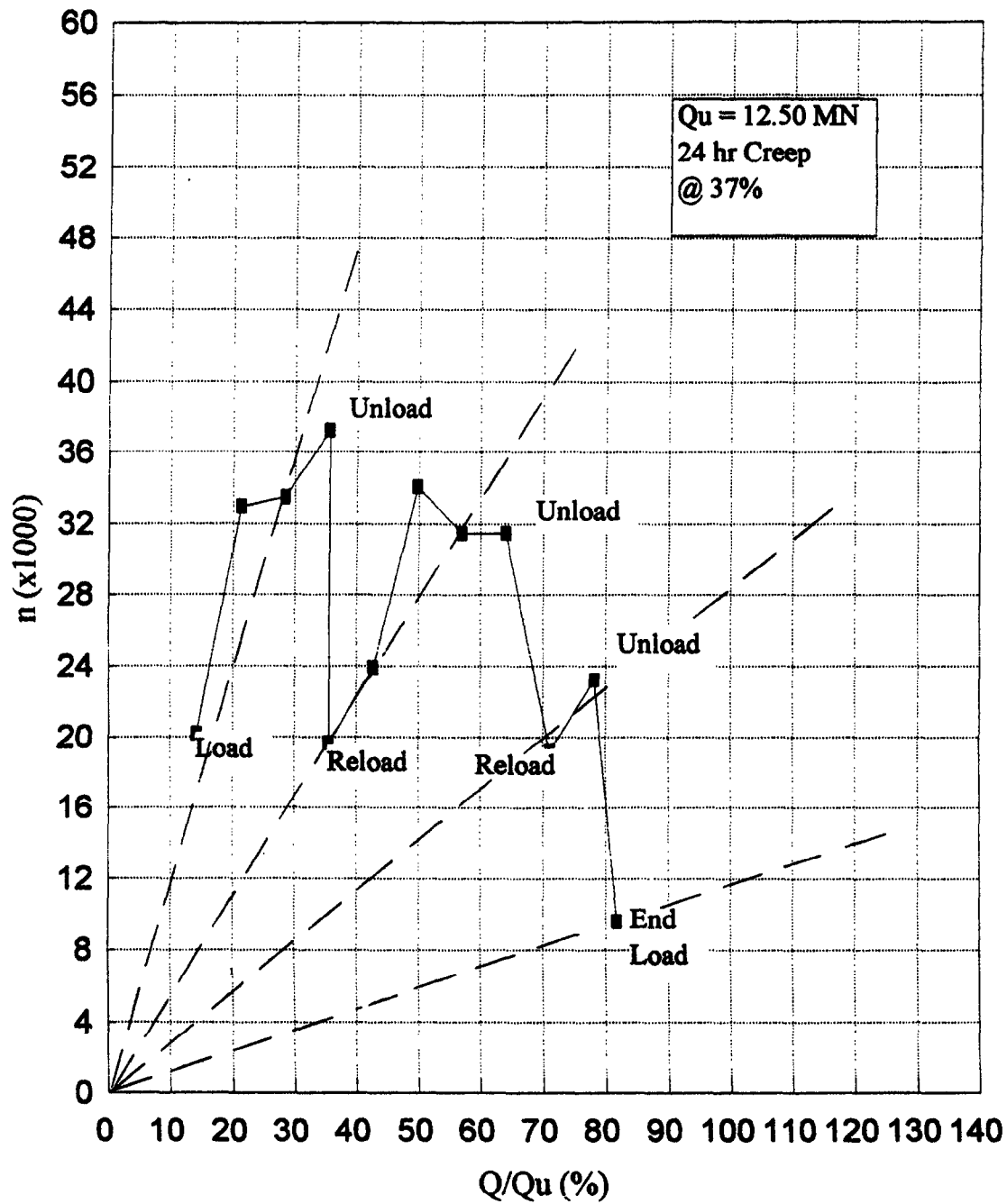
Figure 7.6: Creep Exponent Curve for 3.0-m North Footing - Q_u = 12.50\text{-MN}
