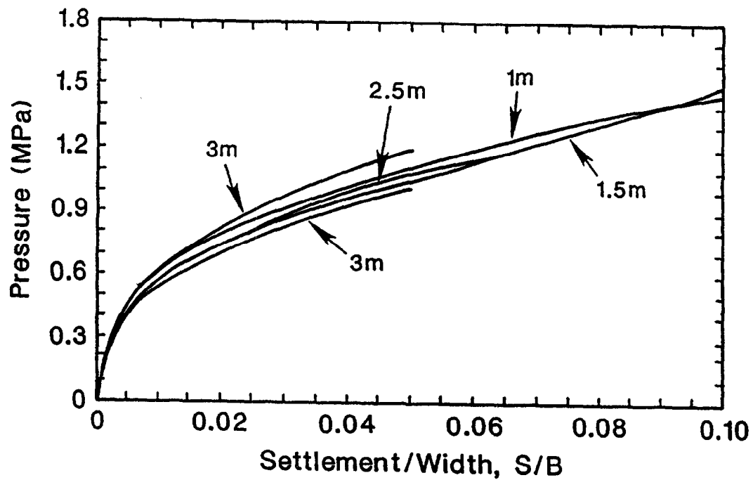
Figure 7.4: Pressure vs. Settlement/Width Curves
