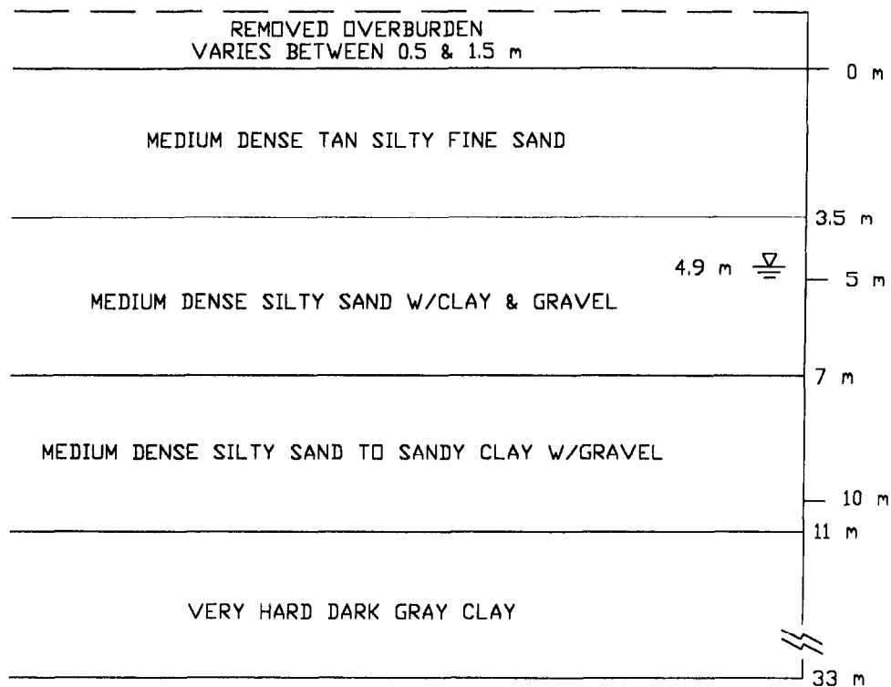
Figure 4.5: General Soil Layering
