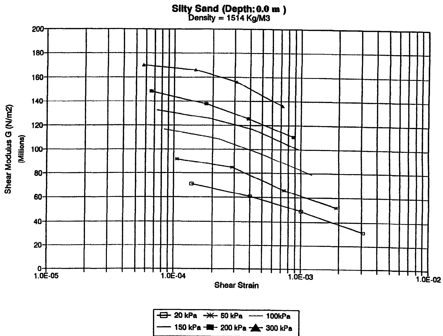
Figure A17: Resonant Column Test Results @ 0.0 m
