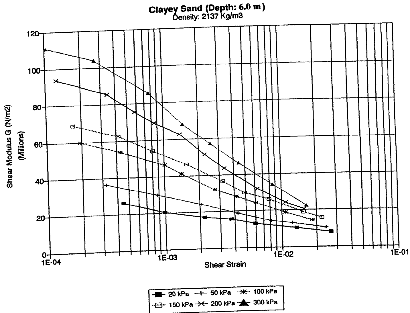
Figure A20: Resonant Column Test Results @ 6.0 m
