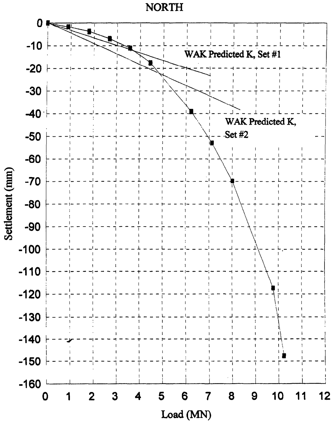
Figure 6.9: Predicted Stiffness on 3.0-m North Footing Before Load Test
