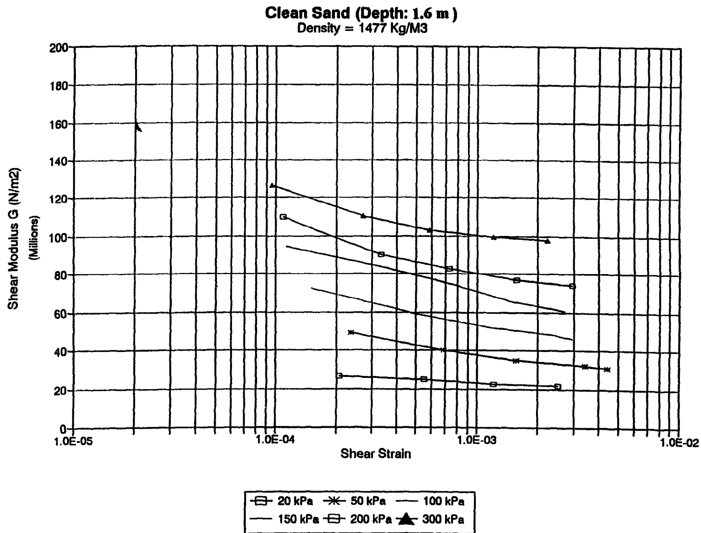
Figure A18: Resonant Column Test Results @ 1.6 m
