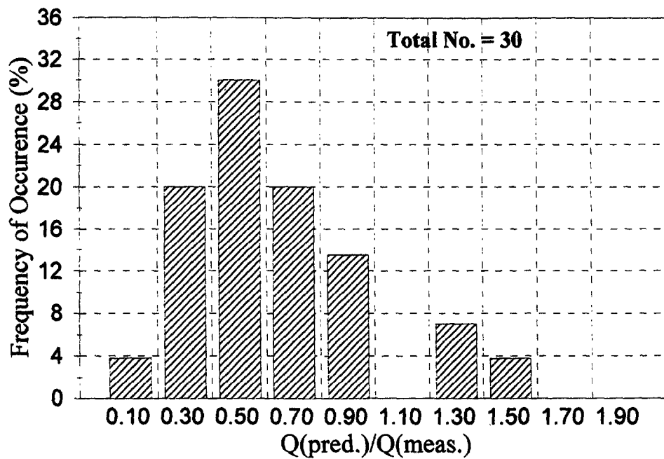
Figure 5.11: Distribution of Q_{pred.}/Q_{meas.} for 150-mm Settlement: 1.0-m Footing
