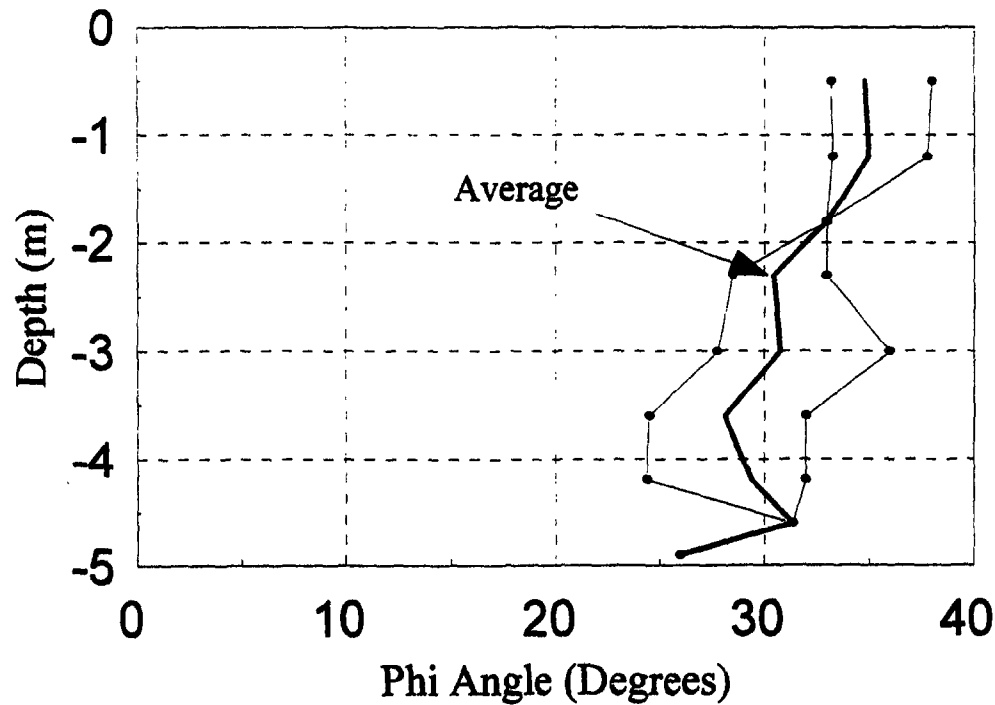
Figure 4.11: Range of BHST Results
