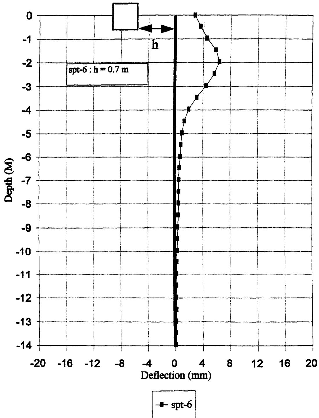
Figure D1: Inclinometer Test - 1.78-MN Failure Load - N-S Direction, 1.0 M Footing
