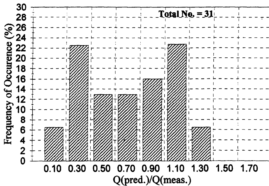
Figure 5.3: Distribution of Q_{pred.}/Q_{meas.} for 25-mm Settlement: 3-m South Footing
