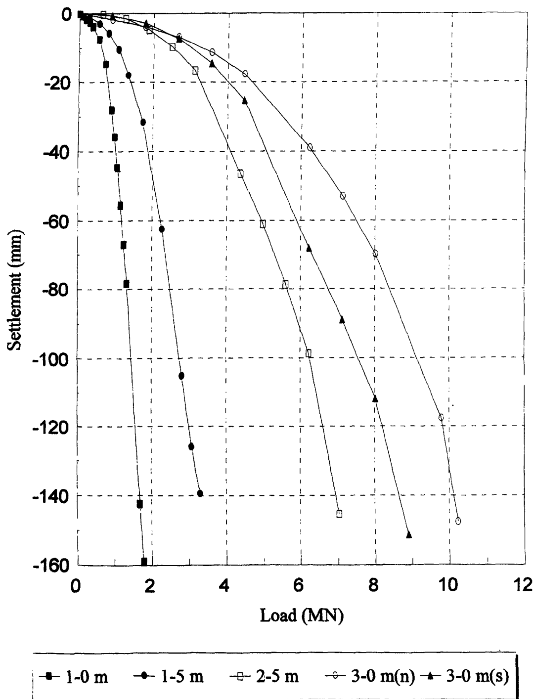
Figure 4.12: 30-Minute Monotonic Load Settlement Curves for All Footings
