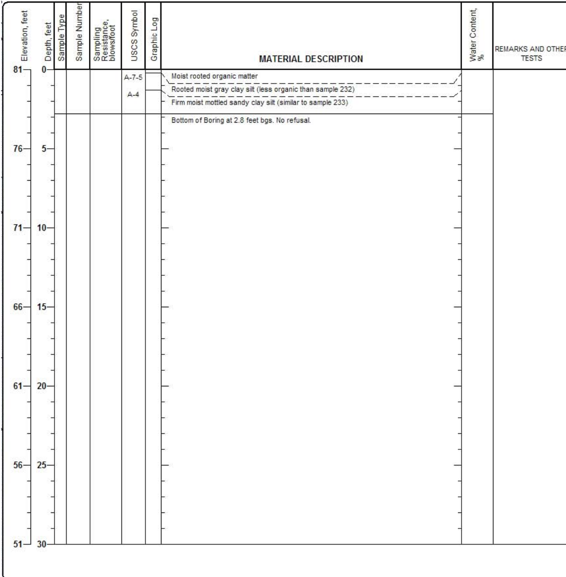
Figure B-12. Boring log, station 268+00.
