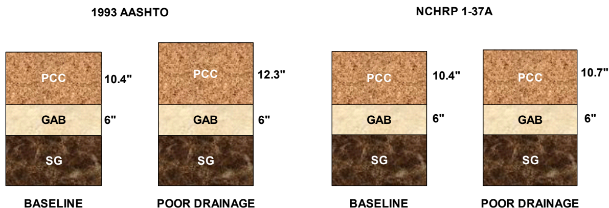
Figure 6-19. Summary of rigid pavement sections: poor drainage scenario.
