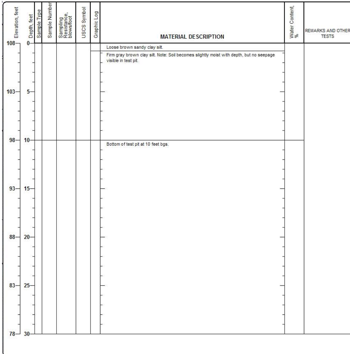
Figure B-15. Test pit log, station 255+50.
