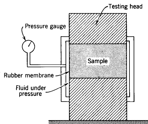
Figure 5-13. Schematic of stabilometer test setup for measuring R-value (Yoder and Witczak, 1975).
