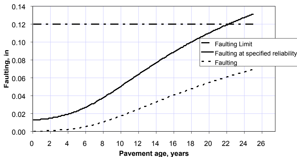
Figure 6-4. Predicted faulting performance for soft subgrade scenario.
