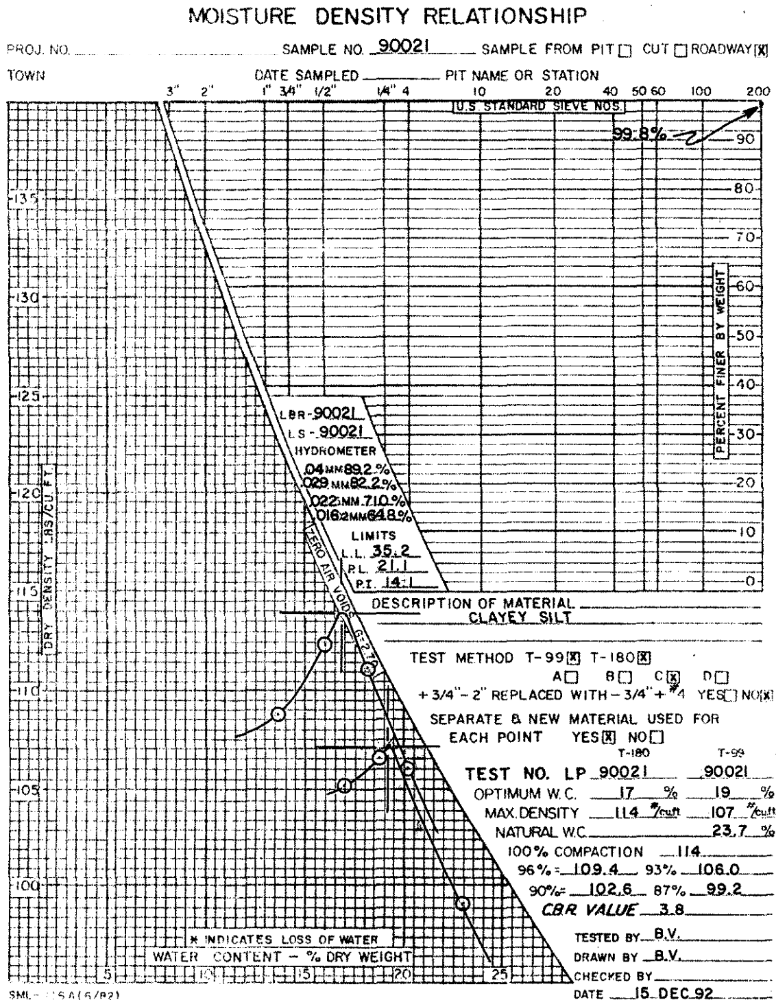
Figure B-21. Compaction curves for clayey silt subgrade soil (sample 90021).
