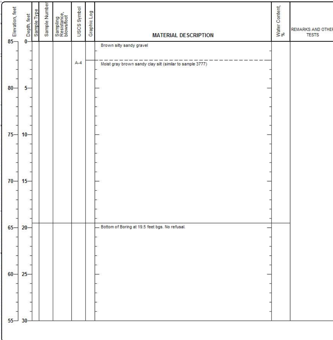
Figure B-10. Boring log, station 262+00.
