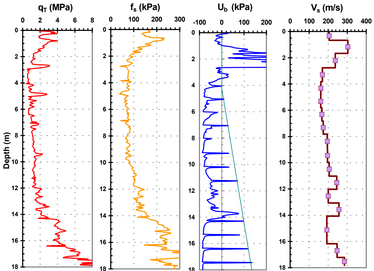
Figure 5-28. Results of Seismic Piezocone Sounding in Residual Soils in Coweta County, Georgia showing four independent readings with depth. Note: Penetration porewater pressures allowed to dissipate at each rod break.
