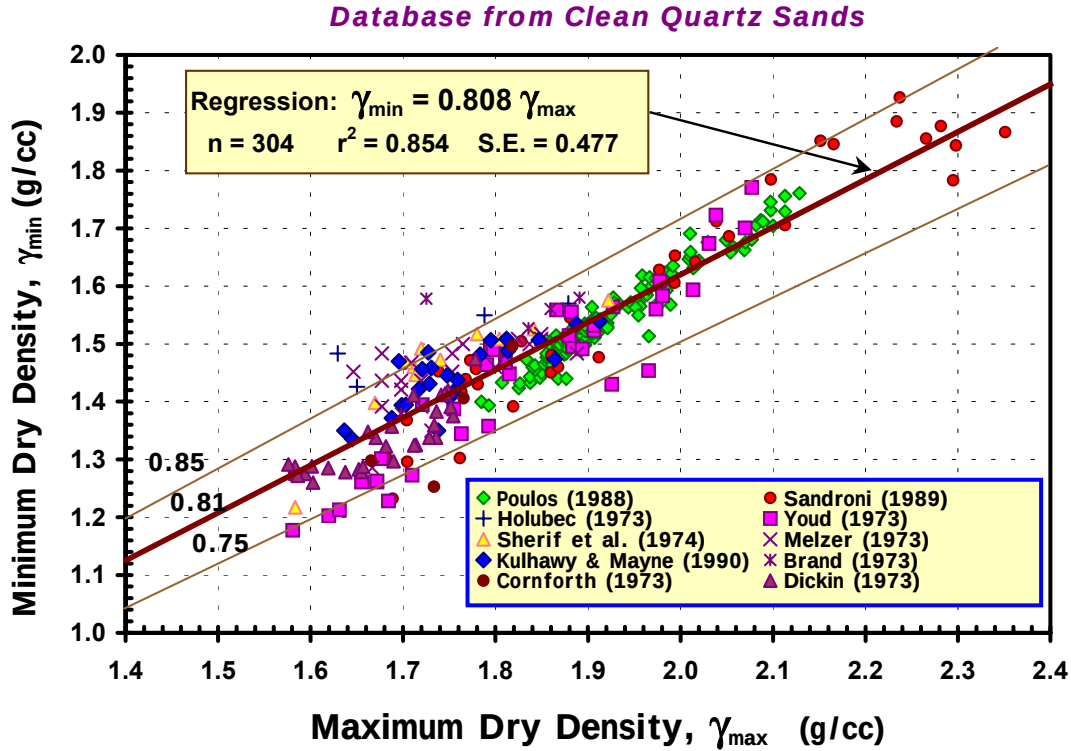
Figure 9-6. Interrelationship Between Minimum and Maximum Dry Densities of Quartz Sands. (Note: Conversion in terms of mass density and unit weight: 1 \text{ g/cc} = 9.8 \text{ kN/m}^3 = 62.4 \text{ pcf} )
