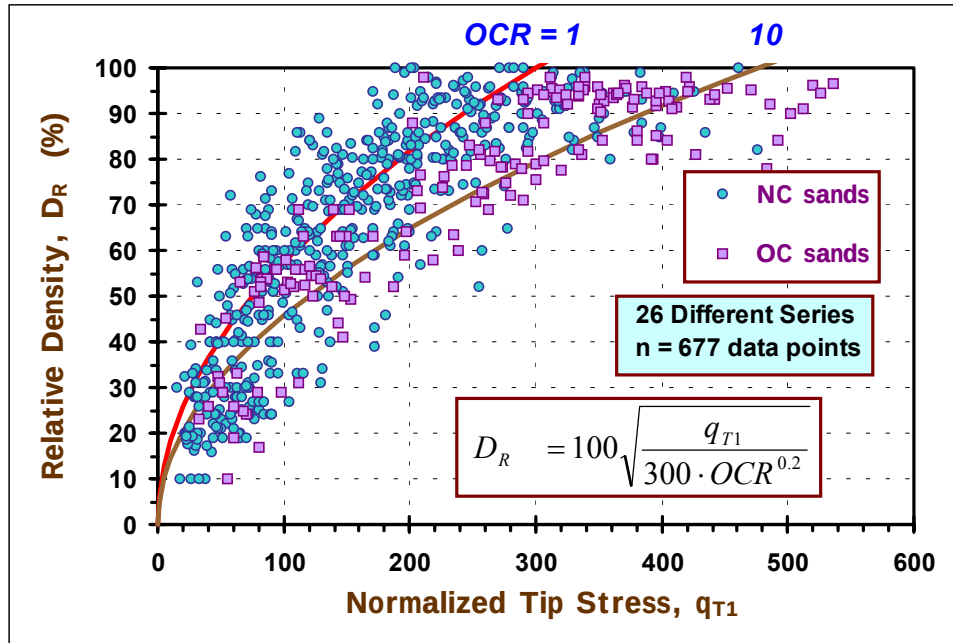
Figure 9-9. Relative Density Evaluations of NC and OC Clean Quartz Sands from CPT Data. Note: normalized resistance is q_{t1} = q_c / (F_{v0}')^{0.5} with stresses in atmospheres (1 atm = 1 tsf = 100 kPa).
