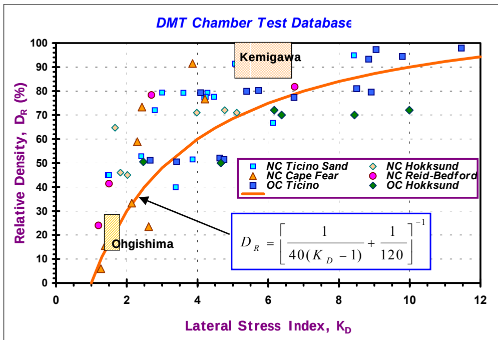
Figure 9-10. Relative Density of Clean Sands Versus DMT Horizontal Stress Index, K_D = (p_0 - u_0) / F_{v0}' .
