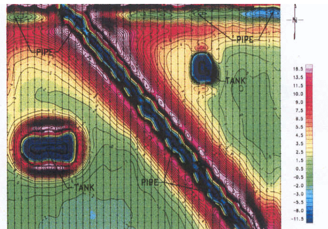
Figure 5-36. EM Survey to Detect Underground Storage Tanks (Geonics EM-31 Survey by GeoVision).
