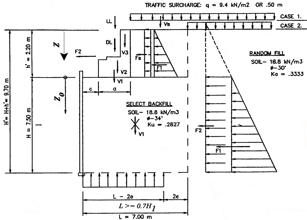
a) Loads on abutment
