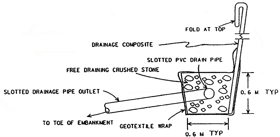
a) GROUND WATER AND SURFACE DRAINAGE
