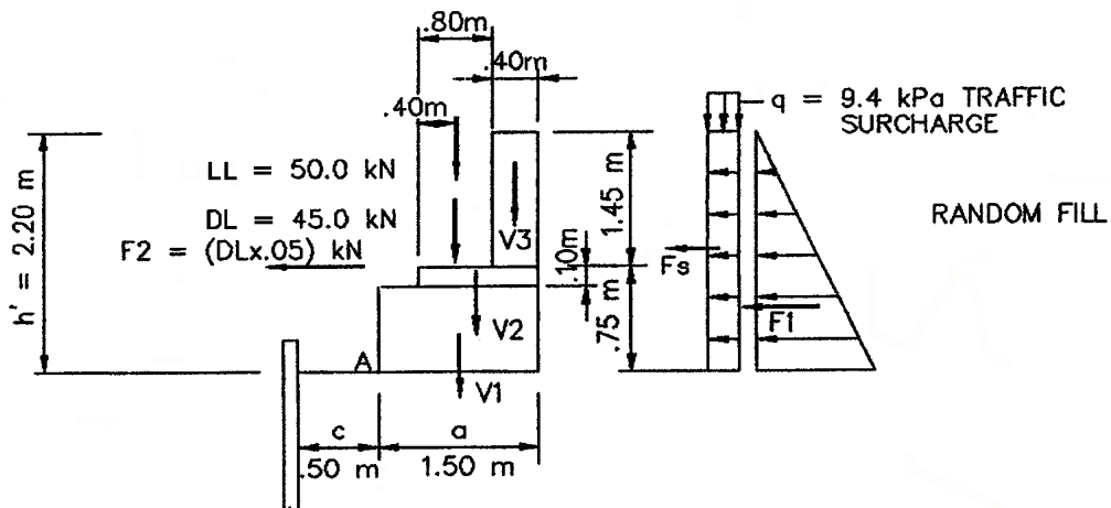
b) Abutment seat configuration
