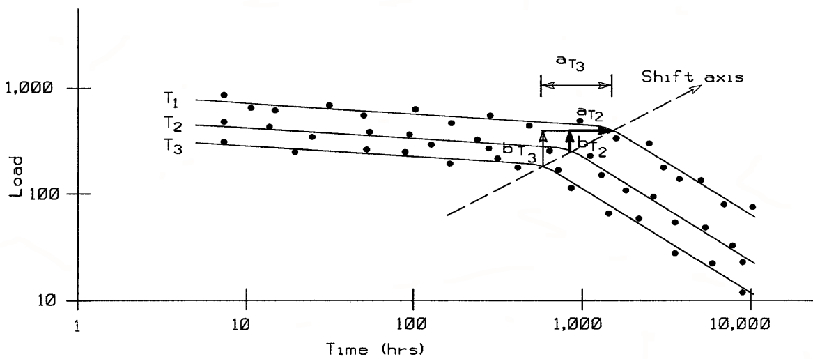
(b) Stress rupture envelope with "knee"
