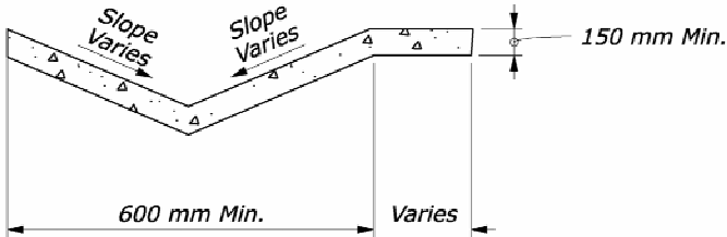
CONCRETE V-DITCH DETAIL
