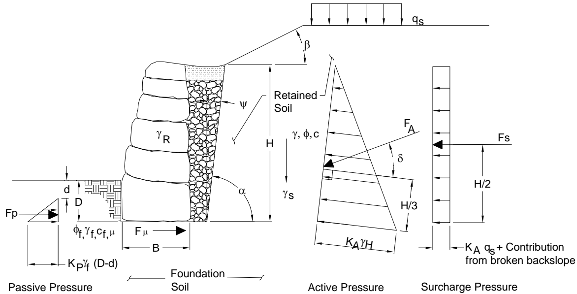
Figure 30. Graphic. Schematic rockery section showing critical dimensions and parameters to be determined for design.
