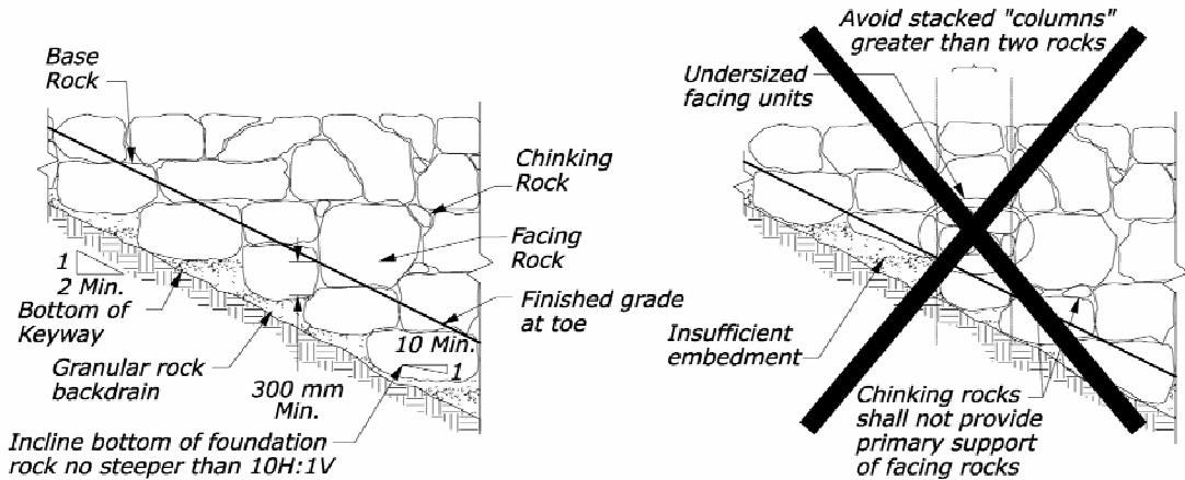
CORRECT PARTIAL TYPICAL PROFILE
