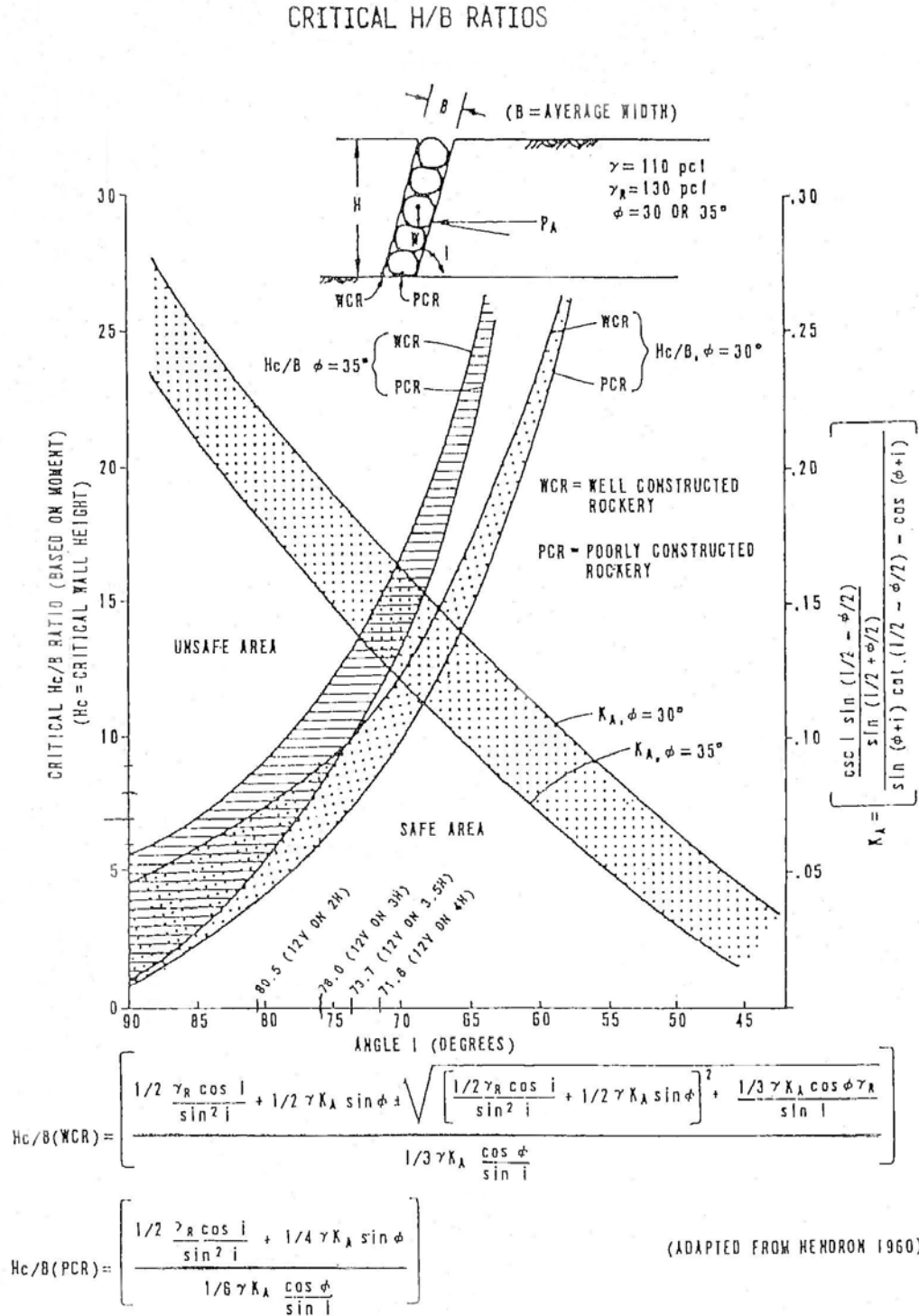
Figure 9. Chart. Critical height-to-base-width (H/B) ratios for poorly constructed rockeries (PCRs) and well-constructed rockeries (WCRs), after Hendron.
