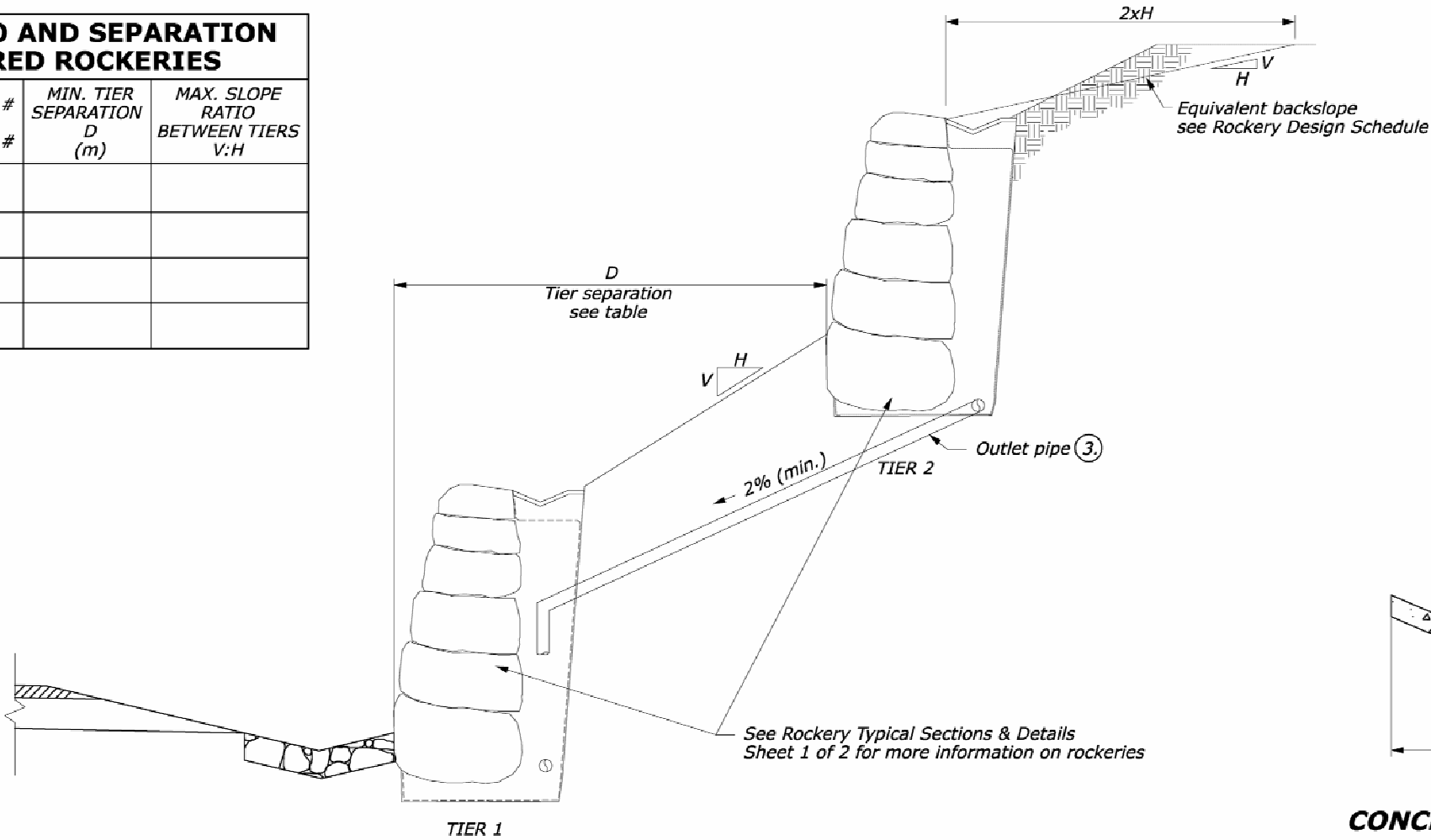
ROCKERY WITH TIERS TYPICAL SECTION
