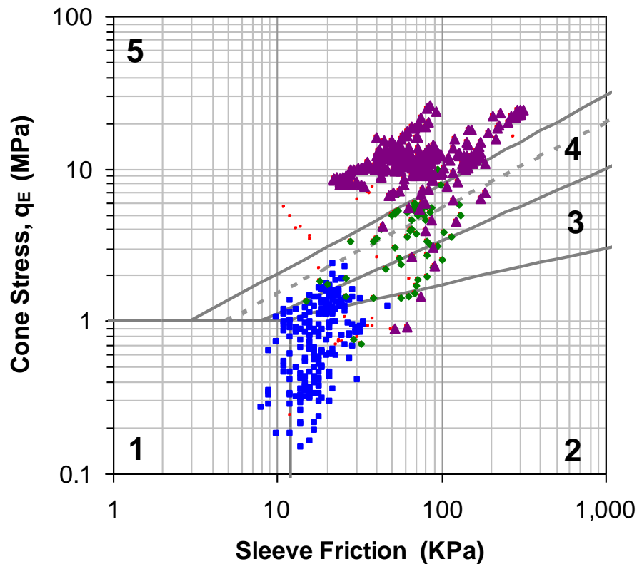
Fig. 2.11 The CPT sounding shown in Fig. 2.1 plotted in a Eslami-Fellenius profiling chart.
