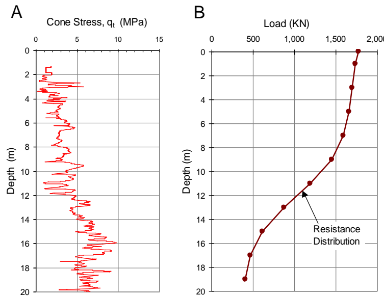
Fig. 8.35A CPT profile
