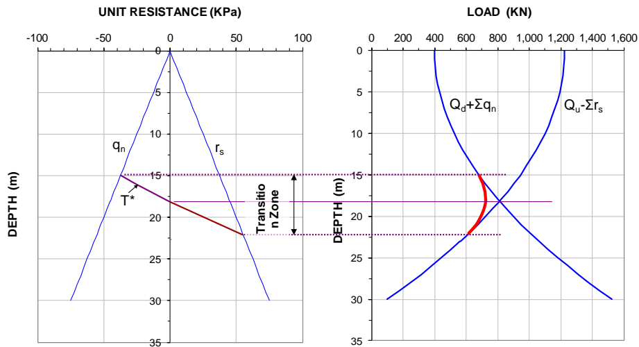
Fig. 7.6b The Principles of Transition from Unit Negative Skin Friction to Unit Positive Shaft Resistance and from Increasing Load to Decreasing Load Distribution ( not the same example as in 7.6a )
