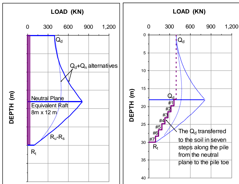
Fig. 7.20 Load distribution and transfer of the dead load to the soil below the neutral plane
