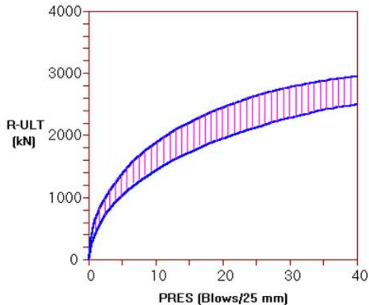
Fig. 7.15 Bearing Graph from WEAP Analysis
