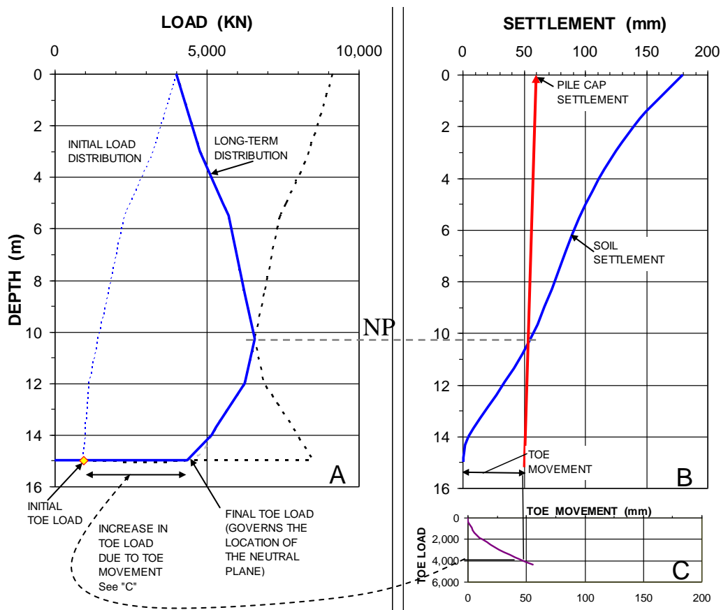
Fig. 8.29 Results of a typical trial-and-error approach to match a toe load, neutral plane location, and pile toe movement due to downdrag in the Unified Design Method
