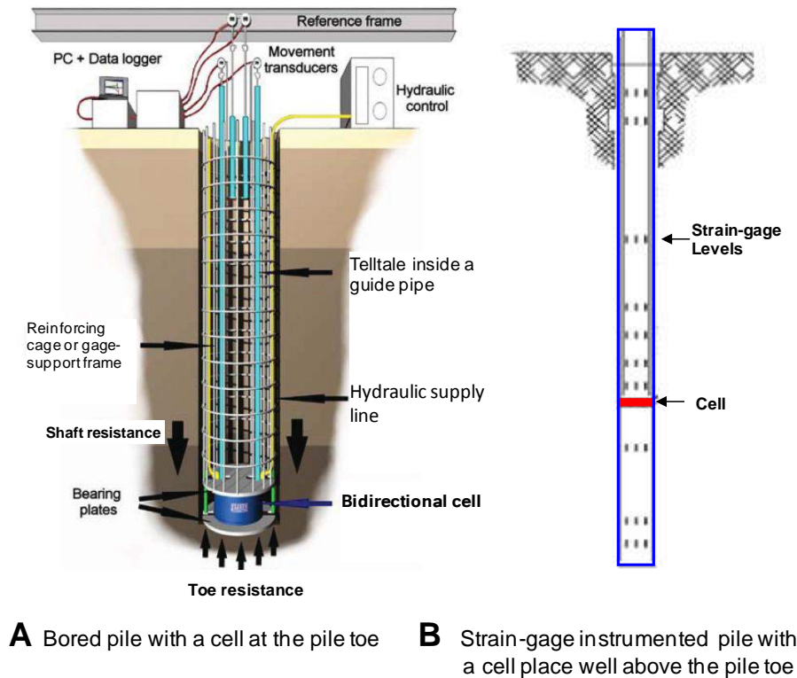
Fig. 8.24 Pile with bidirectional cell (from Loadtest Inc. flier)
