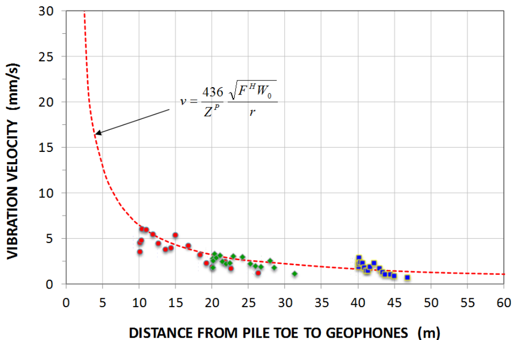
Fig. 9.25 Vibration velocity per Eq. 9.30 plotted with measurements of vibration velocity. (Data from Nilsson 1989, as presented by Massarsch and Fellenius 2014).
