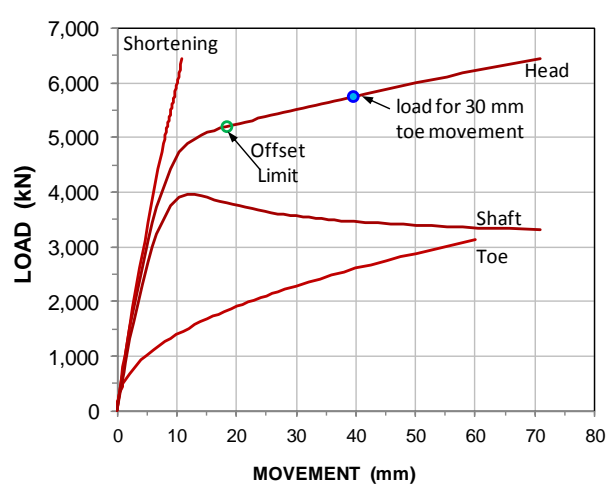
Fig. 8.19 Same pile without residual load
