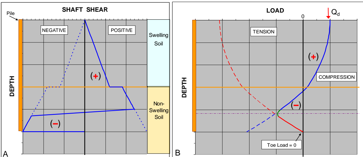
Fig. 7.24 Distributions of unit shaft shear and load for a pile in swelling soil
