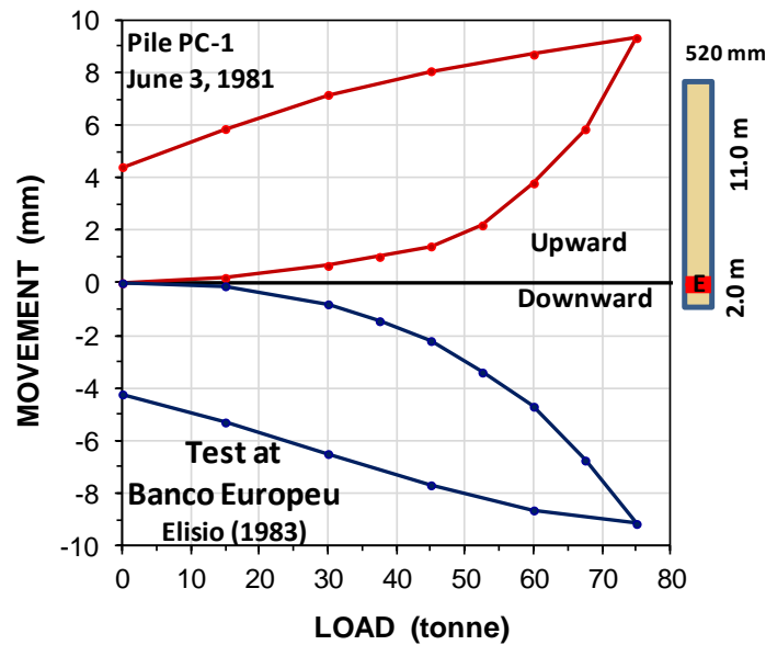
Fig. 8.25 Illustration of the main results of a bidirectional cell test: Upward and downward load-movements measured in a test on a 520-mm diameter, 13 m long pile (data from Elisio 1983).
