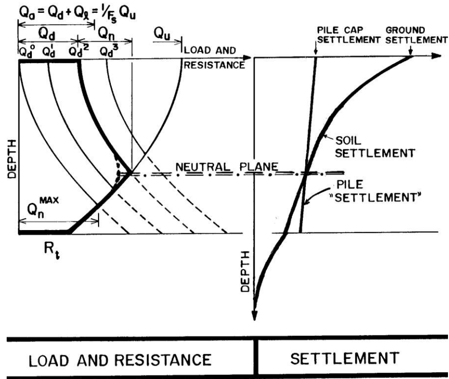
Fig. 7.23 Load-Transfer and Resistance Curves and Settlement Distribution
