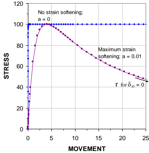
Fig. 8.16 Zhang function for t-z shaft shear force vs. movement
