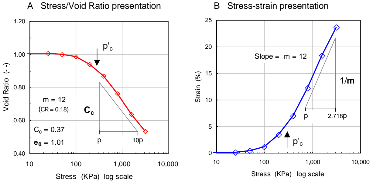
Fig. 3.1 Results from a consolidometer test (data from Bowles, 1988). (The preconsolidation stress is taken directly from the source where it was indicated to have been determined "by eye-balling" to 280 kPa).
