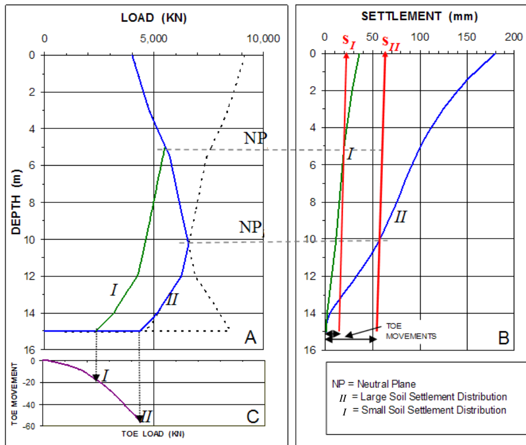
Fig. 8.28 Example of the mutual dependence of soil and pile settlement to load distribution (same case as in Fig. 7.18)
