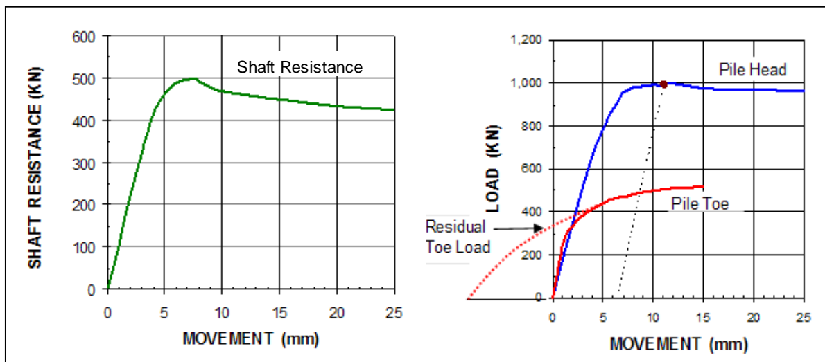
Fig. 7.8 Load-Movement curves for shaft resistance and for total ("Pile Head") and toe resistances.
