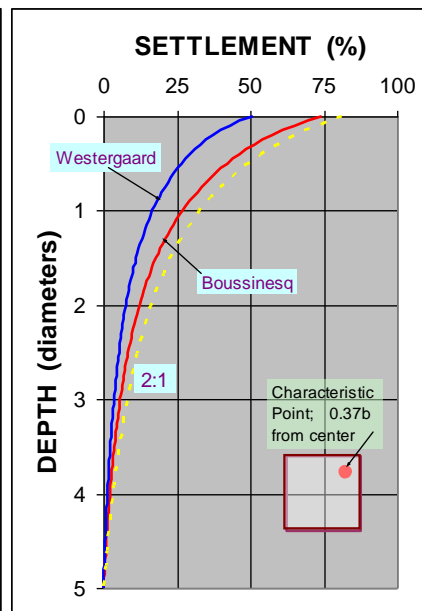
Fig. 1.11 Settlement distributions
