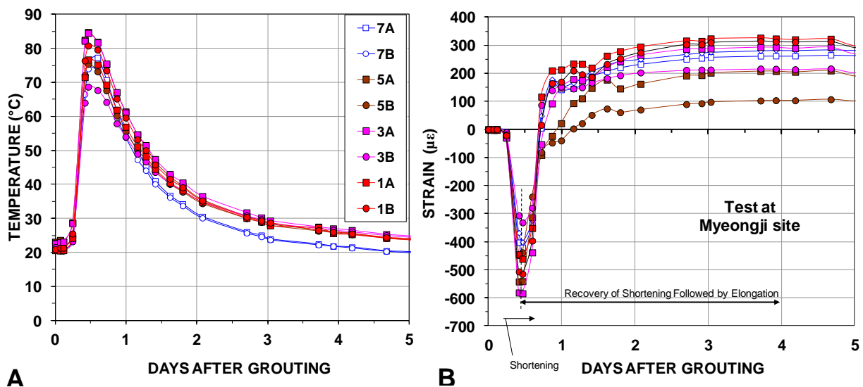
Fig. 8.33 Development of temperature and strain in a 35 m long spun-pile pile during first 5 days after grouting (reducing strain indicates compression/shortening)
