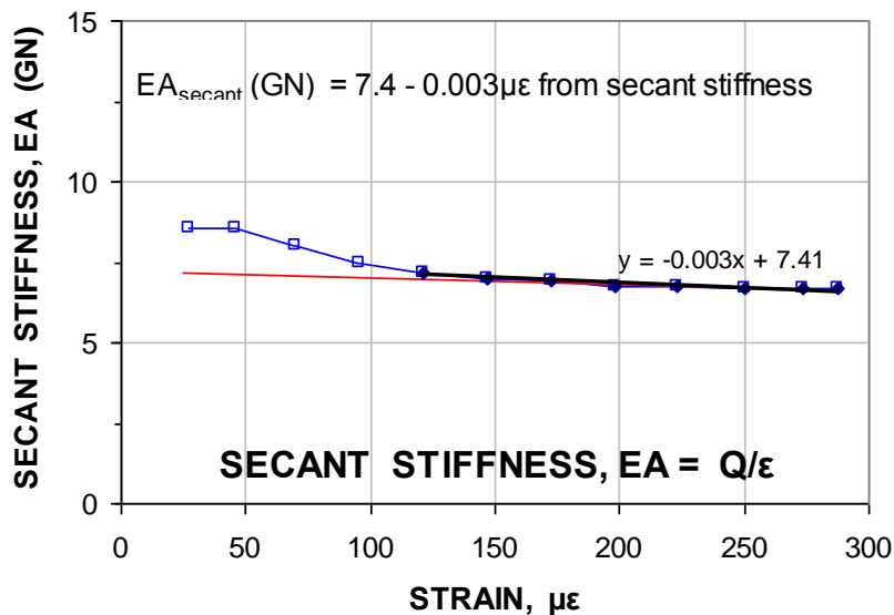
Fig. 8.41 Secant stiffness vs. measured strain for a 400-mm concreted steel pipe pile (Fellenius 2012)
