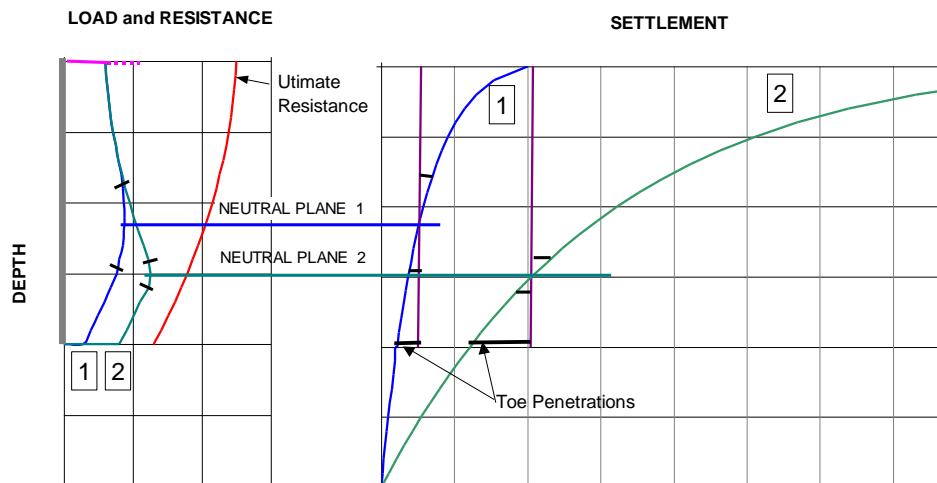
Fig. 7.17 Combination of load-and-resistance diagram and settlement diagram
