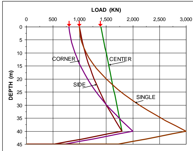
Fig. 7.28 Load distribution in the pile group piles ("Center", "Side", and "Corner") and in a single pile ("Single"), assuming the Center piles fully shielded, and the Center and Corner piles partially shielded from the negative skin friction effect
