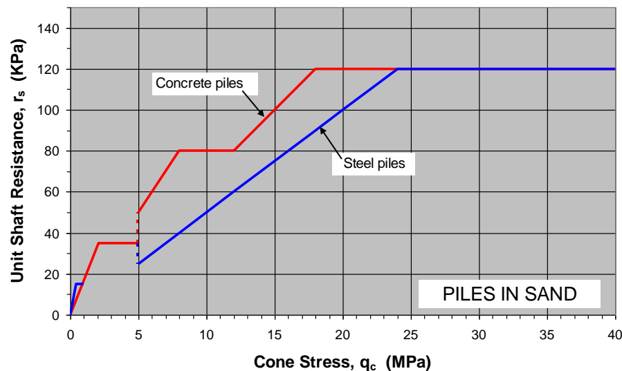
Fig. 7.13B Unit shaft resistance versus cone stress, q_c , for piles in sand according to the LCPC method.
