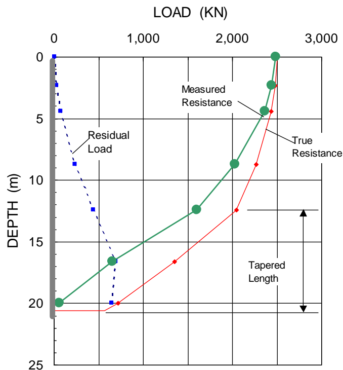
Fig. 8.50 The example case with Measured Load, Residual Load, and True Resistance
