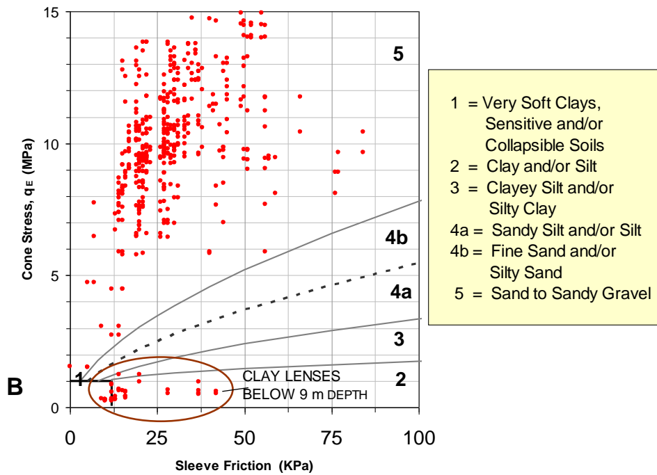
Fig. 2.38 The CPT data from one of the 7-day after cone soundings plotted in an Eslami-Fellenius profiling chart (Eslami and Fellenius 2000).
