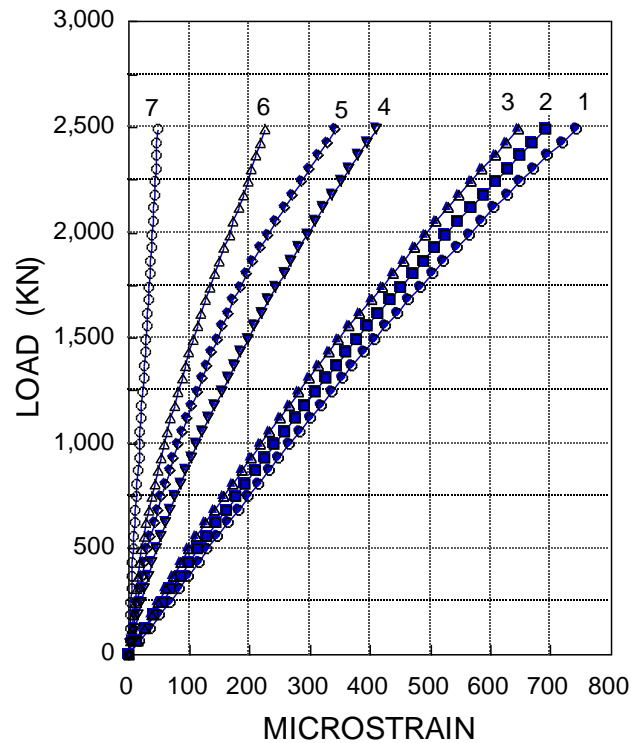
Fig. 8.46 Strain measured at Gage Levels 1 through 7
