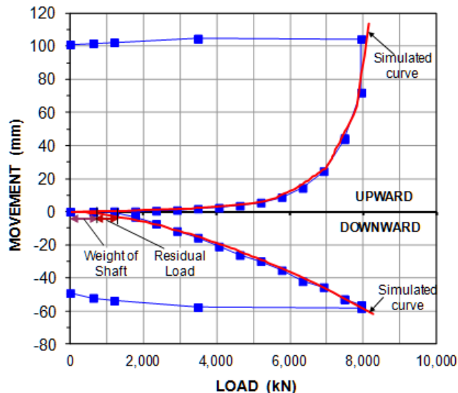
Fig. 8.26 Results of a bidirectional test on a 1,200 mm diameter, 40 m long bored pile
