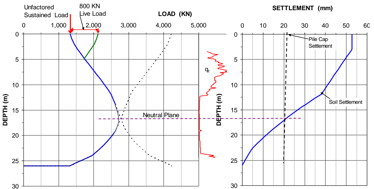
Fig. 8.31 The effect of adding a live load to the pile head
