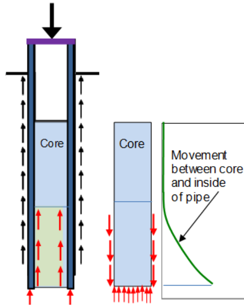
Fig. 7.36 Force vectors in static loading of an open-toe pipe pile with inside soil column, a "core"
