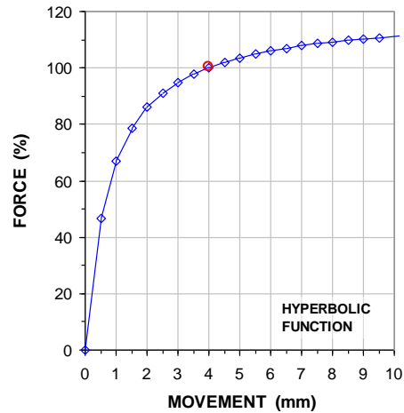
Fig. 8.13 Hyperbolic function for t-z shaft shear force vs. movement
