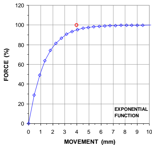
Fig. 8.14 Exponential function for t-z shaft shear force vs. movement
