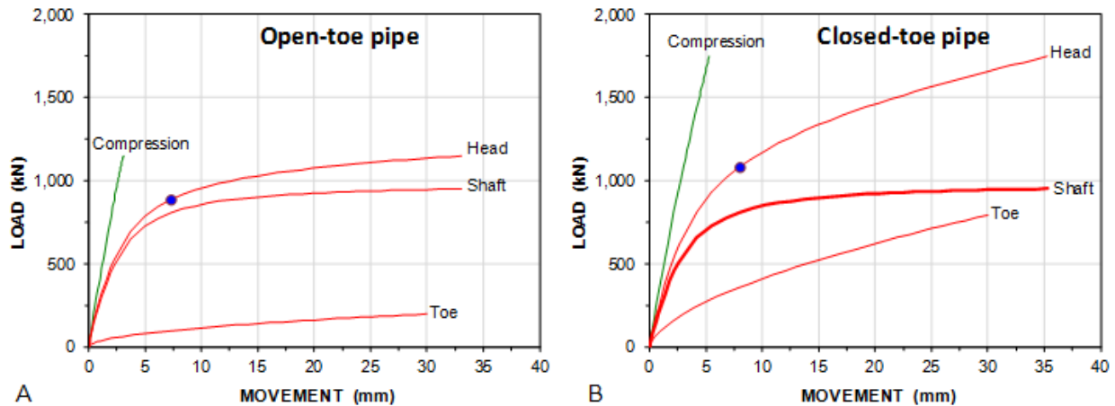
Fig. 7.37 Fig. 20 Load-movement curves for a static loading test on a pipe pile A. Test an open-toe pipe pile and B. Test on a closed-toe pipe pile.
