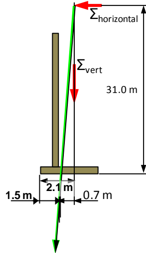
Fig. 5.8 Forces and stresses affecting the wall
