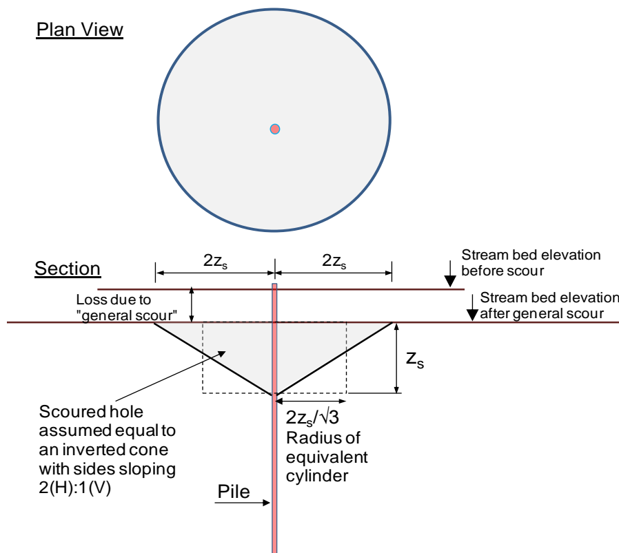
Figure 7.43. Scour configuration according to the FHWA Manual (Hannigan et al. 2006)
