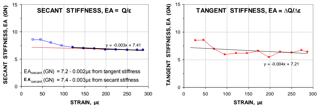
Fig. 8.49 Comparison between stiffness determined from tangent and secant modulus approaches
