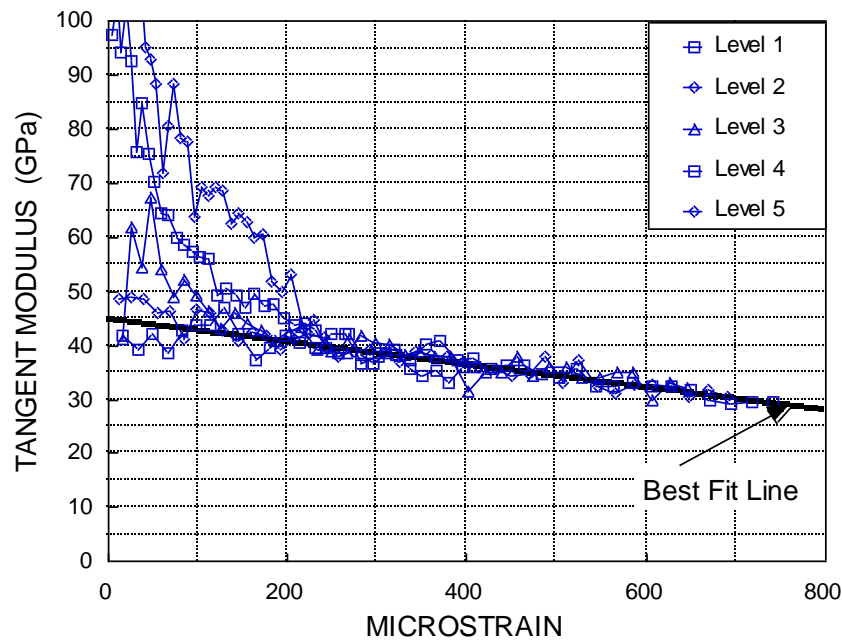
Fig. 8.47 Tangent Modulus Diagram
