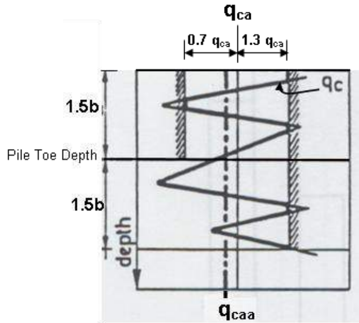
Fig. 7.12 Averaging the cone resistance according to the LCPC method. The “ b ” stands for pile toe diameter. (Bustamante and Gianselli, 1982).
