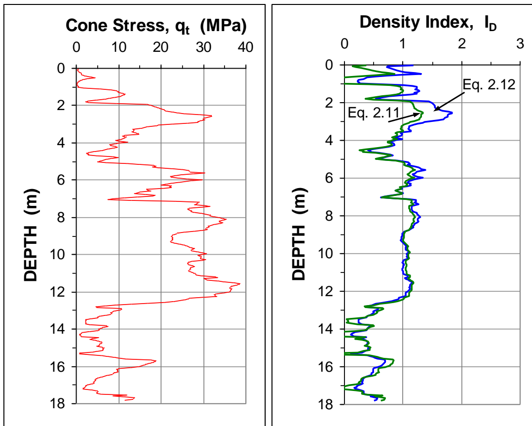
Fig. 2.24 Profiles of cone stress and Density Index, I_D , determined from the CPTU sounding according to Eq. 2.11 and 2.12. No reference values are available from the site. (CPT data from McVay et al. 1999).
