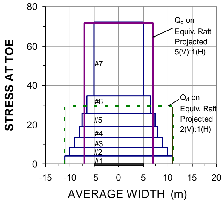
Fig. 7.21 Distribution at the pile toe of projected stresses from the pile dead load
