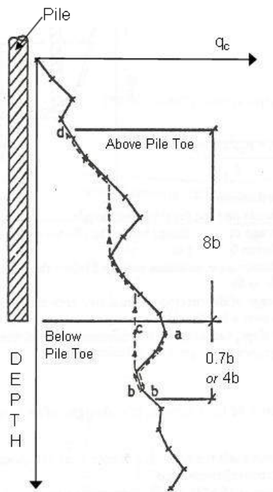
Fig. 7.9 Determining the influence zone for toe resistance (Schmertmann, 1978)
