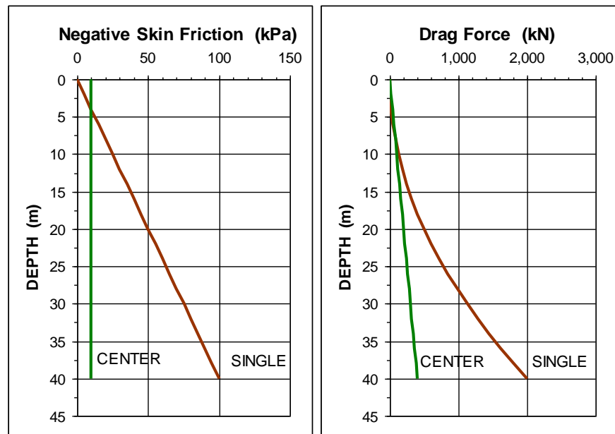
Fig. 7.27 Distributions of unit negative skin friction and of accumulated drag force
