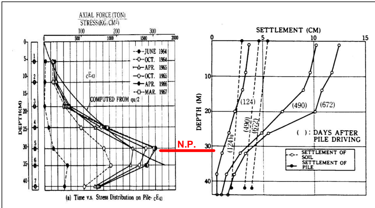
Fig. 7.16 Combination of two diagrams taken from Endo et al. (1969)
