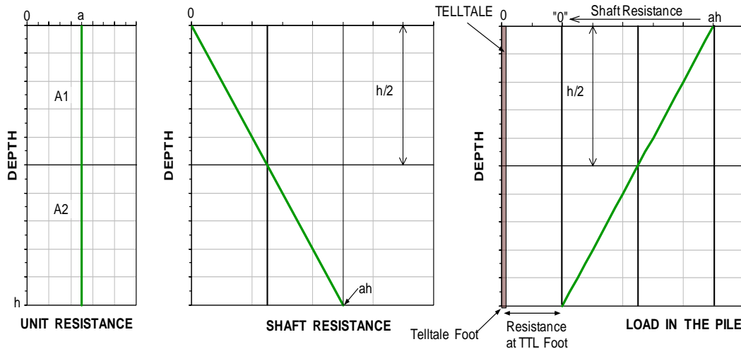
Fig. 8.22 Load distribution for constant unit shaft resistance
