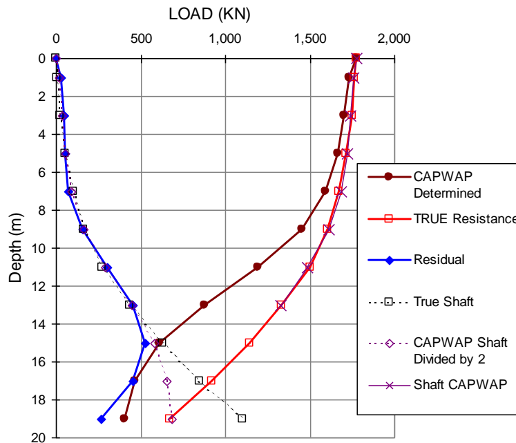
Fig. 8.37 Final Results: Measured Load, Residual Load, and True Resistance
