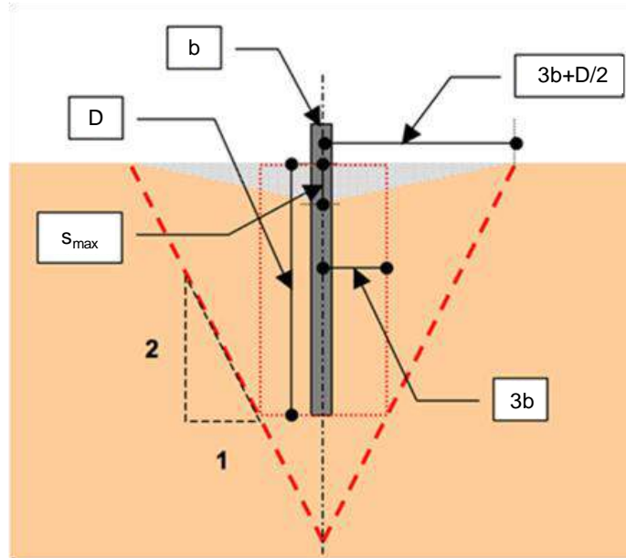
Fig. 9.27 Basic method of estimating settlements adjacent to a single pile in homogeneous sand (after Massarsch 2004)
