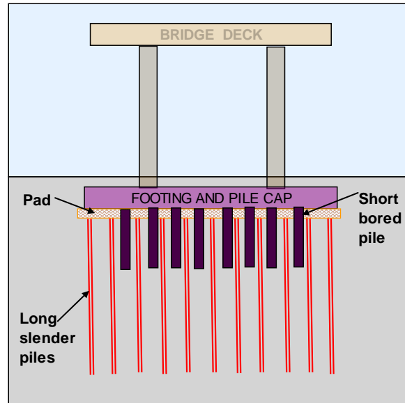
Fig. 7.7 Piled pad foundations for the Golden Ears Bridge piers. (After Sampaco et al. 2008).
