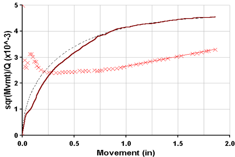
Fig. 8.2 Hansen's Plot for the 80 percent criterion
