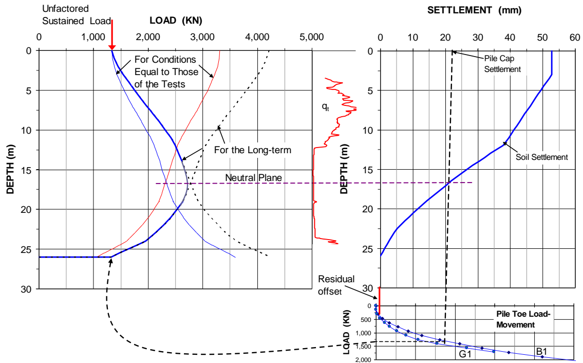
Fig. 8.30 Compilation of test and analysis data: Load distribution in the bidirectional cell static loading test and during long-term conditions, Load distribution of soil settlement, and Load-movement relation for the pile toe determined in the bidirectional test. The soil profile is indicated in the inserted CPT cone stress diagram (Fellenius and Ochoa 2009)
