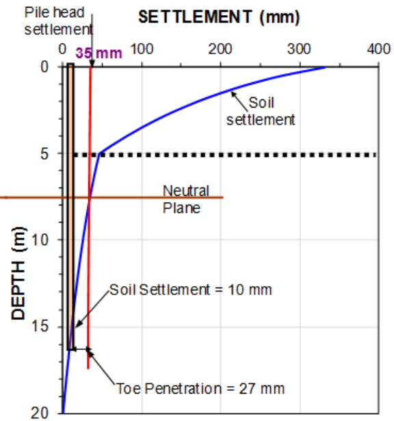
Fig. 10.4B Settlement distribution
