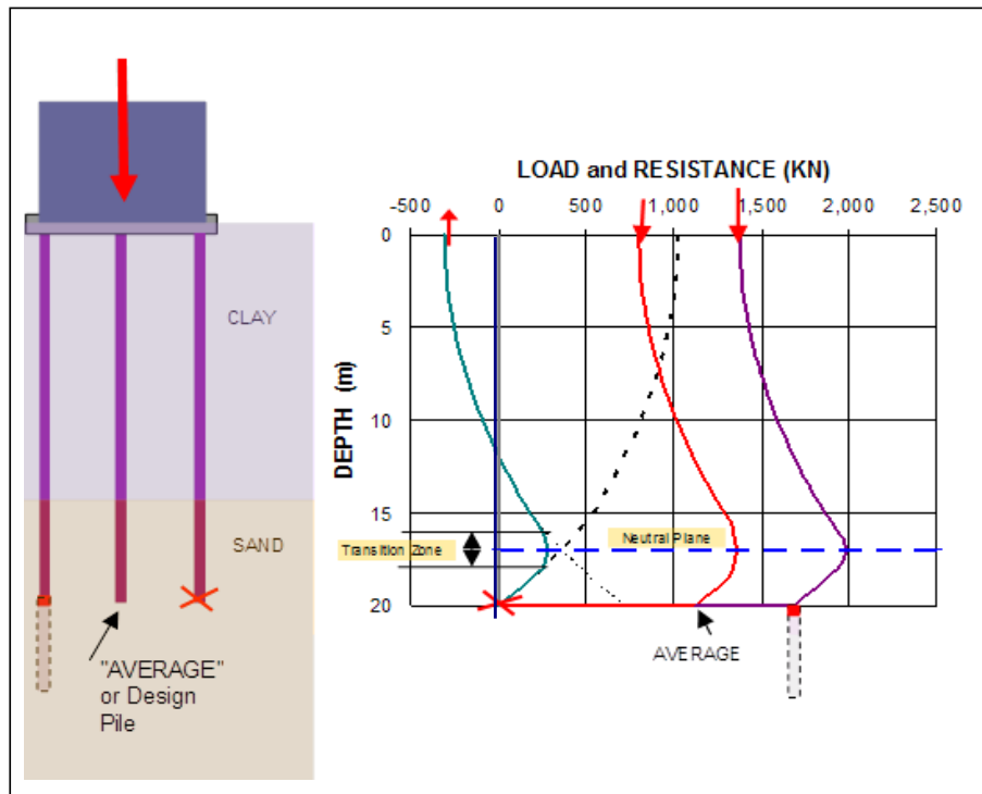
Fig. 7.30 Effect of different toe resistance on the ability of a pile to support the load from the structure
