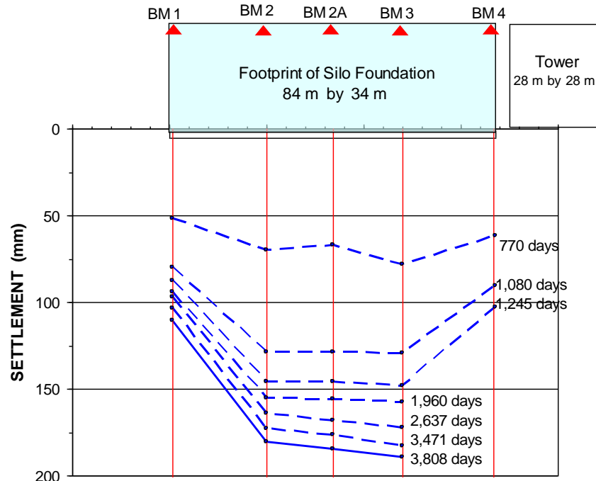
Fig. 7.32 Soil settlement monitored at five benchmarks along the side of the raft.
