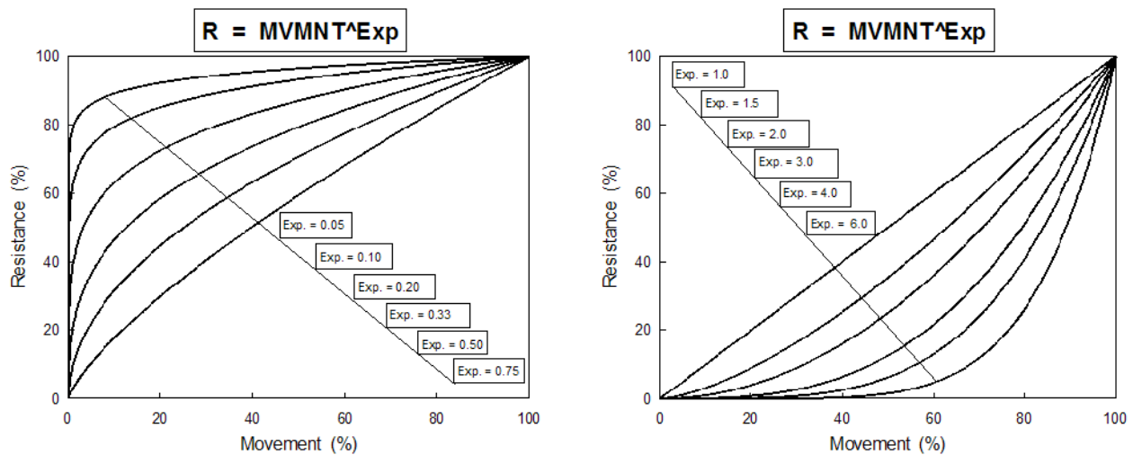
Fig. 8.11 Shape of t-z and q-z curves for a range of exponents
