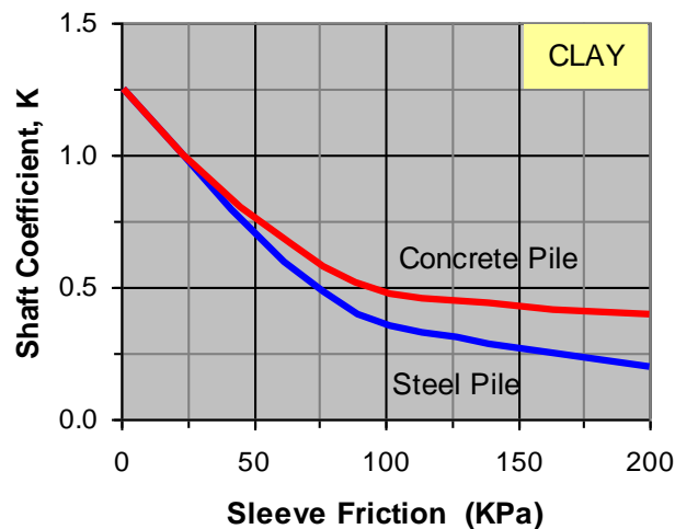
Fig. 7.11 Shaft coefficients for use in Eq. 7.8
