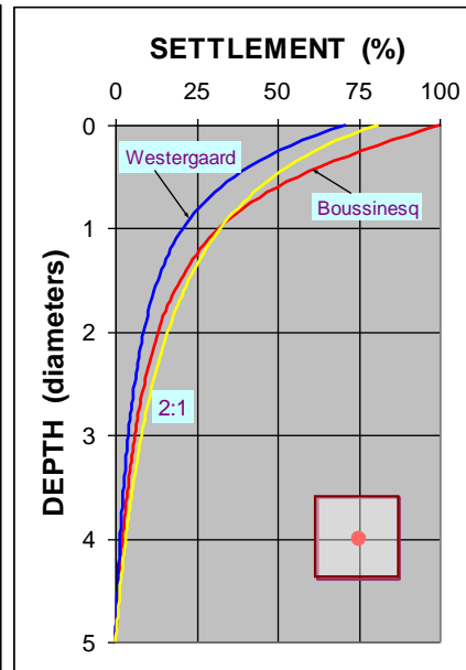
Fig. 1.9 Settlement distributions
