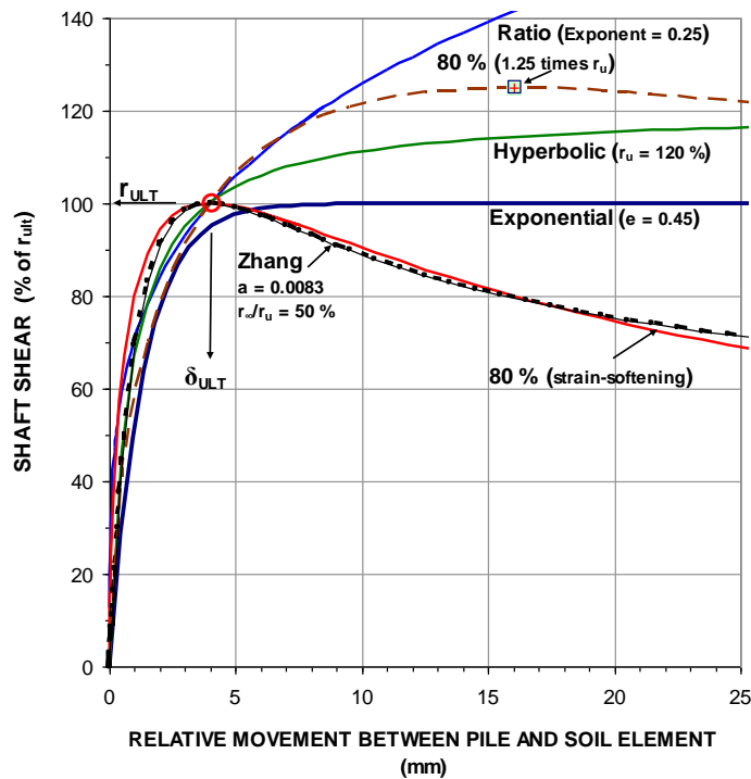
Fig. 8.17 All five function examples compiled
