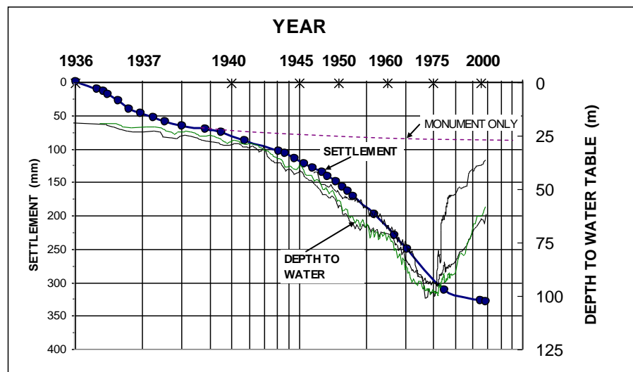
Fig. 3.8 Observed settlement of the San Jacinto Monument plotted together with the observed depths to water in wells near the Monument. (Data from Fellenius and Ochoa 2009a).
