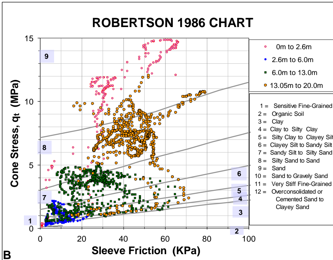
Fig. 2.17 A. Robertson 1986 profiling chart with axes in logarithmic scale B. Robertson 1986 profiling chart with axes in linear scale
