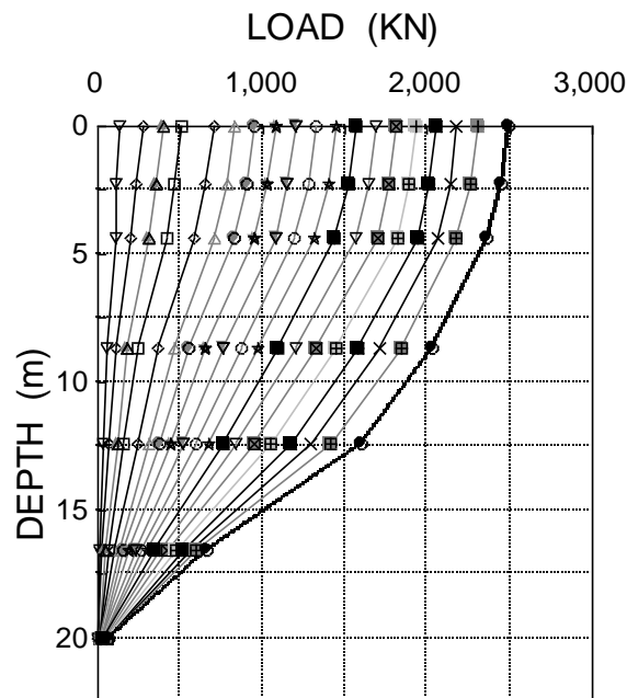
Fig. 8.48 Load distribution for each load applied to the pile head
