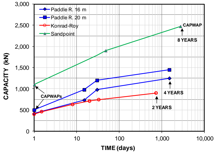
Fig. 7.41 Capacity determined at days after driving
