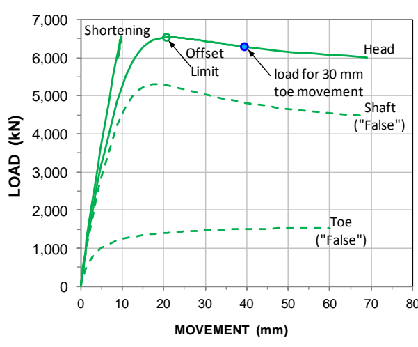
Fig. 8.18 Pile with residual load
