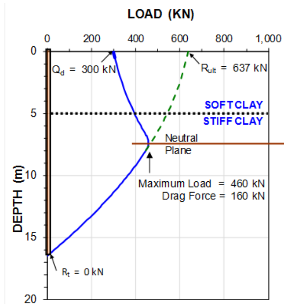
Fig. 10.4A Load distribution
