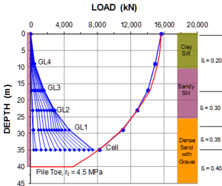
Fig. 8.27 Measured load distributions and the equivalent head-down load-distributions for the last increment of load ( r_t = toe resistance)
