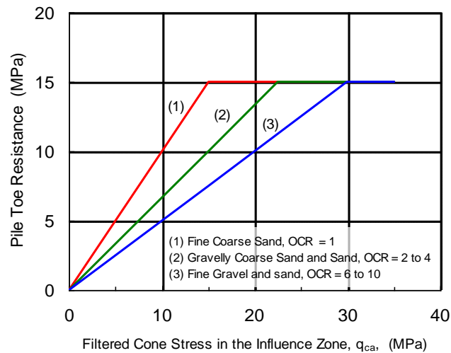
Fig. 7.10 Adjustment of unit toe resistance to OCR
