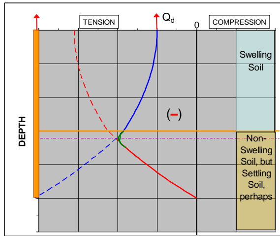
Fig. 7.25 Load distribution for a pile in swelling soil underlain by a settling soil
