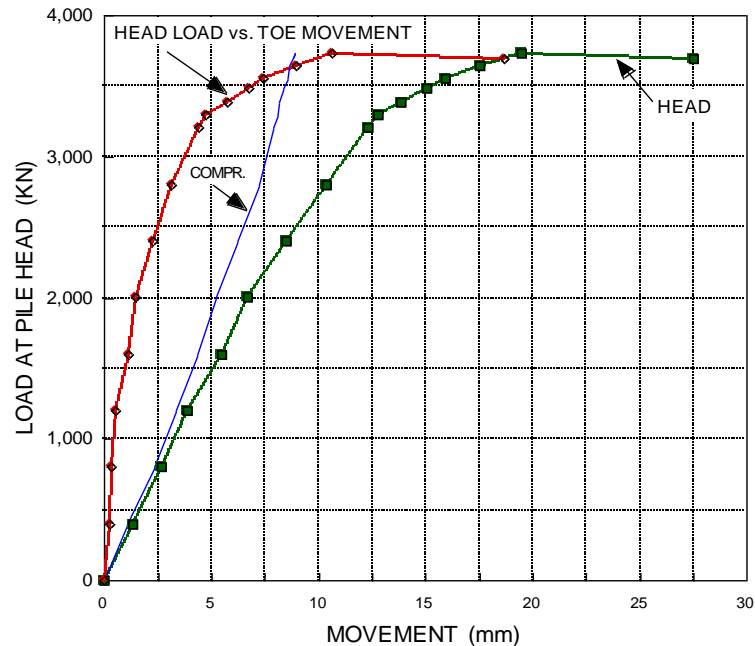
Fig. 8.8 Load-movement diagram of a static loading test on a 20 m long, 450 mm diameter closed-toe pipe pile in compact sand with telltale measurements of toe movement (Fellenius 1999)
