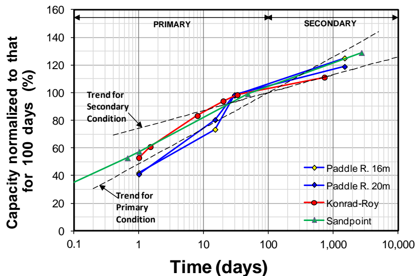
Fig. 7.42 Capacities normalized to 100 % of 100-day values
