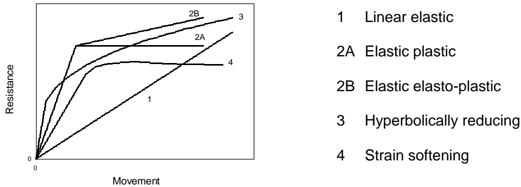
Fig. 8.10 Typical resistance versus movement curves
