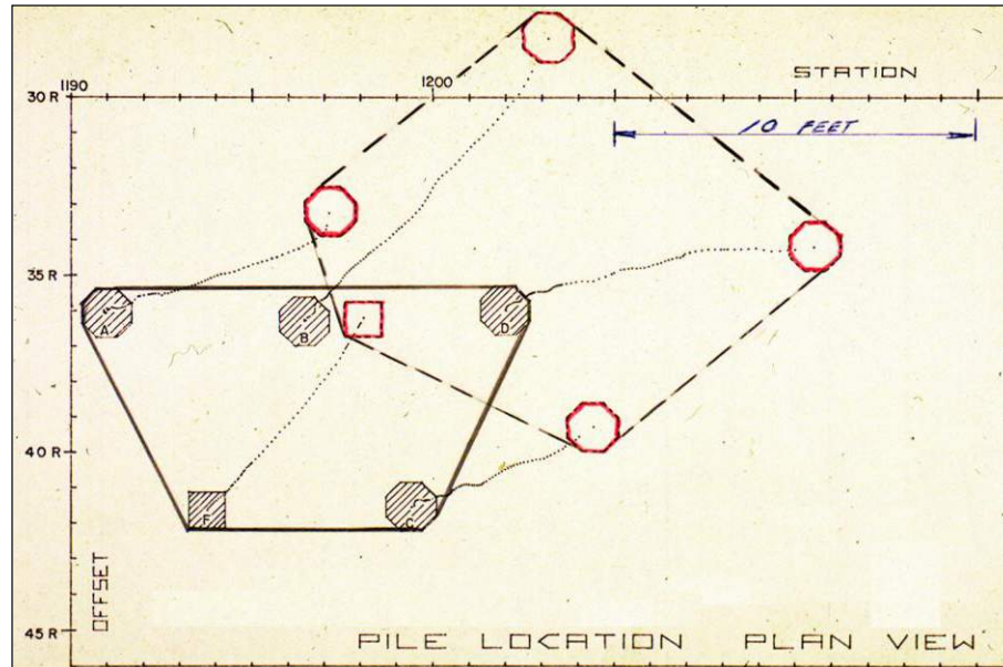
Fig. 7.38 Example of deviations determined by inclinometer measurements in 60 m long prestressed piles.
