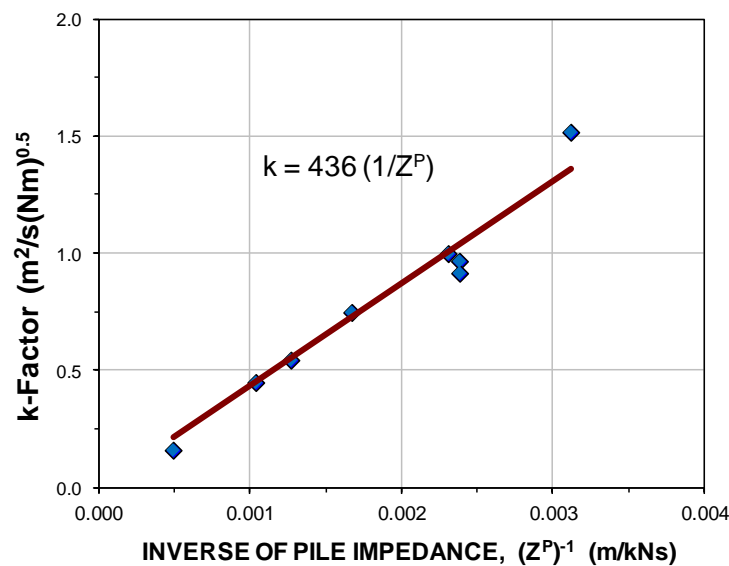
Fig. 9.25 Relationship between k -factor and inverse of pile impedance. Data from Figure 9.23 replotted.
