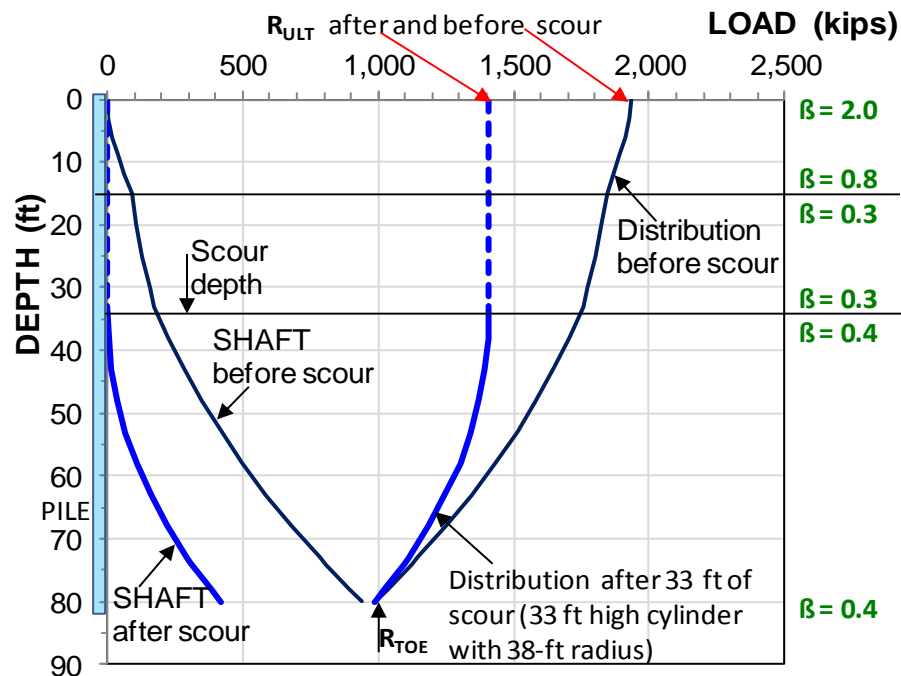
Figure 7.44. Load distributions at "capacity" before and after-scour
