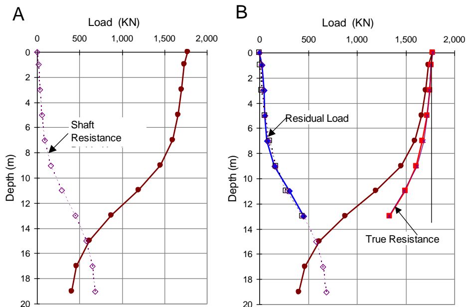
Fig. 8.36 Procedure for determining the distribution of residual load and “true” resistance
