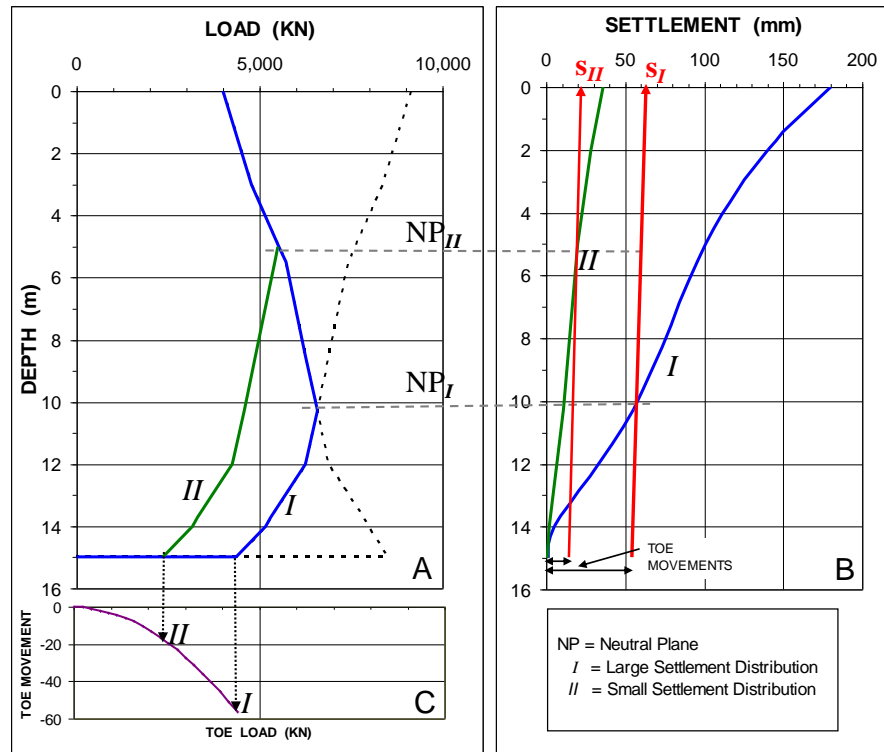
Fig. 7.18 Example of a pile with load and resistance curves determined from a static loading test and subjected to two alternative distributions of settlement (I and II).
