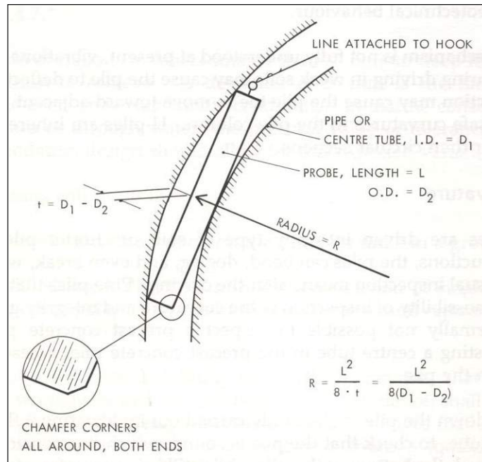
Fig. 7.39 Principle of the curvature probe
