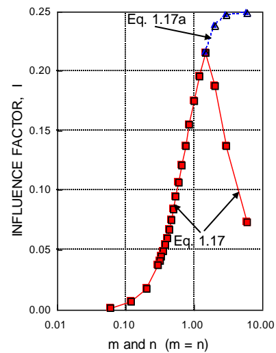
Fig. 1.7. Influence factor
