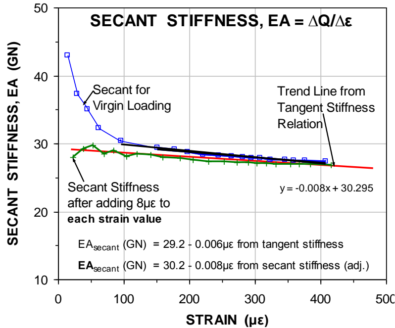
Fig. 8.42 Secant stiffness vs. measured strain for a 900-mm bored pile (Fellenius 2012)
