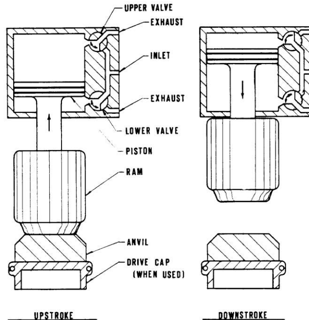
Fig. 9.4 The double-acting air/steam hammer (DFI 1979)
