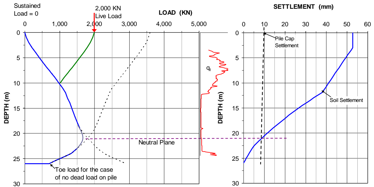
Fig. 8.32 The effect of adding a large live load to a pile with zero dead load.
