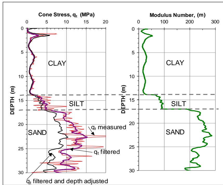
Fig. 3.11 Example of filtered and depth-adjusted q_t and profile of the resulting modulus number, m
