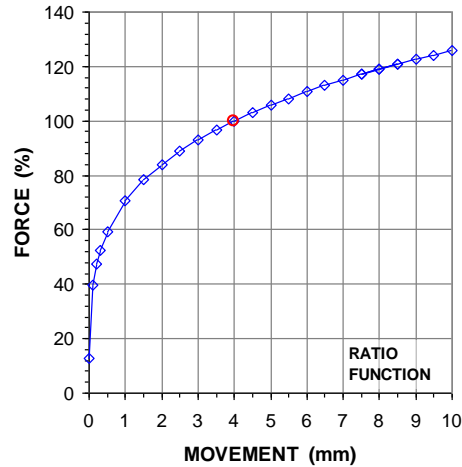
Fig. 8.12 Ratio Function for t-z shaft shear force vs. movement
