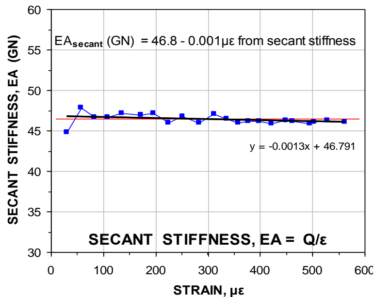
Fig. 8.39 Secant stiffness vs. measured strain for a not-concreted steel pipe pile (Fellenius 2012)
