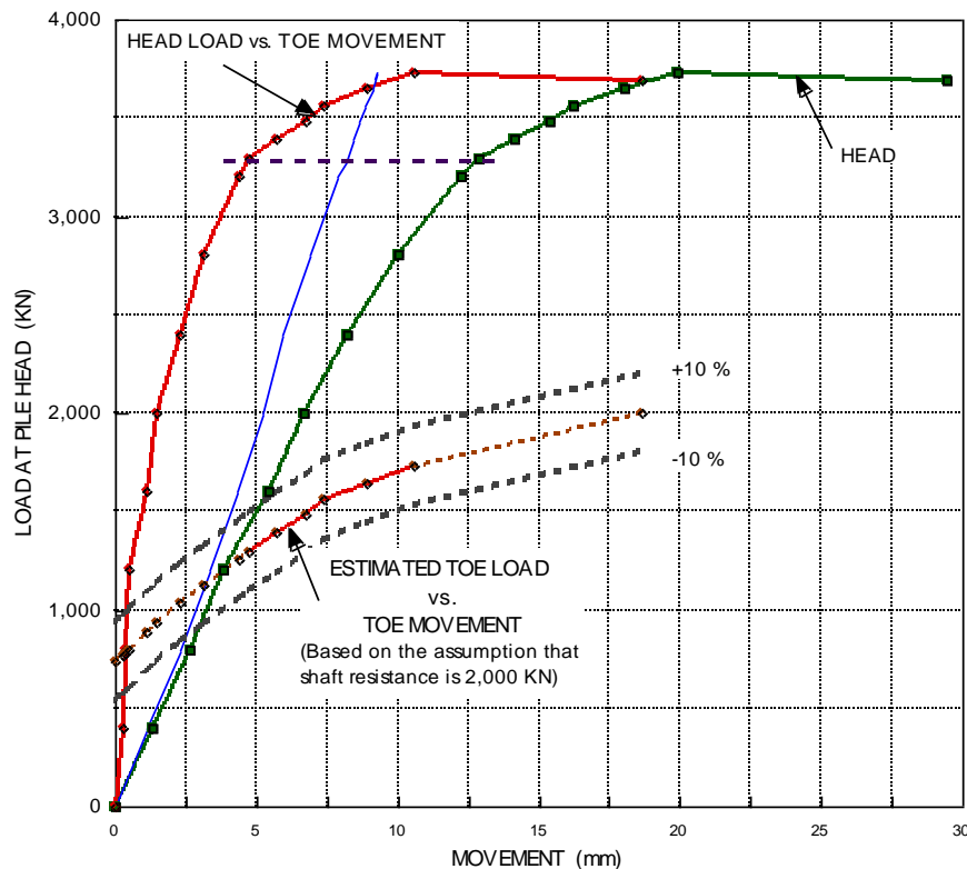
Fig. 8.9 The same test data shown in Fig. 8.8 with the results of analysis of the load-movement of the pile toe, making reference to the results from a static loading test on an adjacent pile instrumented with strain gages indicating a shaft resistance of 2,000 kN (Fellenius 1999)
