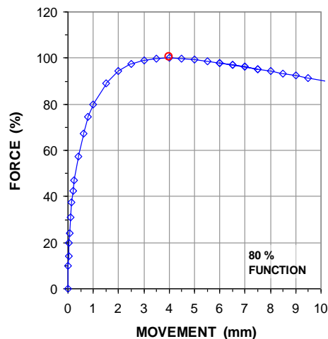
Fig. 8.15 80-% function for t-z shaft shear force vs. movement
