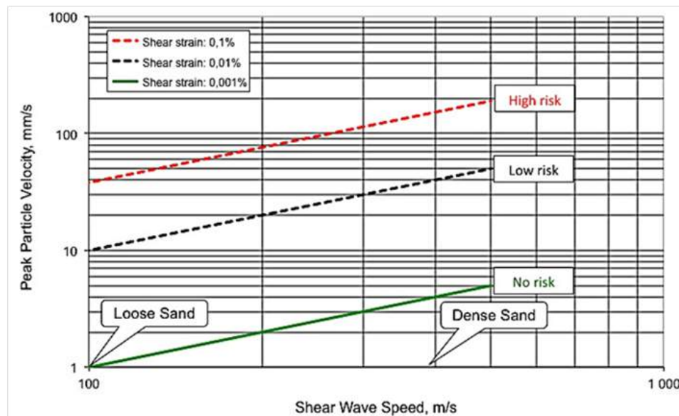
Fig. 9.26 Assessment of settlement risk in sand as function of amplitudes of shear-wave speed, shear strain, and vibration velocity (Massarsch 2008)
