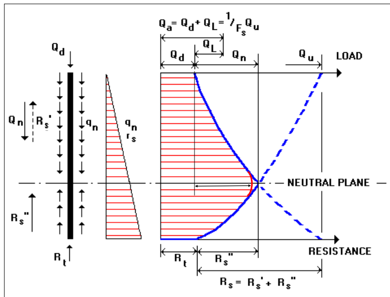
Fig. 7.22 Construing the Neutral Plane and Determining the Allowable Load
