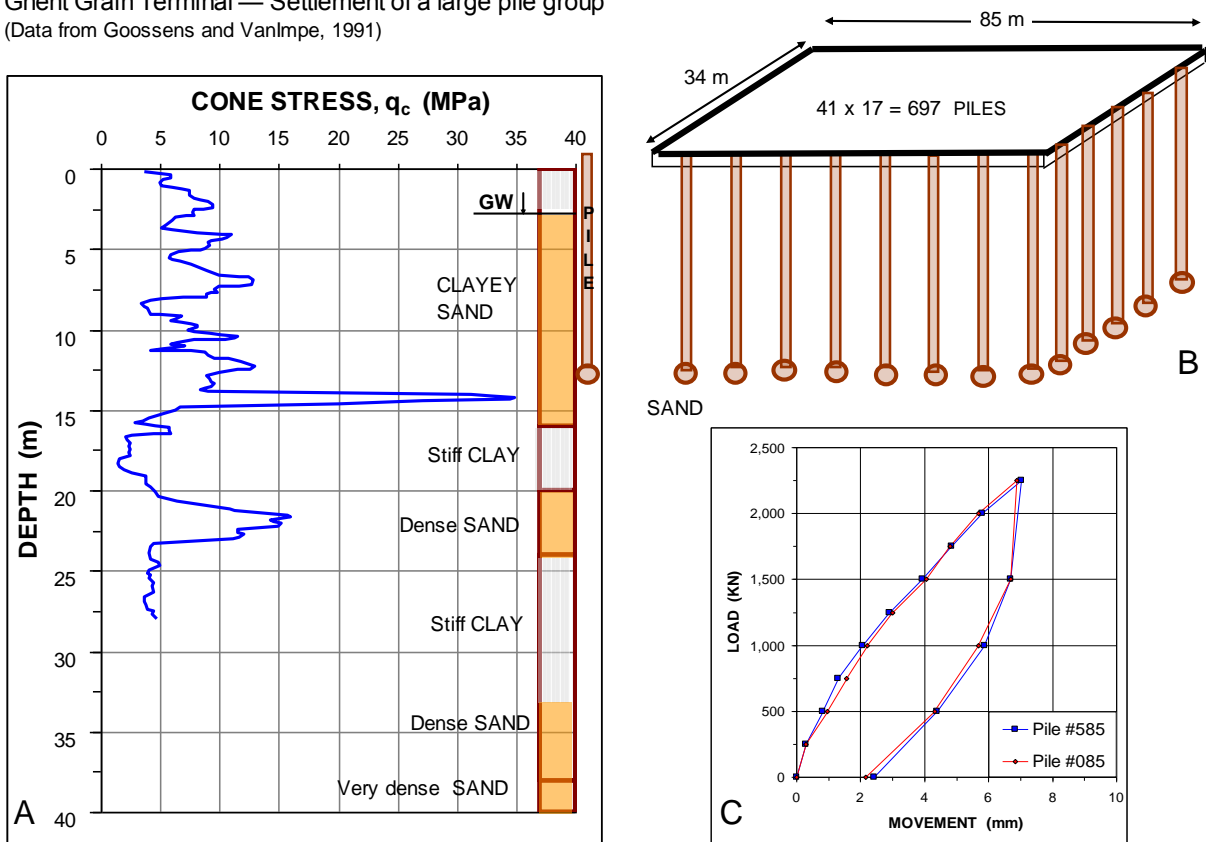
Fig. 7.31 Soil profile (A), pile group (B), and load-movement (C) in two static loading tests
