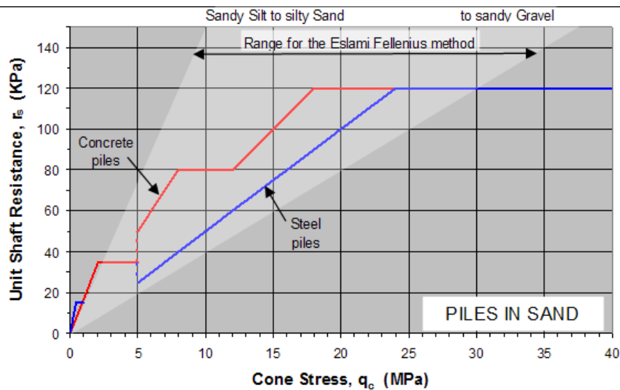
Fig. 7.14 Unit Shaft resistance versus cone stress, q_c , for piles in sand according to the LCPC method (the red and blue lines) and the Eslami-Fellenius method
