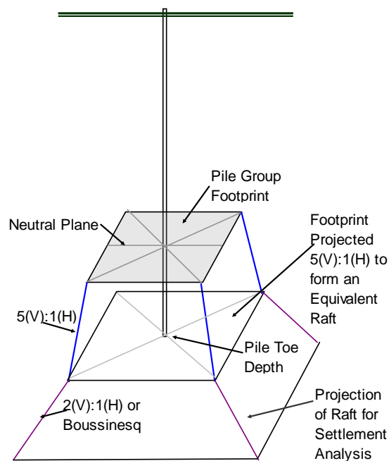
Fig. 7.19 Distribution of stress below the neutral plane for a group of piles. Only one pile is shown.
