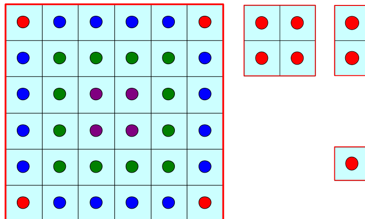
Fig. 7.26 Configuration of the pile groups
