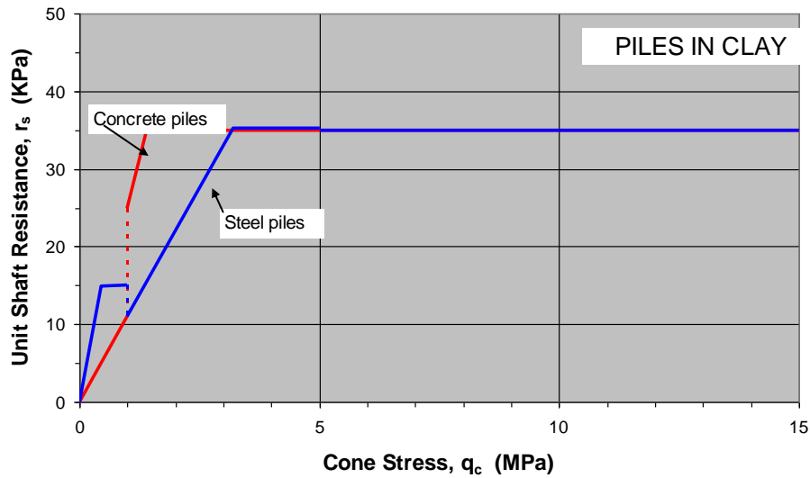
Fig. 7.13A Unit shaft resistance versus cone stress, q_c , for piles in clay according to the LCPC method.
