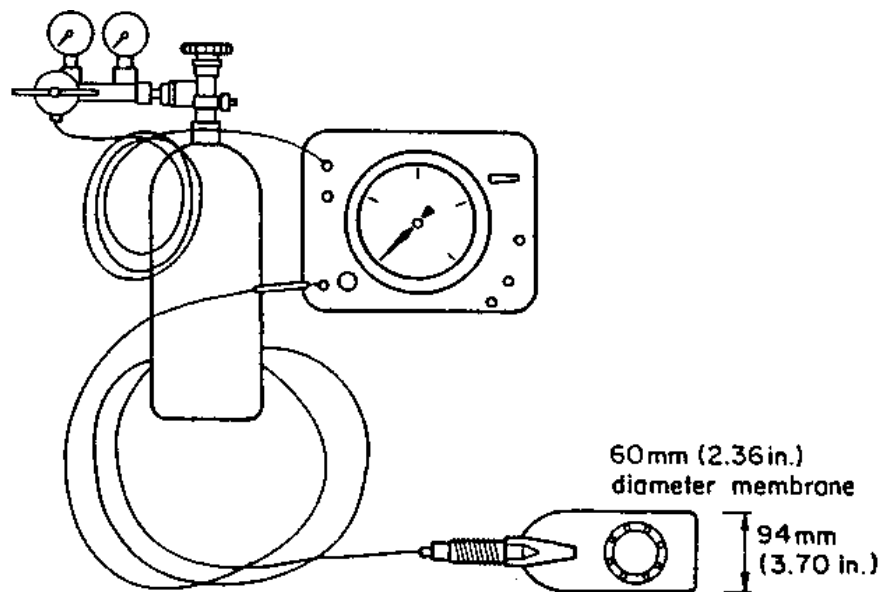
Figure 2-58.—Dilatometer test equipment. (Schmertman [65])
