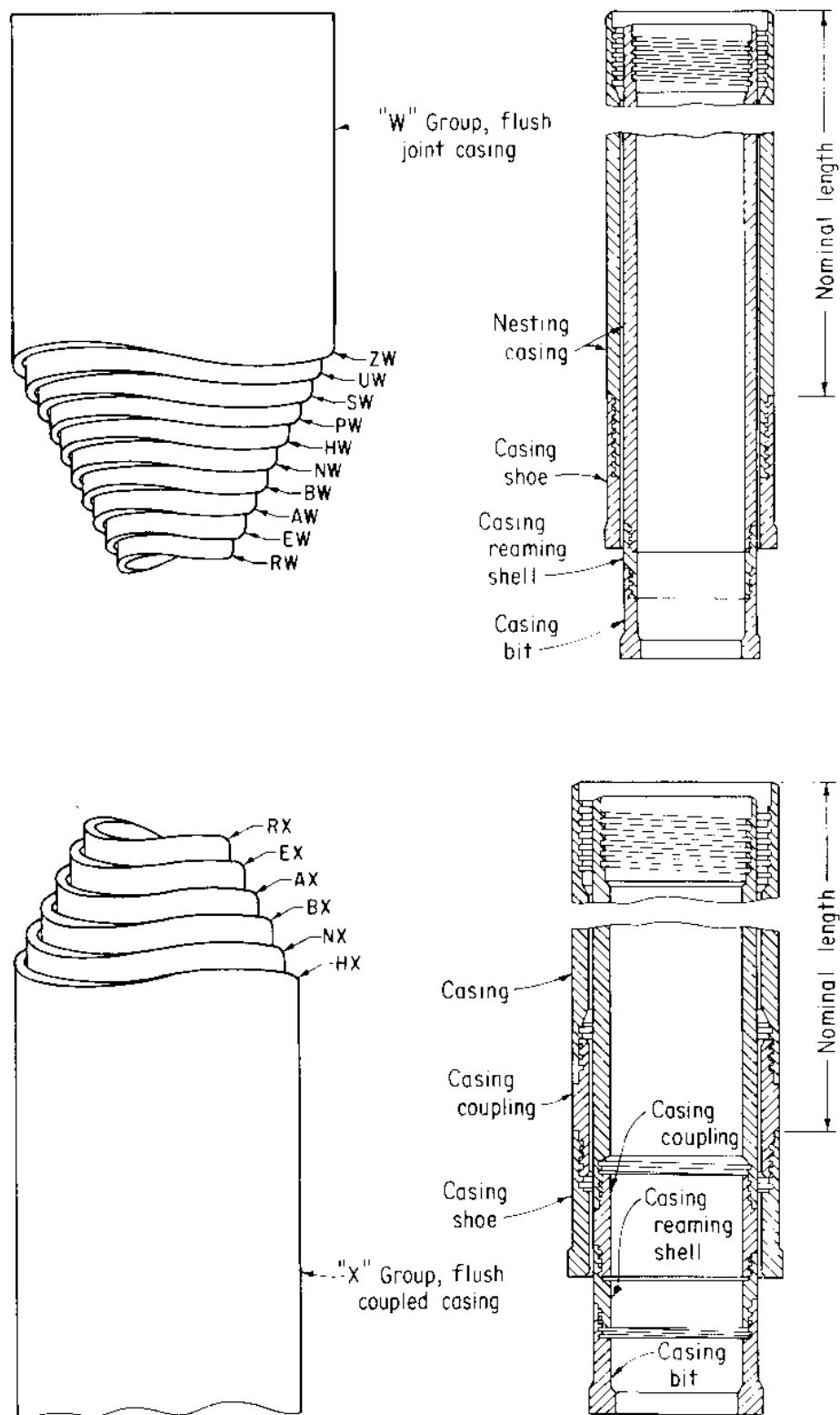
Figure 2-27. — Core drill casing.
