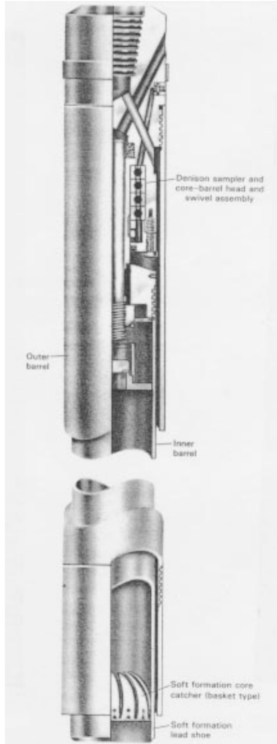
Figure 2-44.—Denison sampler and core barrel.
