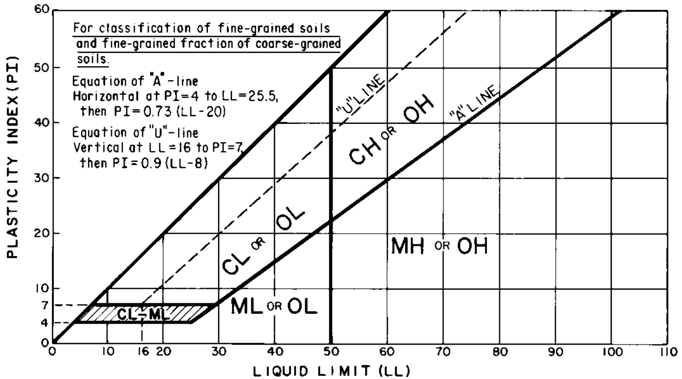
Figure 1-7.—Plasticity chart.
