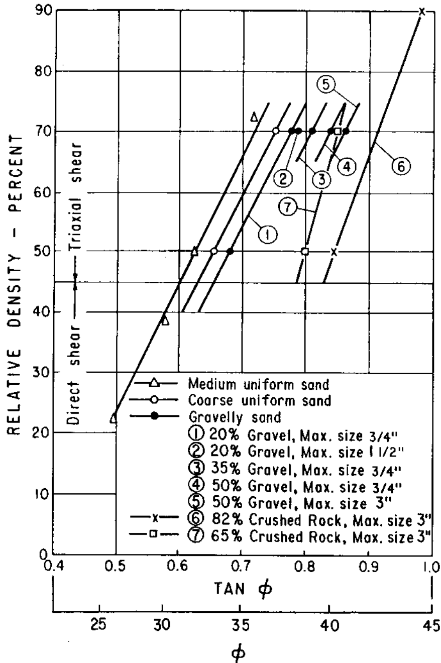
Figure 1-17.—Effect of relative density on the coefficient of friction, \tan \phi , for coarse-grained soils [24, 28].
