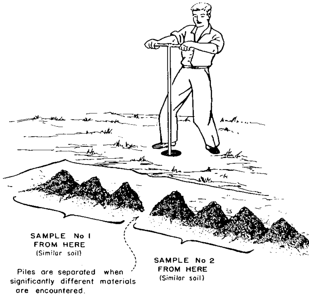
Figure 2-36.—Auger sampling.
