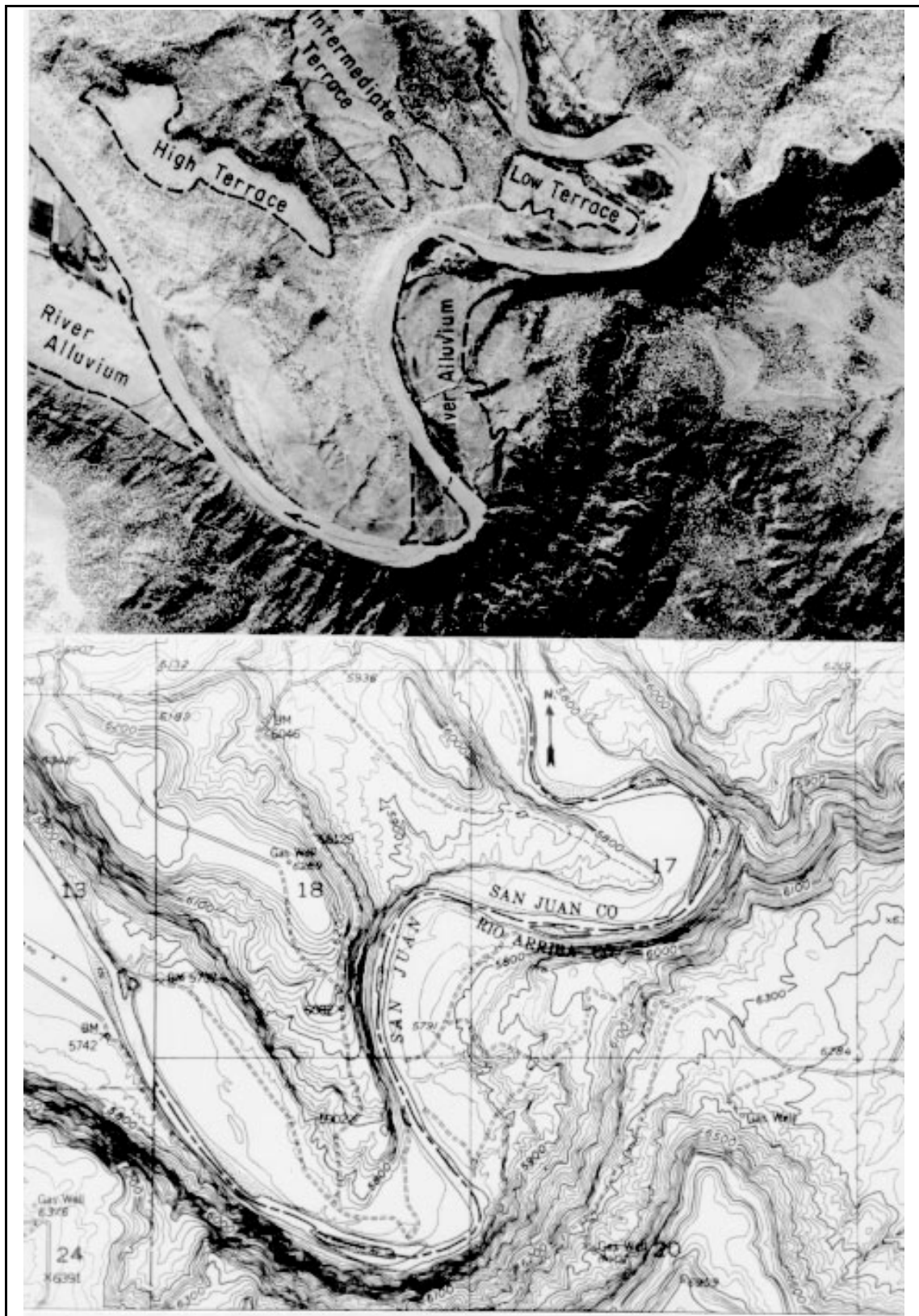
Figure 2-4.—Aerial view and topography of stream deposit showing river alluvium and three levels of gravel terraces. (U.S. Geological Survey)
