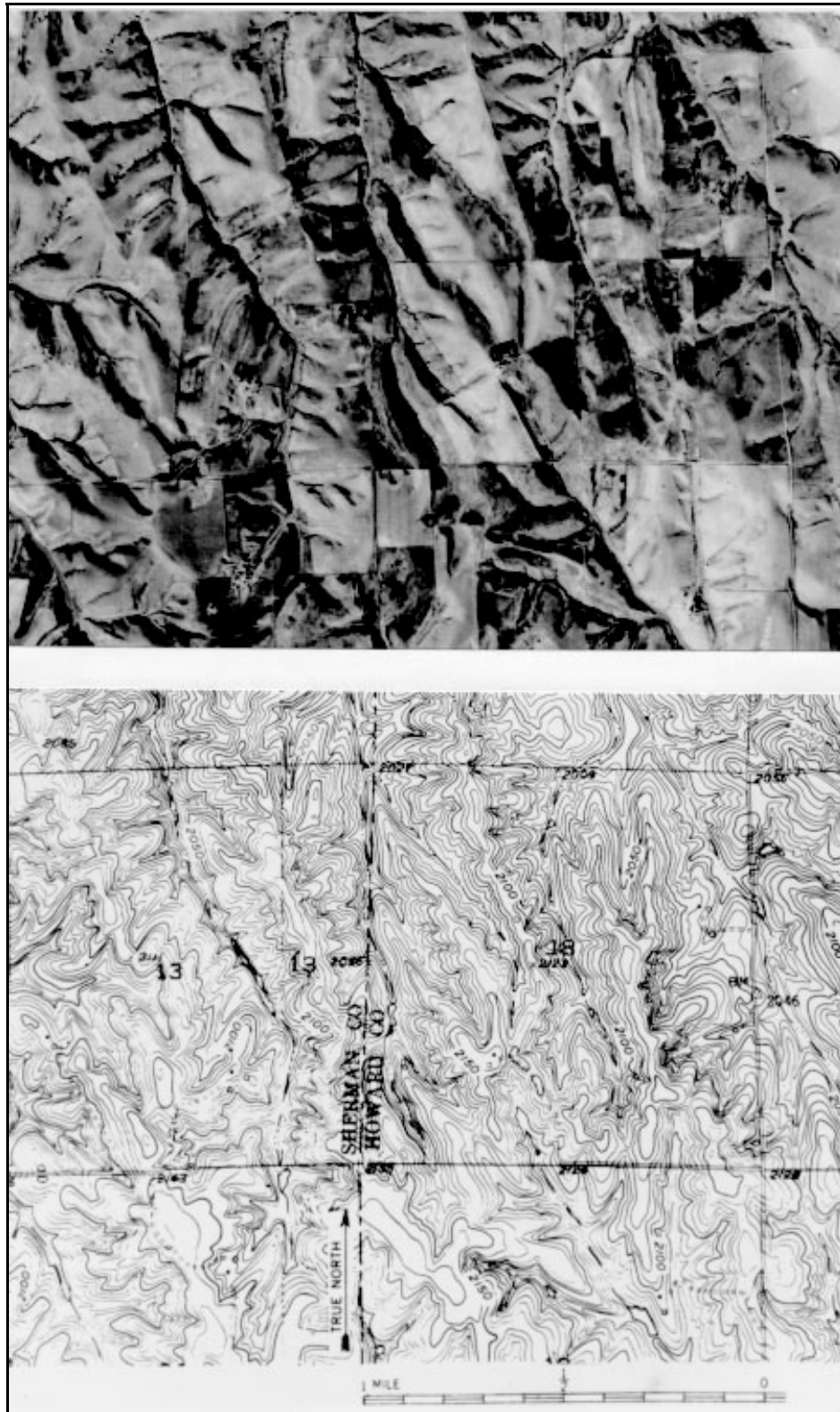
Figure 2-7.—Aerial view and topography of loess identified by smooth silt ridges; usually parallel, right-angle drainage patterns; and steep-sided, flat-bottomed gullies and streams. (Natural Resources Conservation Service)
