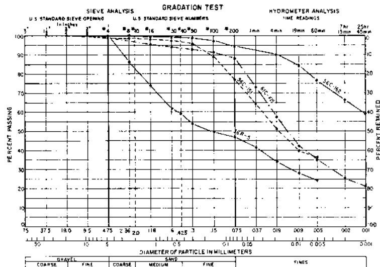
A. GRADATION CURVES
