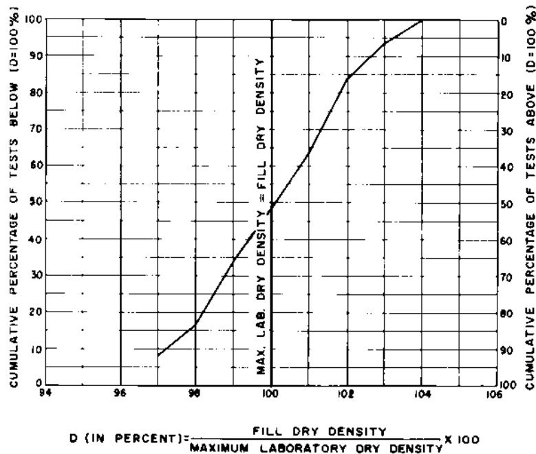
Figure 3-30.—Statistical analysis of test results for density control of fill.
