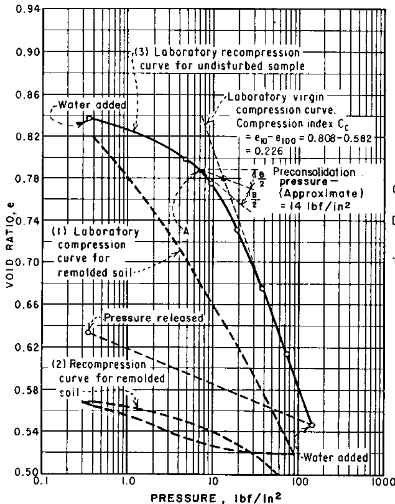
(B) VOID RATIO - PRESSURE CURVES AND PRECONSOLIDATION PRESSURE
