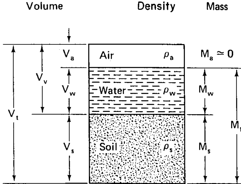
Figure 1-9.—Relationship between air, water, and solids in a soil mass.
