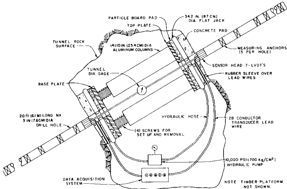
Figure 2-65.—Uniaxial jacking test.
