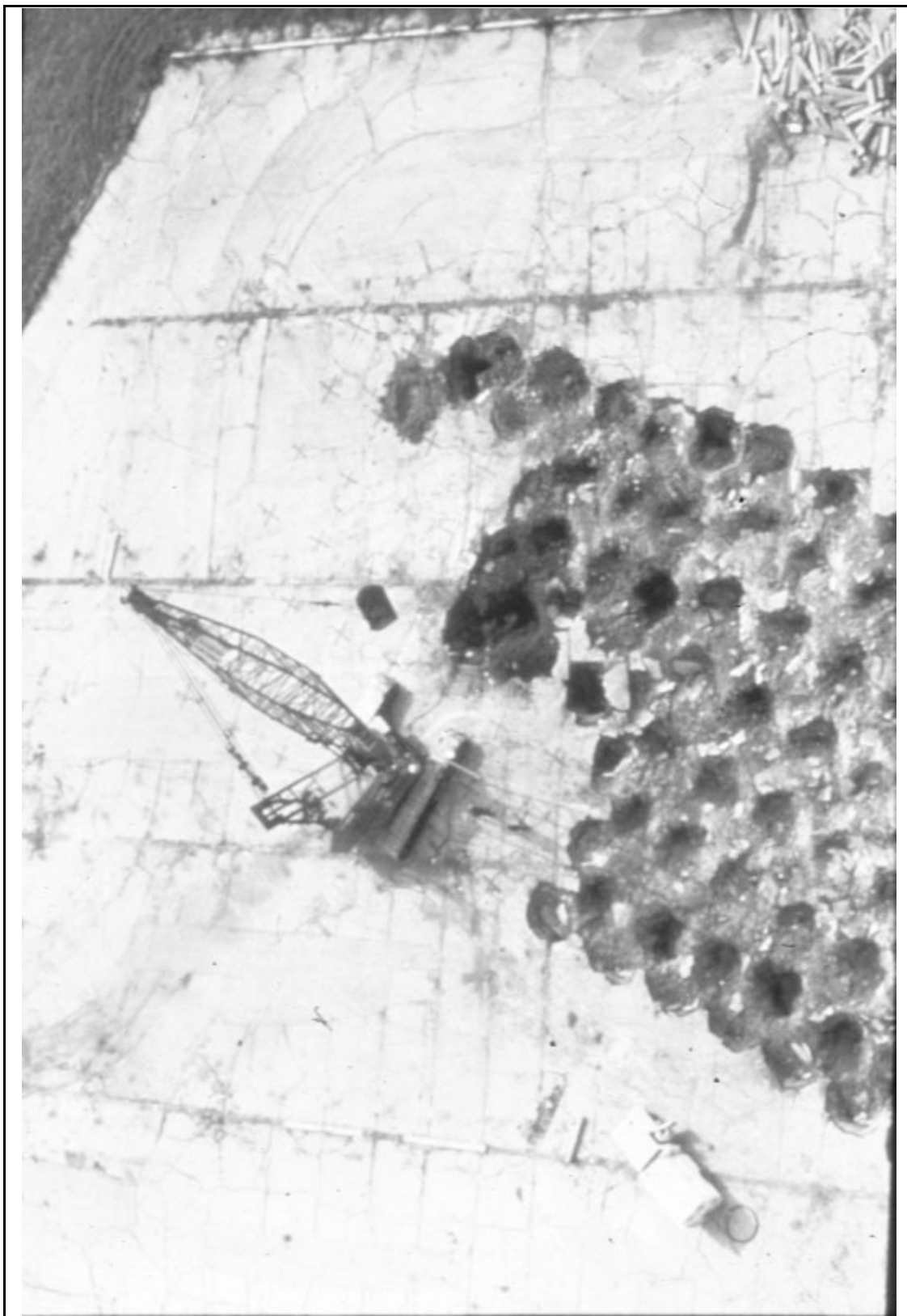
Figure 3-12.—Photograph of dynamic compaction showing crane, weight, and impact pattern (Hayward Baker, Inc.)
