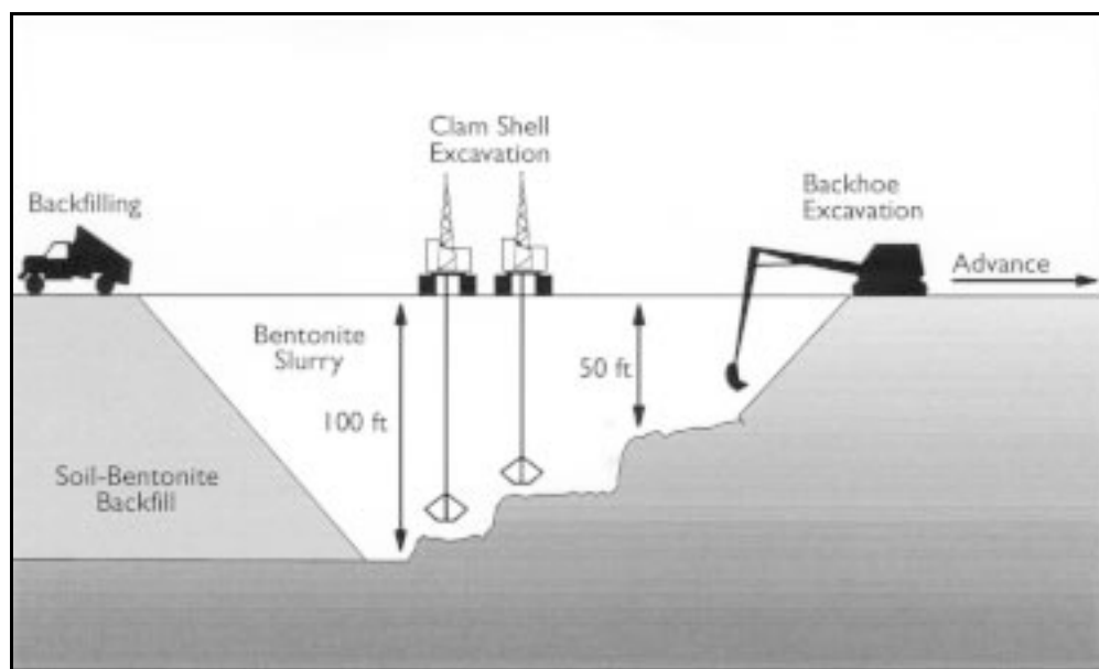
Figure 3-10.—Schematic drawing showing slurry wall construction methods—backhoe and clamshell excavation and surface backfill method. (Hayward Baker, Inc.)
