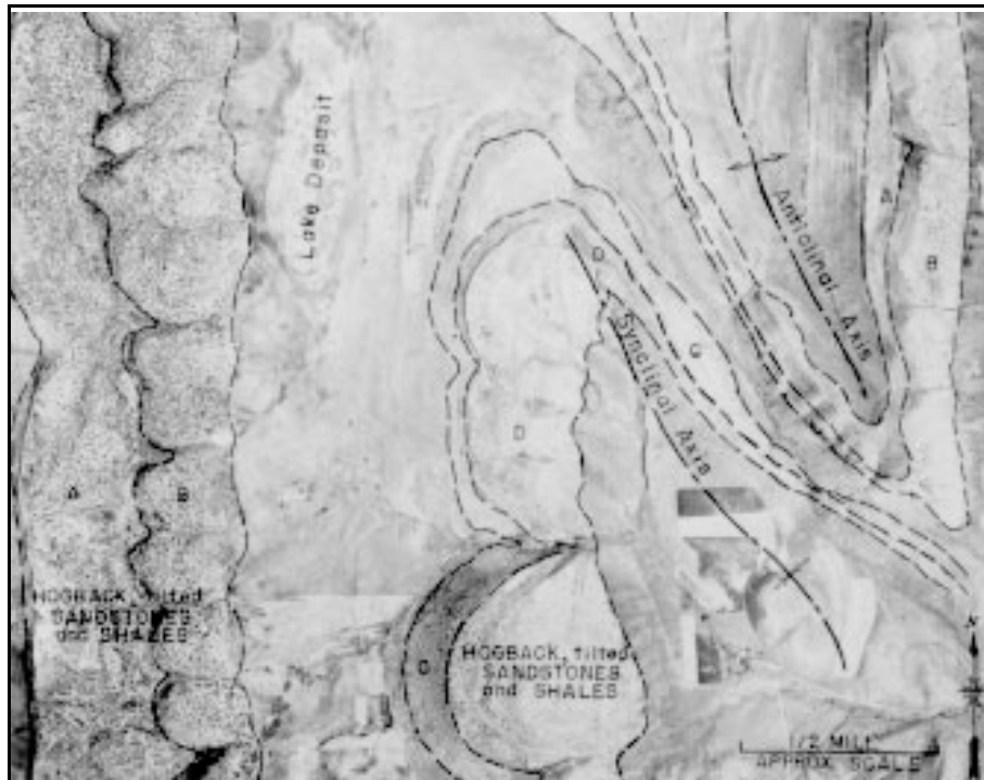
Figure 2-2.—Rock strata illustrating folding in sedimentary rocks. (A) Satanka formation, (B) Lyons formation, (C) Morrison formation, and (D) Lower and Middle Dakota formation. (U.S. Forest Service)
