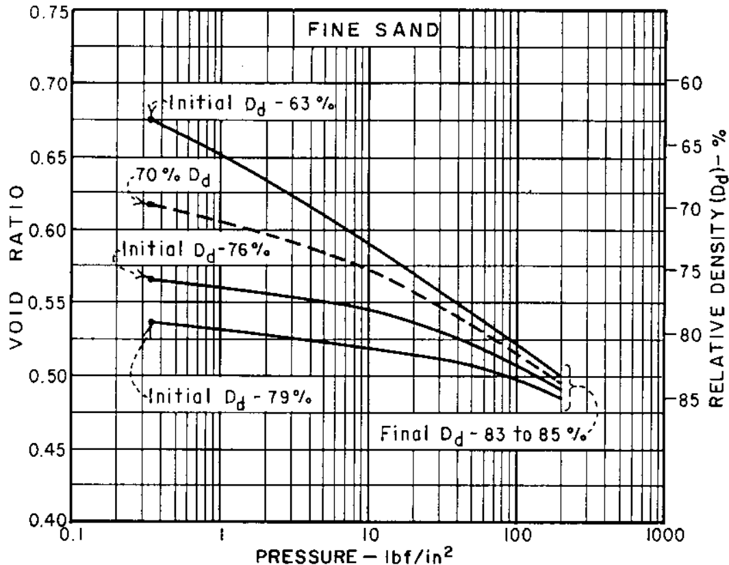
Figure 1-26.—Compressibility characteristics of a fine sand in relation to placement relative density [37].
