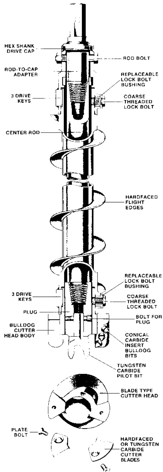
Figure 2-23.—Hollow-stem auger with center plug.
