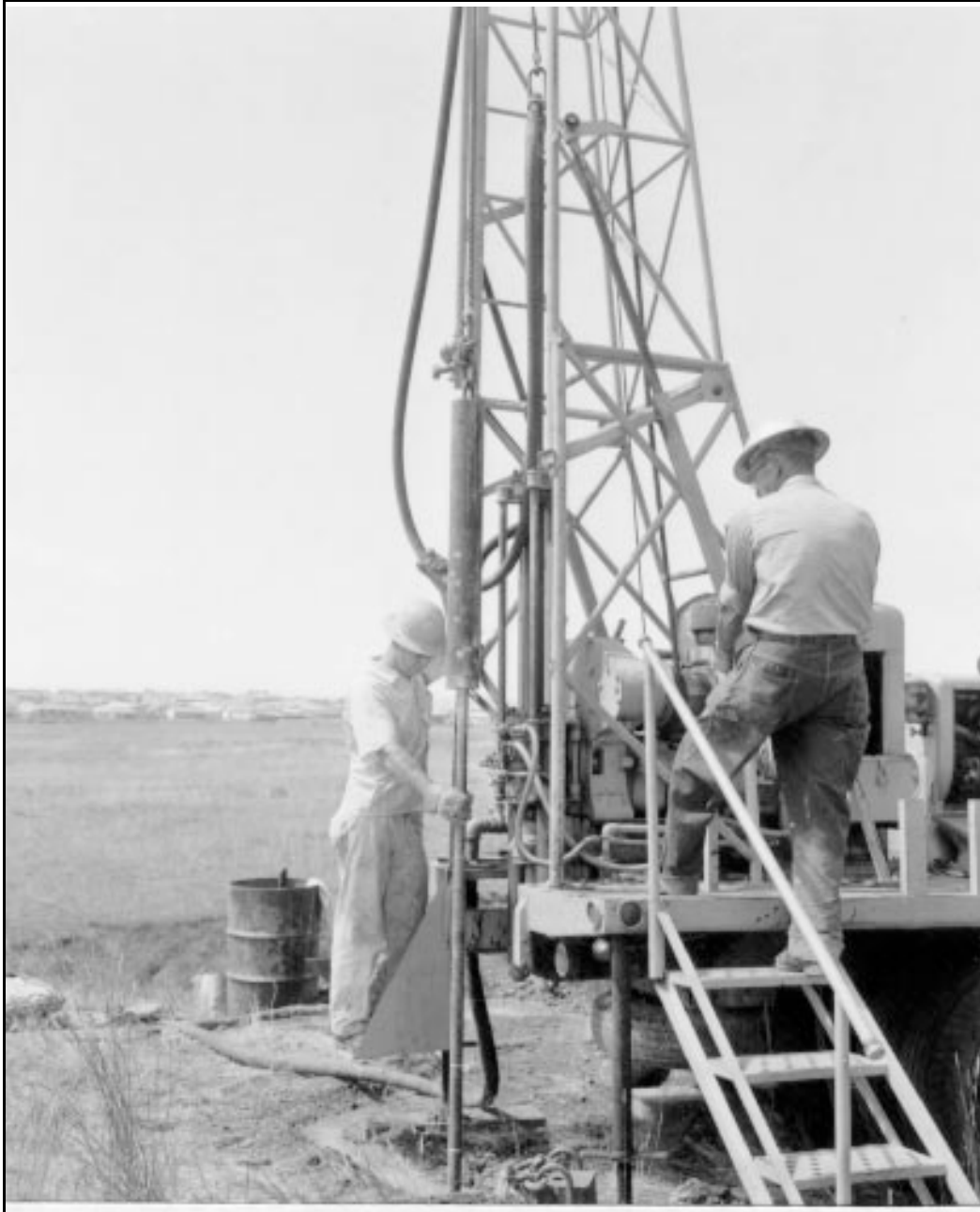
Figure 2-51.—Standard drilling equipment used to perform penetration tests.
