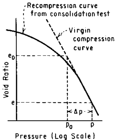
(A) METHOD OF DETERMINING THE COMPRESSION INDEX, C_c
