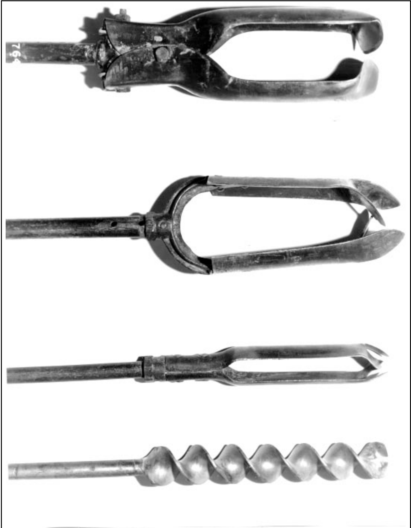
Figure 2-21.—Types of hand augers (2-inch helical, 2- and 6-inch Iwan, and 6-inch Fenn [adjustable]).
