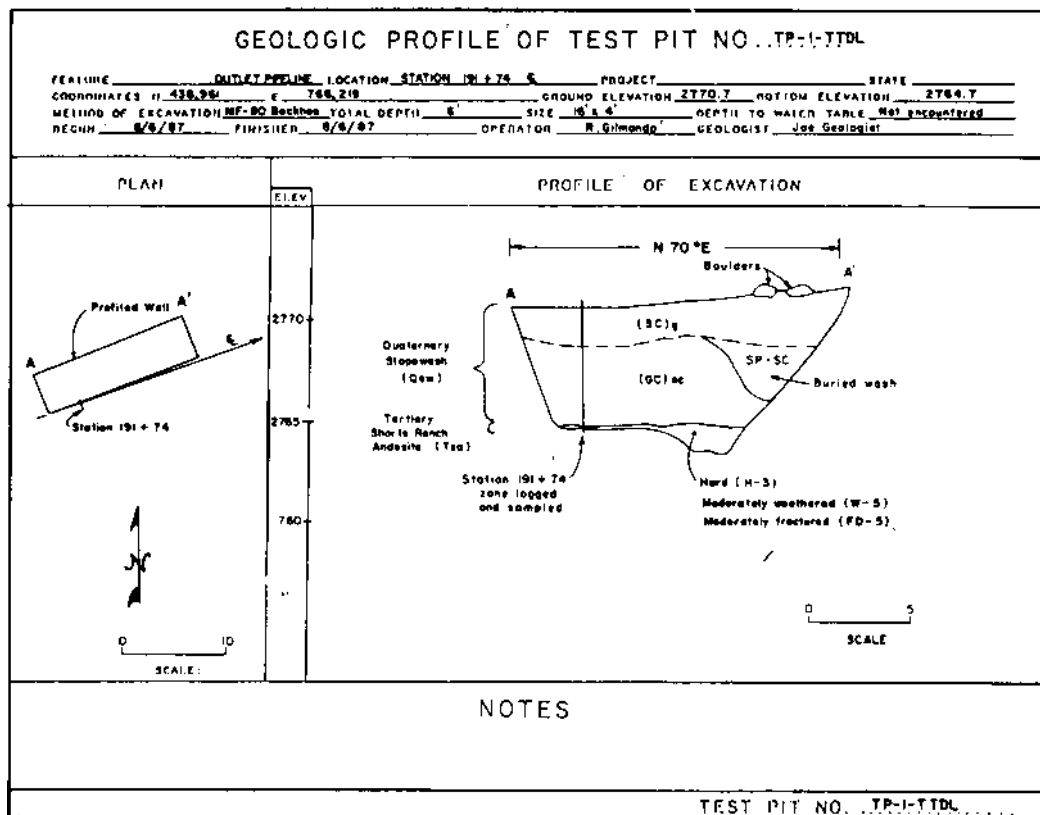
Figure 2-72.—Geologic interpretation in test pit (geologic profile).
