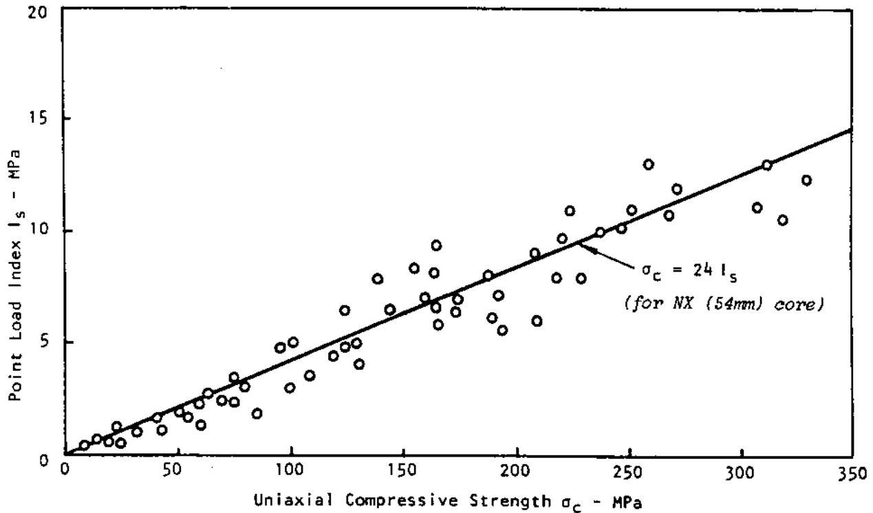
Figure 2-62.—Relationship between point-load strength index and uniaxial-compressive strength. 1\text{MPa} = 10.2\text{ kg/cm}^2 = 145\text{ lb/in}^2 .
