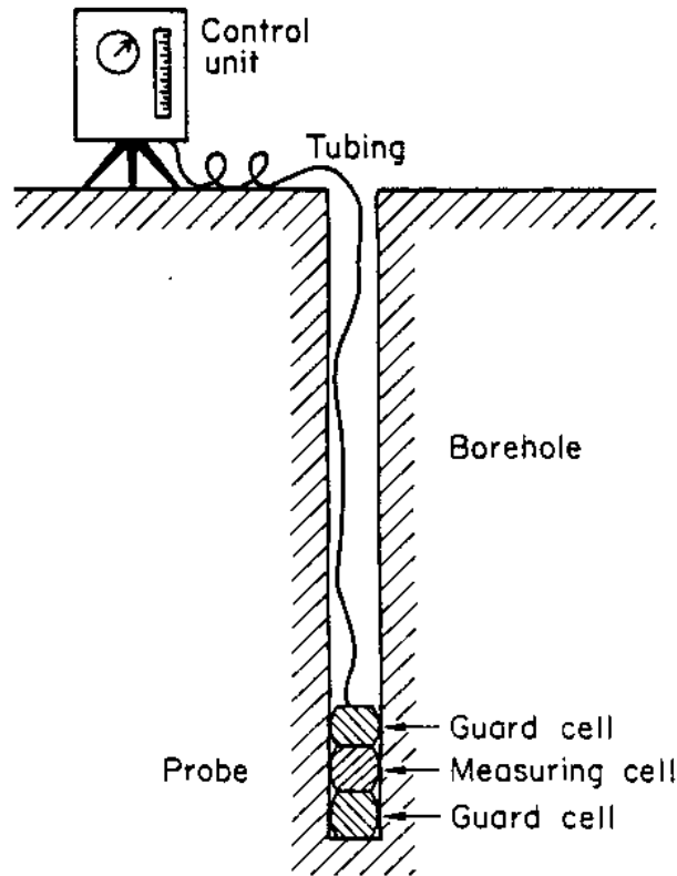
Figure 2-55.—Menard pressuremeter equipment. (Baguelin, Jézéquel, and Shields [58])
