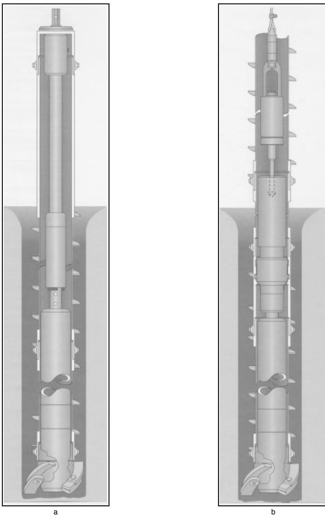
Figure 2-42.—Overshot wire-line a) and rod type b) continuous sampling system. (Mobile Drill Co.)
