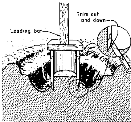
(A) Level area and drive cylindrical sampler slightly into soil. Carefully excavate trench around cylinder and trim to cutting bit with knife.
