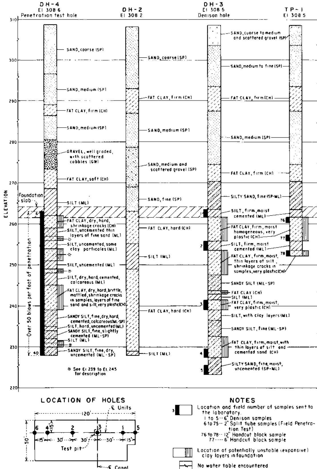
Figure 2-10.—Soil profile at a pumping plant.
