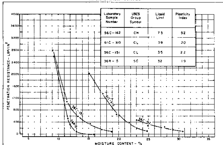
B. PENETRATION RESISTANCE CURVES
