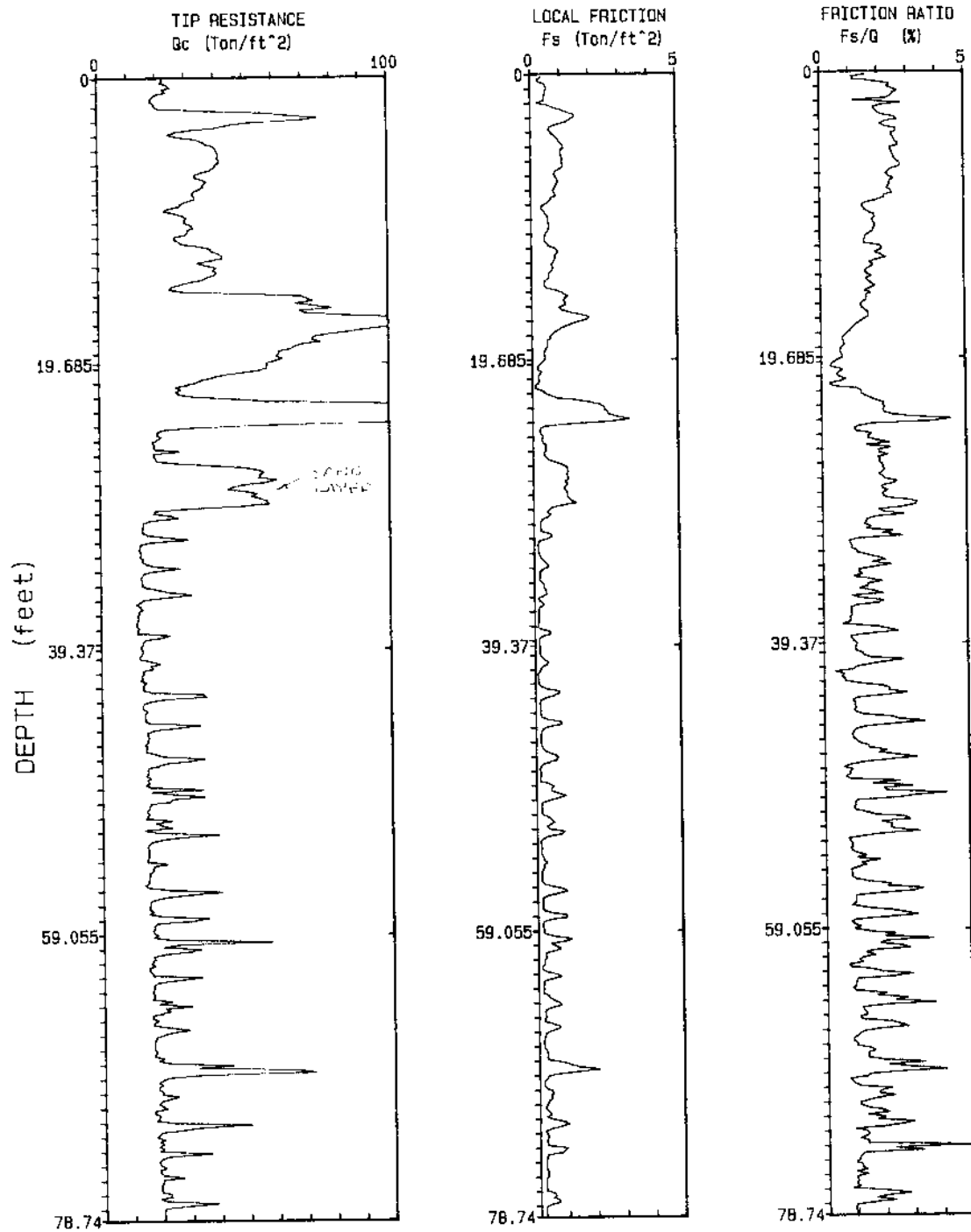
Figure 2-53.—Example of electronic cone penetrometer data.
