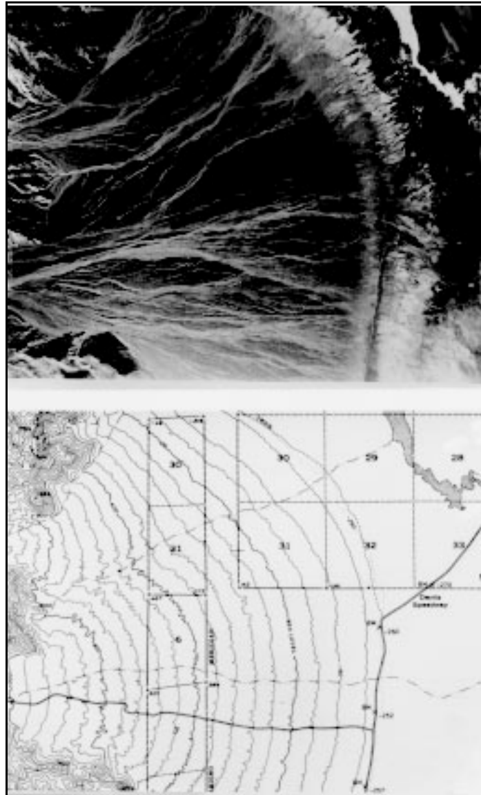
Figure 2-5.—Aerial view and topography of an alluvial fan, a potential source of sand and gravel. (U.S. Geological Survey)
