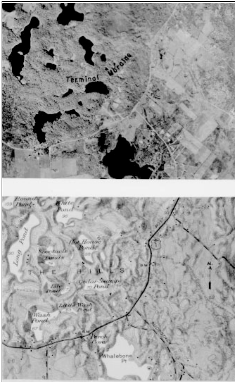
Figure 2-6.—Aerial view and topography of terminal moraine of continental glaciation. (Natural Resources Conservation Service)
