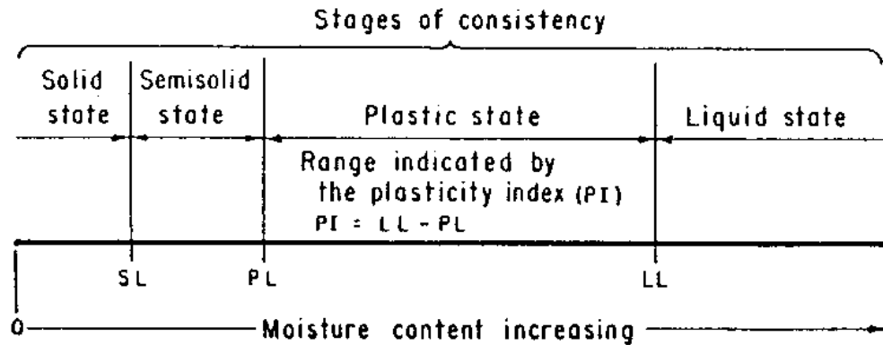
Figure 1-5.—Consistency limits.
