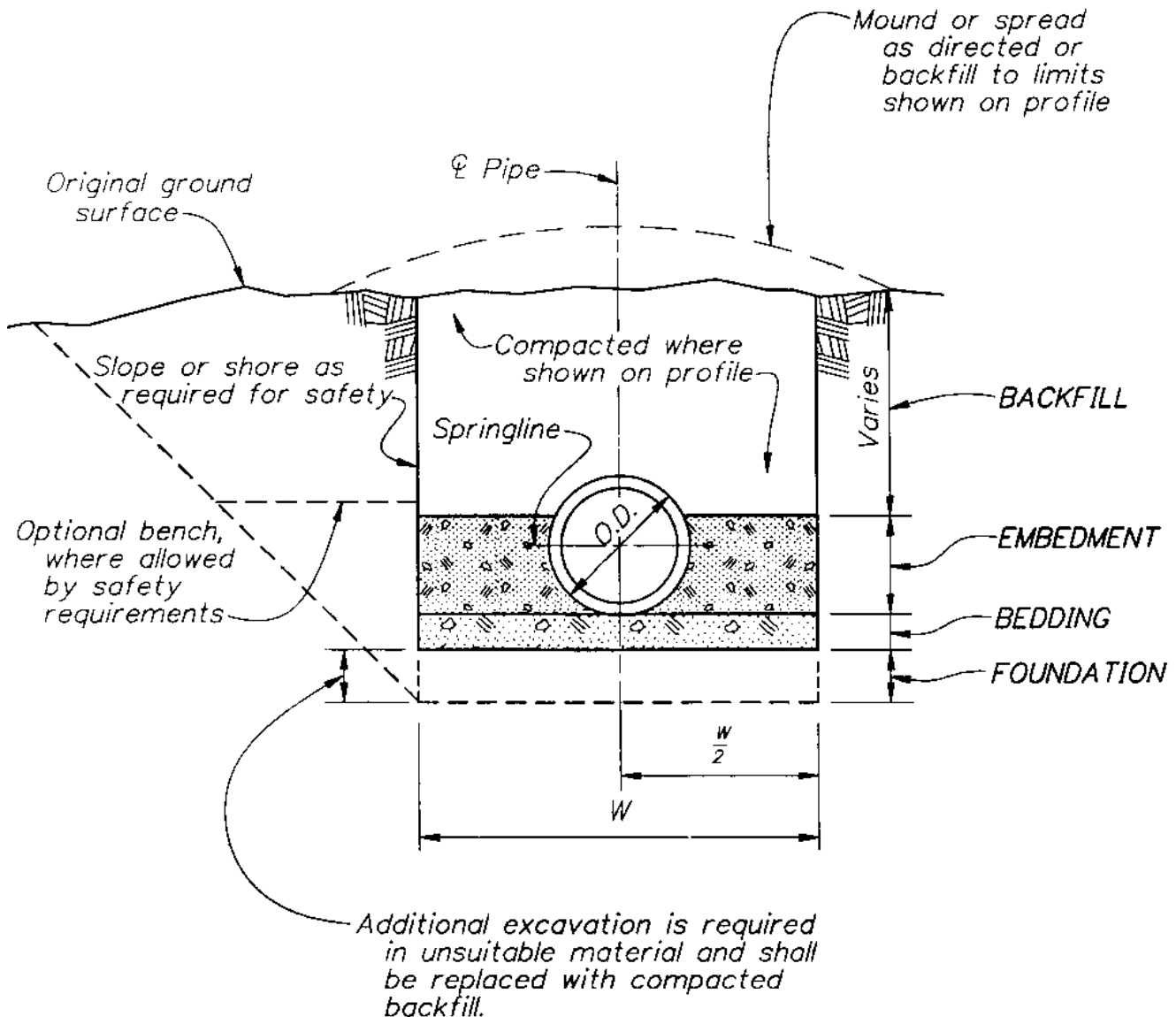
Figure 3-38.—Typical trench details.
