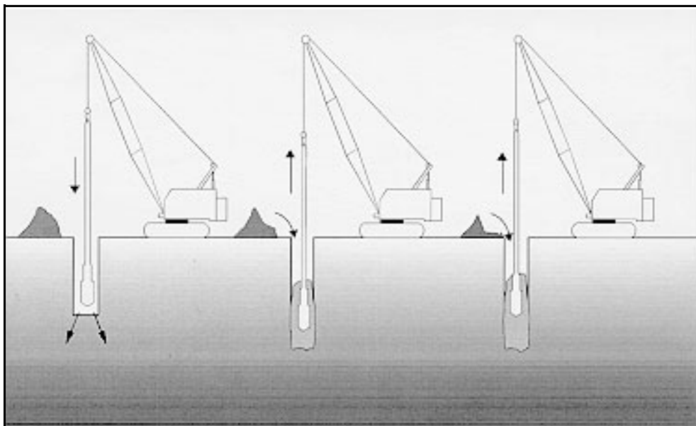
Figure 3-13.—Schematic drawing of vibro-replacement—backfill can be added by top feed (illustrated) or bottom feed methods. (Hayward Baker, Inc.)
