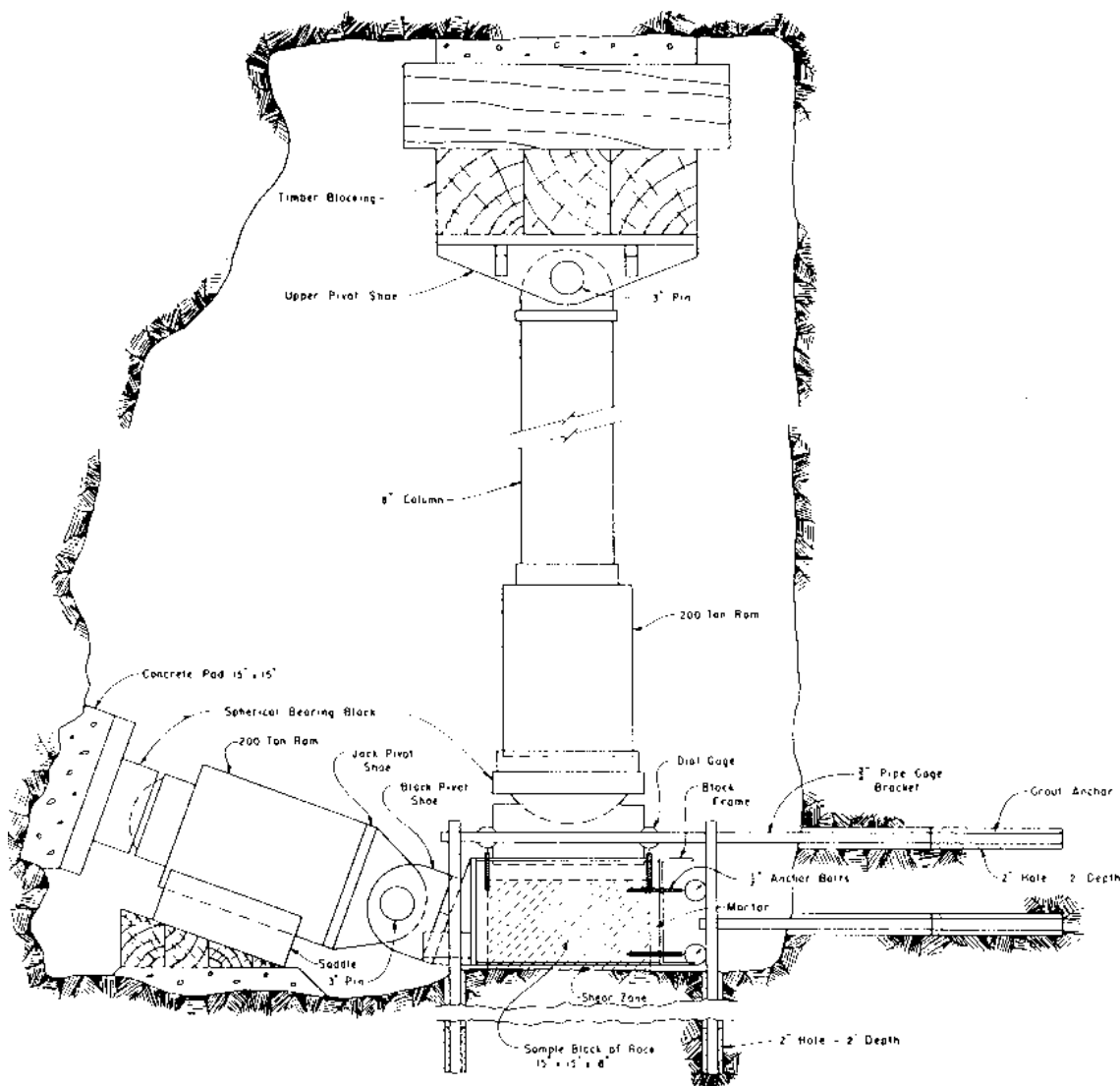
Figure 2-64.—Shear and sliding friction testing equipment, Auburn damsite.
