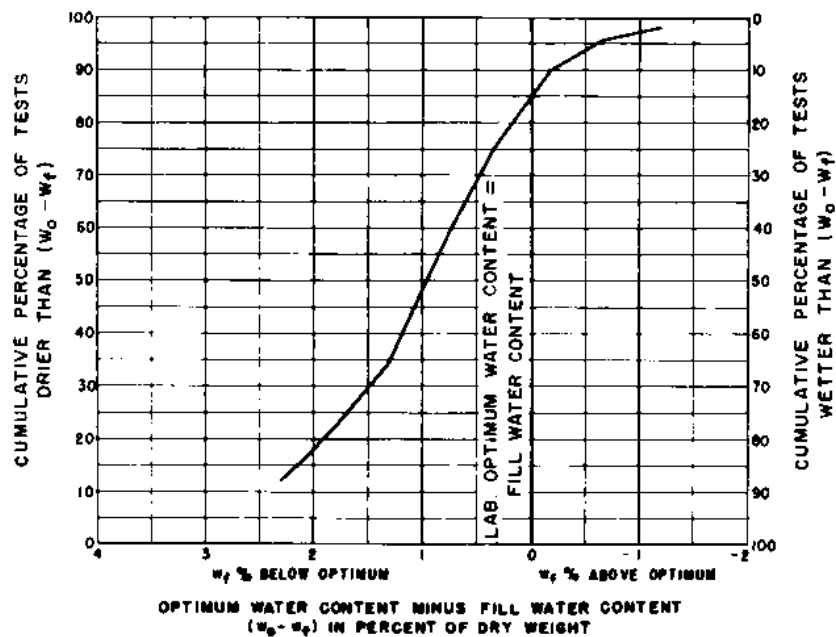
Figure 3-31.—Statistical analysis of test results for moisture control of fill.
