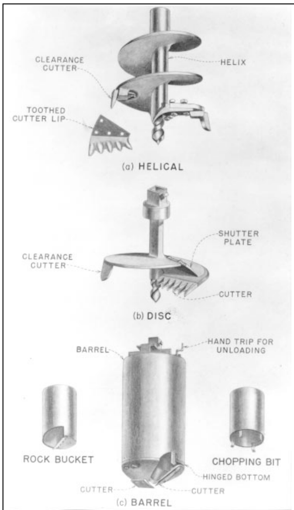
Figure 2-24.—Illustration of the helical, disc, and barrel types of machine-driven augers showing basic differences. (U.S. Department of the Navy)
