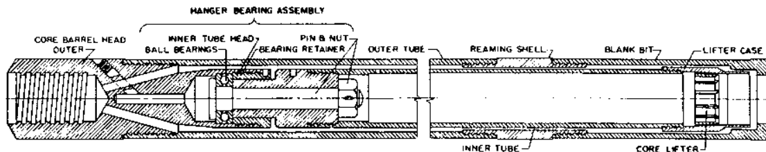
M-DESIGN, CORE LIFTER IN INNER BARREL
