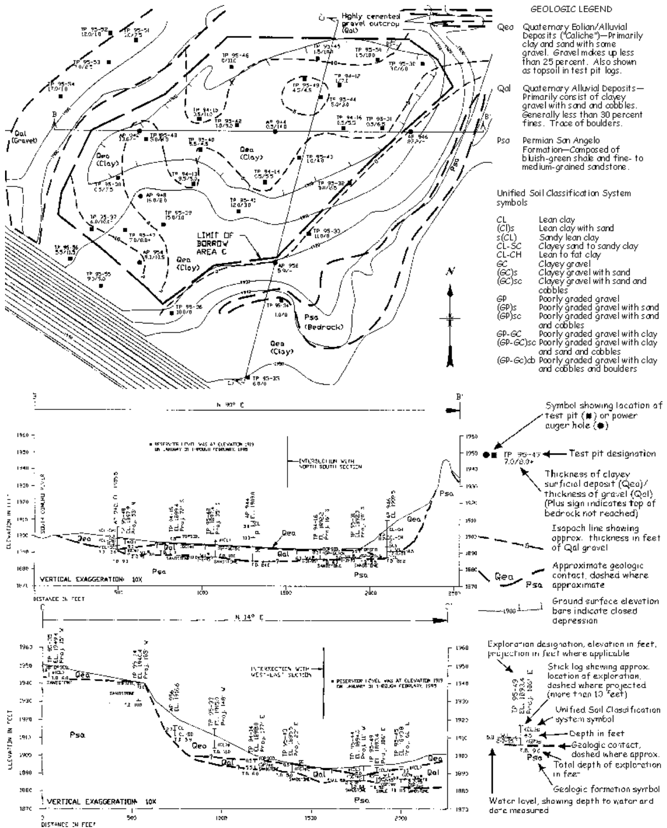
Figure 2-14.—Exploration for embankment materials—borrow area location map and typical cross sections.
