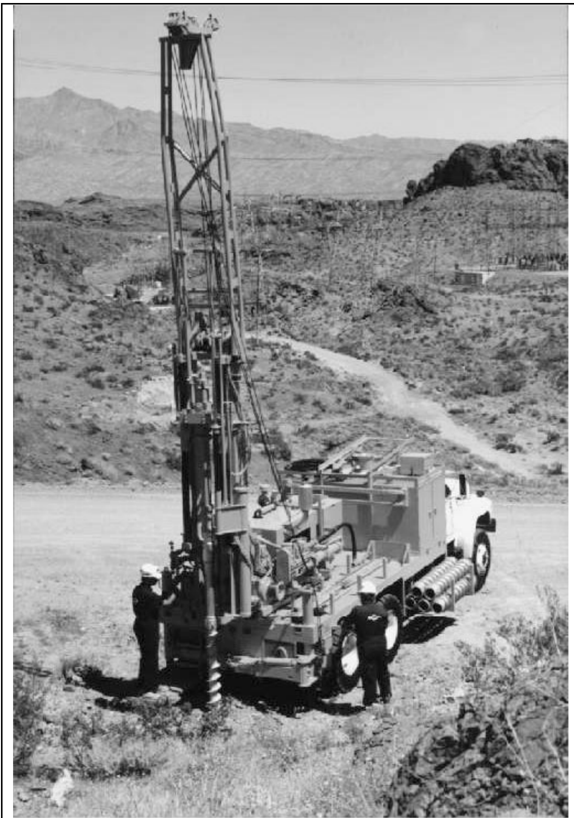
Figure 2-28.—Photograph of typical rotary drill showing some of the essential equipment for rotary drilling. (Central Mine Equipment Company)
