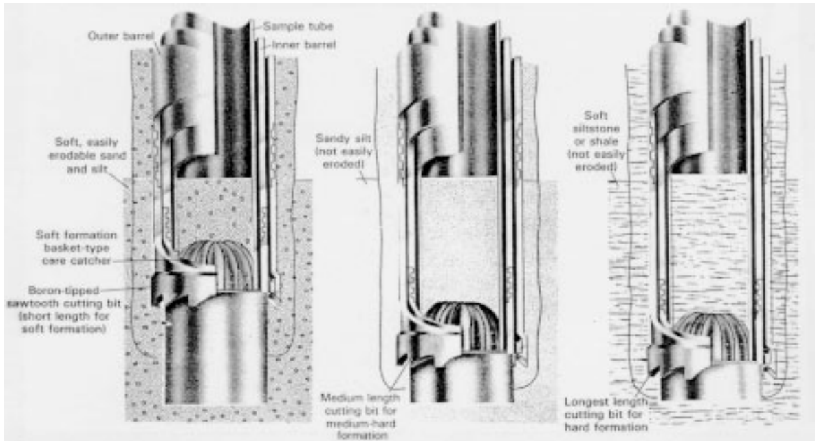
Figure 2-45.—Relationship of inner-barrel protrusion using different-length, Denison-sampler cutting bits for drilling.
