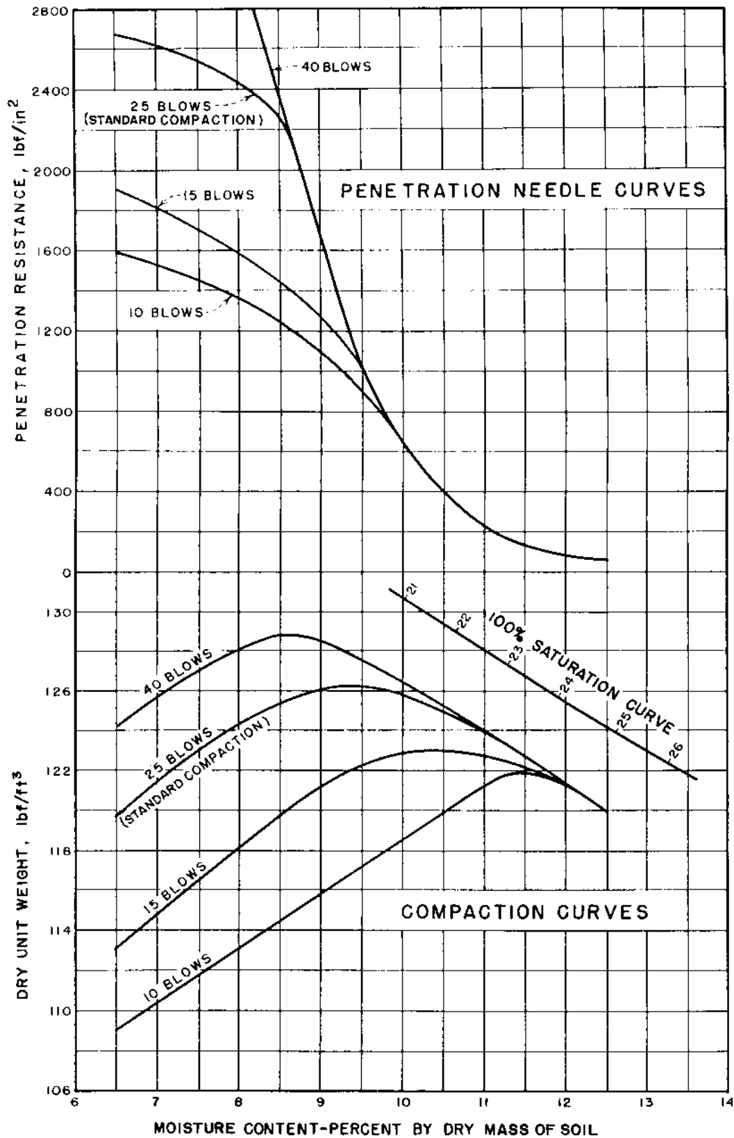
Figure 1-11.—Effect of compactive effort on the compaction and penetration-resistance curves.
