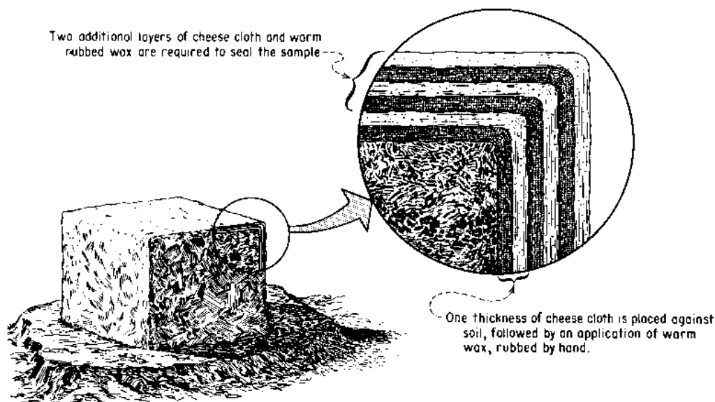
(A.) METHOD FOR SEALING HAND-CUT UNDISTURBED SAMPLES
