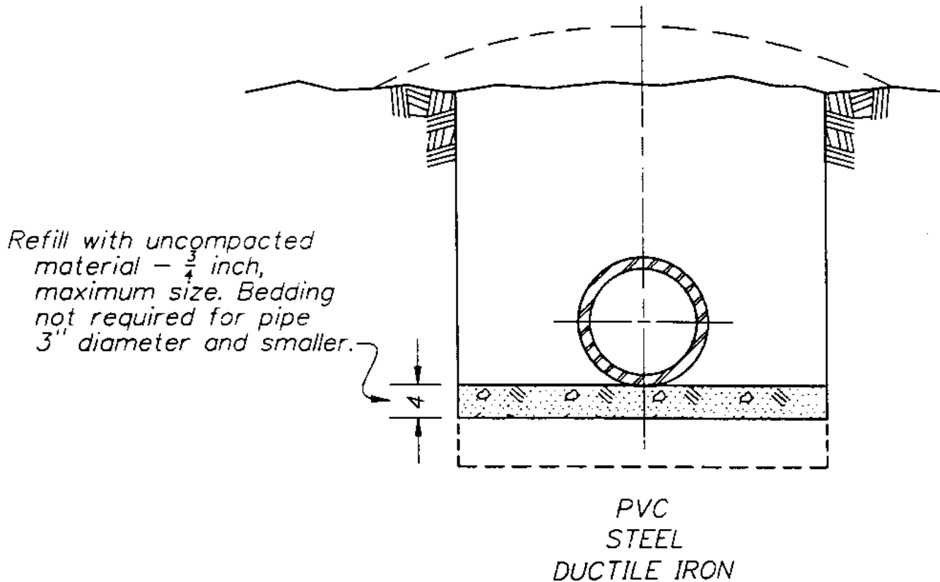
Figure 3-37.—Installation requirements of pipe 250-mm in diameter and smaller.
