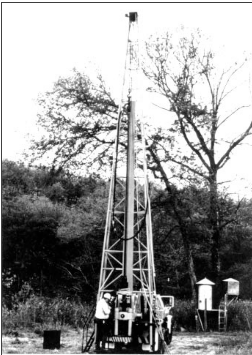
Figure 2-30.—Fluted Kelly drill setup. Automatic pull-down chuck assembly and breakout table.
