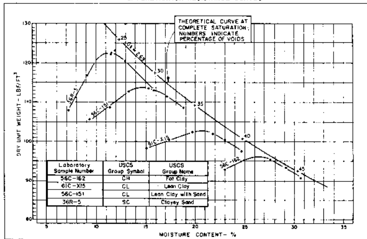
C. COMPACTION CURVES
