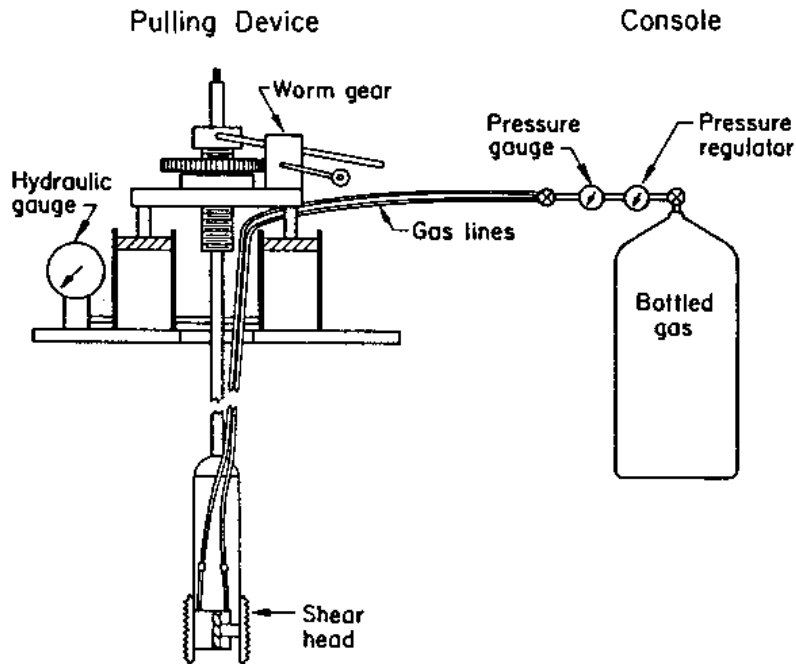
Figure 2-57.—Borehole shear device. (Wineland [61])
