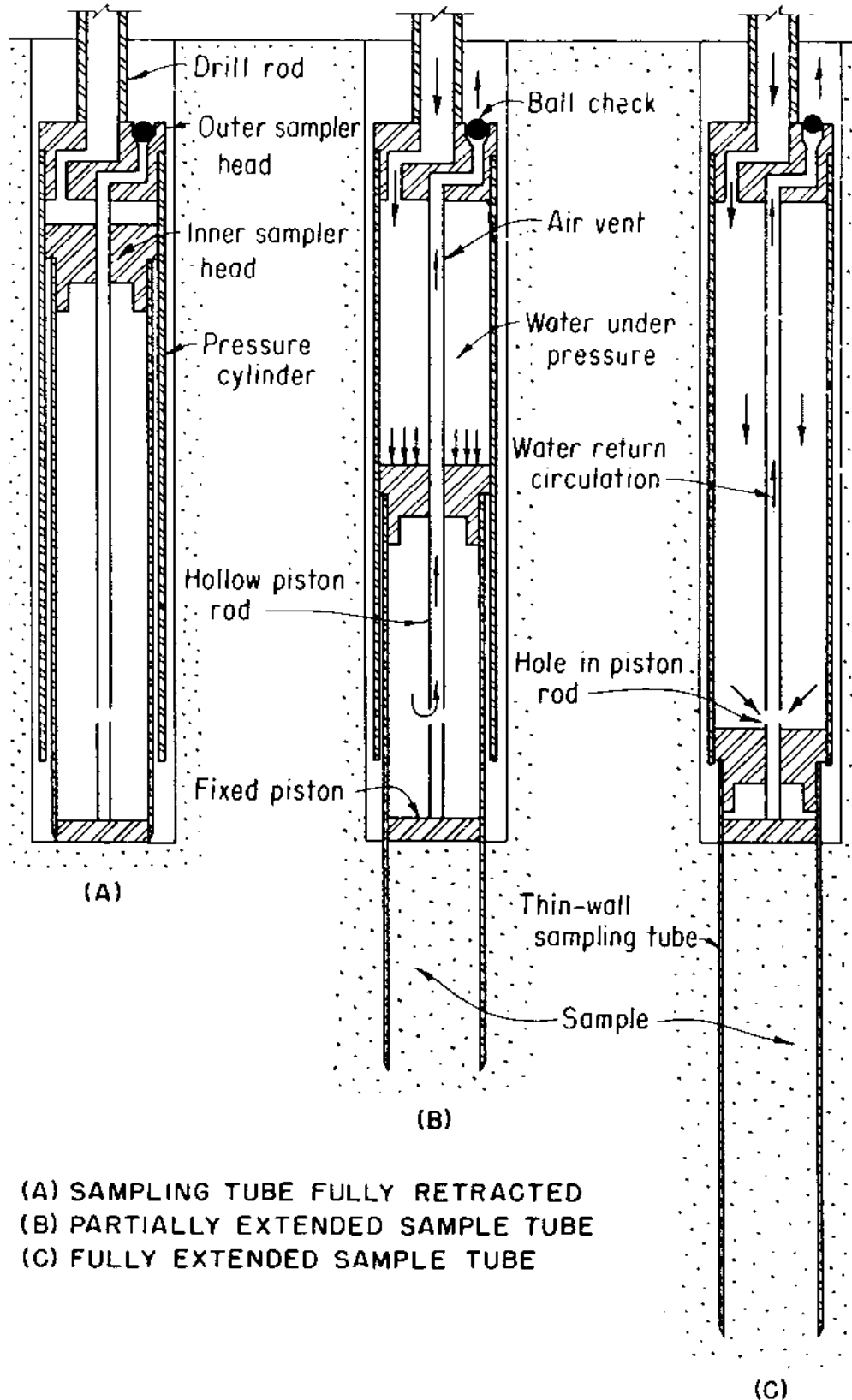
Figure 2-41.—Thinwall fixed-piston sampler (Osterberg type).
