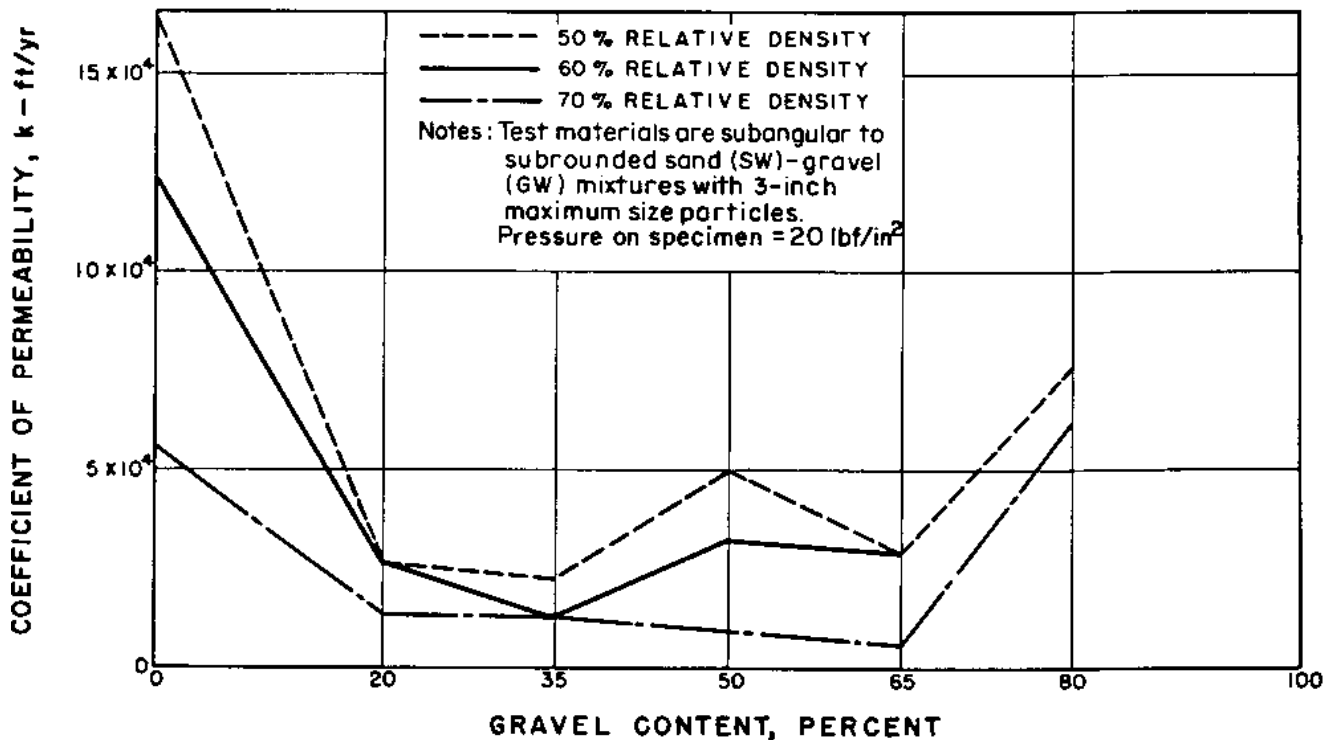
Figure 1-33.—Relationship of permeability to gravel content for specimens of various relative densities.
