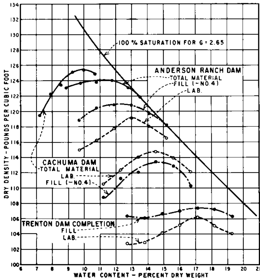
Figure 3-23.—Average field and laboratory compaction curves.
