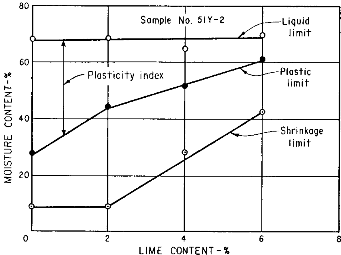
Figure 1-31.—Effect of lime on shrinkage limit, plastic limit, and liquid limit.
