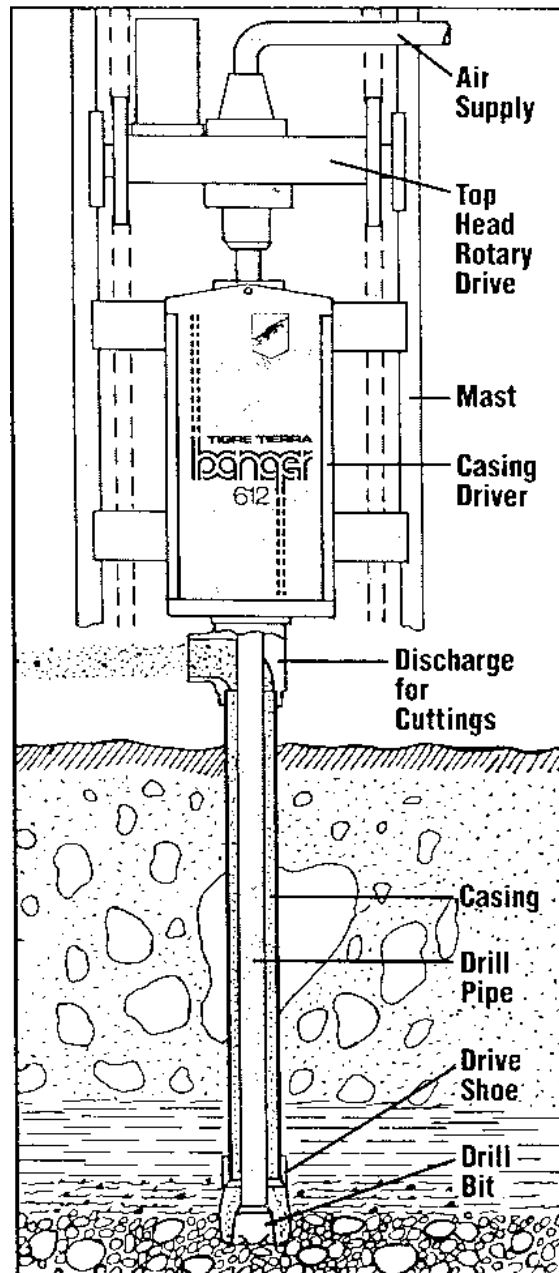
Figure 2-32. — Casing drivers can be fitted to top-head drive rotary rigs to simultaneously drill and drive casing. (Aardvark Corporation)
