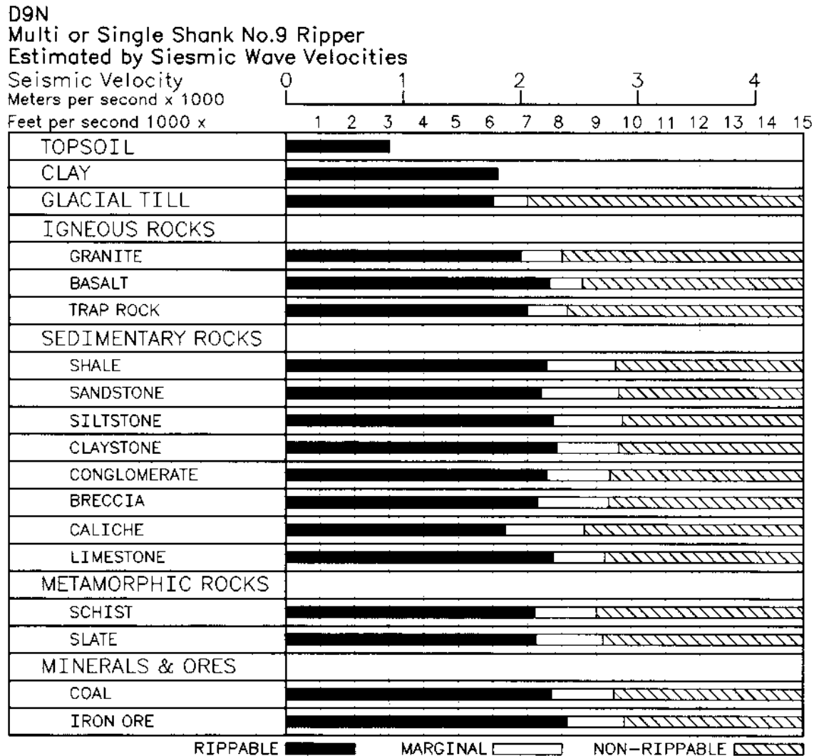
Figure 2-50.—Rock rippability as related to seismic P-wave velocities. (Caterpillar Tractor Co.)
