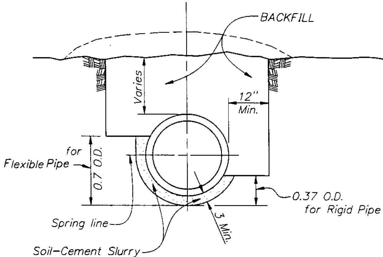
Figure 3-40.—Soil-cement slurry installation.
