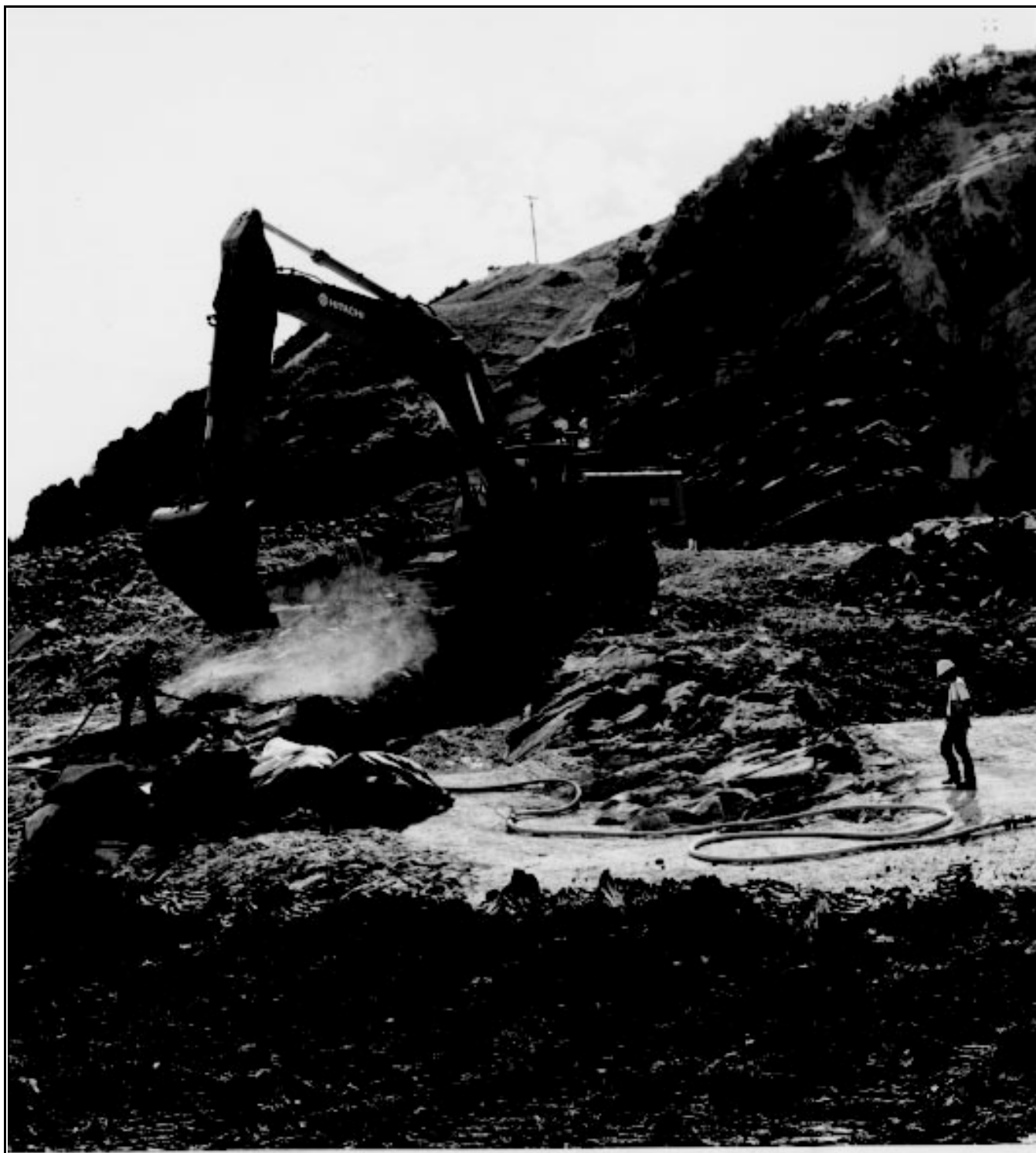
Figure 3-17.—Foundation preparation for the impervious (zone 1) foundation at Jordanelle Dam, Utah. The workman near the backhoe is using a high pressure mixture of air and water. The backhoe has a metal plate welded across its bucket teeth to provide a smooth edge for scraping. Inspector in right center, and impervious fill shown in foreground (July 1990).
