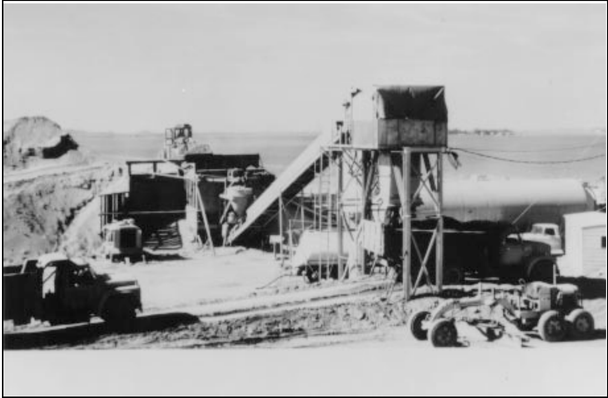
Figure 3-44.—Soil stockpile and pugmill for mixing soil-cement at Lubbock Regulating Reservoir in Texas.
