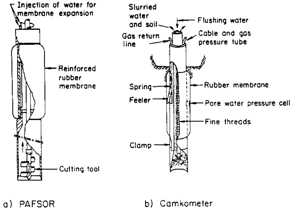
Figure 2-56. —Self-boring pressuremeters. (Jamiolkowski, Ladd, Germaine, and Lancellotta [60])
