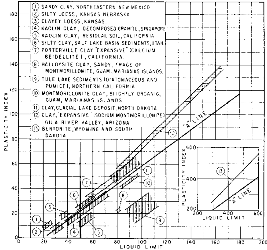
Figure 1-8.—Typical relationships between the liquid limit and the plasticity index for various soils.
