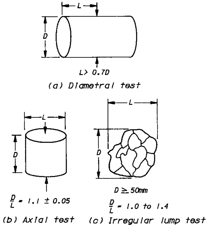
Figure 2-61.—Point-load strength testing variations (a) diametral test, (b) axial test, (c) irregular lump test.
