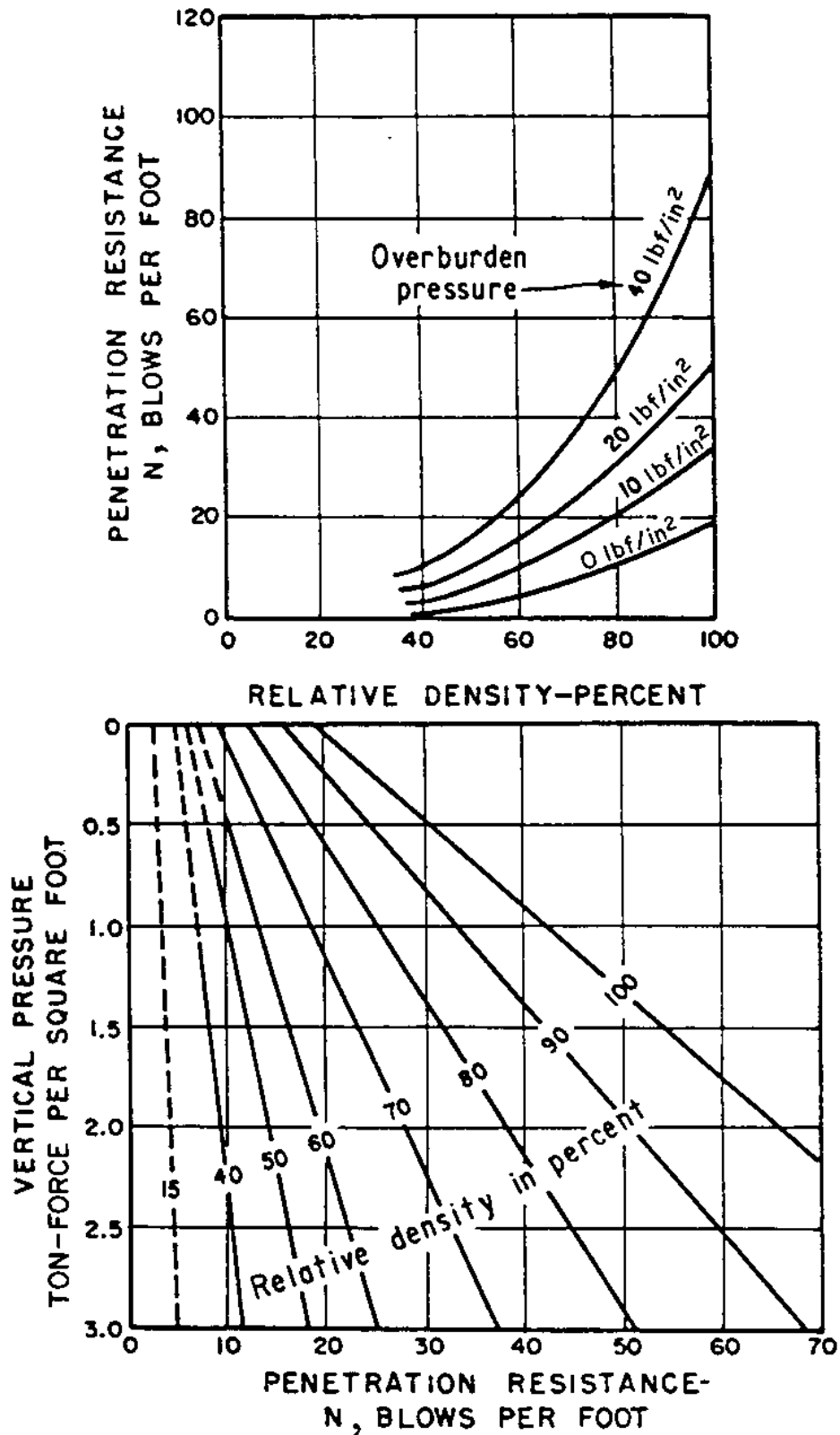
Figure 1-15.—Criterion for predicting relative density of sand from the penetration resistance test.
