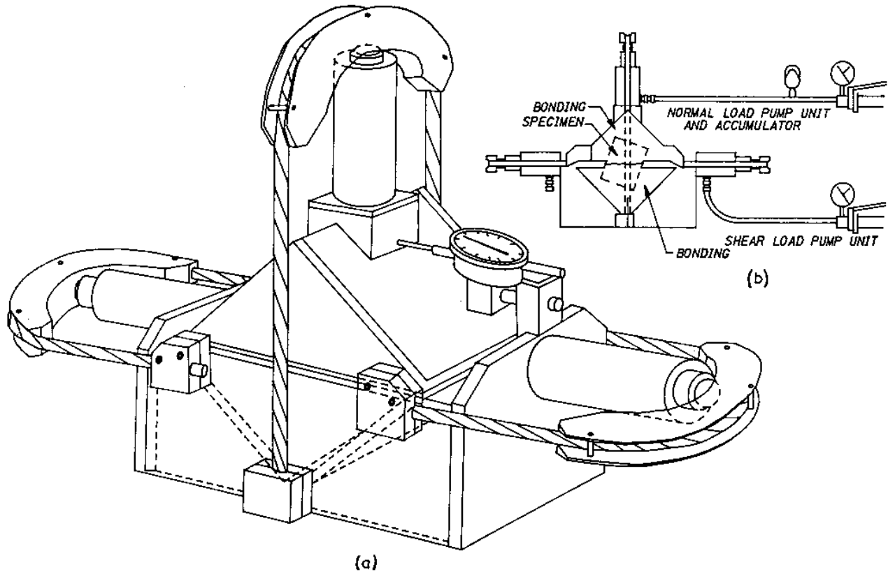
Figure 2-63.—Sketch of portable direct shear device.
