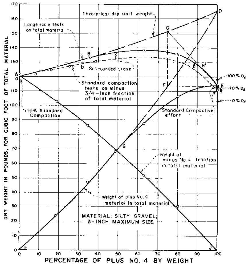
Figure 1-14.—Maximum dry unit weight versus gravel content for compacted soils.
