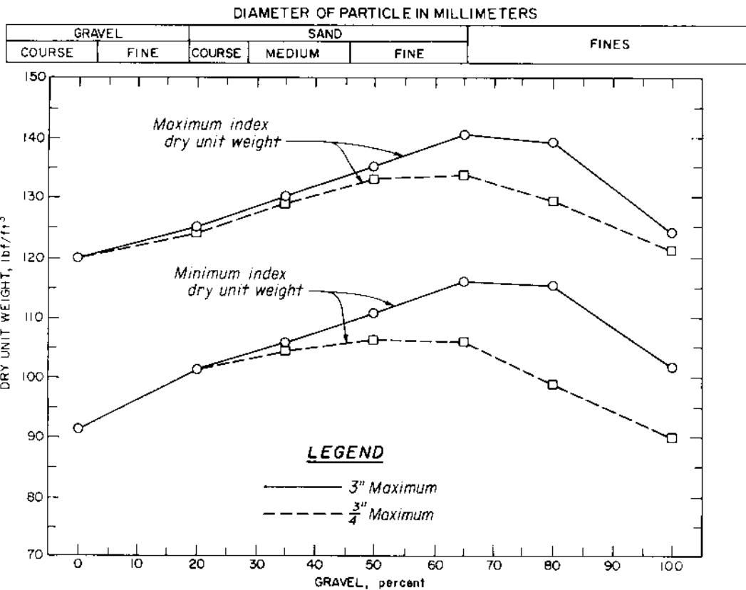
Figure 1-13.—Maximum and minimum index dry unit weights of typical sand and gravel soils [15].
