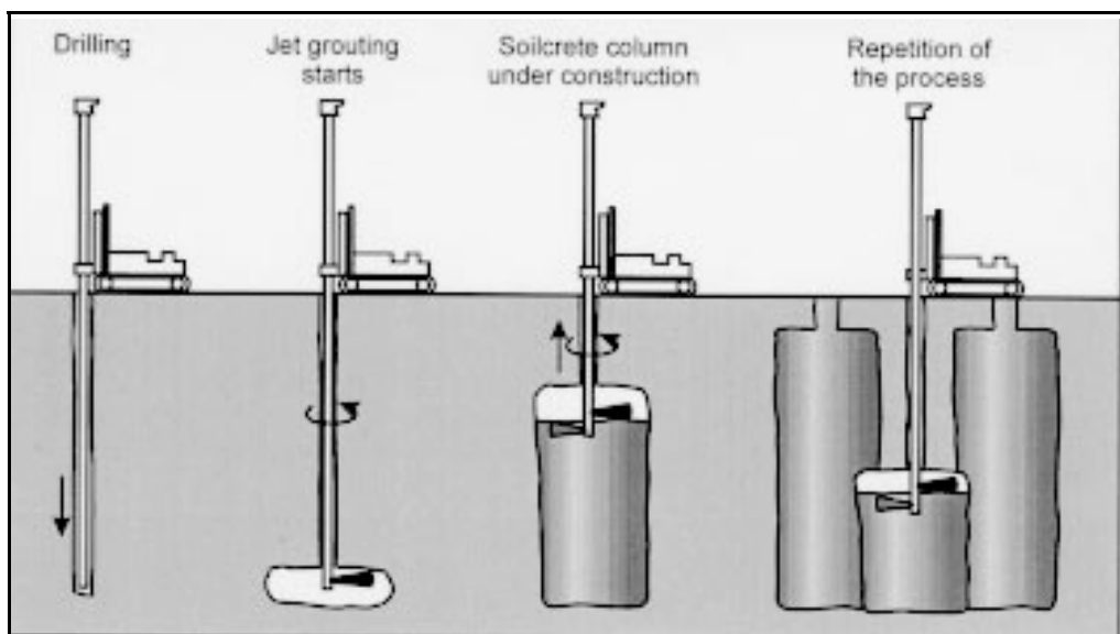
Figure 3-14.—Schematic drawing of jet grouting process showing construction of columns. (Hayward Baker, Inc.)
