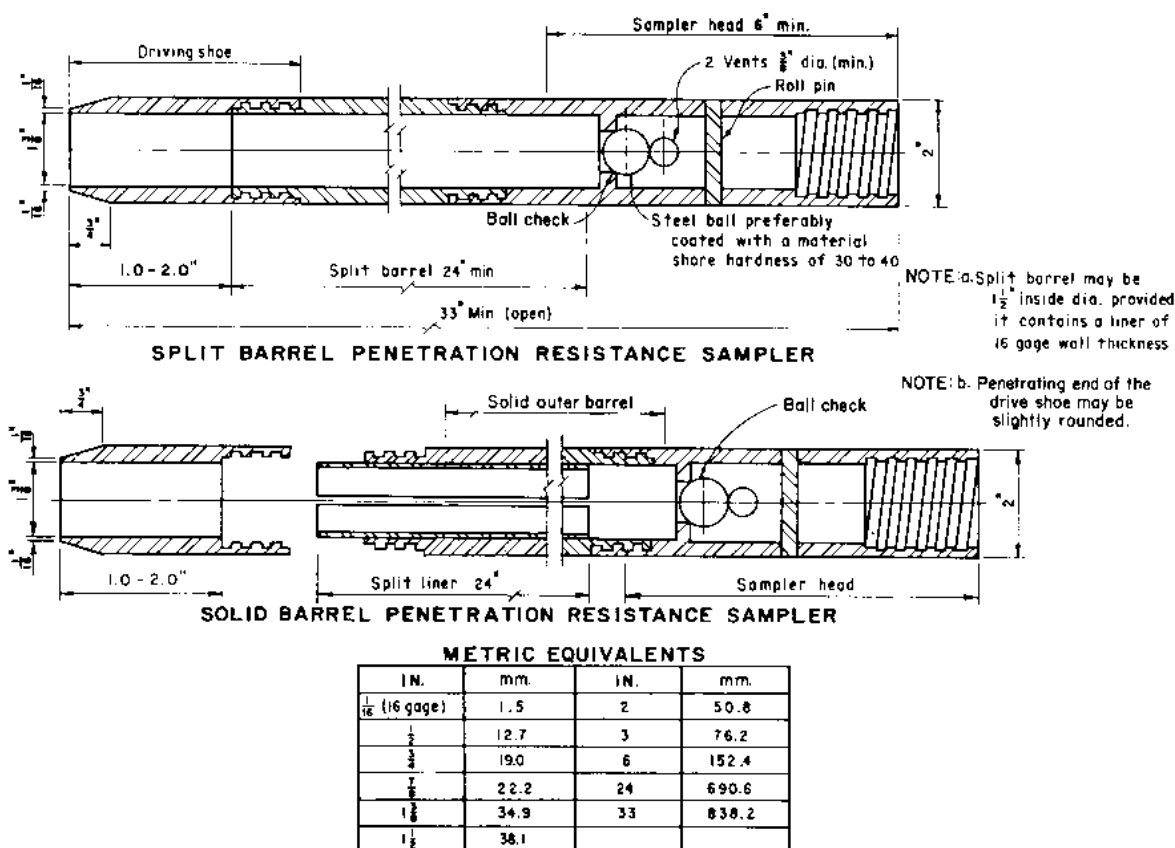
Figure 2-52.—Sampler requirements for penetration resistance testing.
