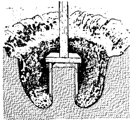
(B) Continue to drive sampler tube and excavate as shown. Core must be exercised to prevent breaking the core by filling the sampler tube.
