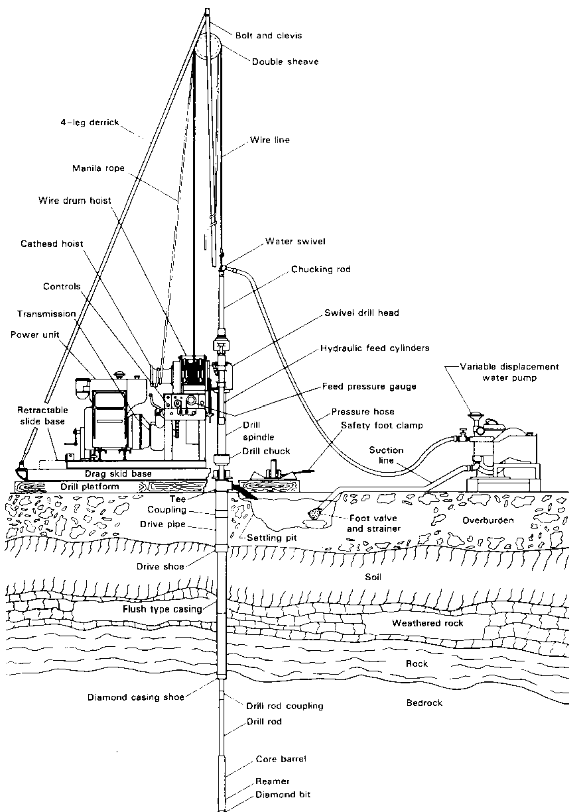
Figure 2-34.—Typical diamond drilling rig for exploration. (Acker Drill Co., Inc.)
