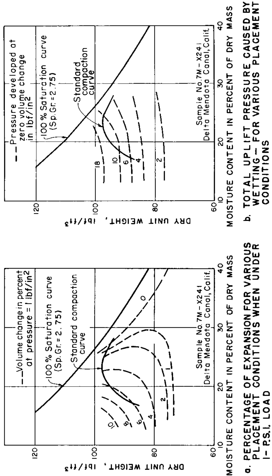
Figure 1-28. — Typical expansive clay. Effects of placement moisture content and dry unit weight on expansion characteristics [40].
