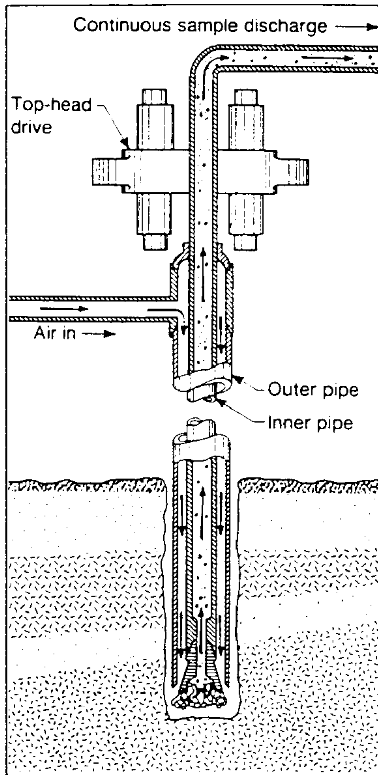
Figure 2-31.—Dual-wall reverse-circulation method.
