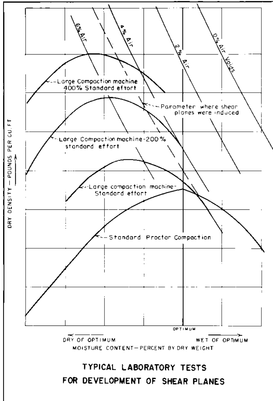
Figure 3-29.—Typical laboratory tests for the development of shear planes.
