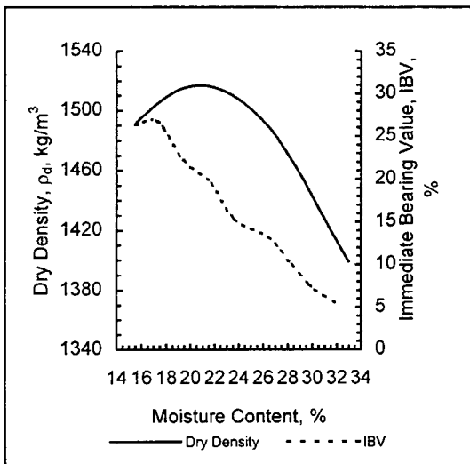
SC with 5% LKD
