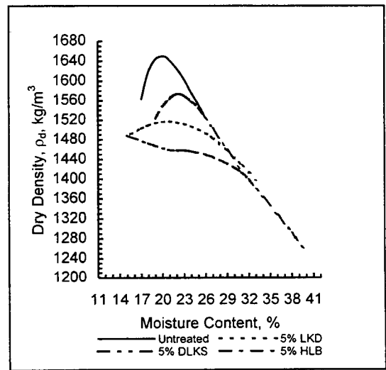
SC Density
