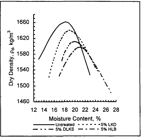
SiCL Density
