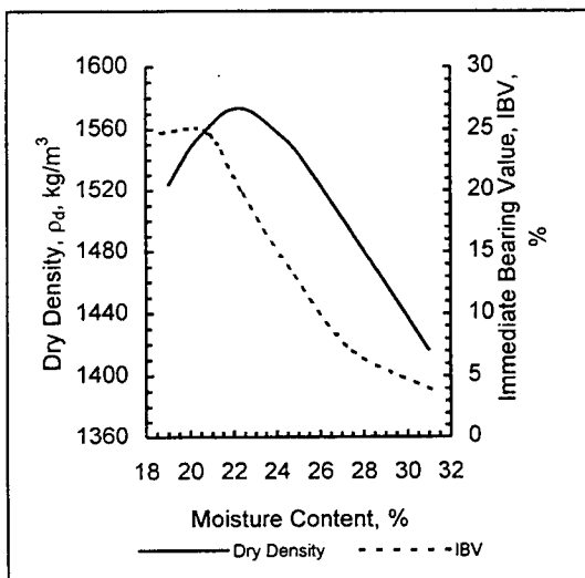
SC with 5% DLKS
