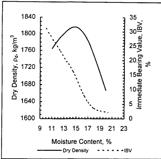
Untreated Clay
