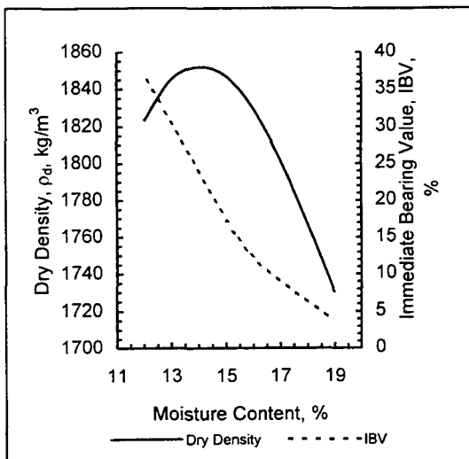
CL with 3% HLB
