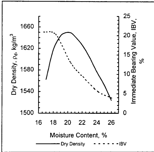
Untreated SC
