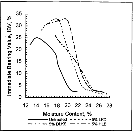
SiCL IBV
