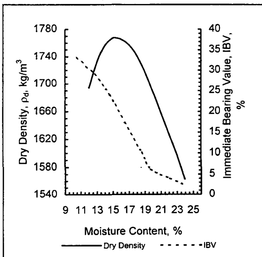
Clay with 5% DLKS
