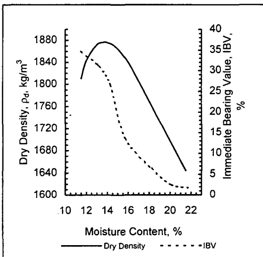
CL with 5% DLKS
