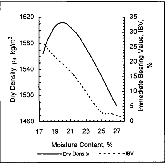
SiCL with 5% DLKS
