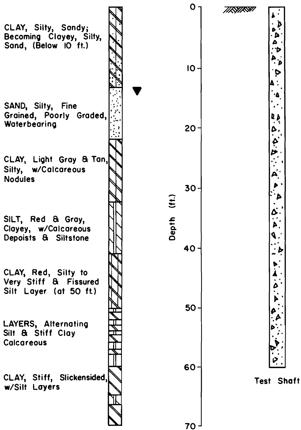
Fig. 4. Soil and shaft profile, HB & T test site (Site IV) (After Barker and Reese, 1970).
